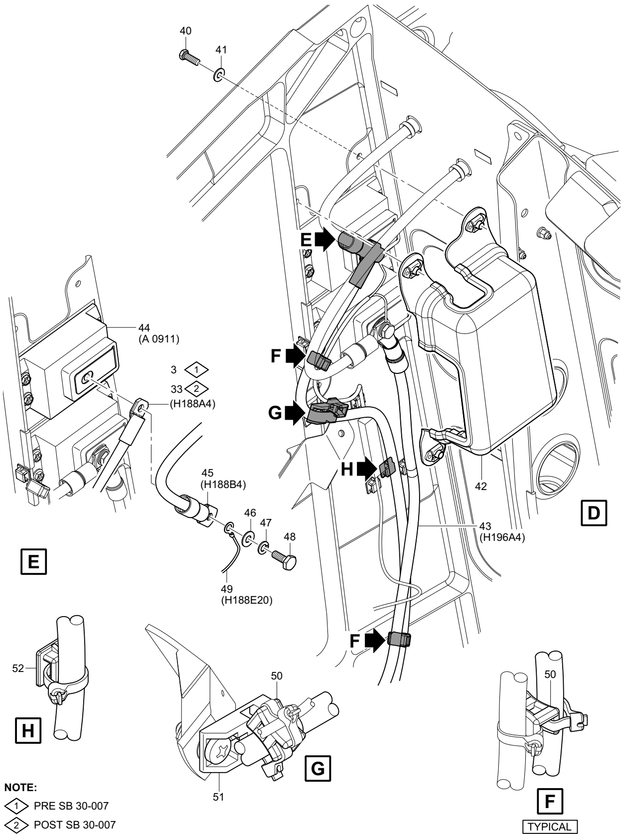
MSN 101 thru MSN 337 - Replace the LH Solid State Relay Figure 1 (Sheet 5 of 9)
