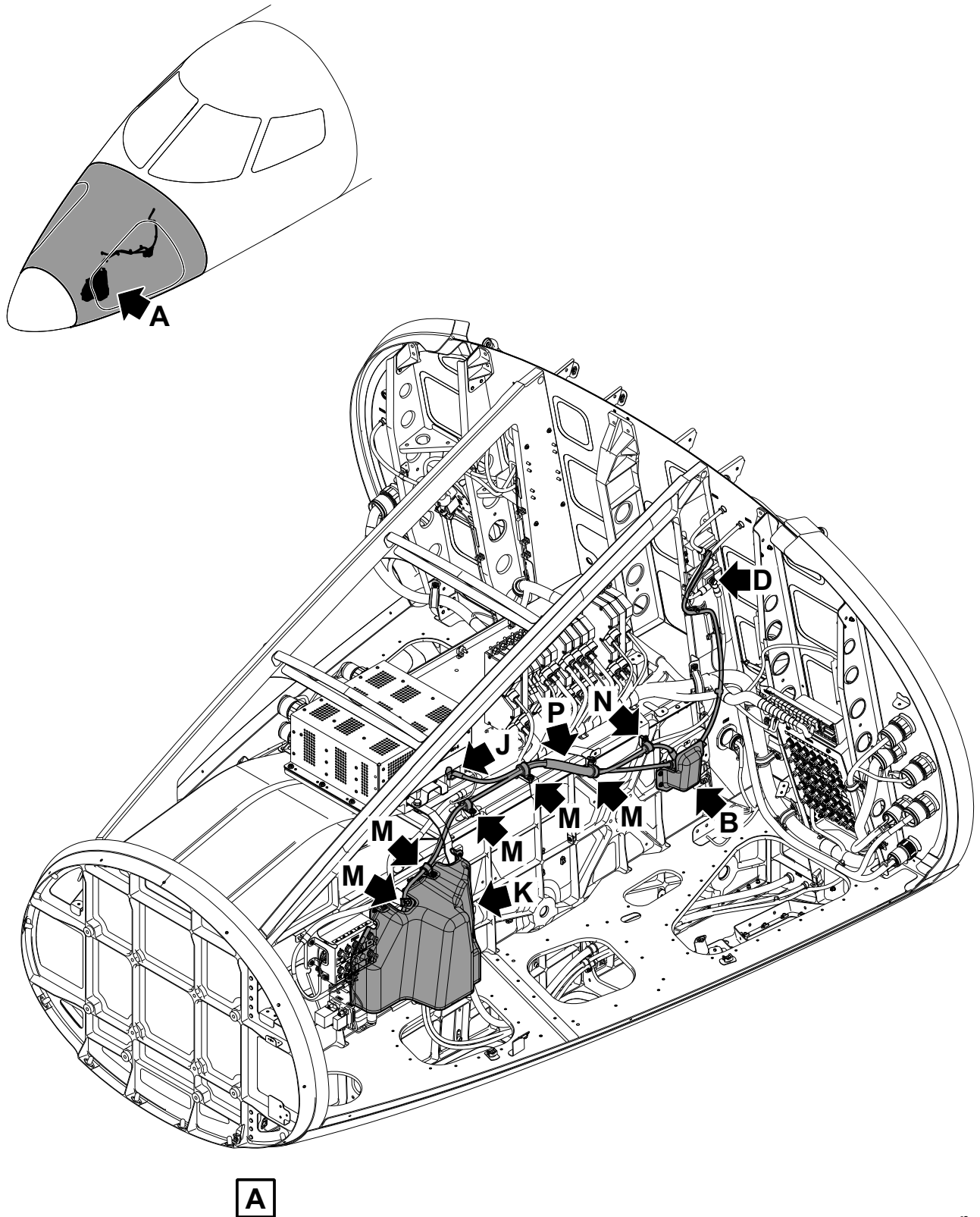
MSN 101 thru MSN 337 - Replace the LH Solid State Relay Figure 1 (Sheet 1 of 9)
