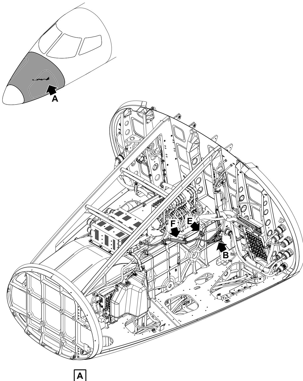
MSN 501 thru MSN 590 - Replace the LH Solid State Relay Figure 2 (Sheet 1 of 5)
