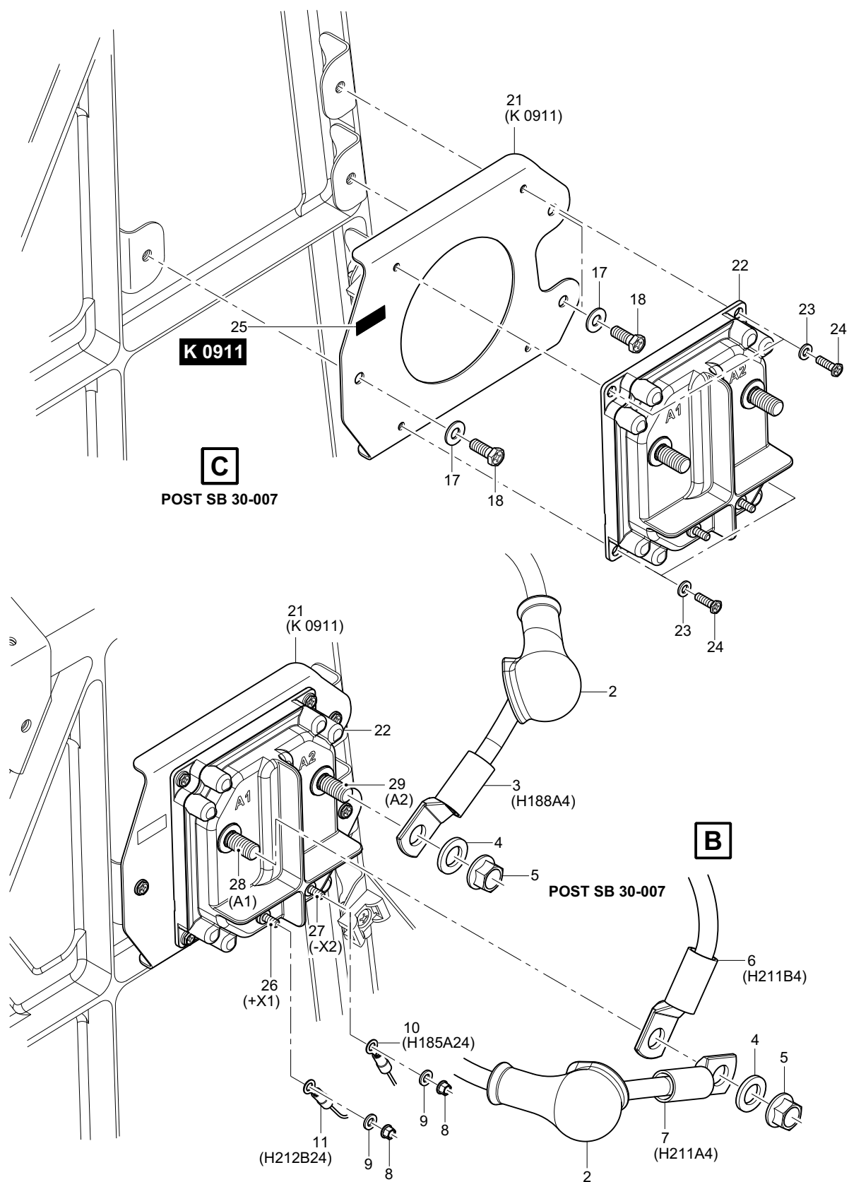
MSN 501 thru MSN 590 - Replace the LH Solid State Relay Figure 2 (Sheet 4 of 5)
