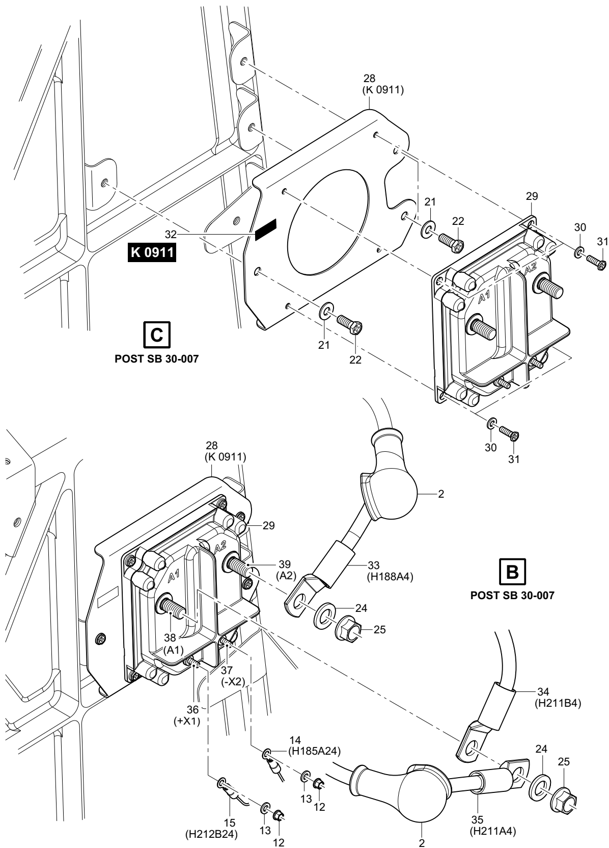
MSN 101 thru MSN 337 - Replace the LH Solid State Relay Figure 1 (Sheet 4 of 9)
