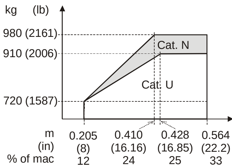
Figure 6-2 Use of Weight and Balance Diagram
