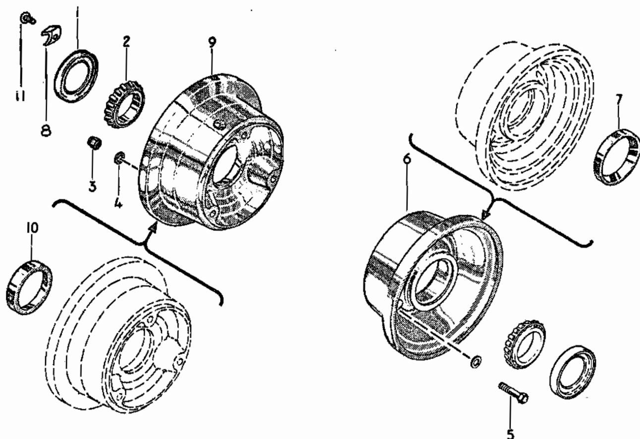
Figure 4 Nosewheel Assembly 9532186
