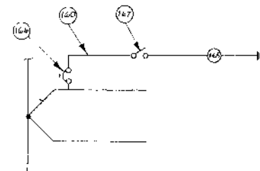
INSTALLATION OF MARKER BEACON RECEIVER OFF SHIP'S BUS BAR
