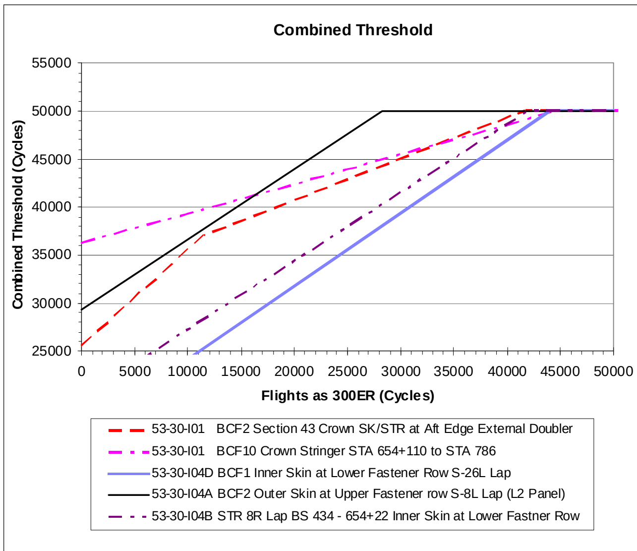
FIGURE 2. Combined Passenger and Freight Life Threshold
