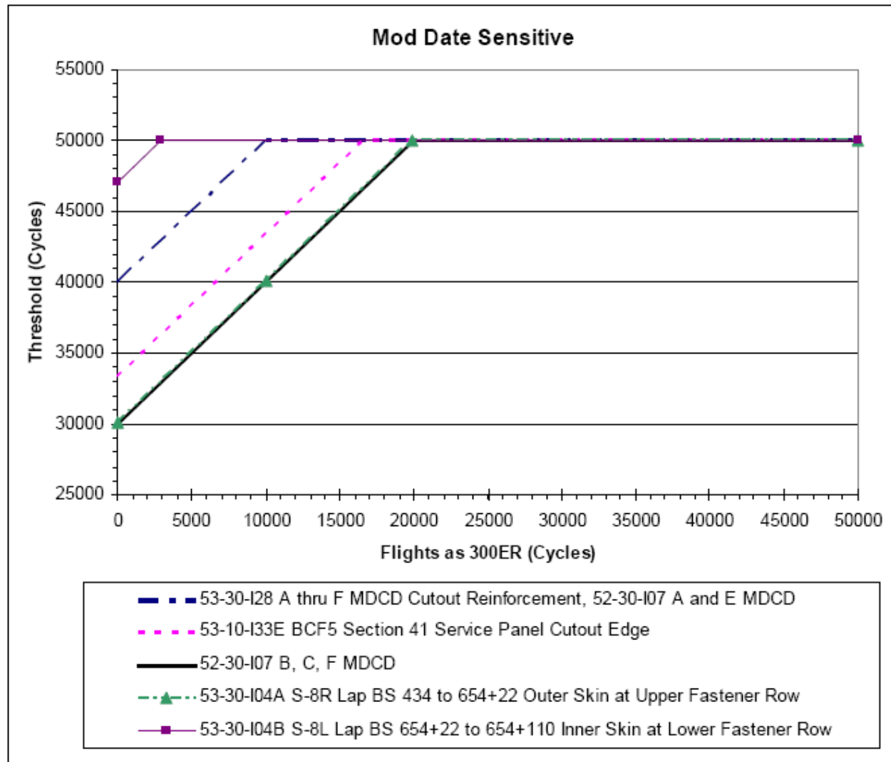
FIGURE 3. Mod Date Sensitive Structure
