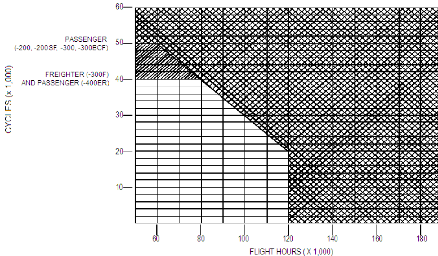
FIGURE 1. FLIGHT LENGTH SENSITIVE (FLS) THRESHOLD CURVE
