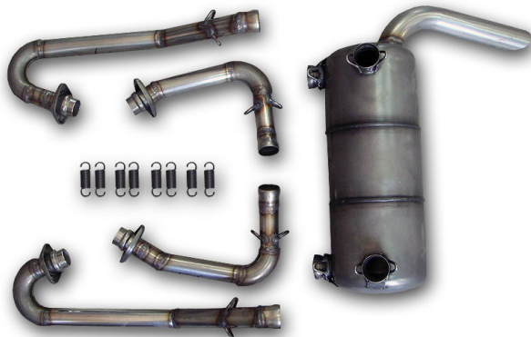
NAME: Exhaust system (80 hp, a set) PART NO.: A22LS-03-756 WEIGHT: 4.4 kg PRICE:
