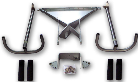
NAME: Yokes with control column (a set) PART NO.: A22LS-05-001 WEIGHT: 3.5 kg PRICE:
