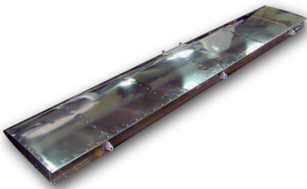
NAME: Stabilizer, not painted PART NO.: A22LS-01-300 WEIGHT: 6.3 kg PRICE:
