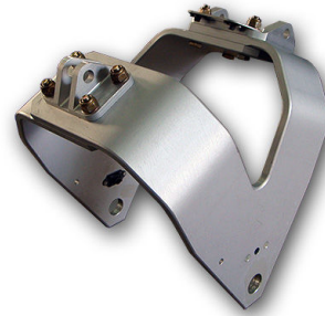
NAME: Nose wheel fork PART NO.: A22LS-02-002 WEIGHT: 2.15 kg PRICE:
