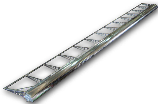
NAME: Flaperon, not covered PART NO.: A22LS-01-152 R A22LS-01-152 L WEIGHT: 3.3 kg PRICE:
