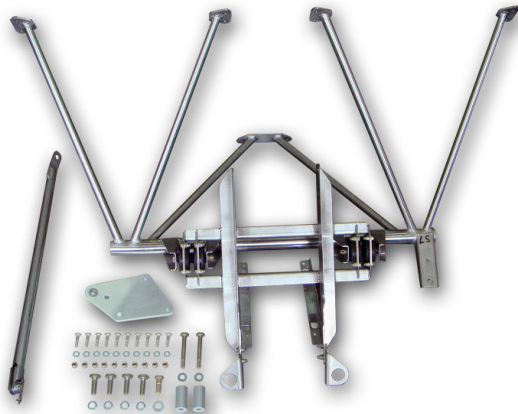
NAME: Engine mount (a set) PART NO.: A22LS-03-001 WEIGHT: 4.9 kg PRICE:
