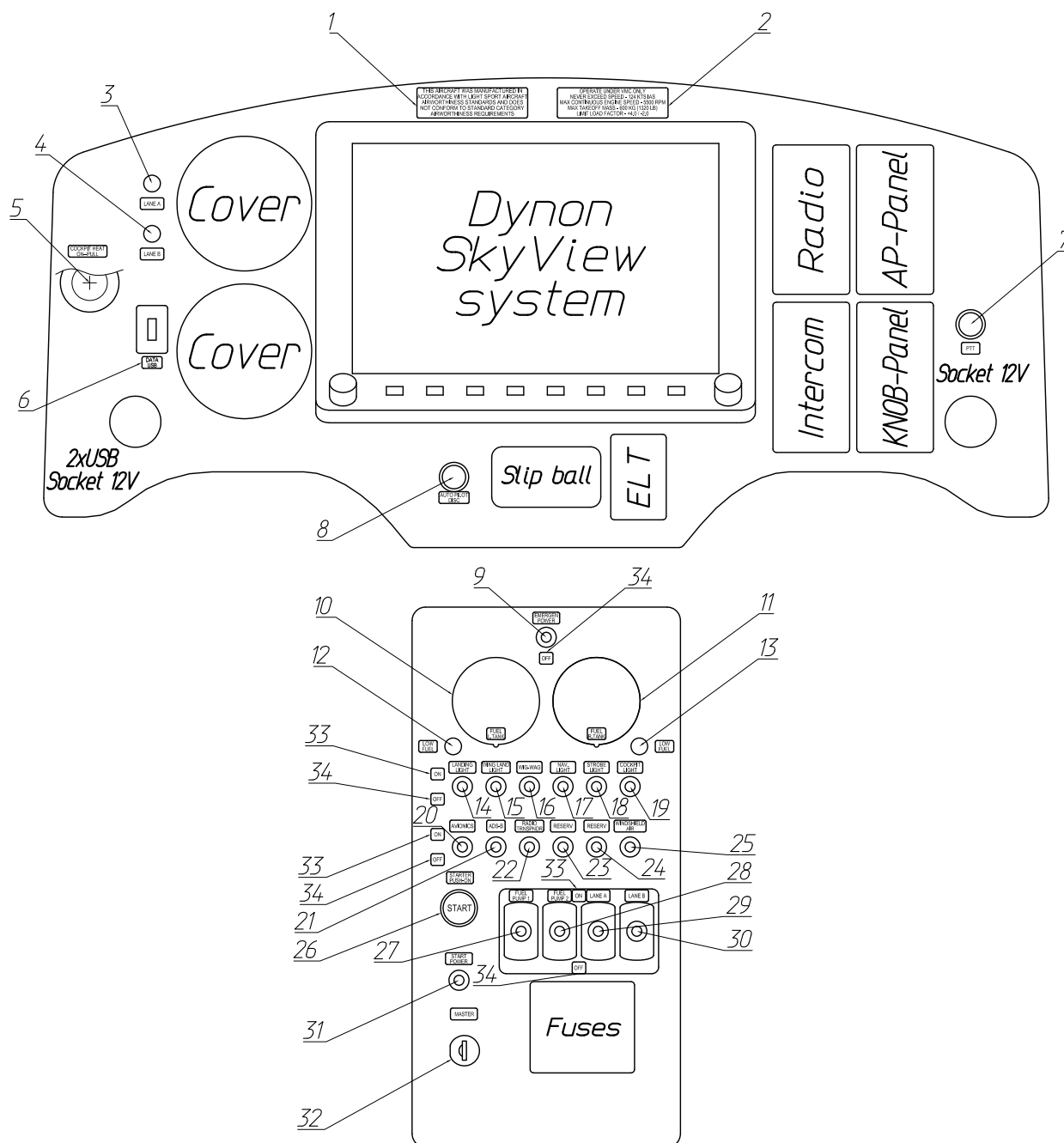
Fig. 11 Instrument panel
