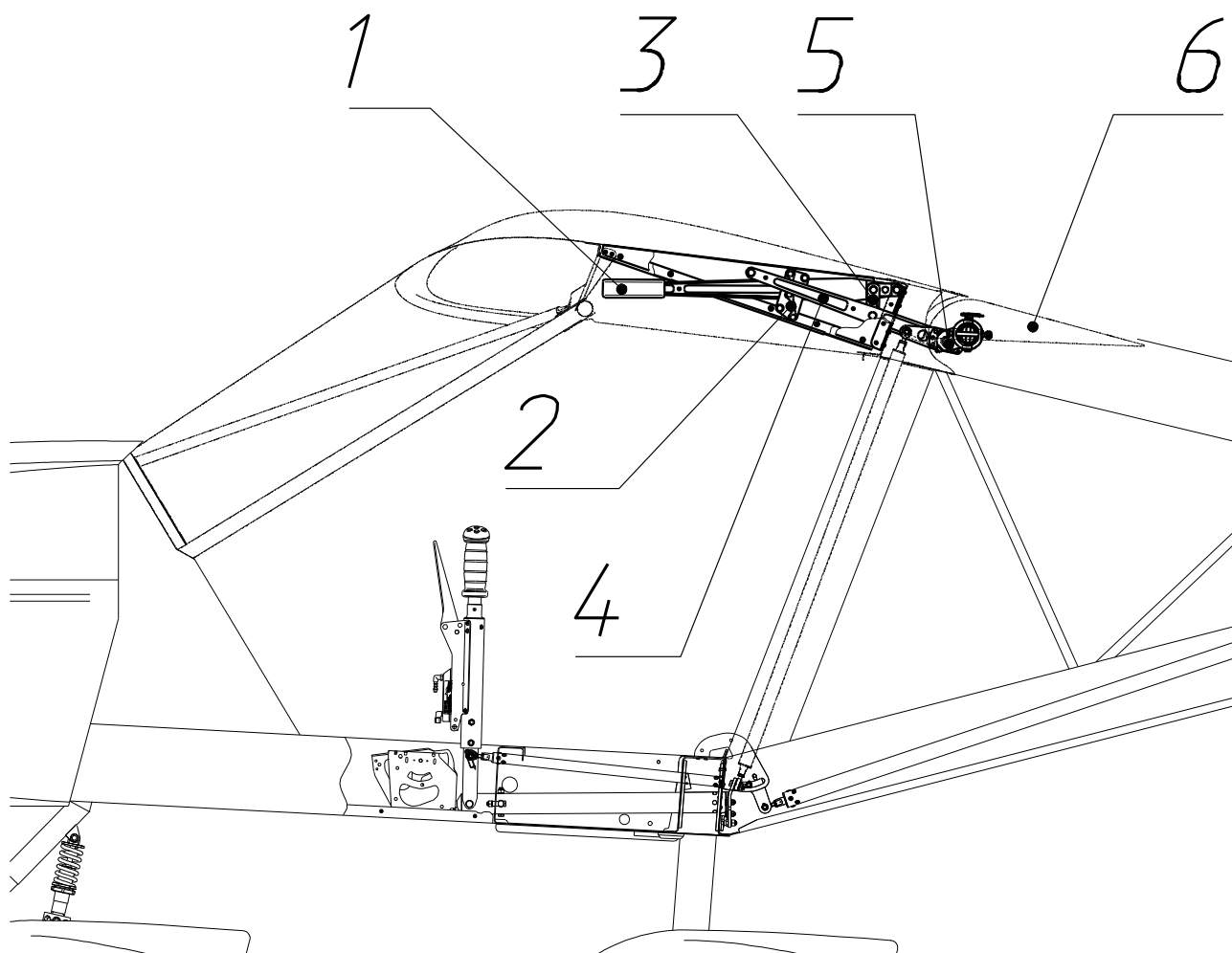
Fig. 8. Flap extension mechanism
