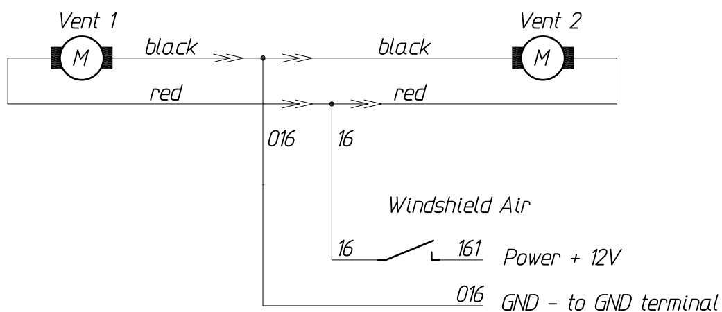
Fig. 18. Wiring diagram for installation of the windshield air fans
