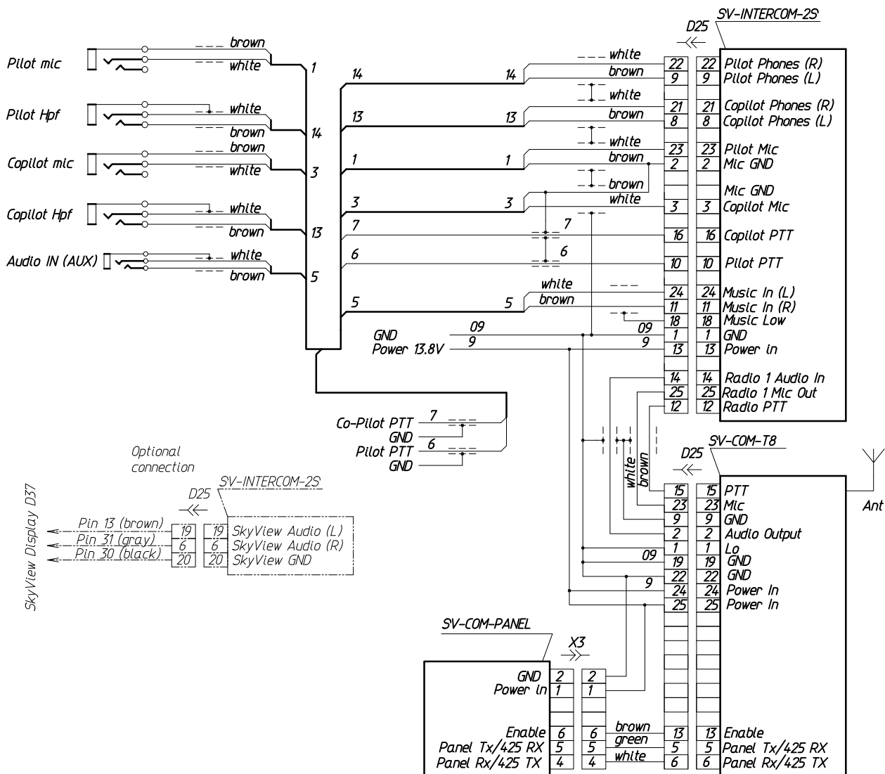
Fig. 17. Wiring diagram for installation of the SV-COM radio
