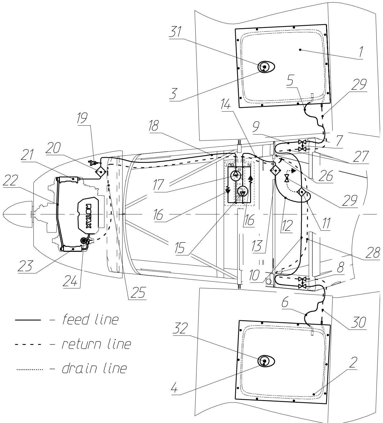
Fig. 3. Fuel system schematic
