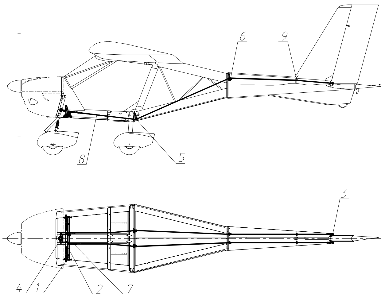
Fig. 6. Rudder and nose landing gear control system
