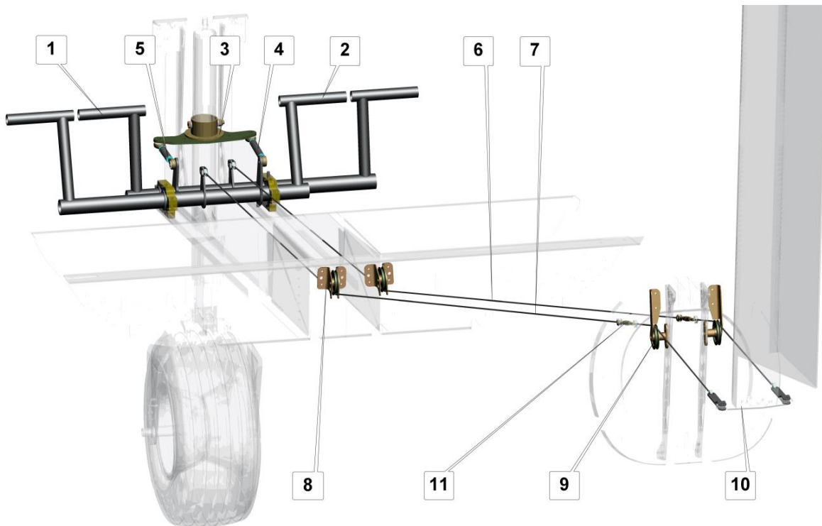
Fig. 6. Rudder and nose landing gear control system
