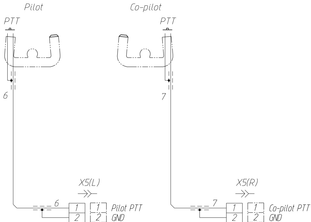
Fig. 20 Wiring diagram for installation PTT buttons
