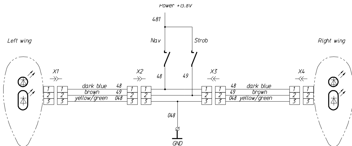
Fig. 15 Wiring diagram for installation of strob and navigation lights
