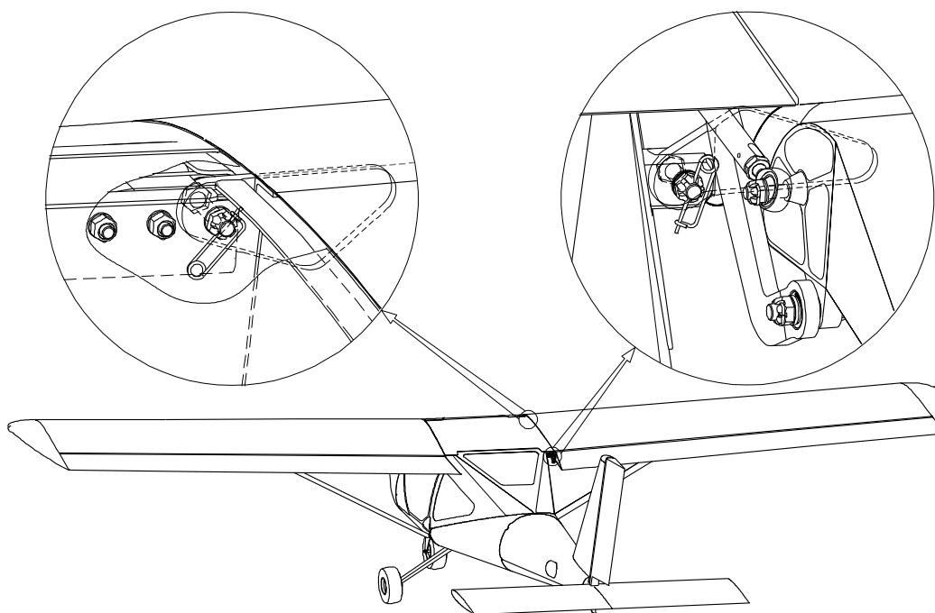
Fig. 22 Wing removal – wing-to-fuselage attachment points
