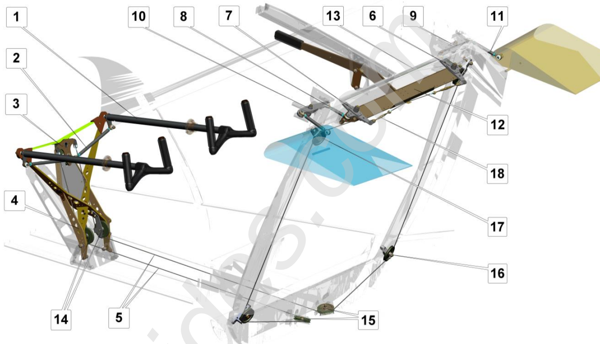
Fig. 7. Control system of flaperons (drooping ailerons)
