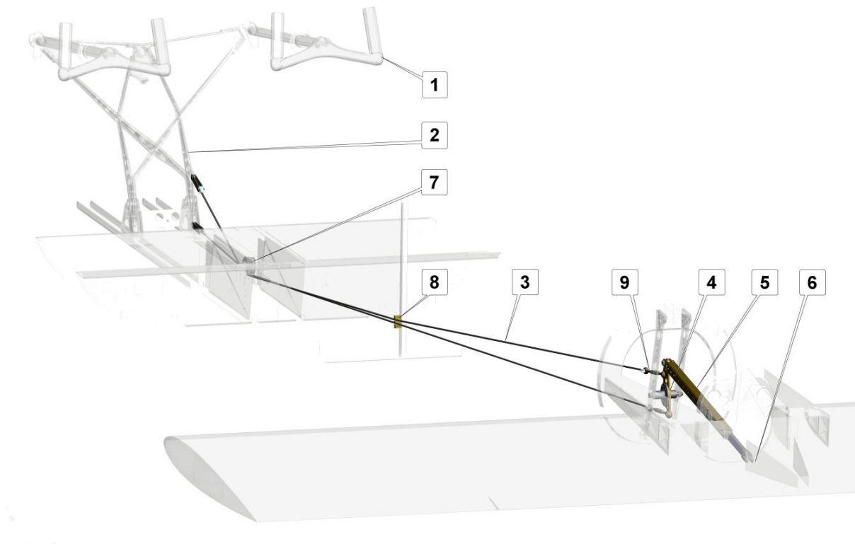
Fig. 4 AFHT control system
