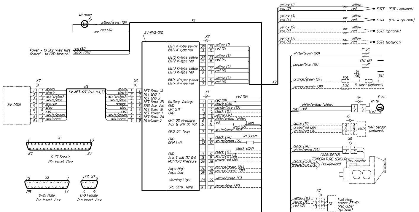
Fig. 17. Wiring diagram for installation of SV-EMS-220
