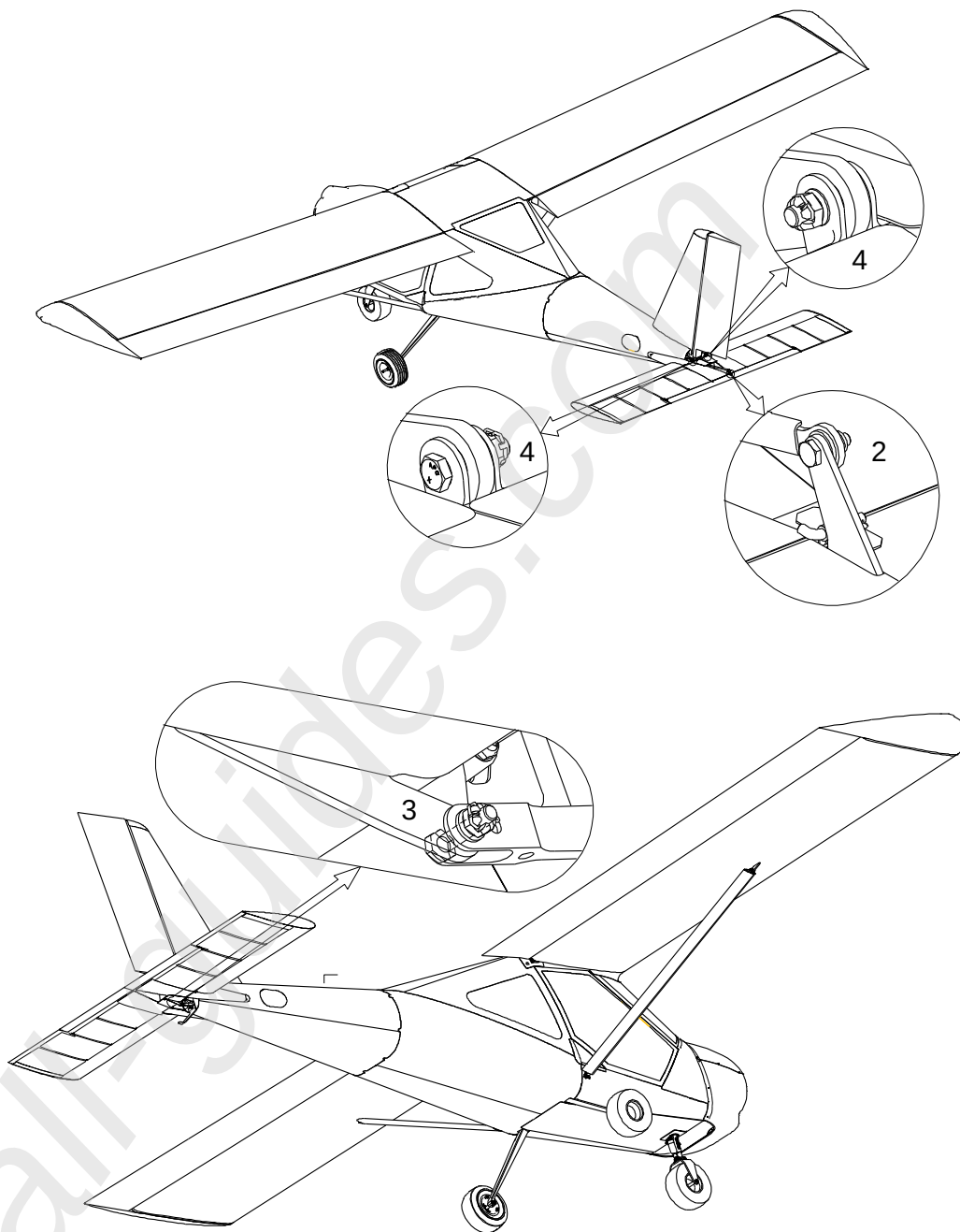
Fig. 24 Removal of the AFHT
