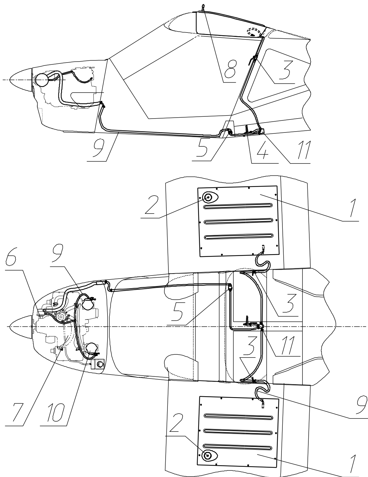
Fig. 3. Fuel system schematic
