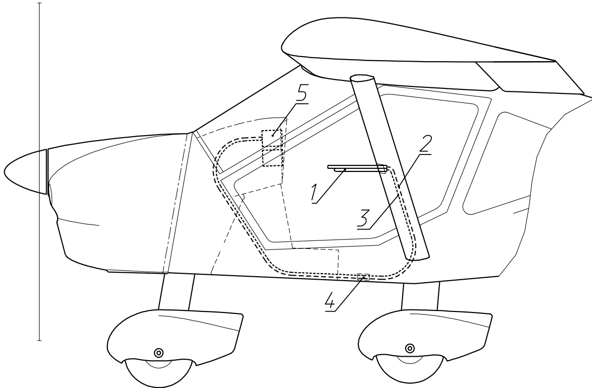
Fig. 14 Full and static pressure system
