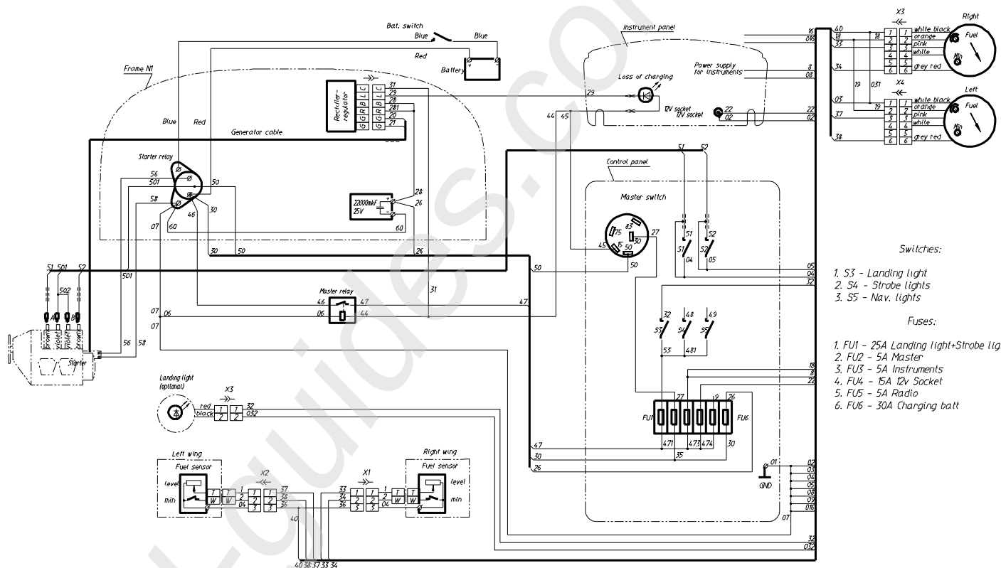
Fig. 16 Wiring diagram of A-32 electrical system (main)
