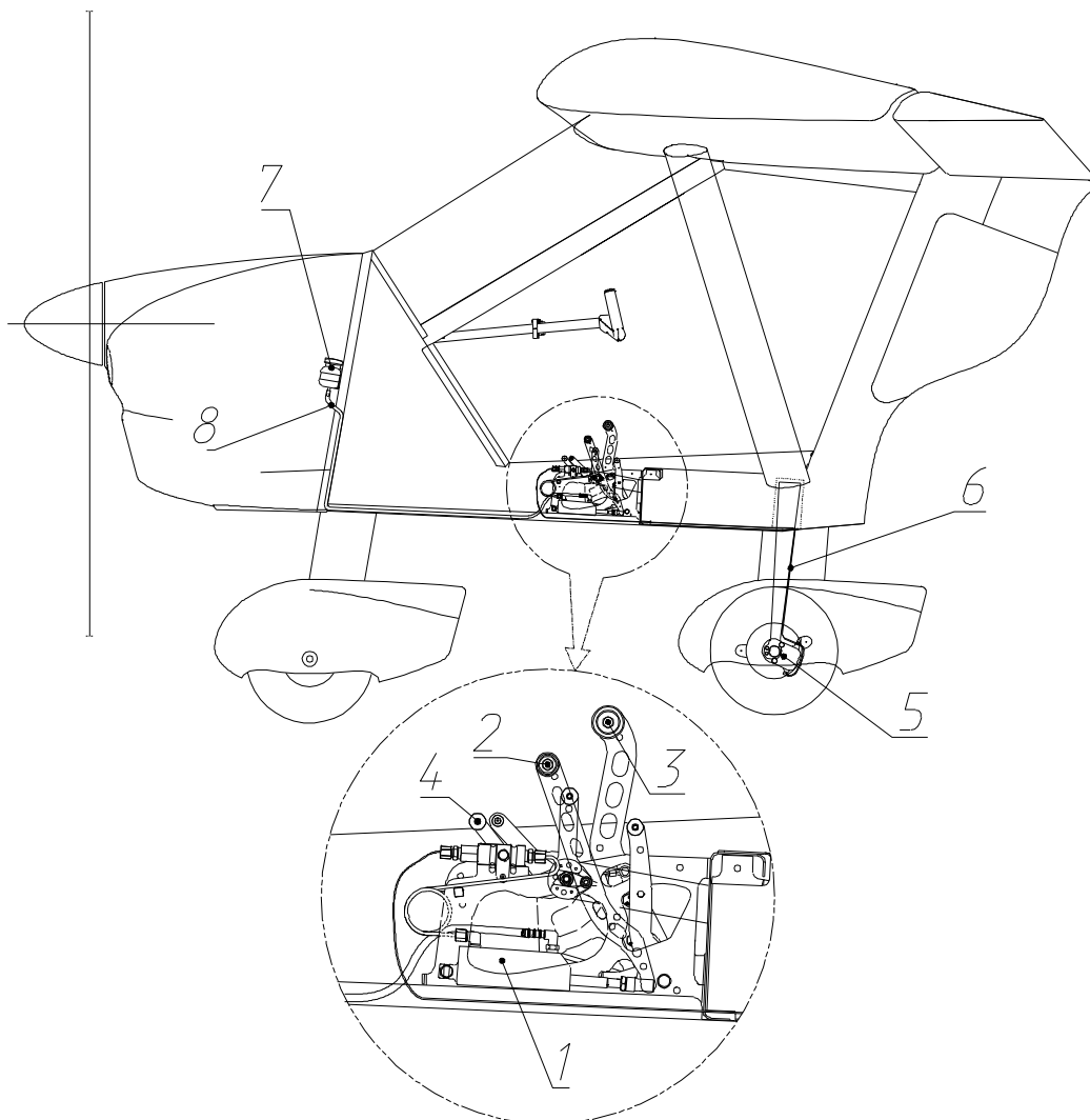
Fig. 12. Brake control system
