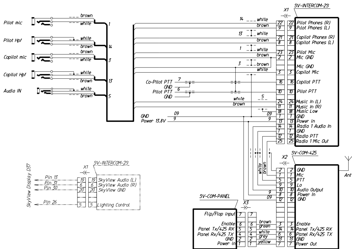
Fig. 19 Wiring diagram for Dynon SkyView radio
