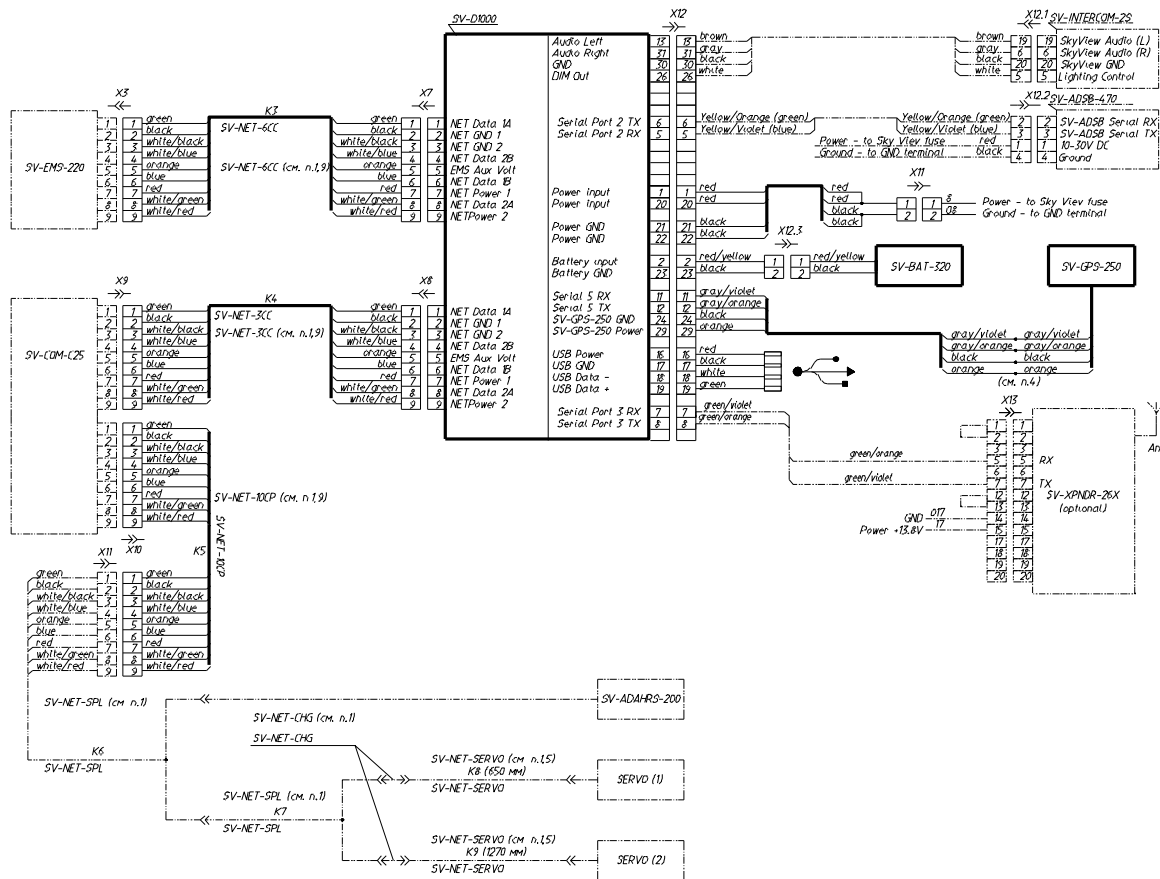
Fig. 18. Wiring diagram for installation of SV-D1000, SV-GPS-250, SV-BAT-320, SV-ADAHRS-200
