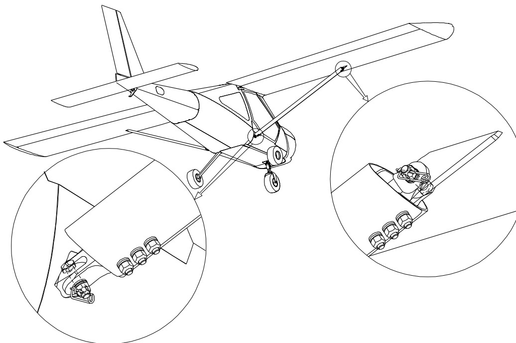
Fig. 23 Wing removal – wing strut attachment points
