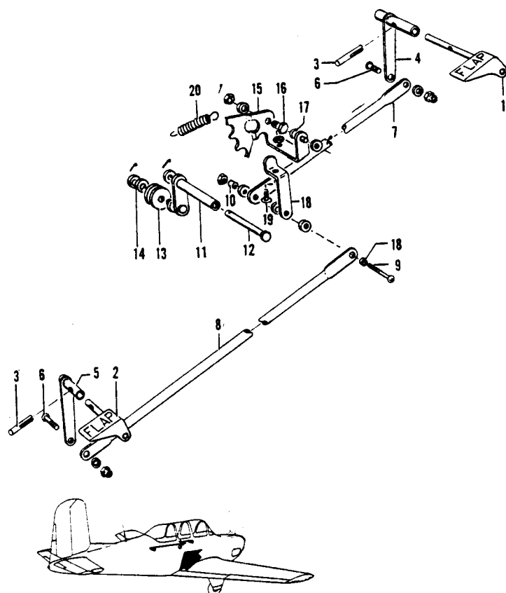
Figure 37. Flap Switch Control Installation
