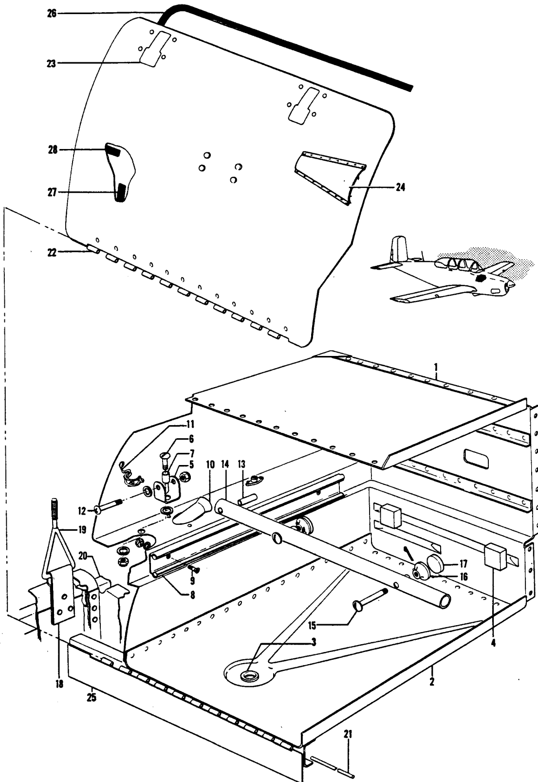
Figure 31. Battery Box Installation
