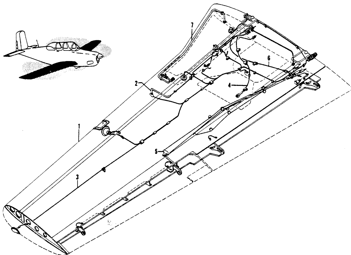
Figure 3. Wing Assembly
