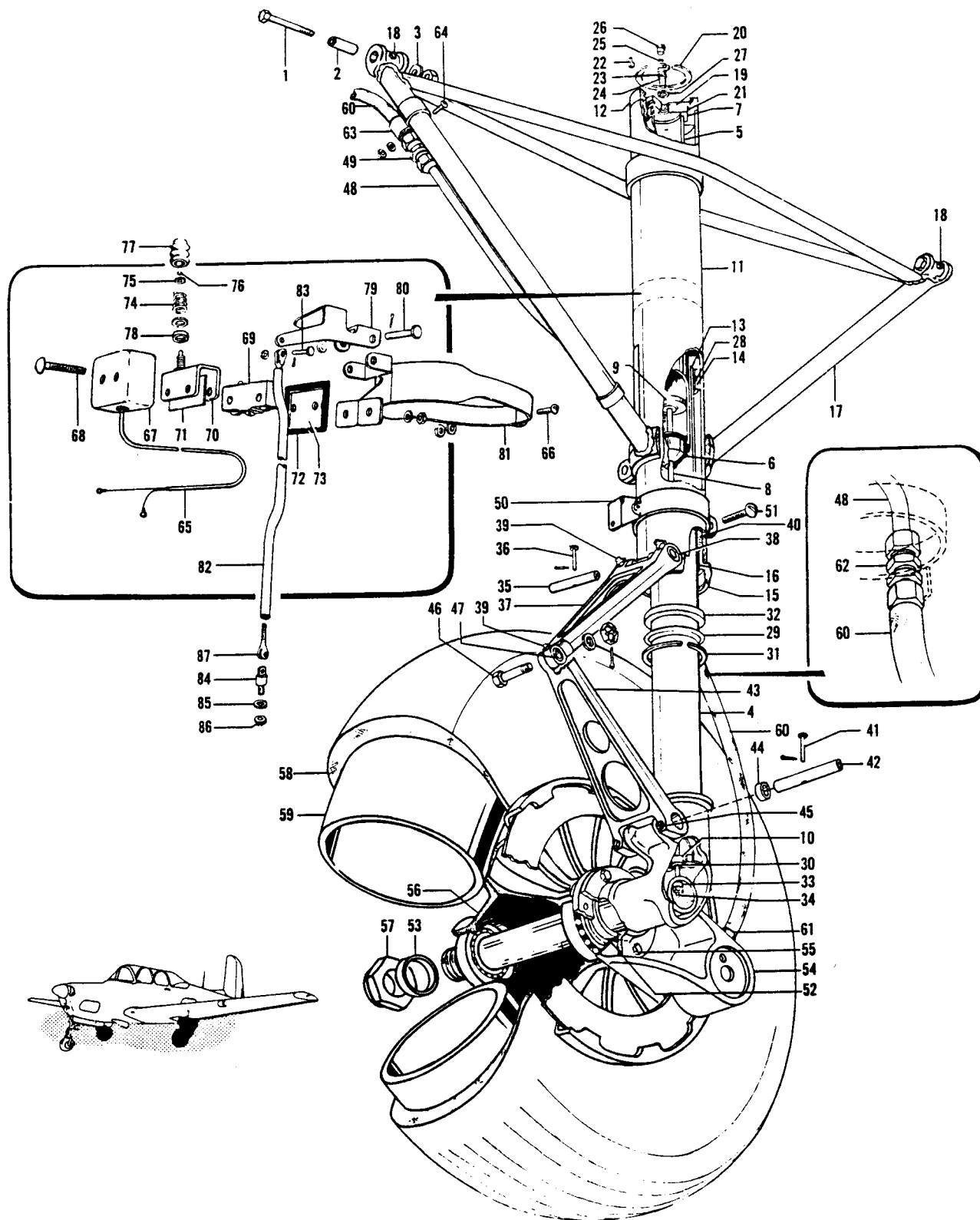
Figure 70. Main Alighting Gear Installation
