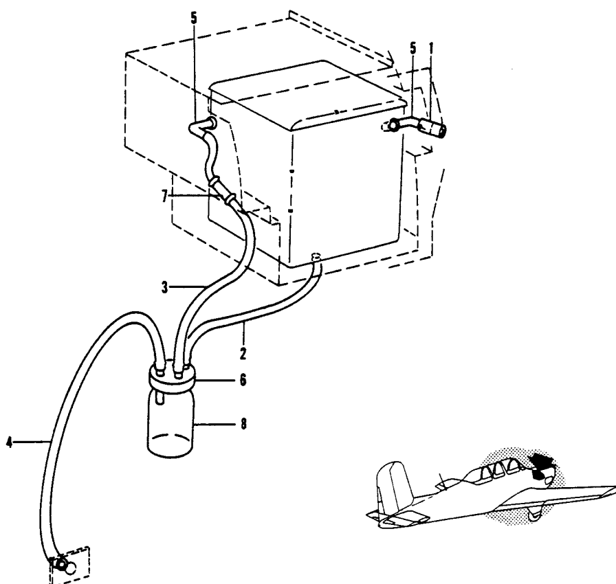
Figure 48. Battery Jar Installation
