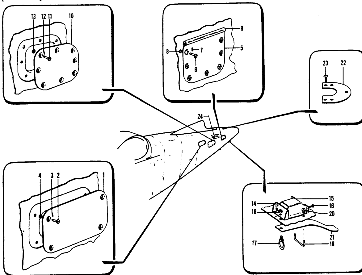
Figure 34. Aft Fuselage Structure Assembly
