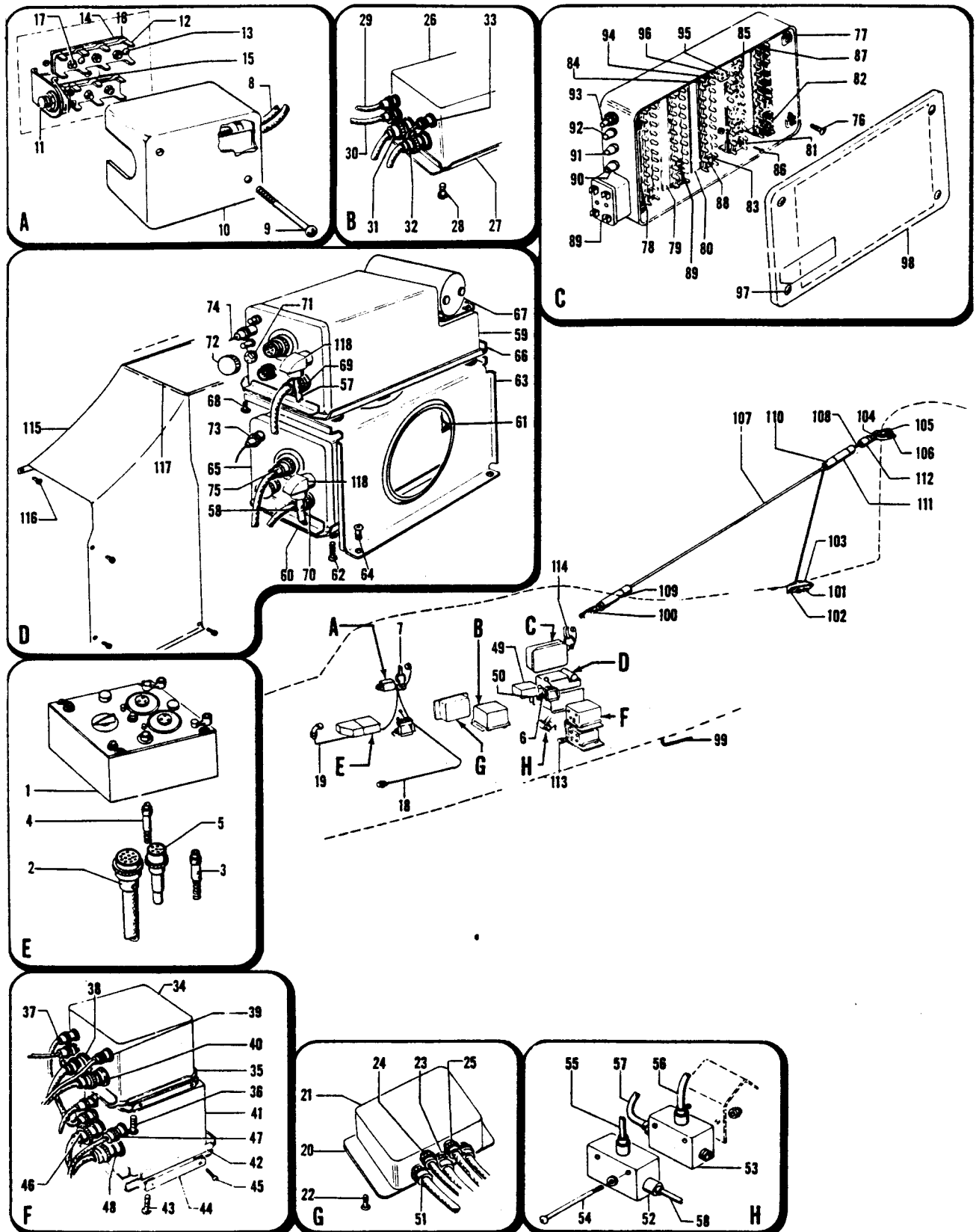
Figure 63. Radio Installation
