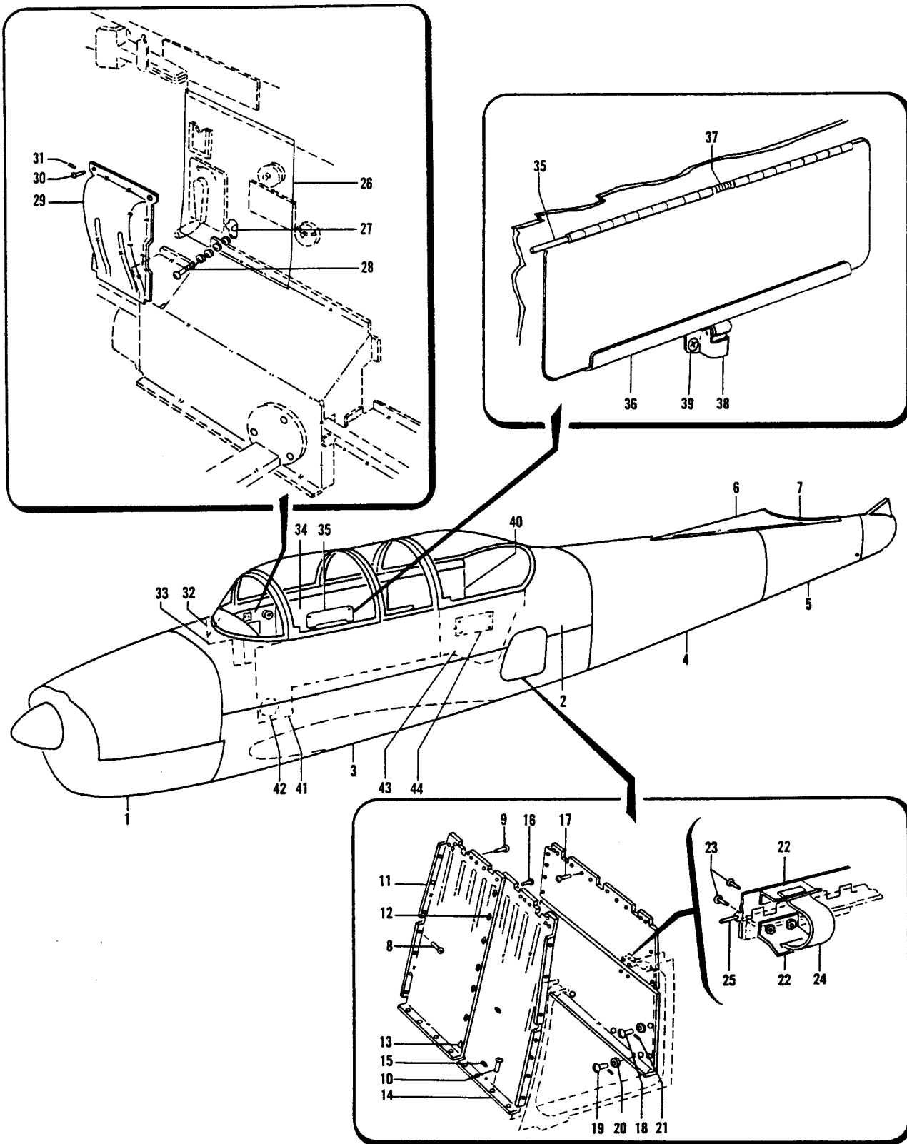
Figure 28. Fuselage Structure Assembly
