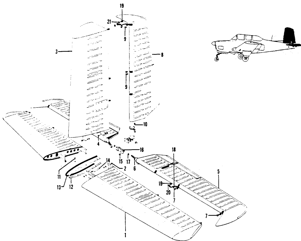
Figure 15. Empennage Installation
