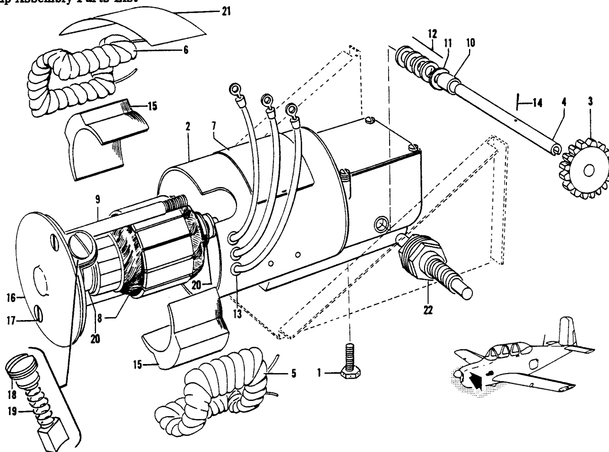
Figure 42. Flap Motor Control Installation
