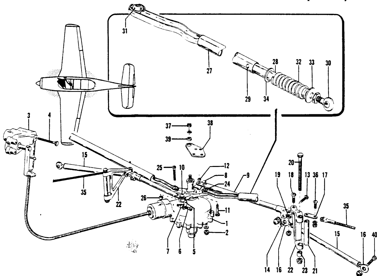
Figure 38. Landing Gear Retract Mechanism Installation
