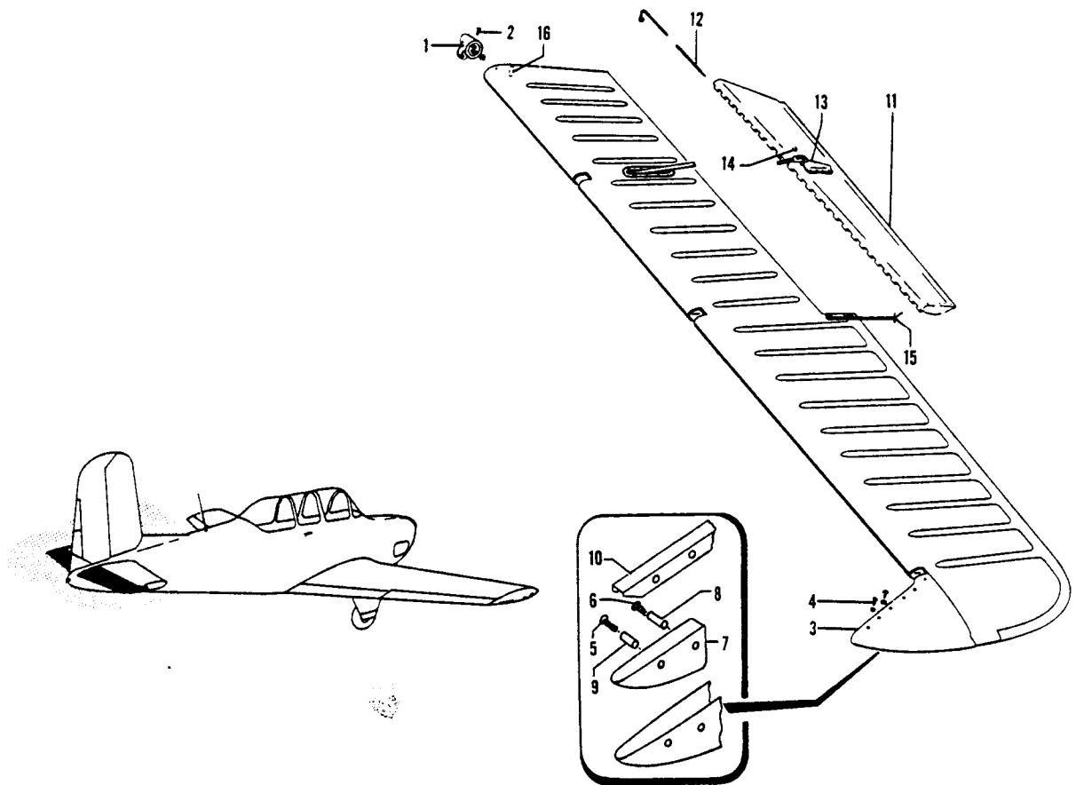
Figure 18. Elevator Assembly
