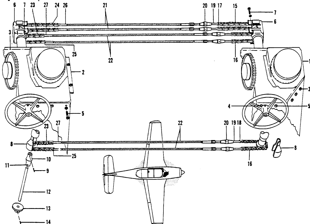
Figure 57. Cockpit Trim Tab Control Installation
