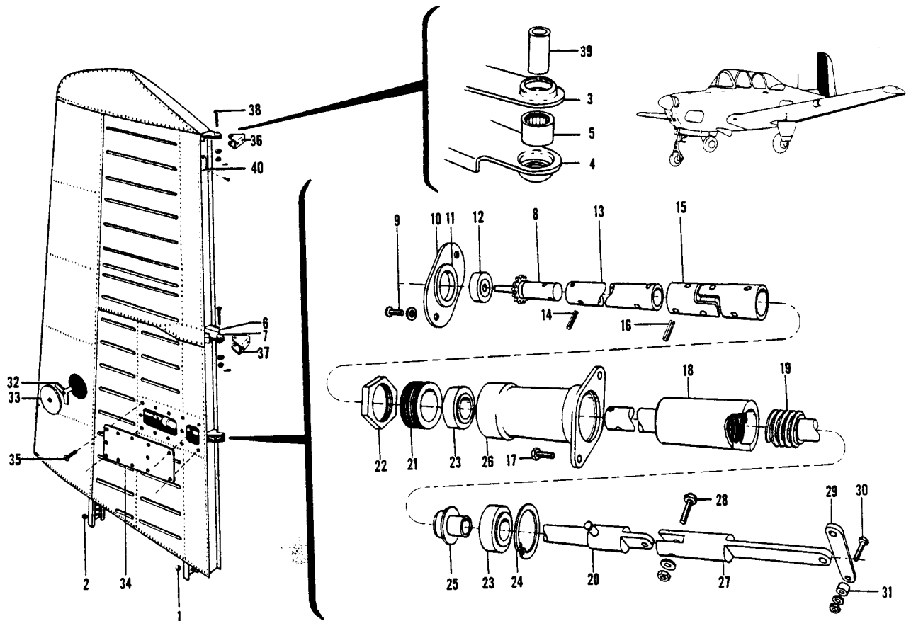
Figure 17. Vertical Stabilizer Assembly
