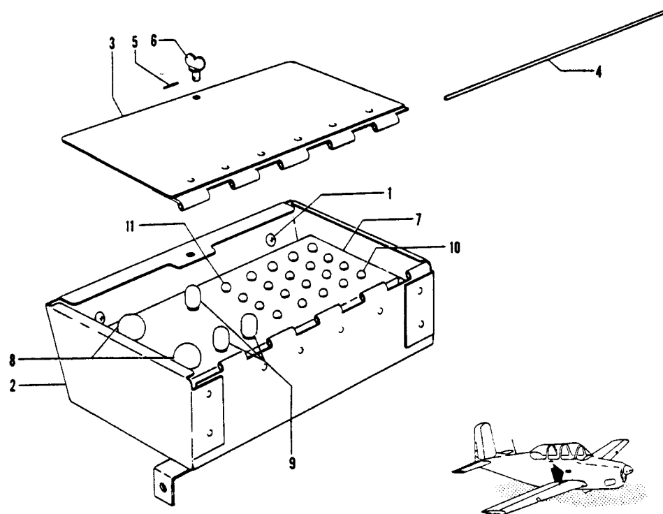
Figure 69. Spare Lamp Box Installation
