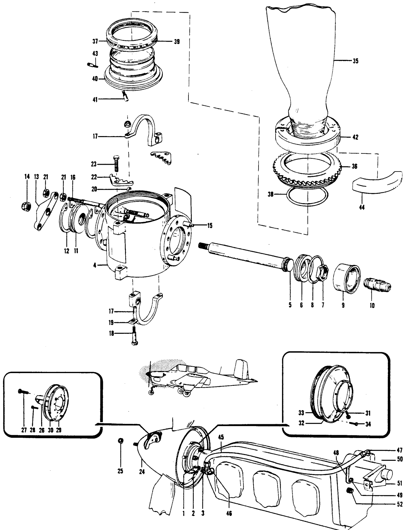
Figure 79. Engine Propeller Installation
