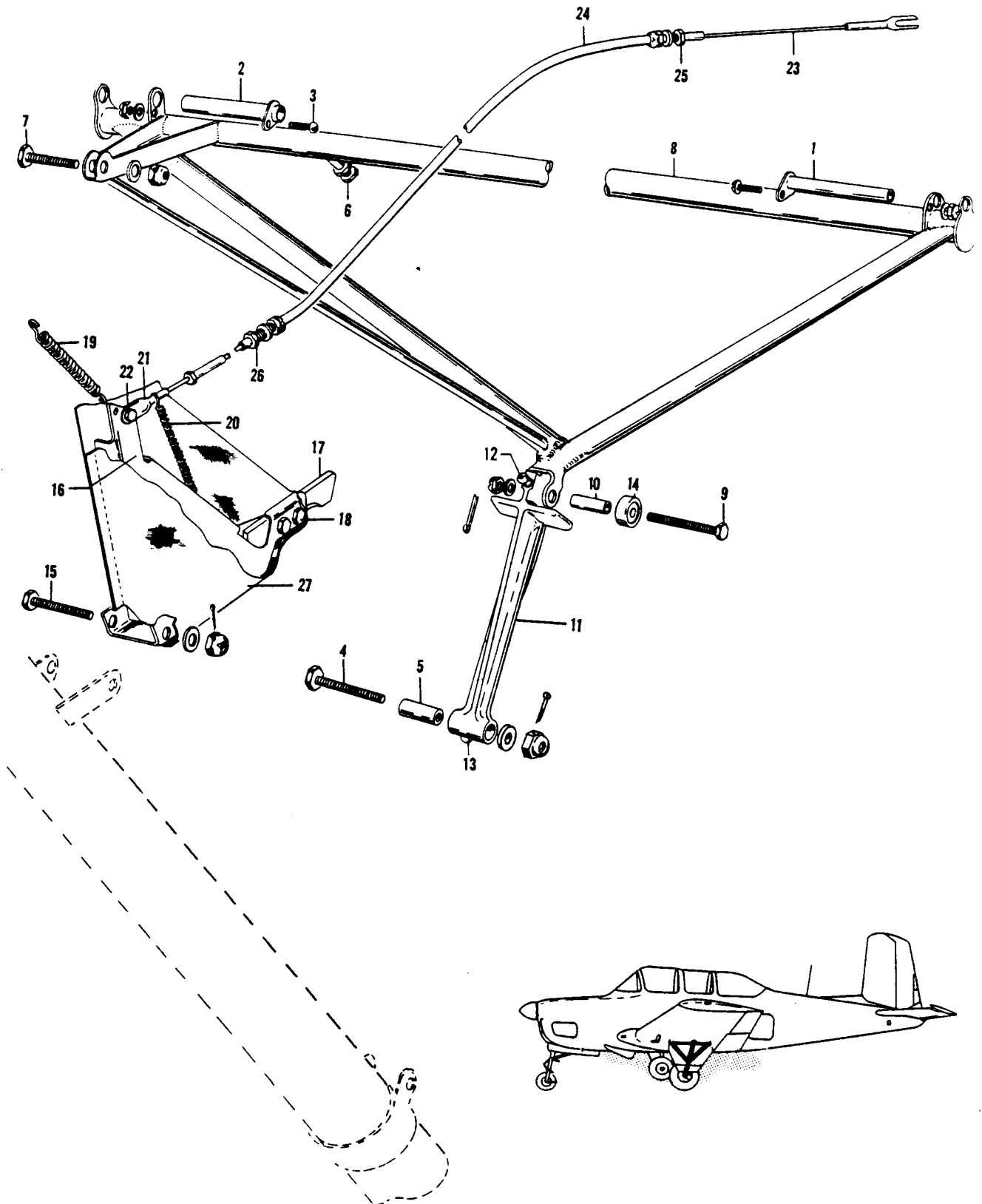
Figure 10. Wing Landing Gear Retract Mechanism Installation
