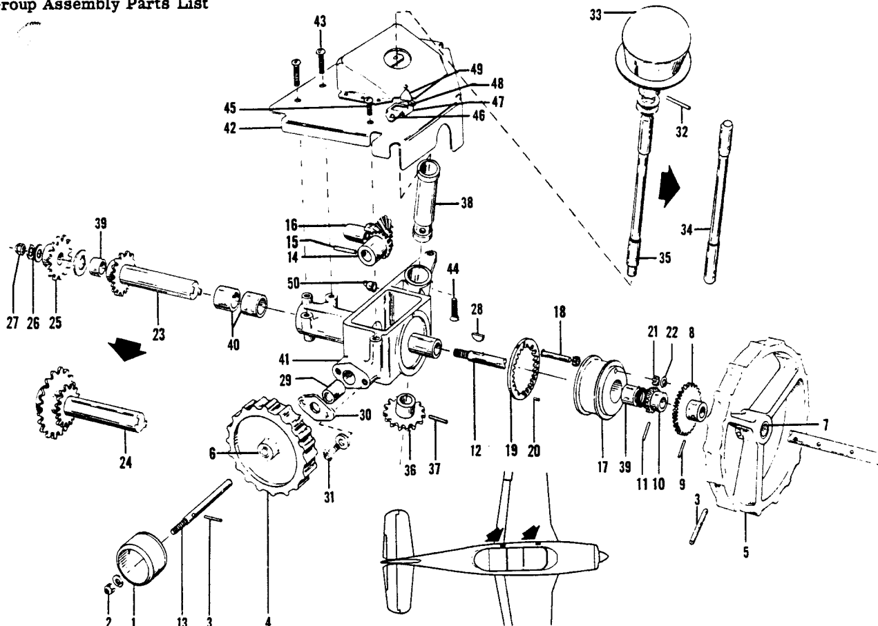
Figure 58. Cockpit Trim Tab Control Assembly
