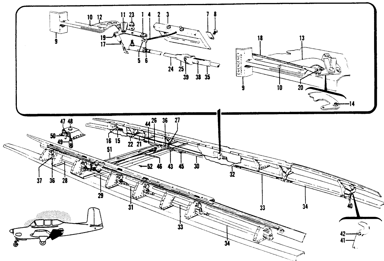
Figure 35. Emergency Canopy Release Installation
