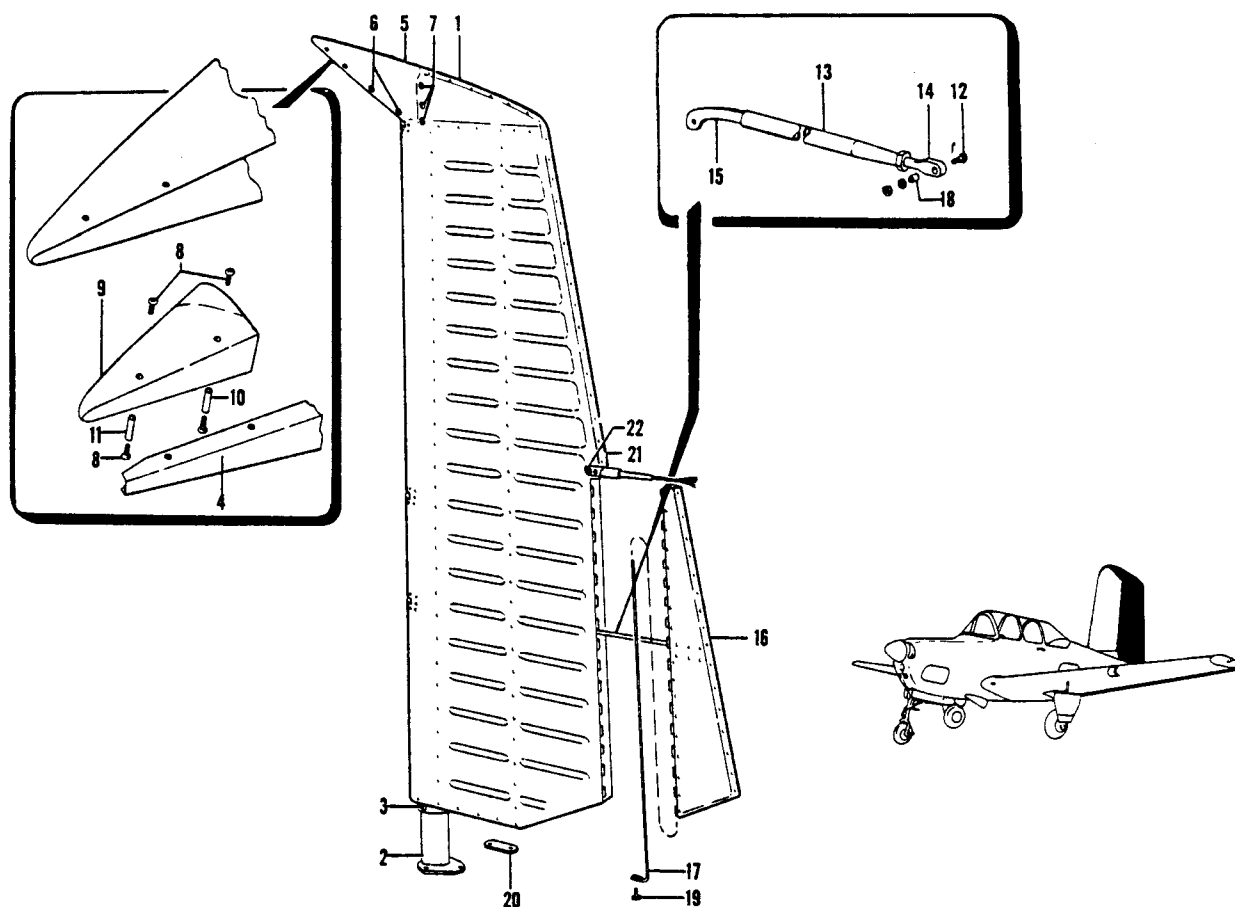
Figure 19. Rudder Assembly
