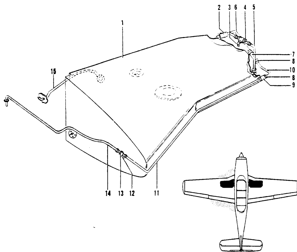
Figure 13. Wing Fuel System Installation
