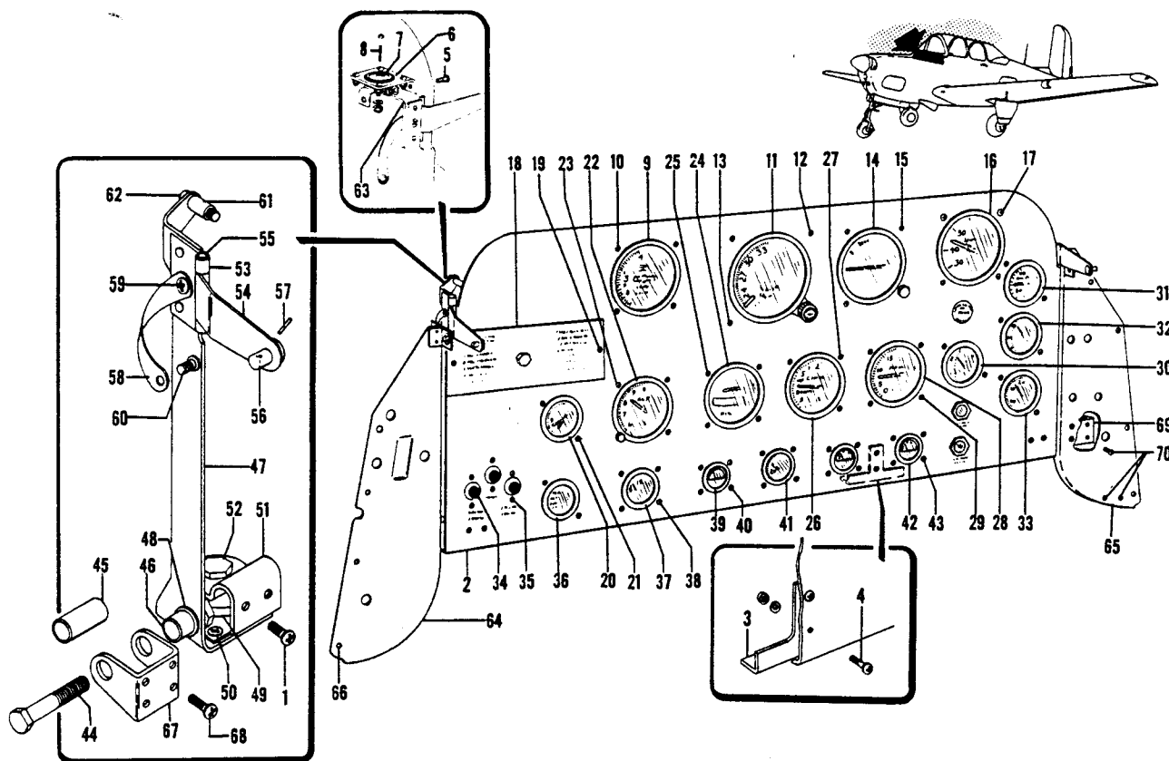
Figure 26. Instrument Panel Installation
