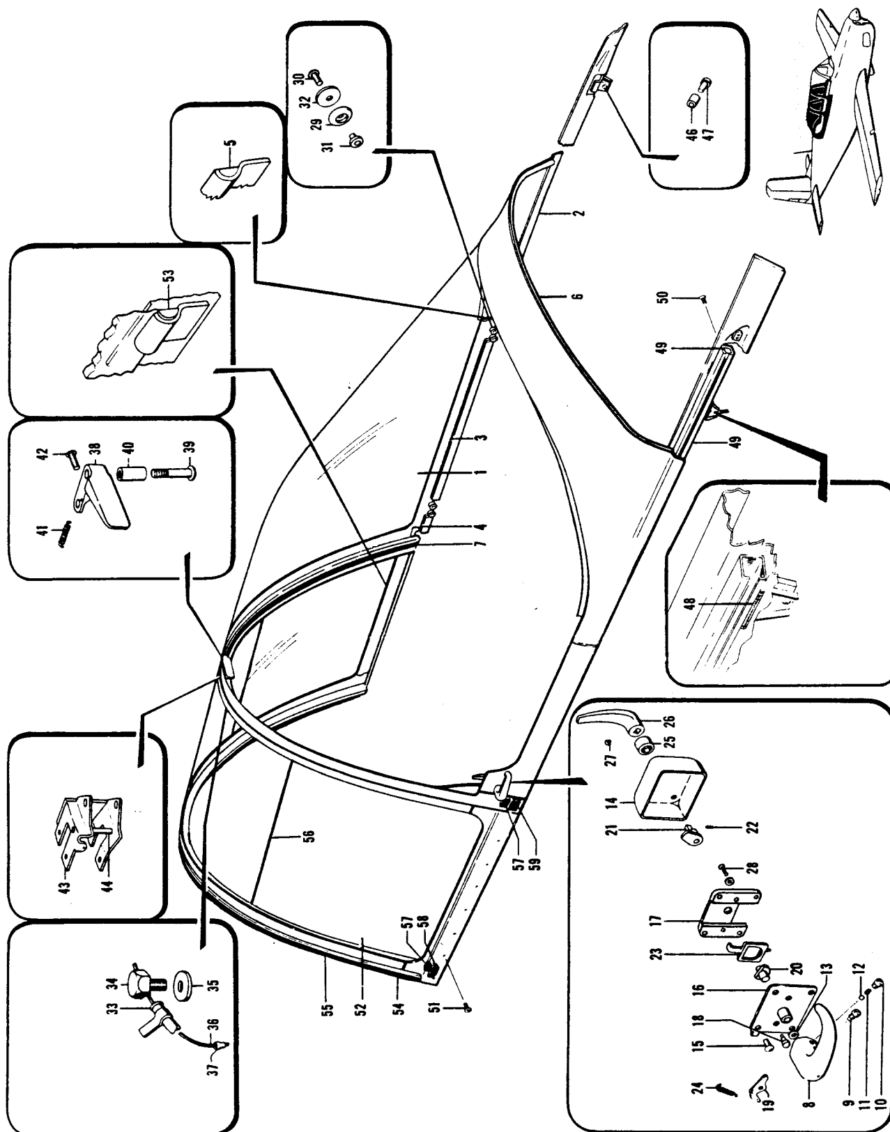
Figure 67. Rear Fuselage Canopy Installation
