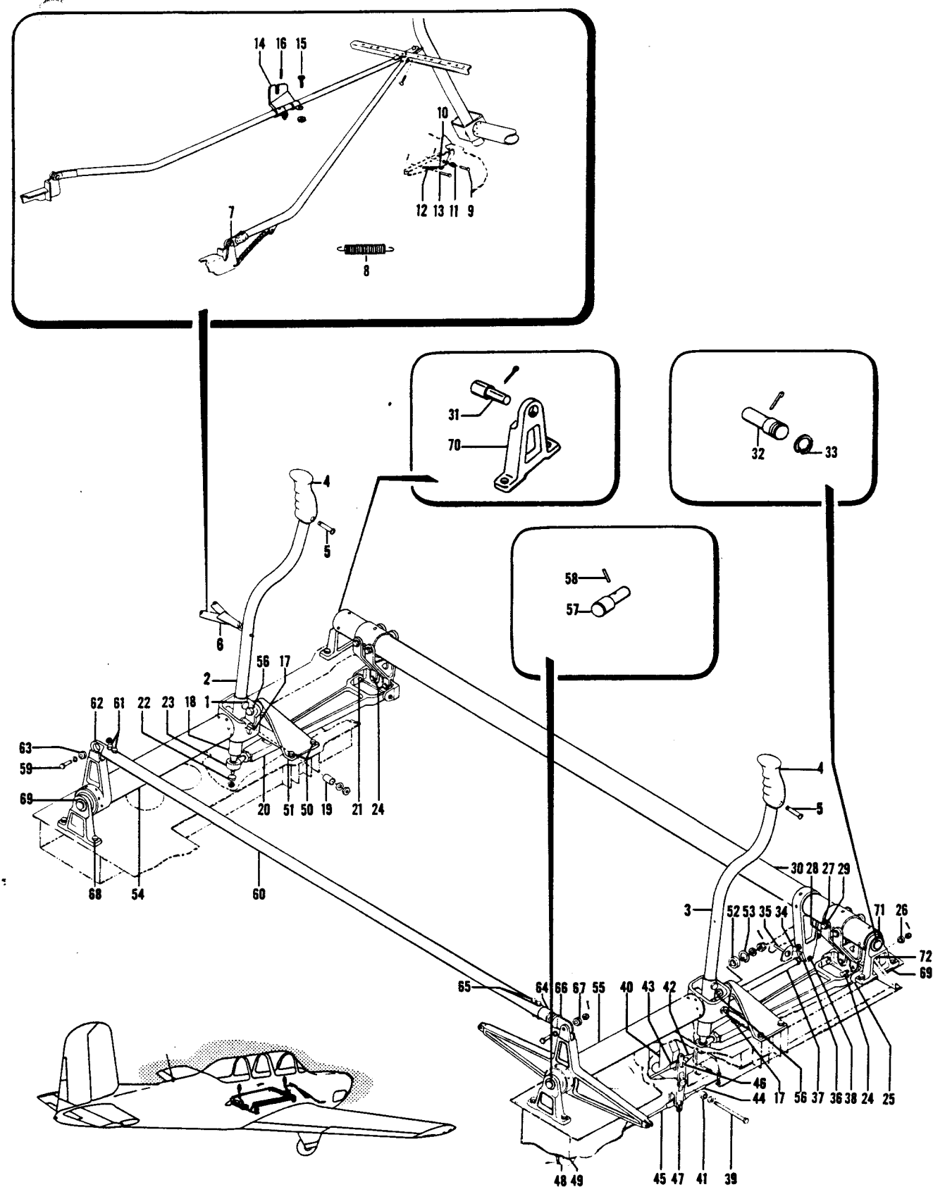
Figure 54. Cockpit Stick Flight Controls Installation
