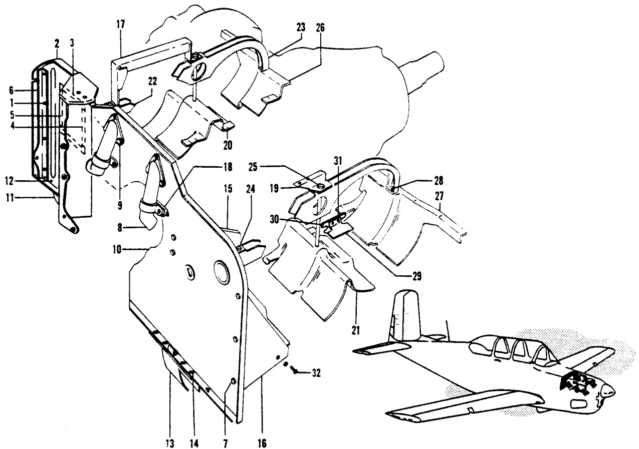
Figure 74. Engine Baffle Installation
