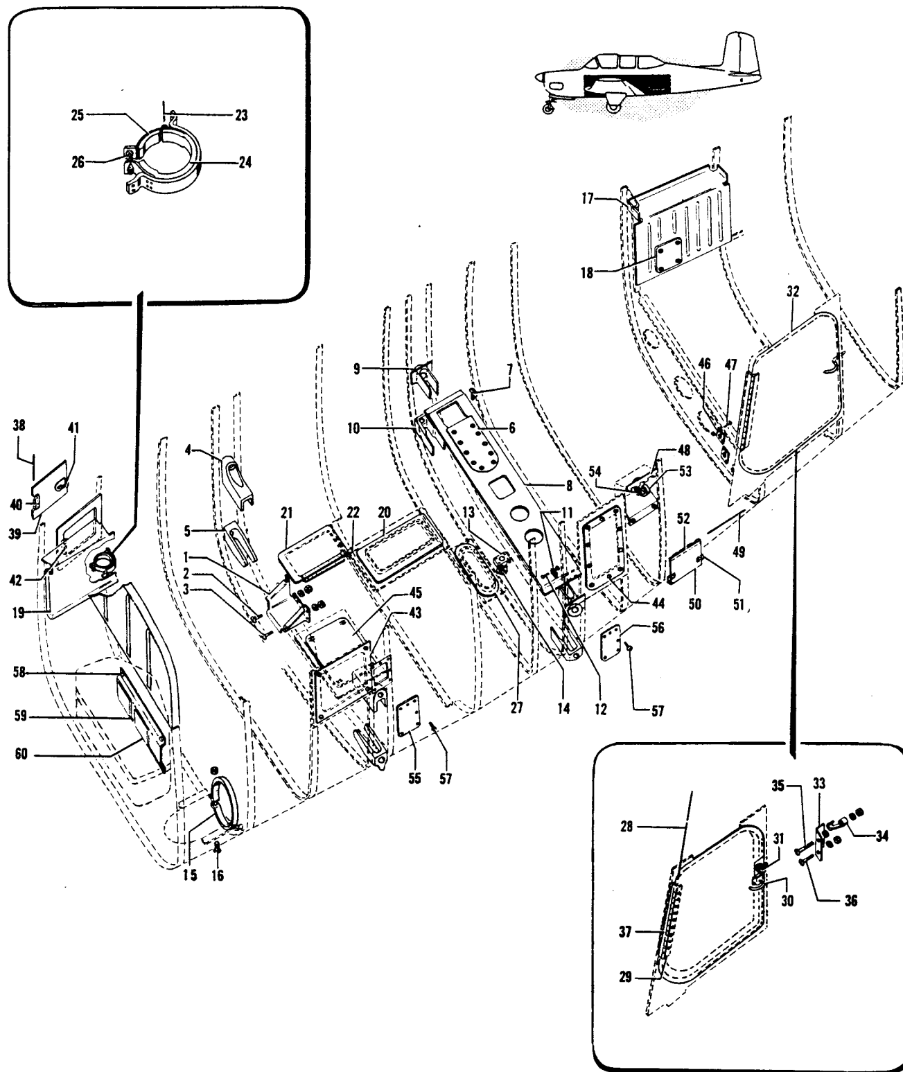
Figure 32. Fuselage Lower Cockpit Structure Assembly
