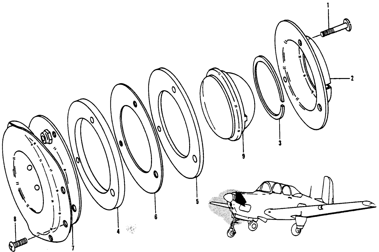
Figure 46. Passing Light Installation
