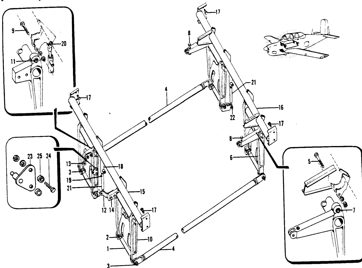
Figure 55. Rudder Pedal Control Installation
