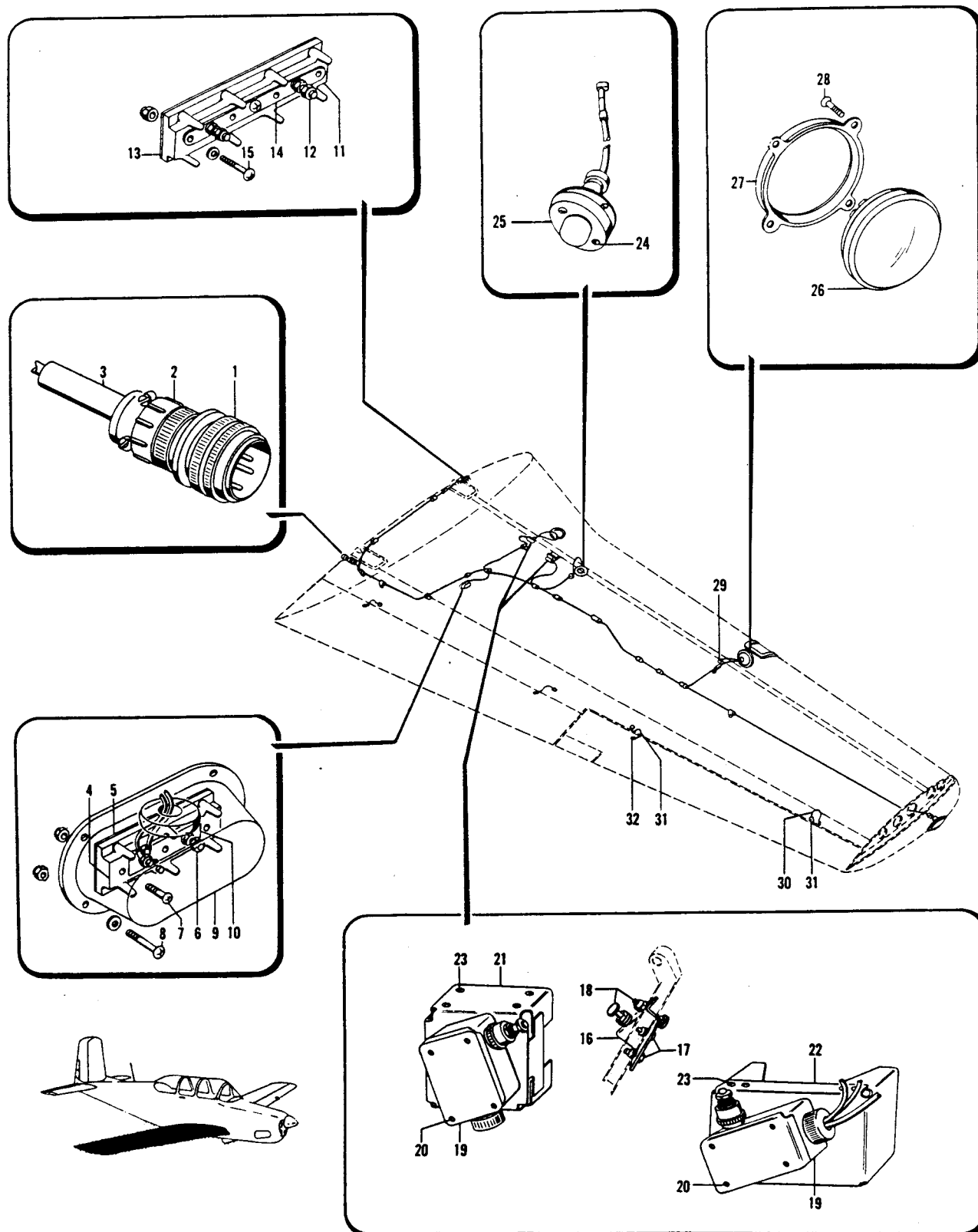
Figure 9. Right Hand Wing Electrical Installation
