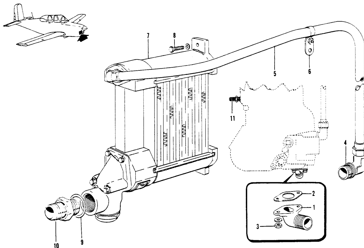
Figure 77. Engine Oil System Installation
