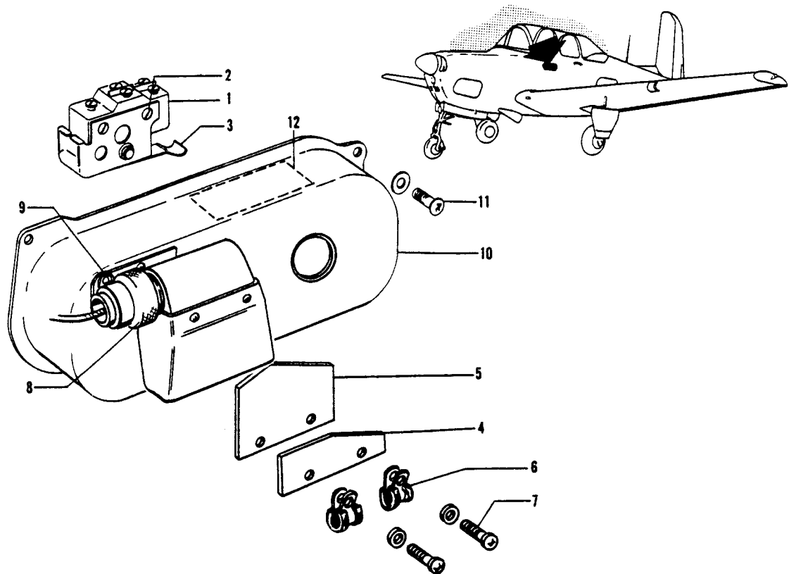
Figure 50. Throttle Warning Switch Installation
