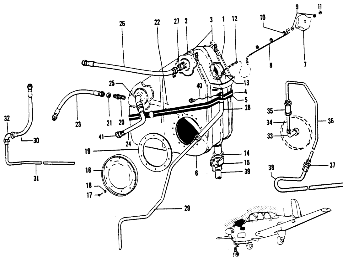
Figure 23. Fuselage Oil System Installation
