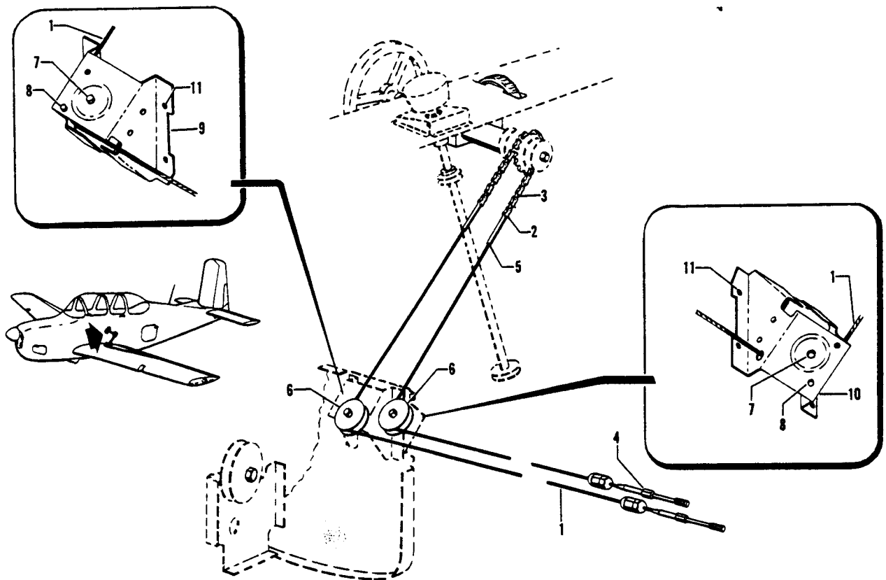
Figure 59. Aileron Trim Tab Control Cables
