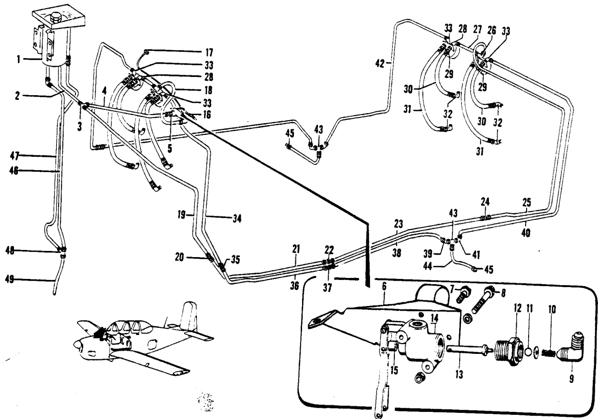
Figure 27. Fuselage Hydraulic Brake Plumbing Installation
