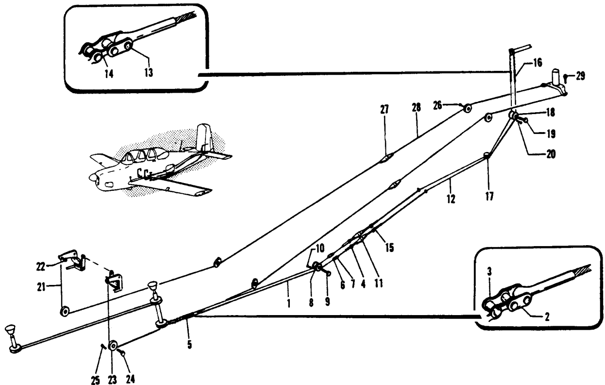
Figure 61. Rudder and Rudder Tab Control Cables
