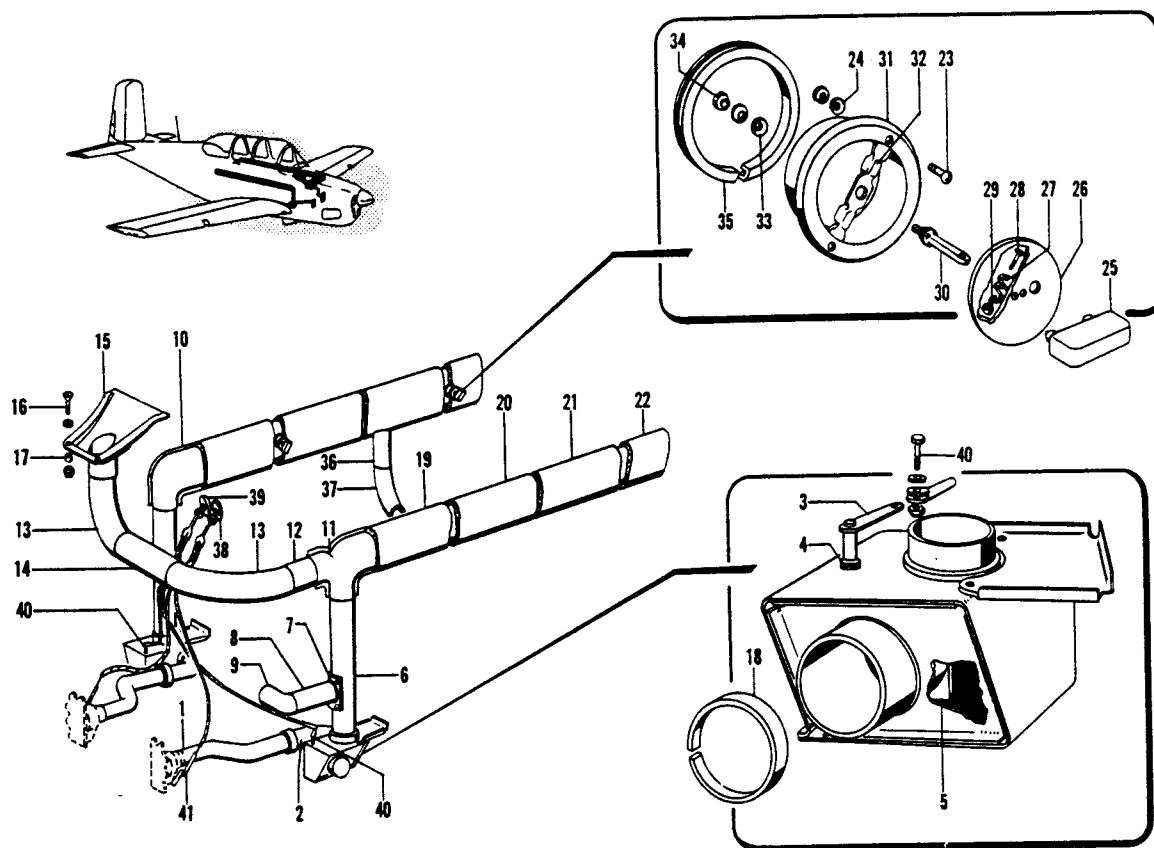
Figure 25. Heat and Vent Installation
