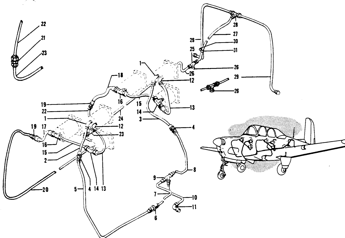
Figure 43. Fuselage Pitot and Static Air Piping Installation
