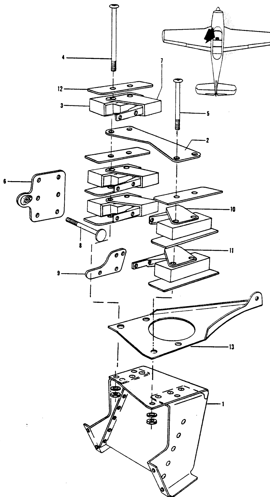
Figure 51. Landing Gear Limit Switch Assembly
