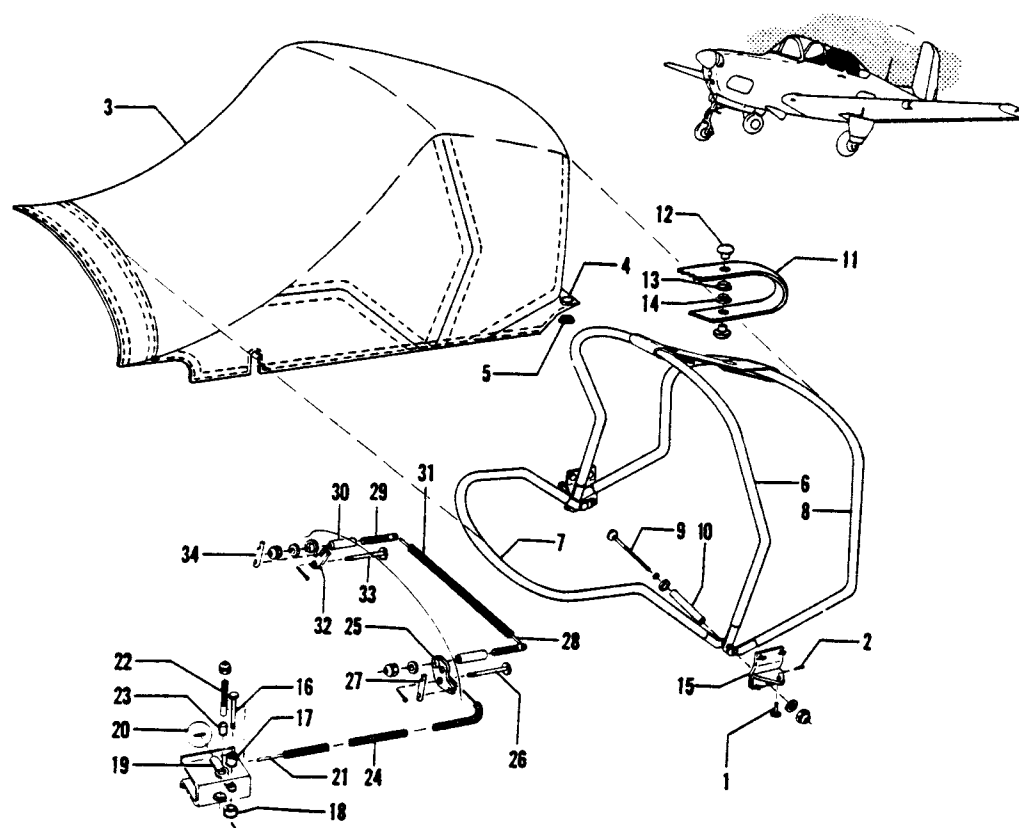
Figure 68. Blind Flying Hood Installation
