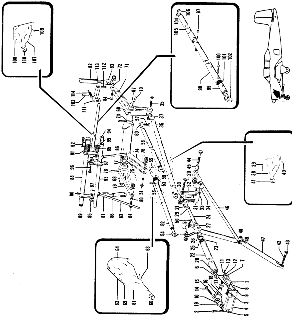
Figure 21. Nose Wheel Retract Mechanism Installation
