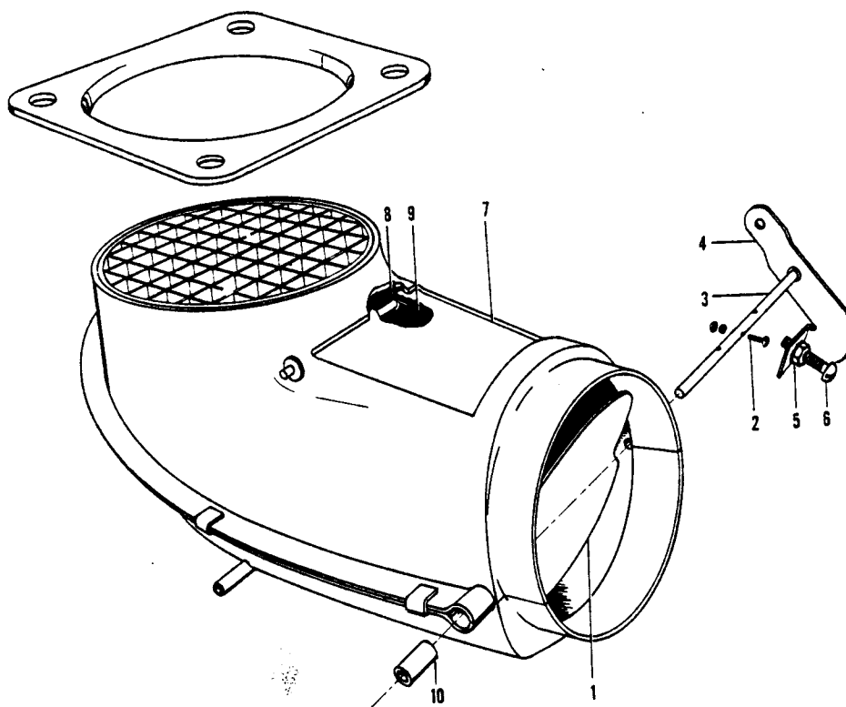
Figure 76. Carburetor Air Valve Assembly
