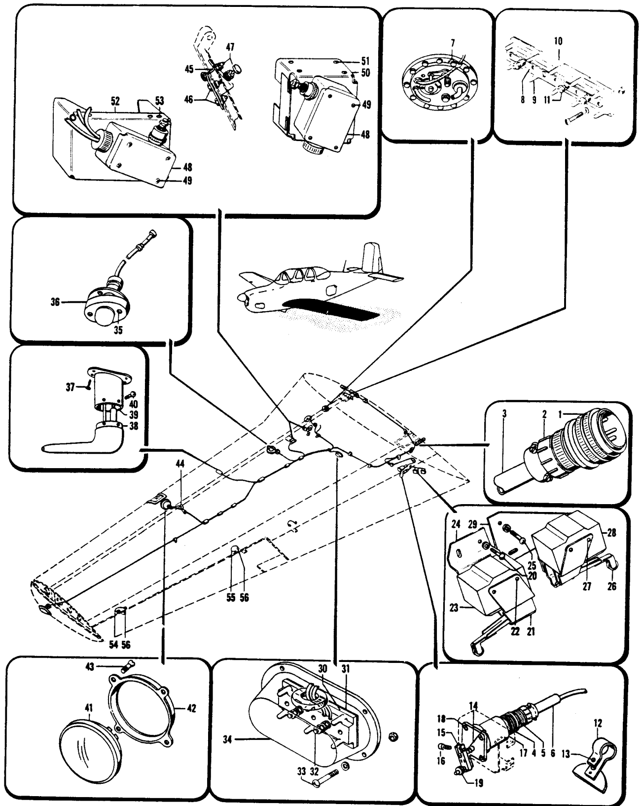
Figure 8. Left Hand Wing Electrical Installation
