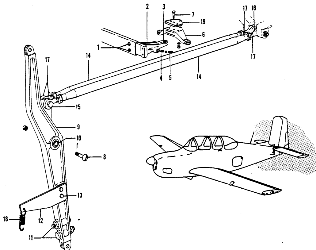
Figure 56. Rear Flight Control Installation
