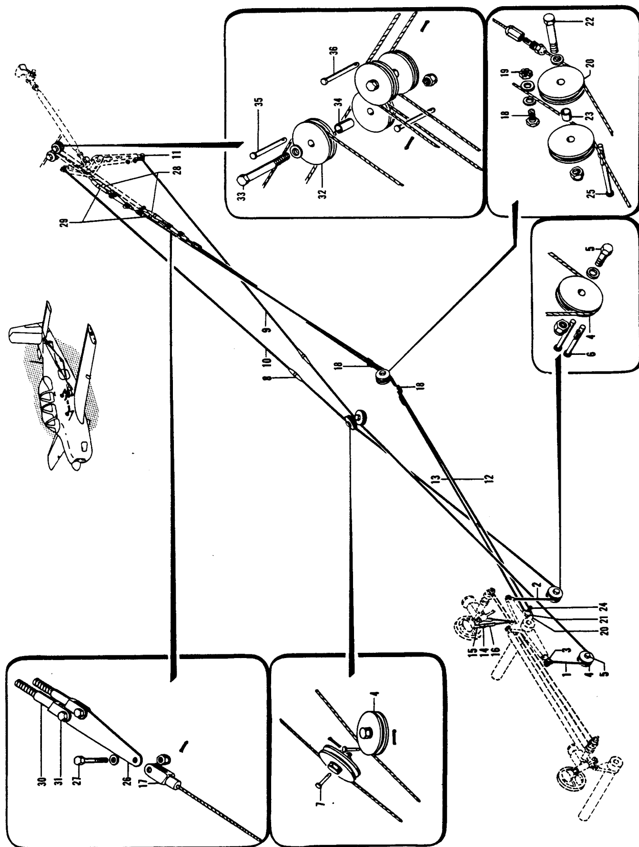
Figure 60. Elevator and Elevator Tab Control Cables
