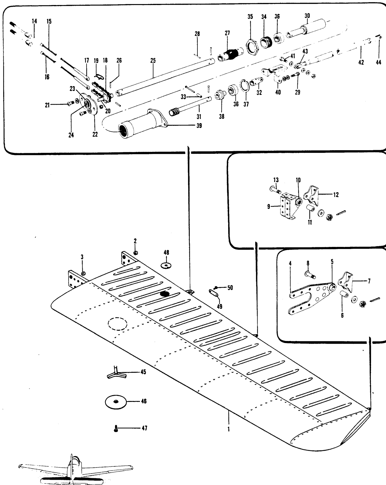
Figure 16. Horizontal Stabilizer Assembly
