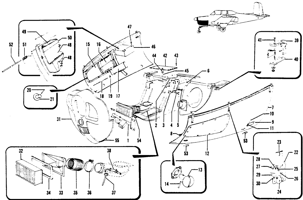
Figure 29. Forward Fuselage Structure Assembly
