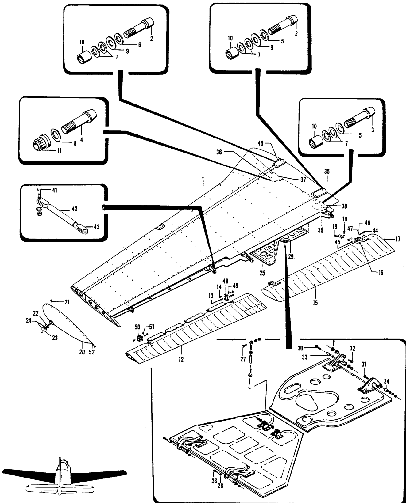
Figure 2. Wing Installation
