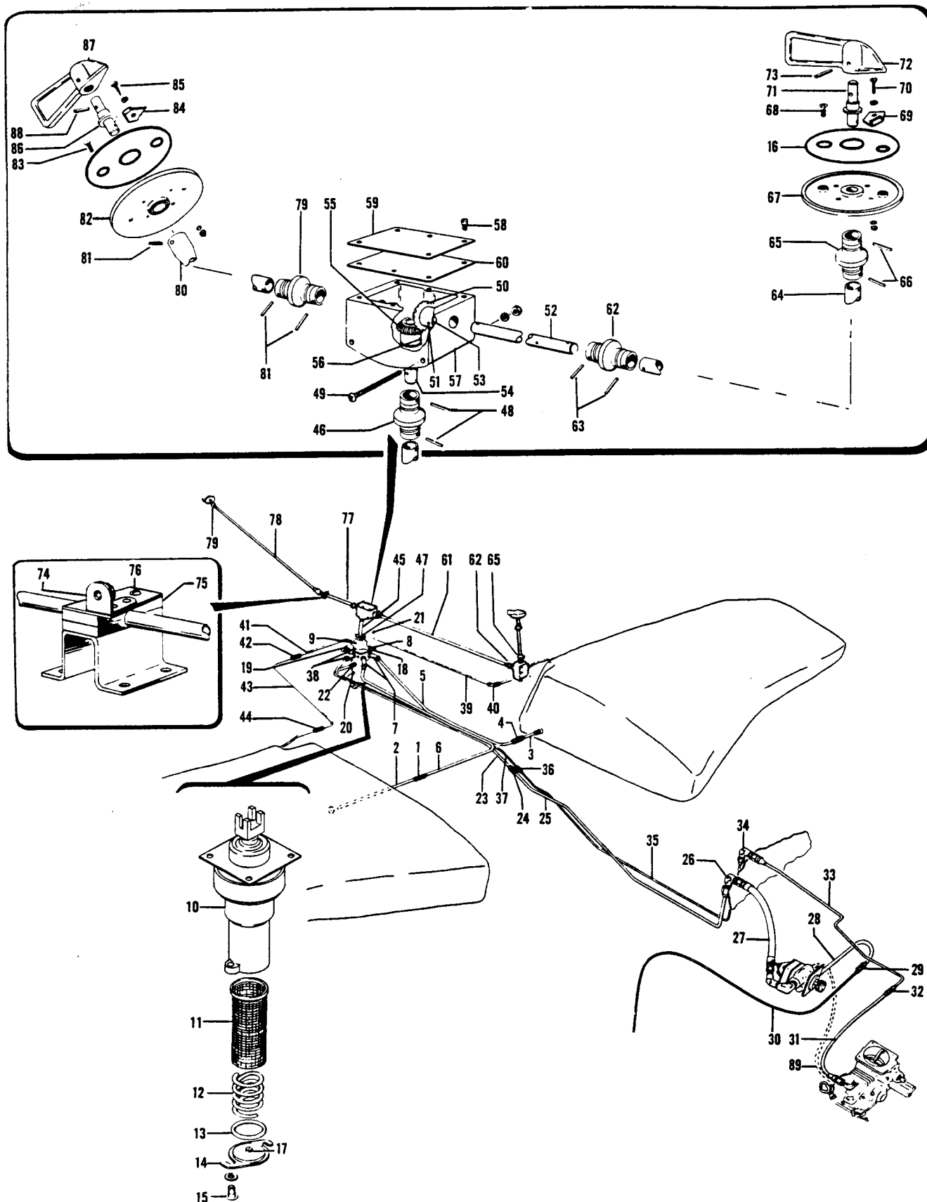
Figure 36. Fuselage Fuel System Installation
