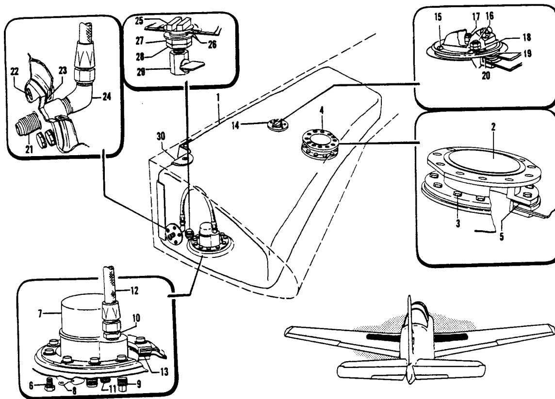
Figure 14. Wing Fuel Cell Installation
