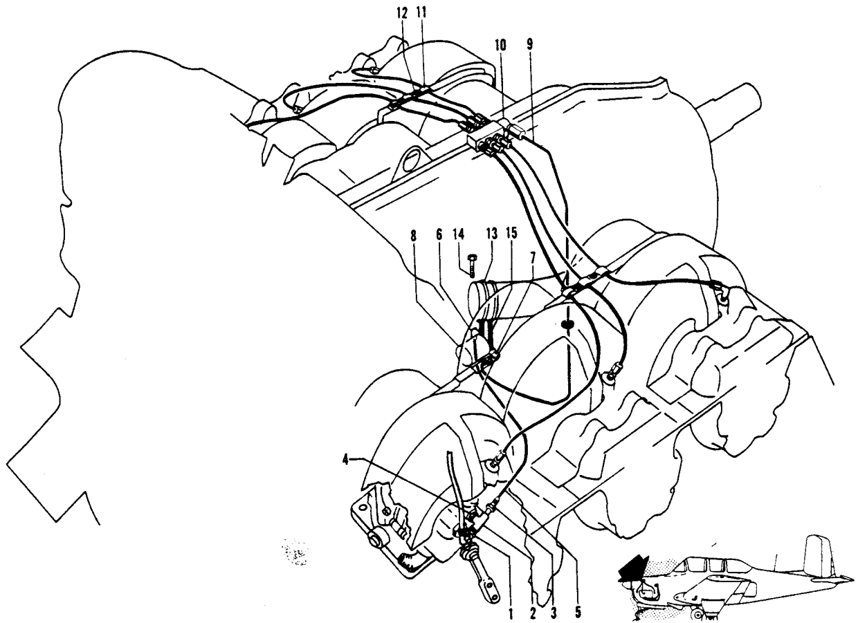
Figure 78. Engine Primer Installation
