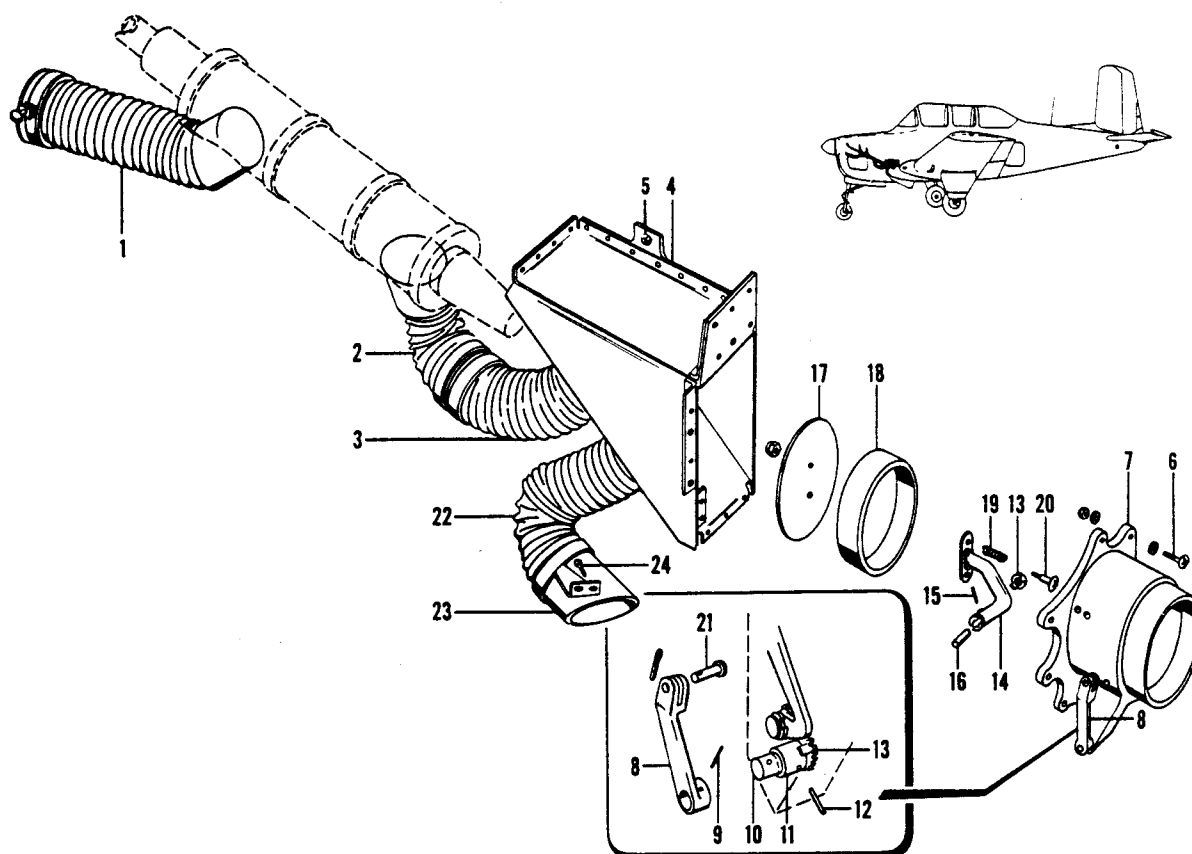
Figure 24. Cockpit Heat Installation
