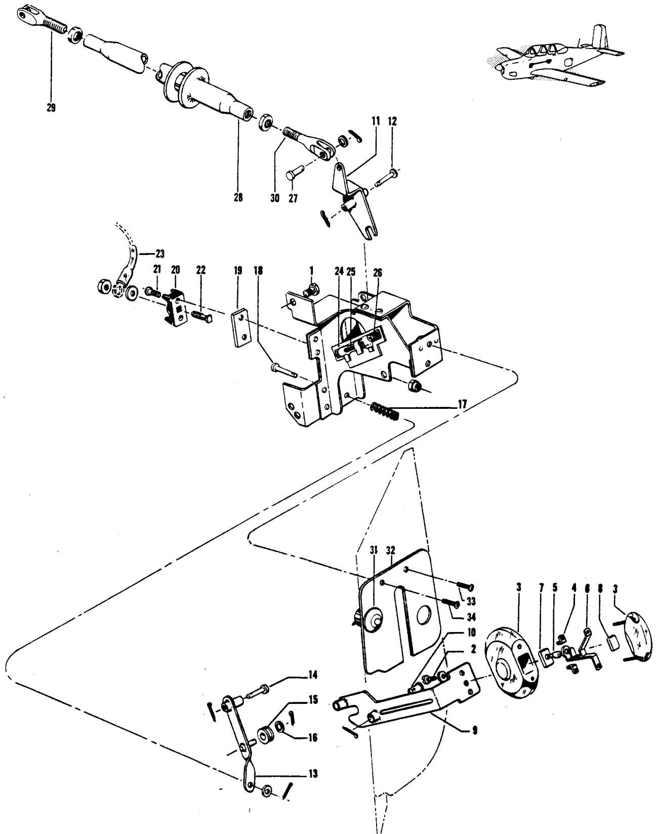
Figure 52. Landing Gear Control Switch Installation
