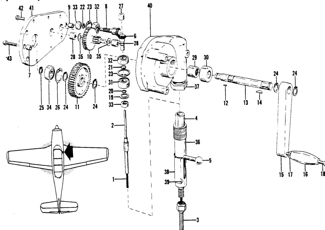
Figure 40. Landing Gear Hand Retract Mechanism Assembly
