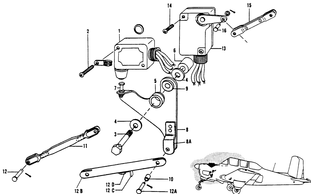
Figure 47. Nose Gear Indicator Switch Installation
