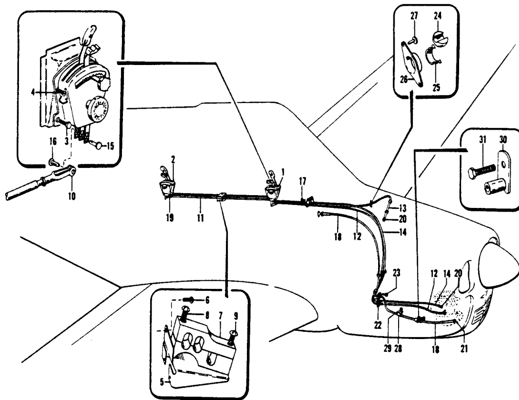
Figure 62. Engine Control Installation
