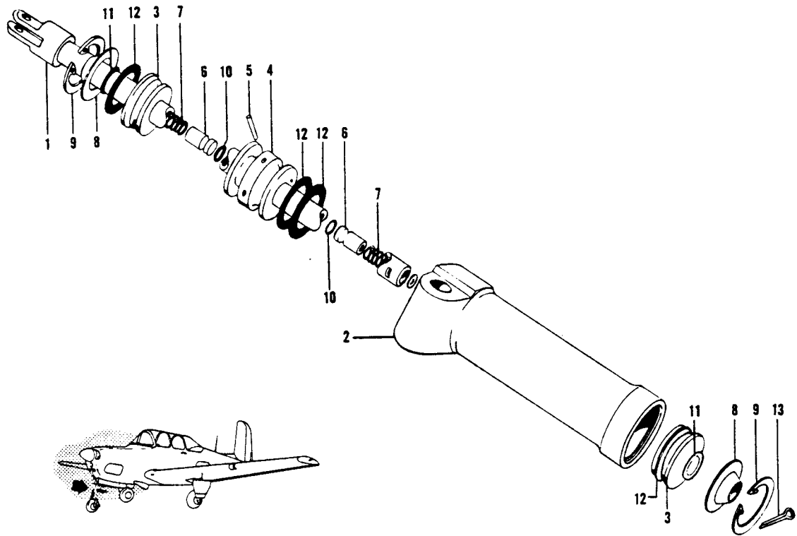
Figure 72. Nose Gear Shimmy Dampener
