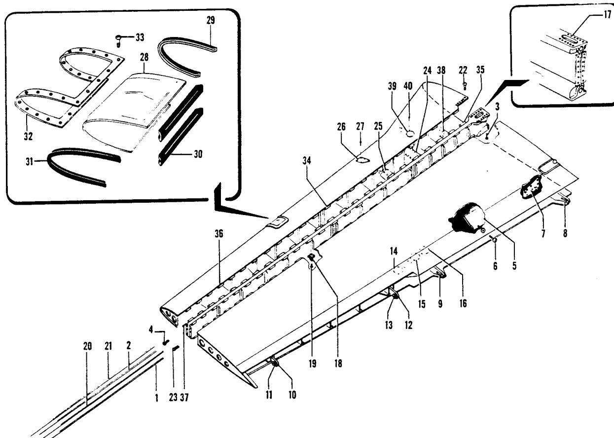
Figure 6. Wing Structure Assembly
