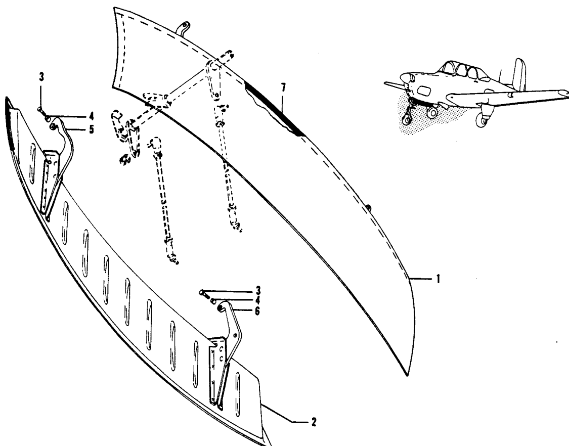
Figure 22. Nose Wheel Door Installation
