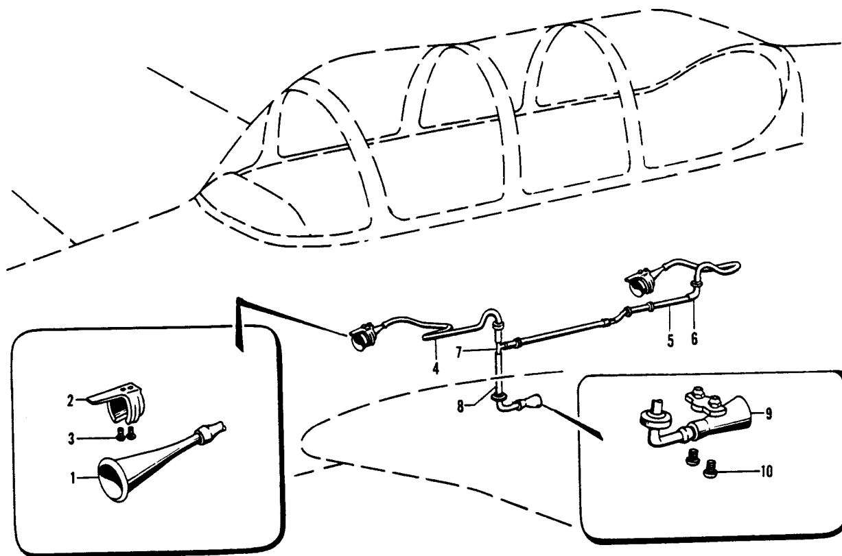
Figure 64. Pilot and Copilots Relief Tube Installation
