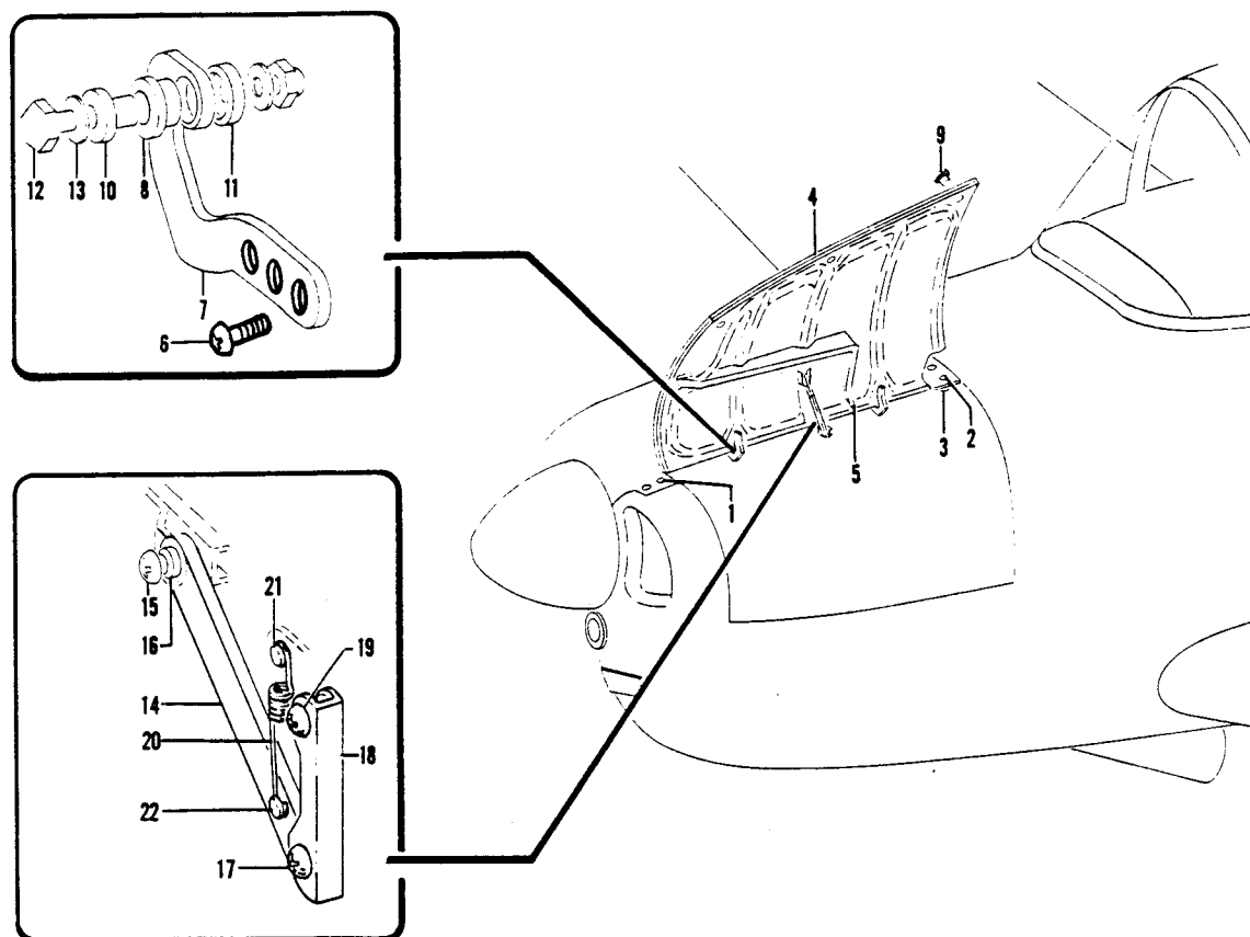
Figure 80. Engine Cowling Assembly
