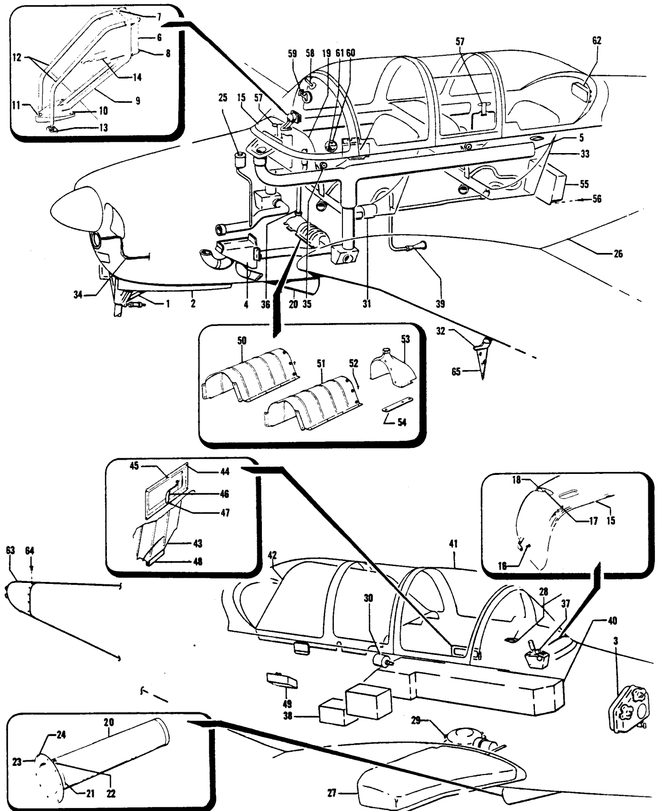
Figure 20. Fuselage and Equipment Assembly
