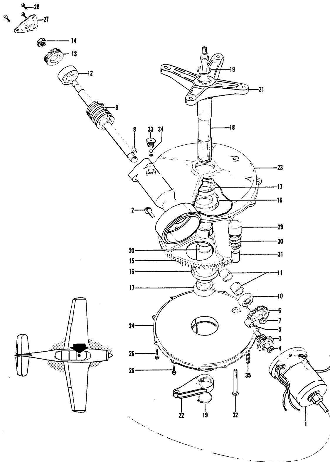
Figure 39. Landing Gear Retract Actuator Assembly
