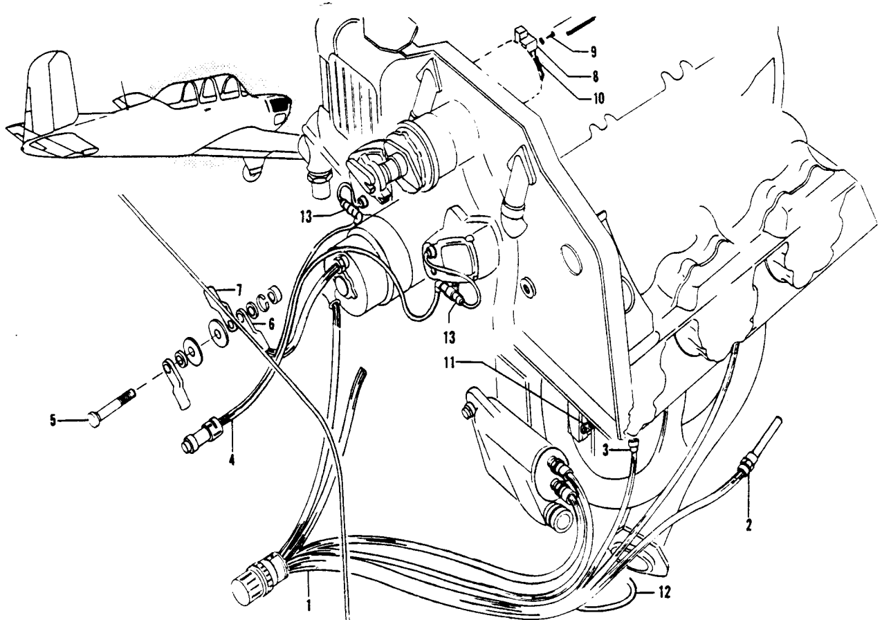
Figure 75. Power Plant Electrical Installation
