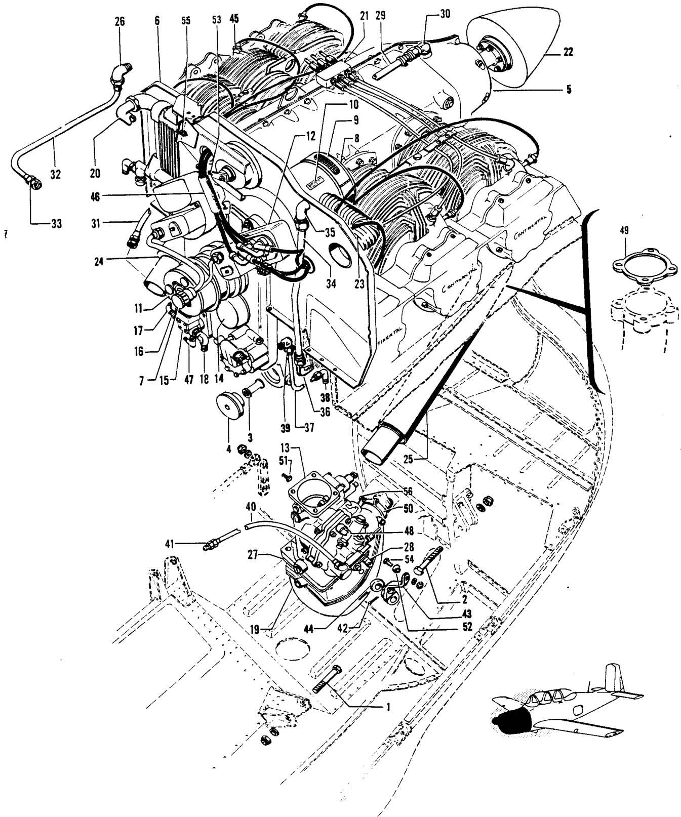
Figure 73. Power Plant Installation
