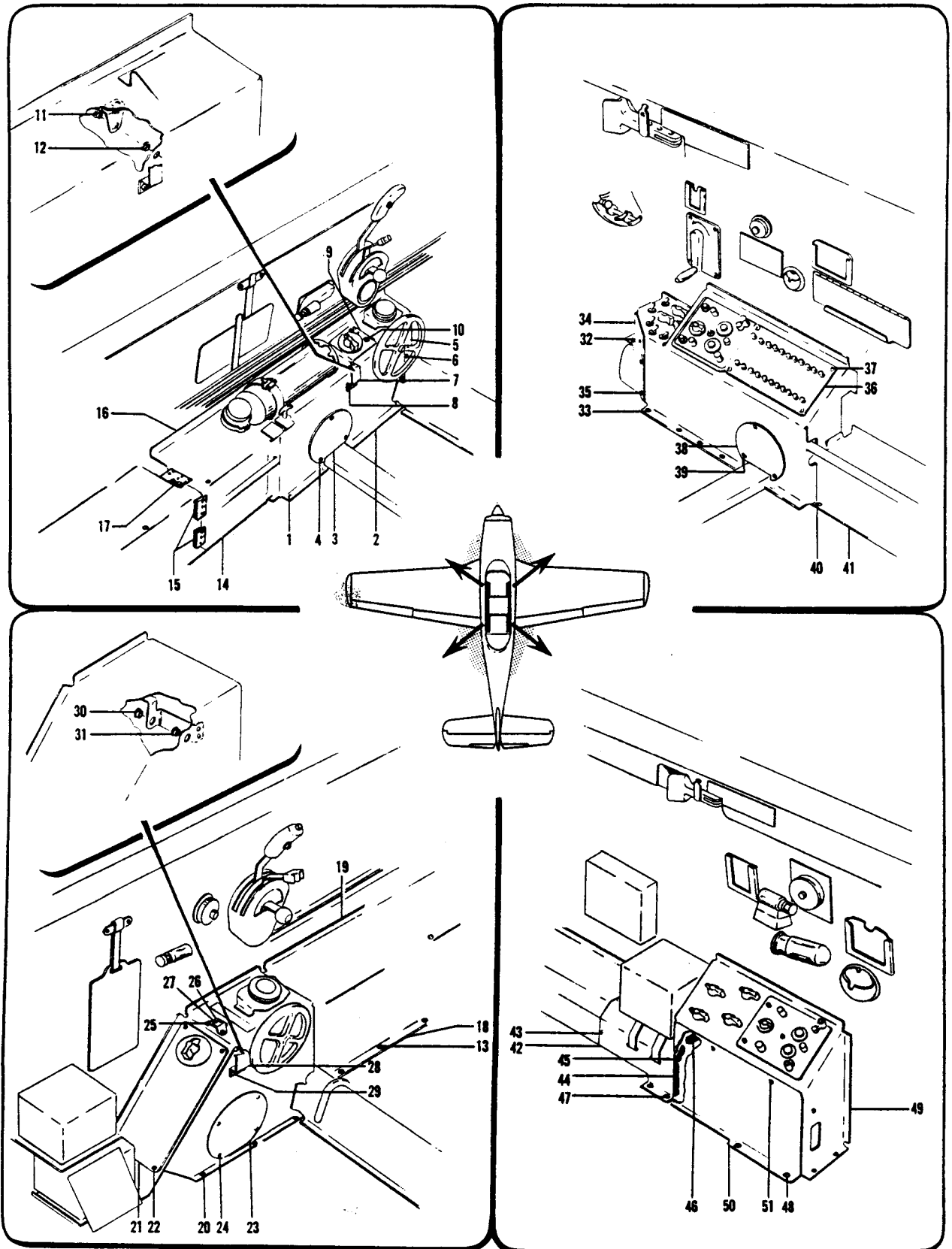
Figure 65. Cockpit Console Installation
