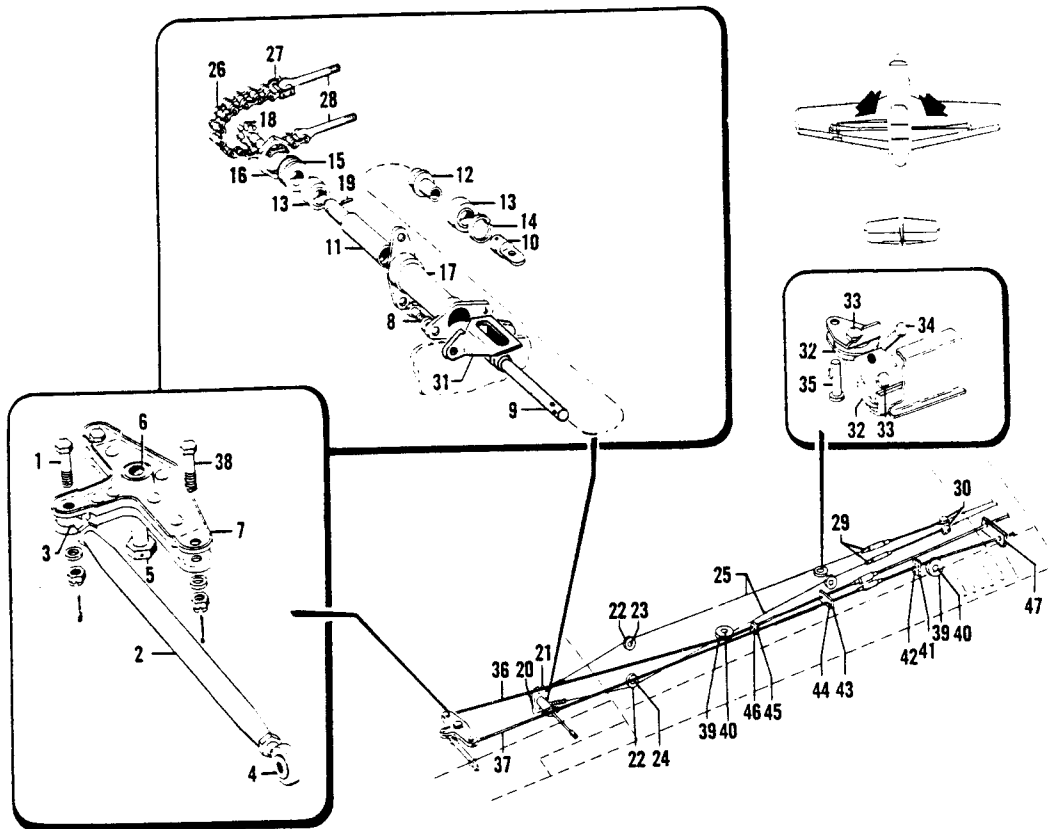
Figure 11. Wing Flight Controls Installation
