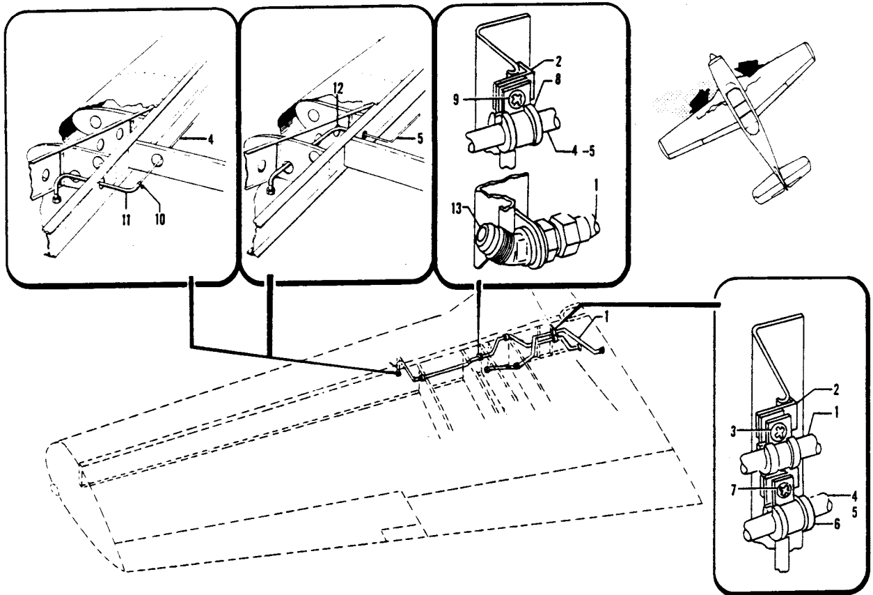
Figure 7. Wing Piping Installation
