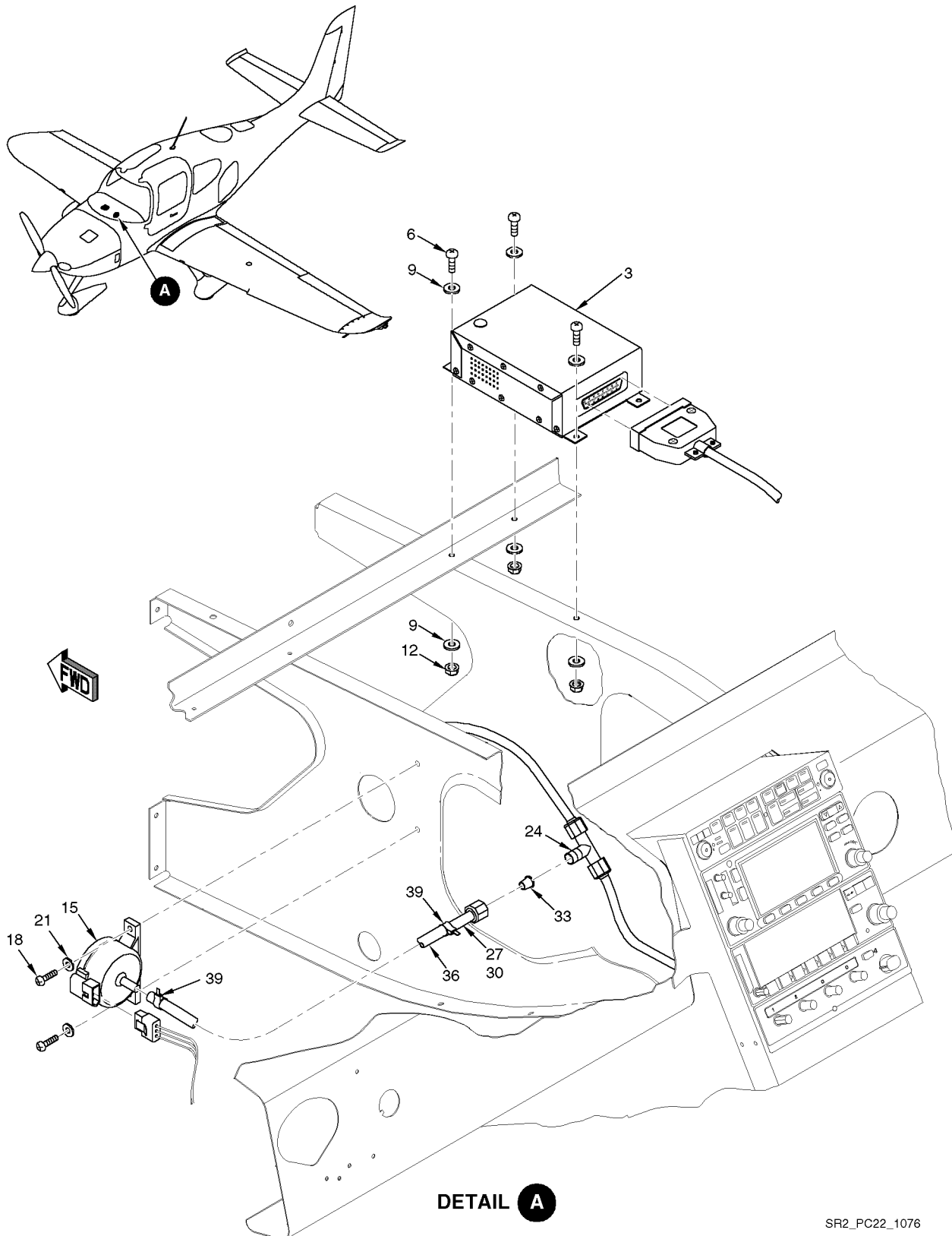
Figure 01 Pitch Computer and Altitude Transducer Installations
