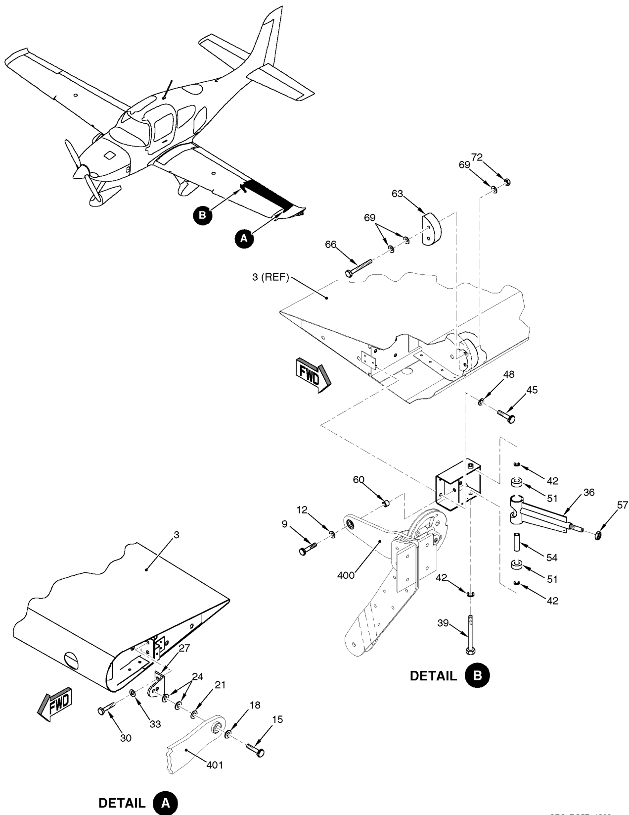
Figure 02 Aileron Installation
