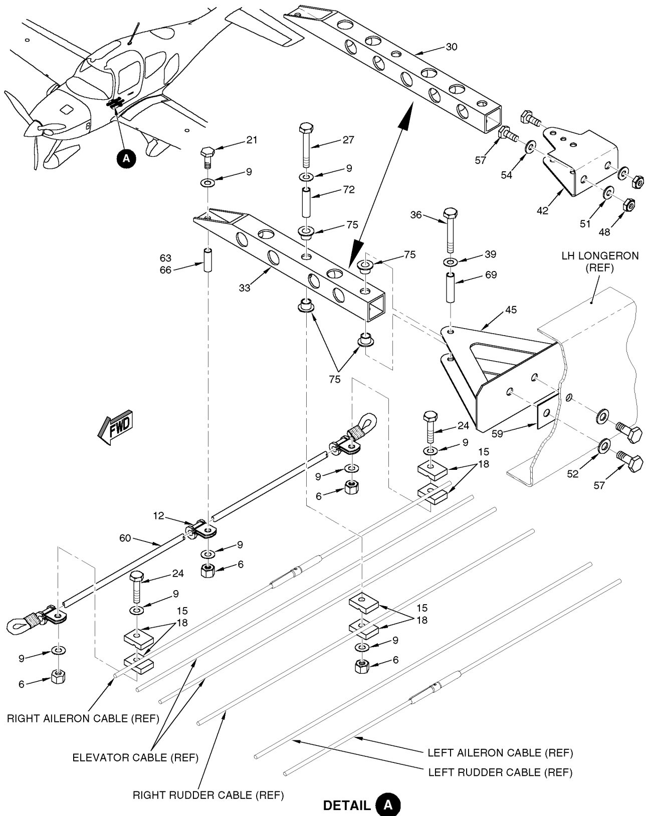
Figure 04 Rudder/Aileron interconnect Installation
