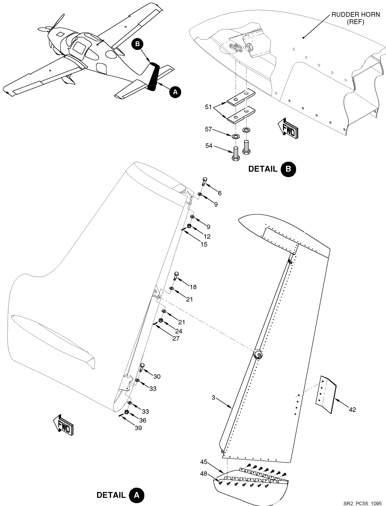
Figure 01 Rudder Installation
