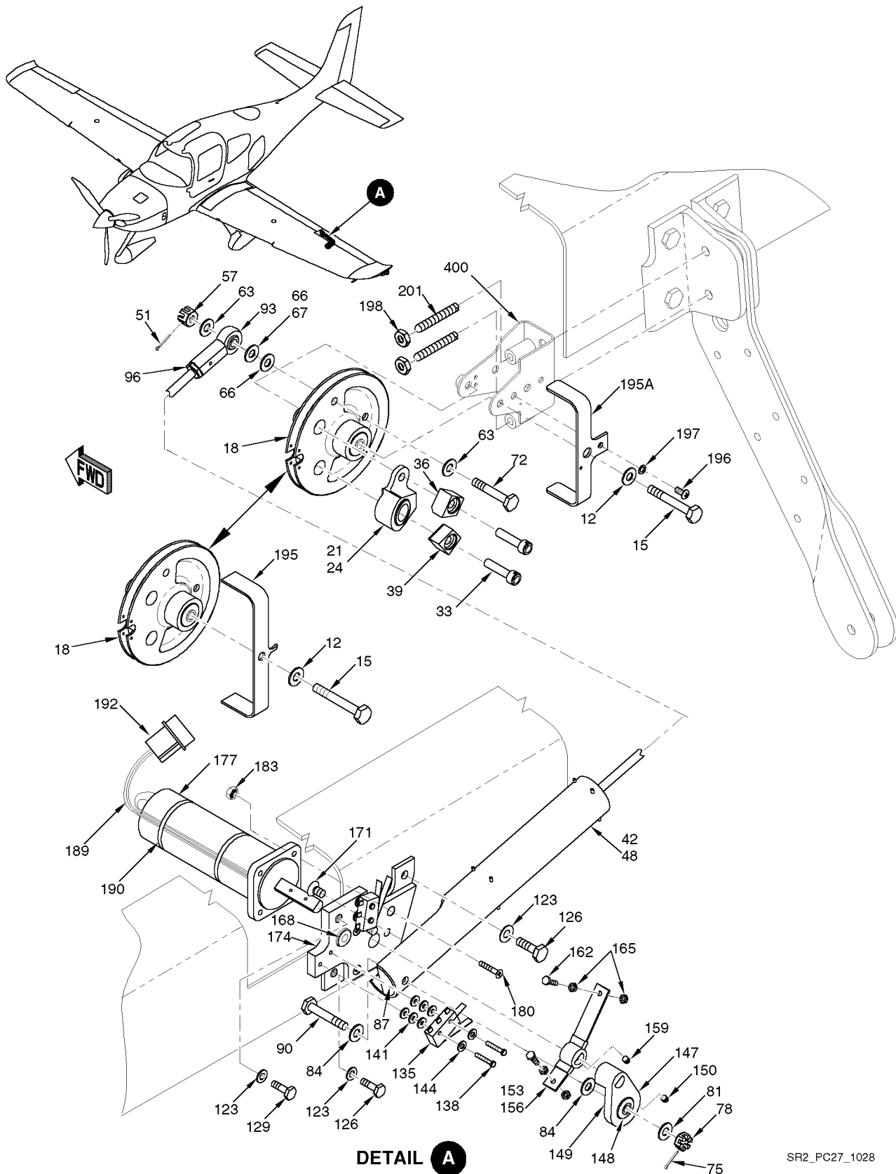
Figure 03 Roll Trim System Installation
