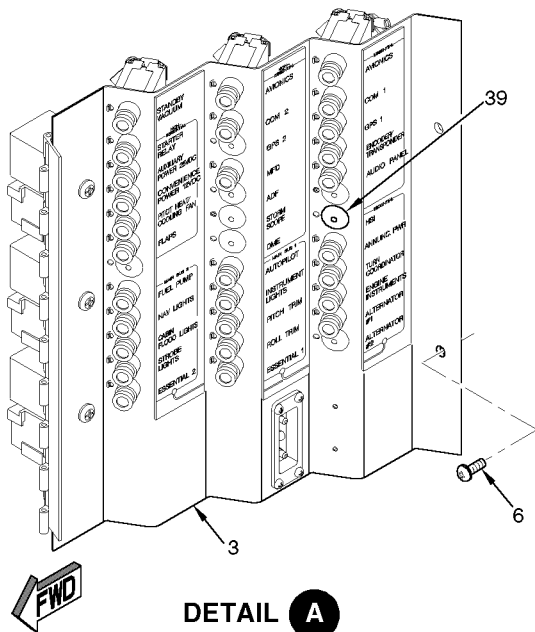
Figure 03 Circuit Breaker Panel Installation
