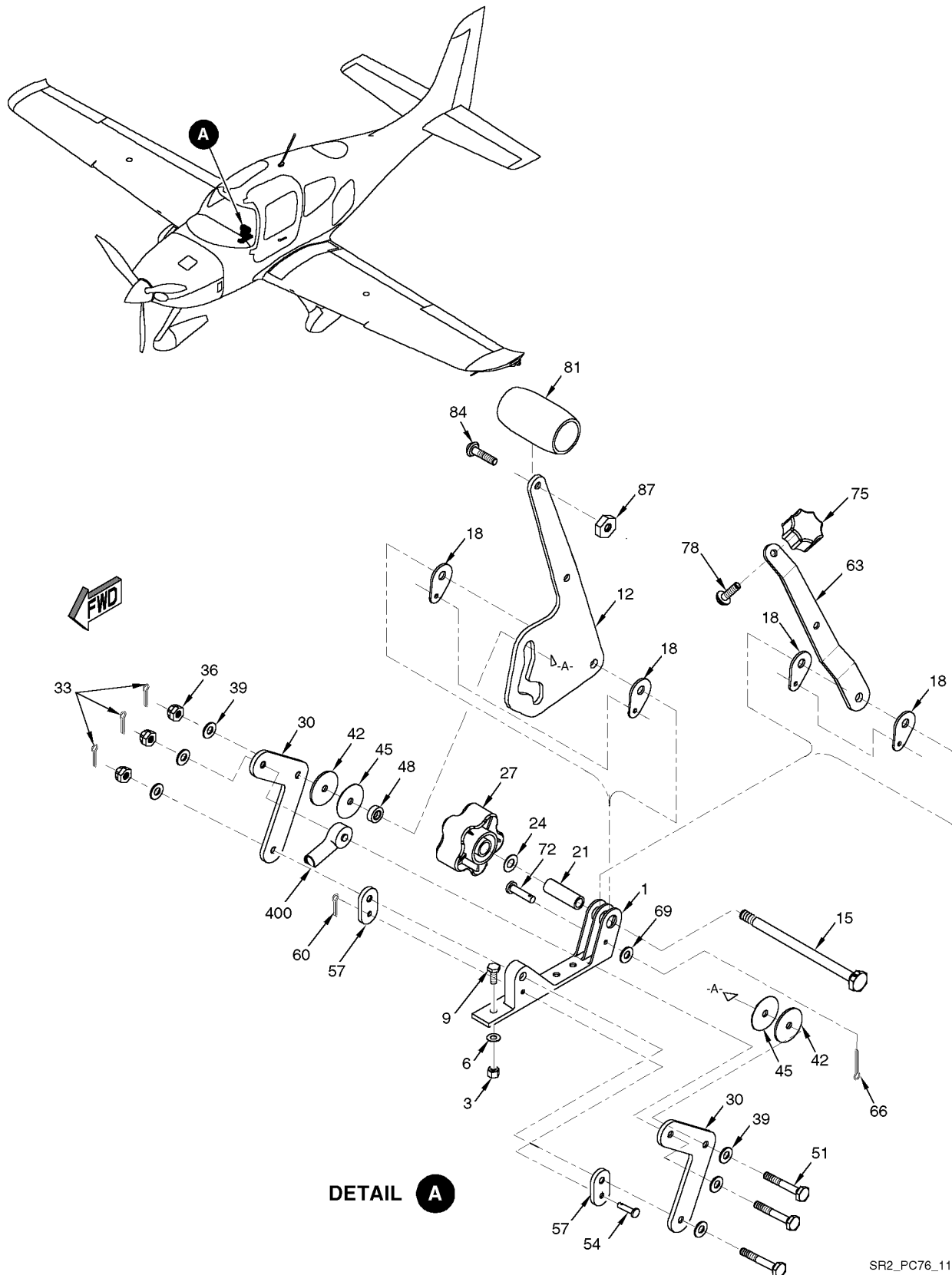
Figure 01 Engine Control Assembly
