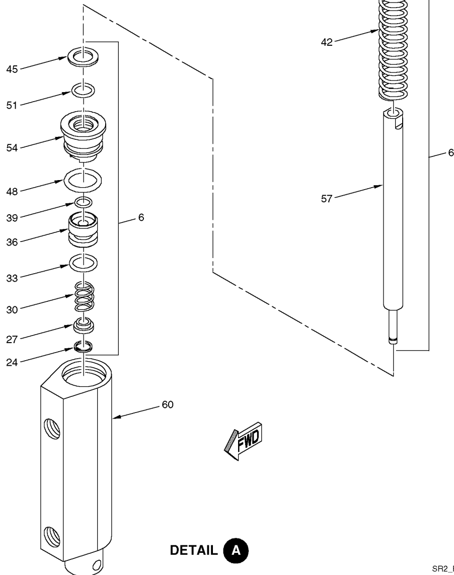
Figure 03 Master Cylinder Assembly
