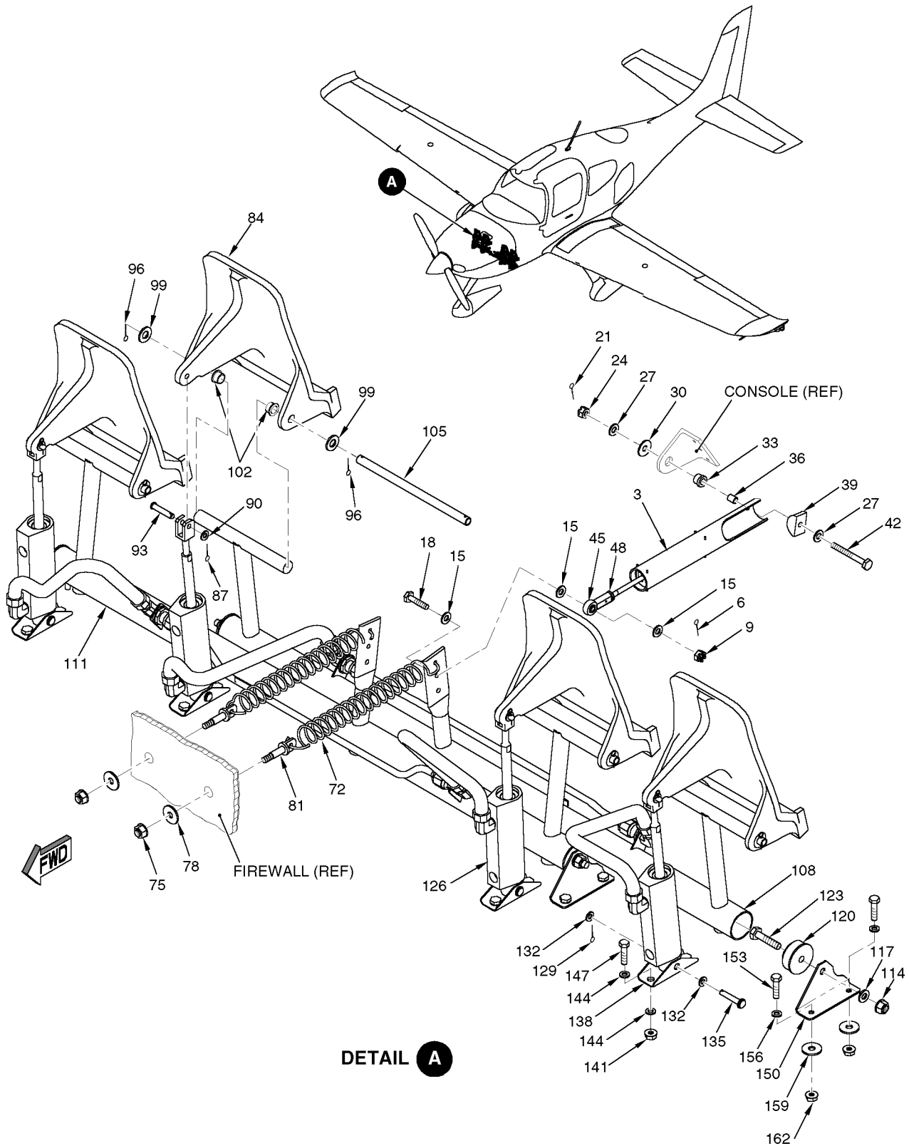
Figure 02 Rudder Pedal Assembly Installation
