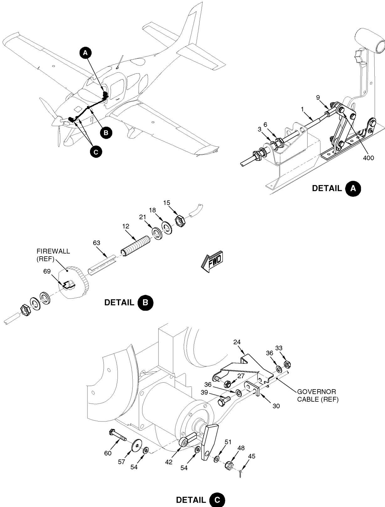
Figure 04 Governor Control Installation
