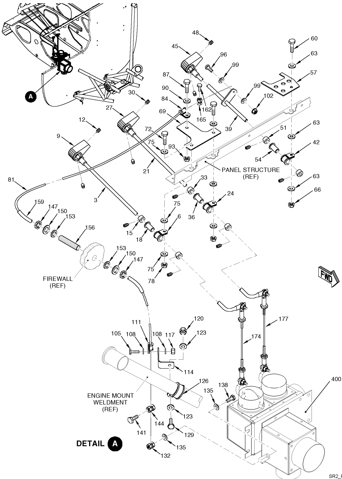
Figure 01 Cabin Air Installation
