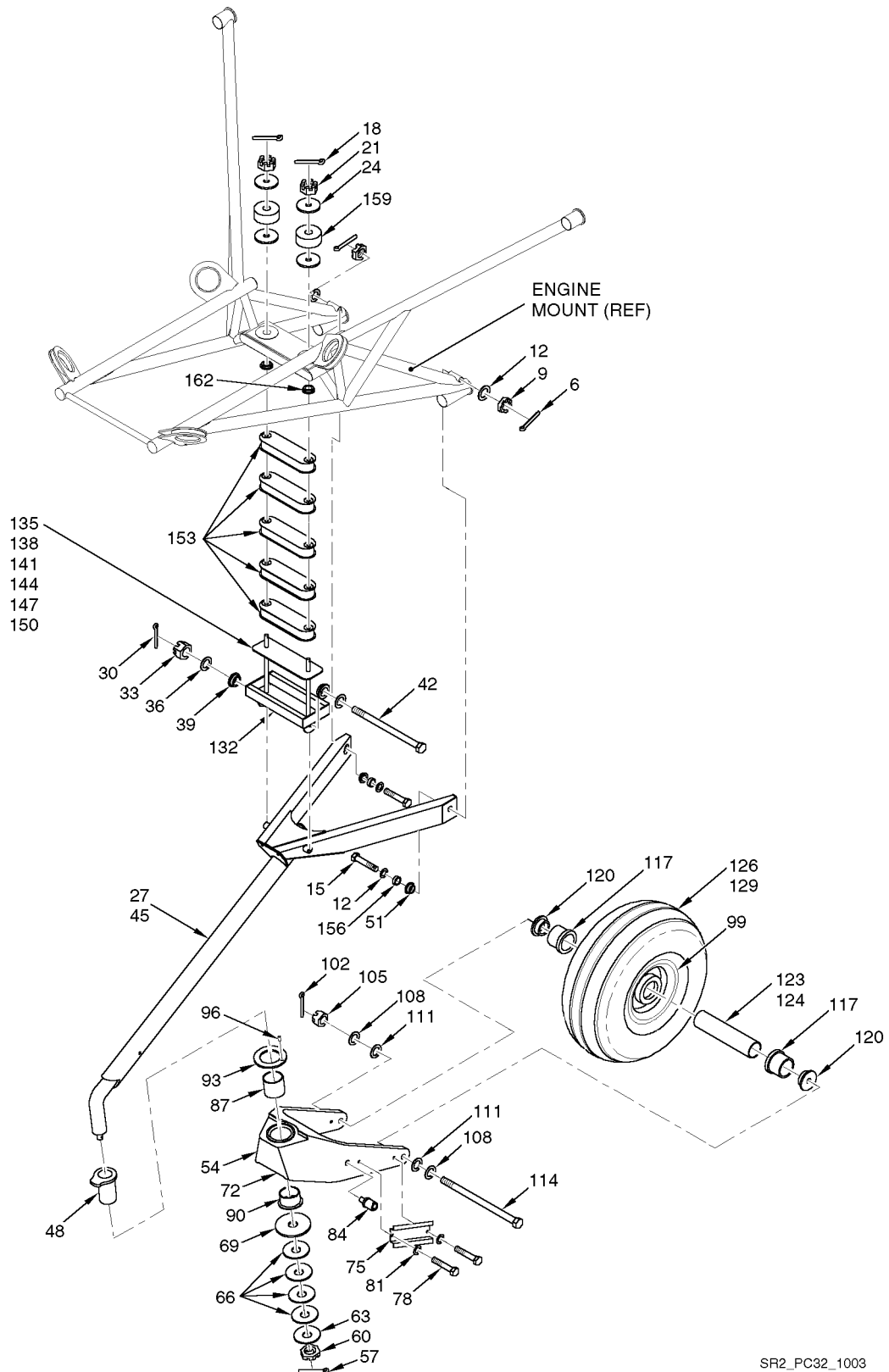
Figure 02 Nose Landing Gear Assembly and Installation
