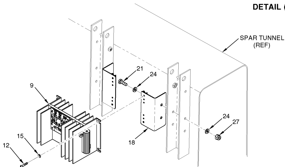
DETAIL C
