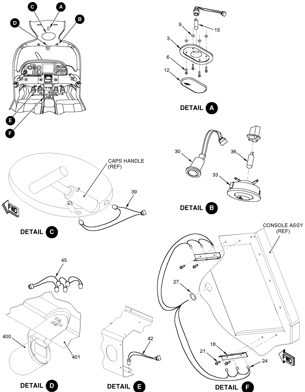
Figure 01 Interior Light Installation
