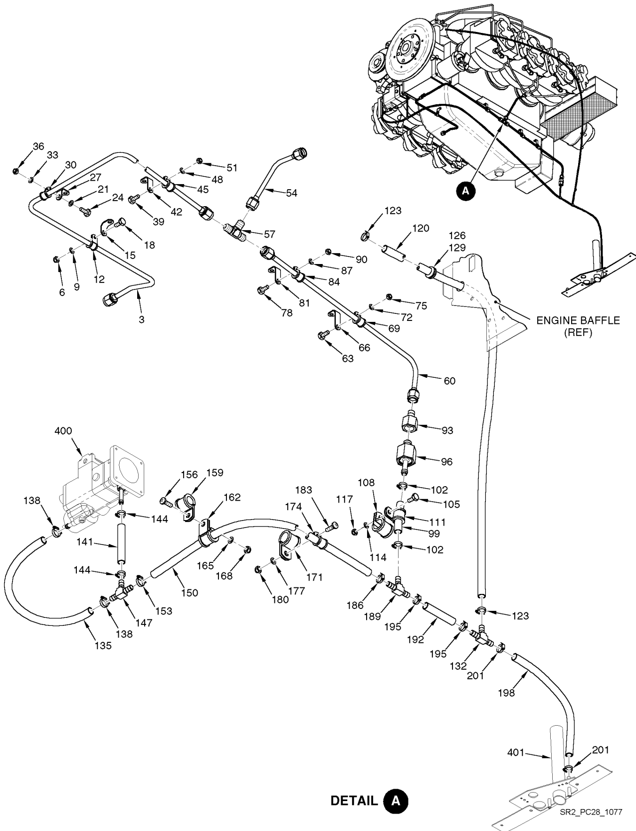
Figure 01 Engine Drains
