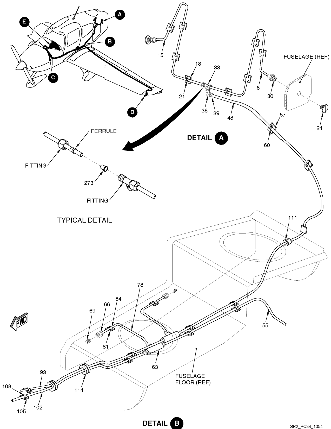
Figure 01 Pitot-Static System and Installations (Sheet 1 of 3)
