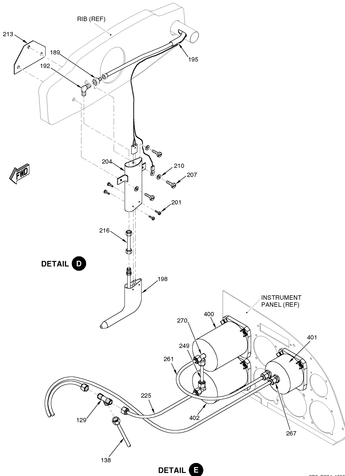
Figure 01 Pitot-Static System and Installations (Sheet 3 of 3)
