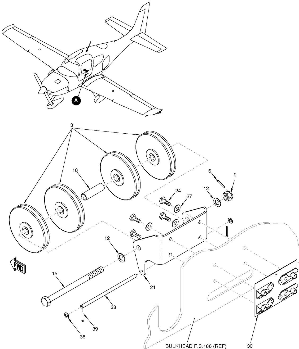
DETAIL A
