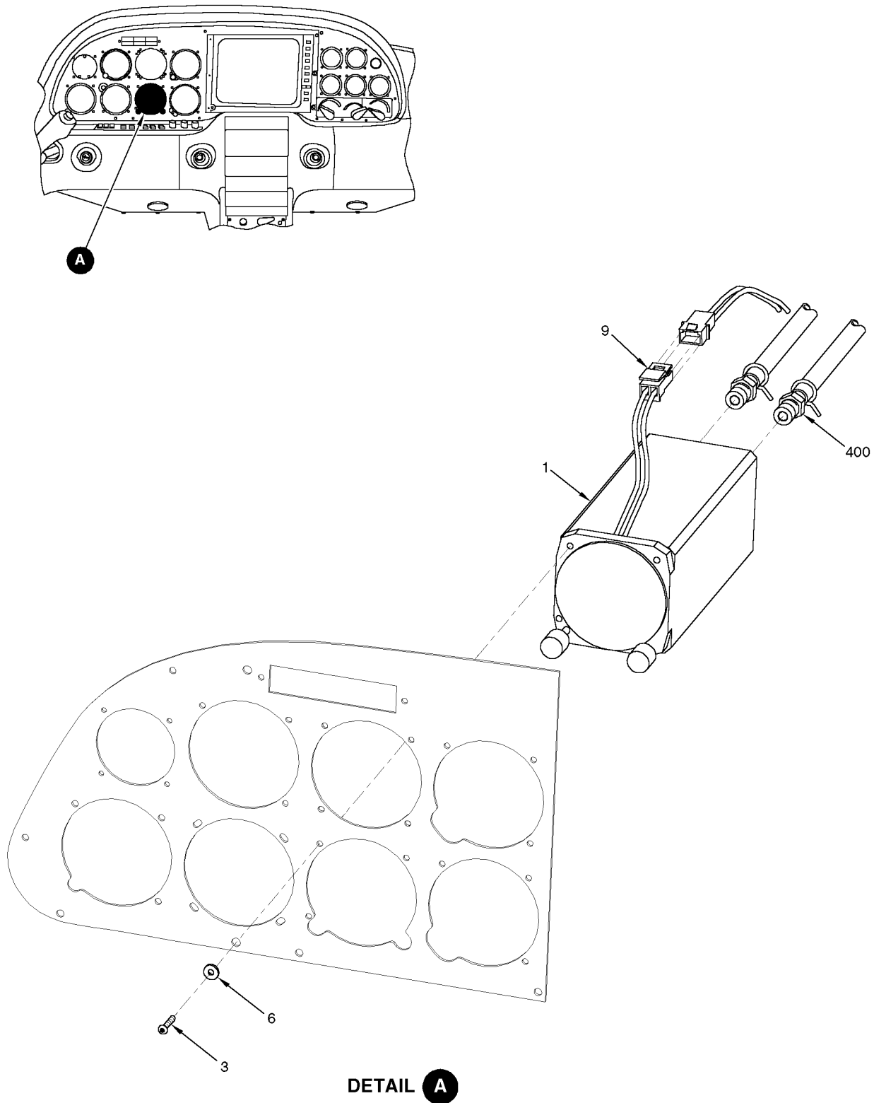
Figure 03 Directional Gyro Installation
