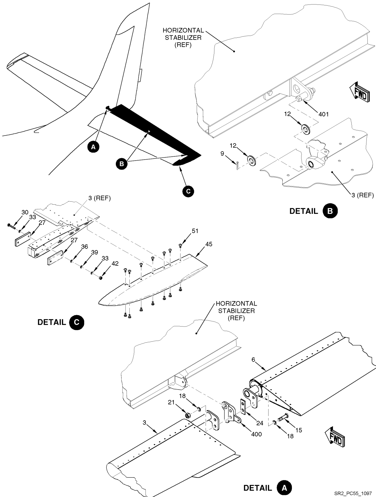
Figure 01 Elevator Installation
