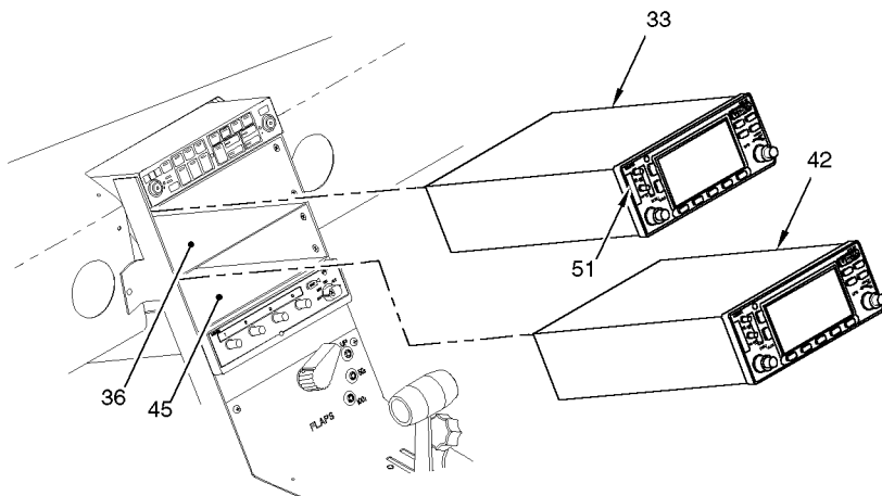
OPTION B
