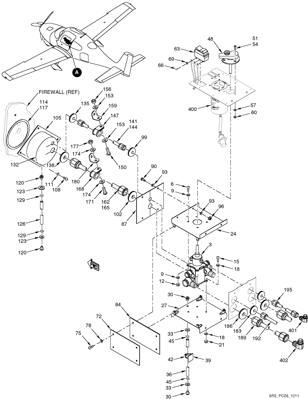
Figure 01 Cabin Fuel System Installation
