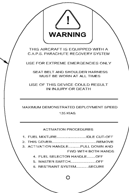
Figure 01 Interior Placards and Overlays (Sheet 3 of 3)
