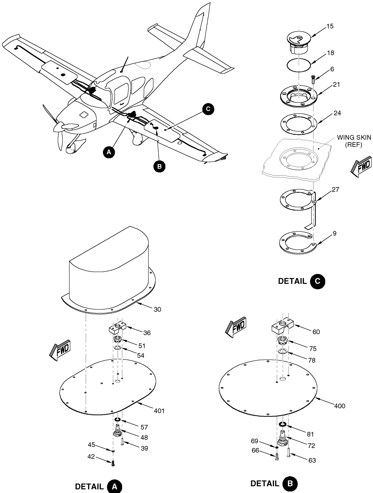
Figure 01 Wing Fuel System Installation
