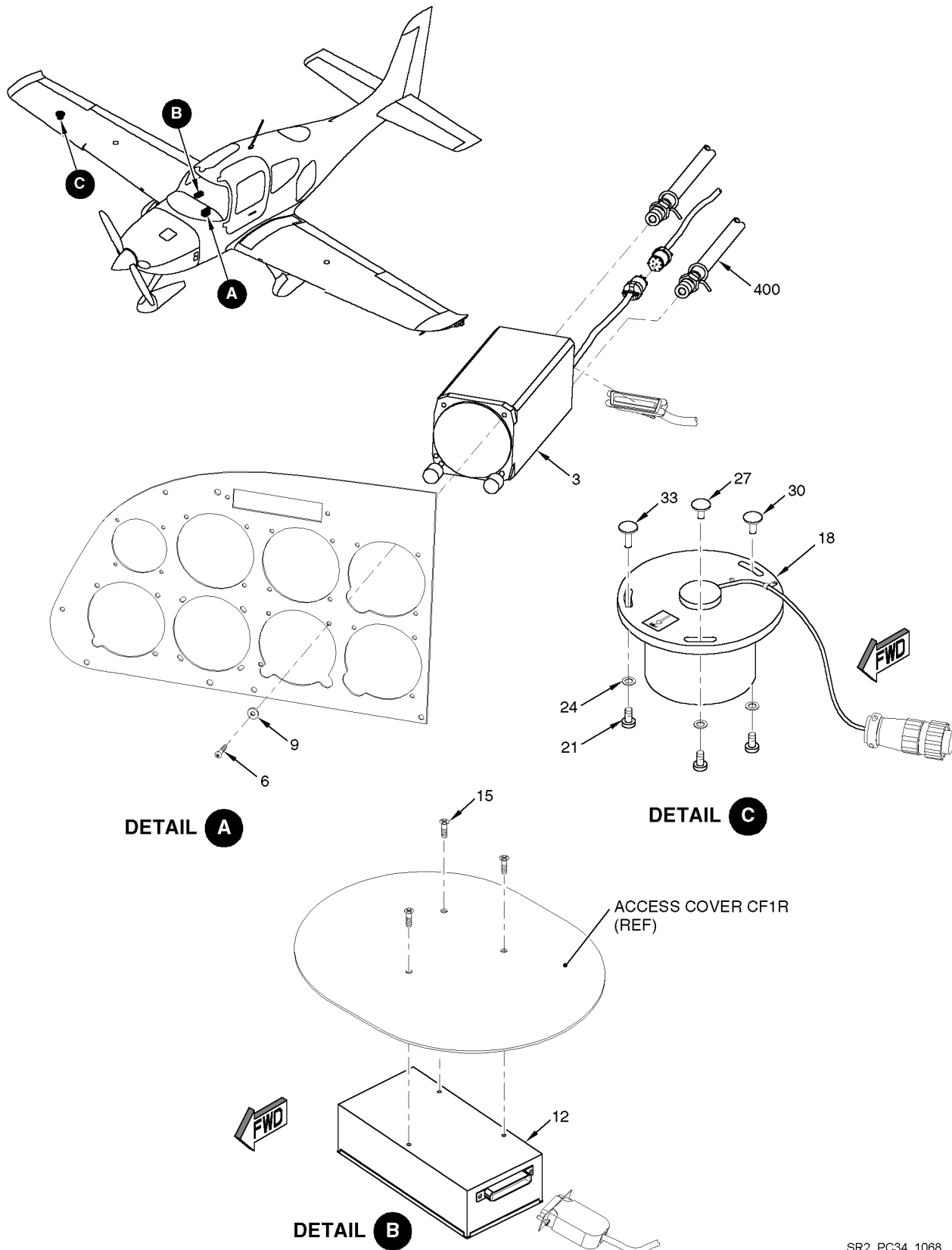
Figure 04 HSI Installation
