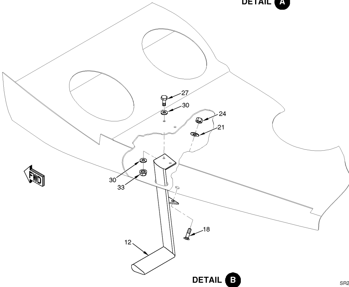
Figure 02 Entry Step and Handle Installation
