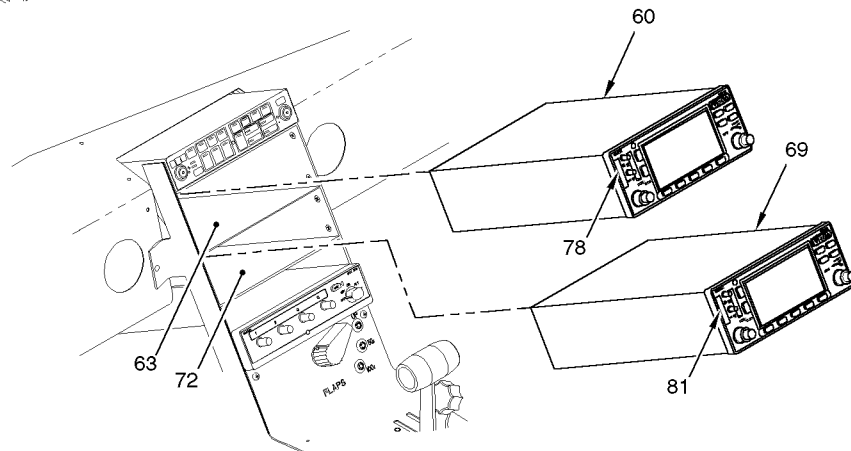
OPTION C
