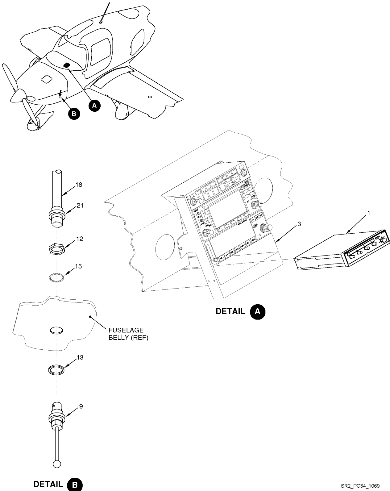
Figure 05 Transponder and Antenna Installations
