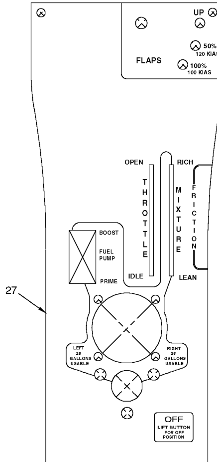
DETAIL F
