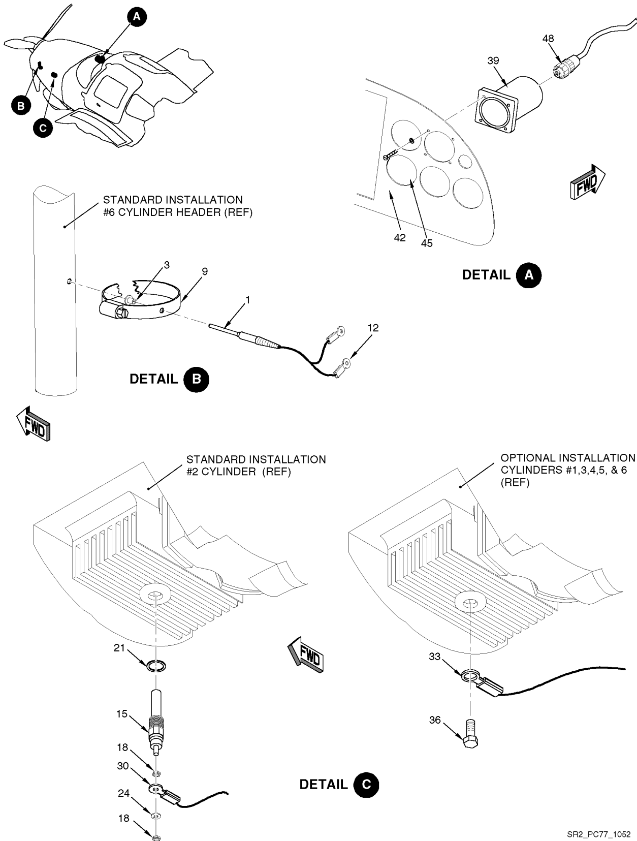
Figure 01 EGT, CHT Sensors and Gage Installations
