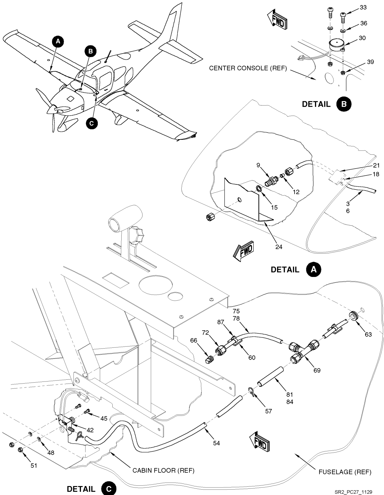
Figure 01 Stall Warning System
