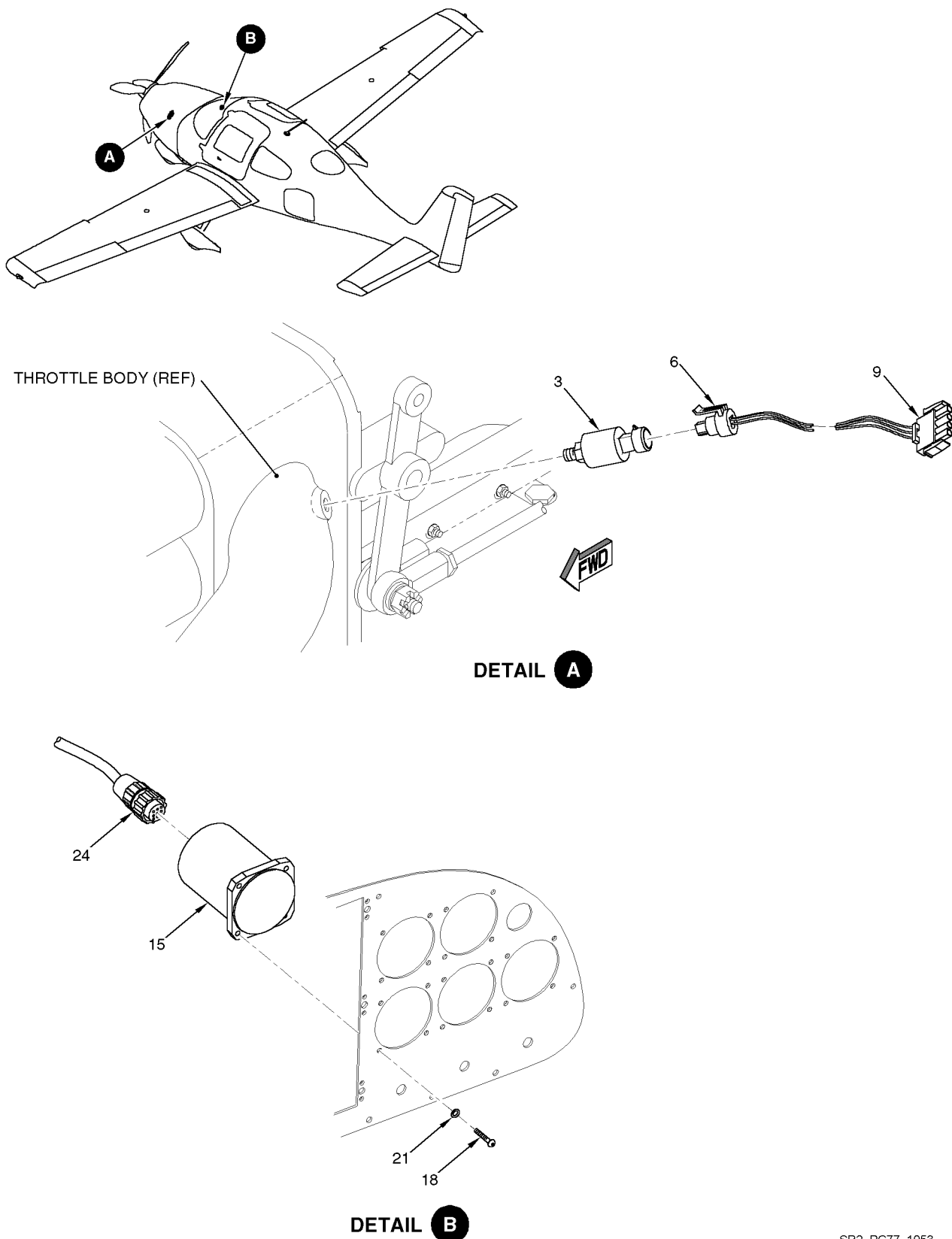
Figure 02 MAP Sensor and MAP/Fuel Flow Gage Installations
