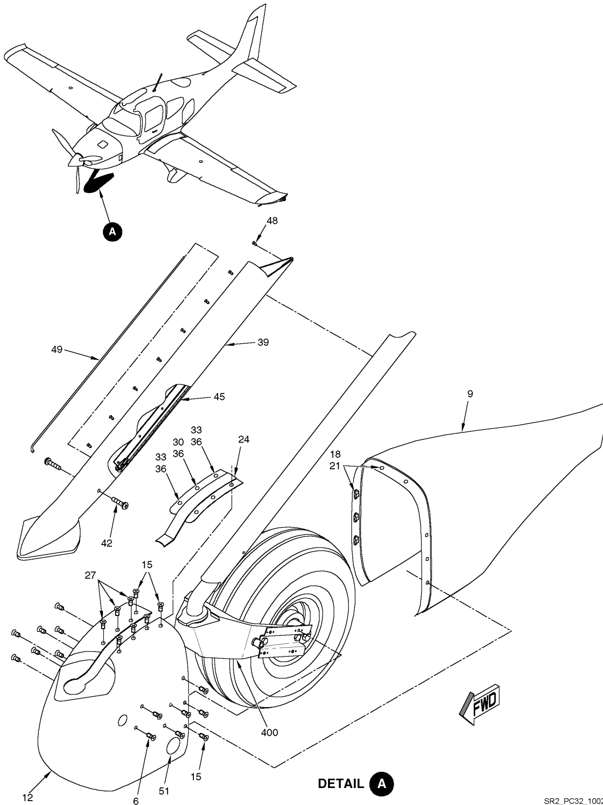
Figure 01 Nose Landing Gear Fairing Assembly and Installation
