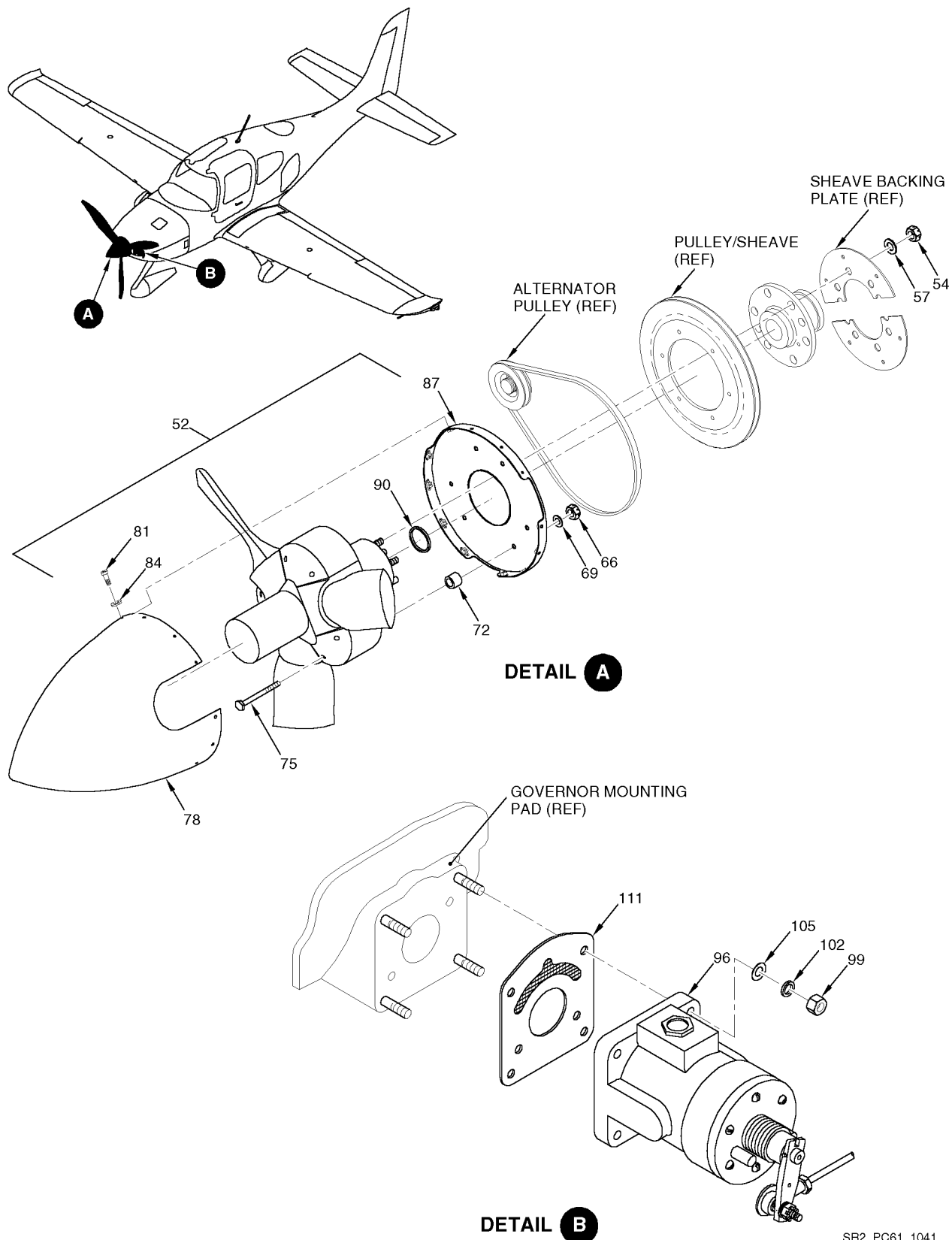
Figure 01 Propeller Installation
