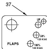
DETAIL G
