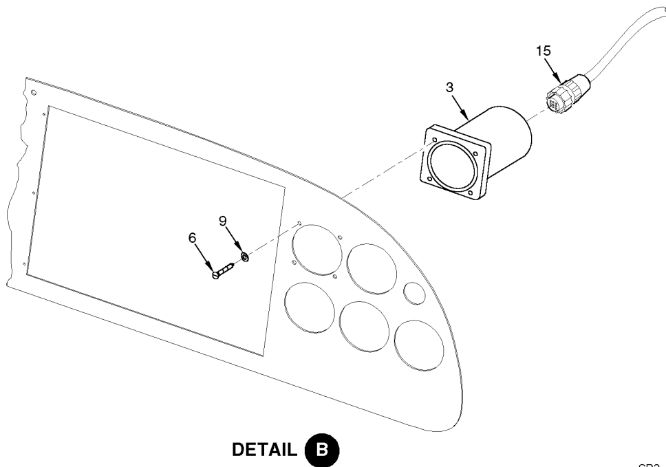
Figure 01 Tachometer and Sensor Installation
