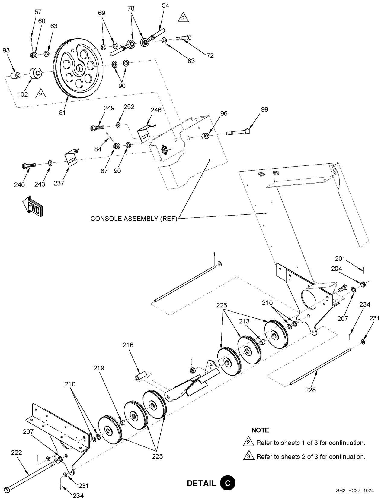
Figure 02 Flight Control Installation (Sheet 3 of 3)
