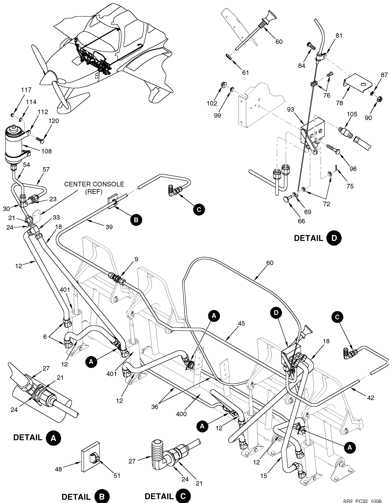
Figure 01 Brake System Installation
