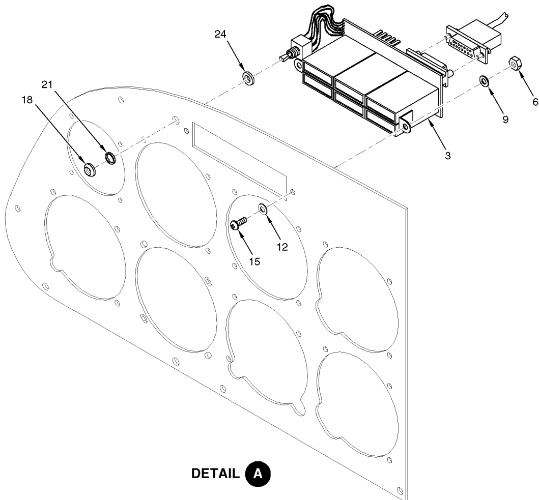
Figure 01 Annunciator Panel Installation
