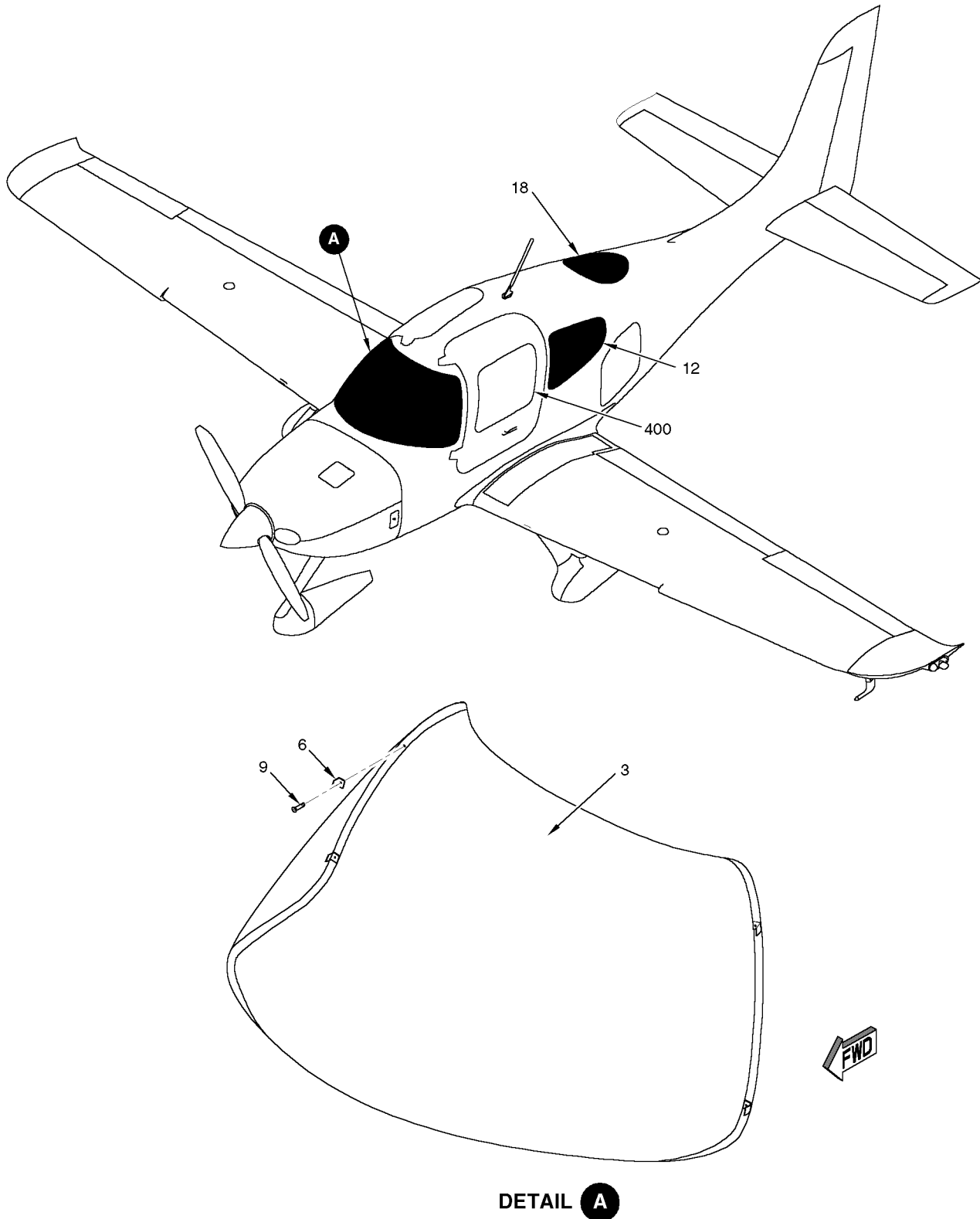
Figure 01 Fuselage Window Installation
