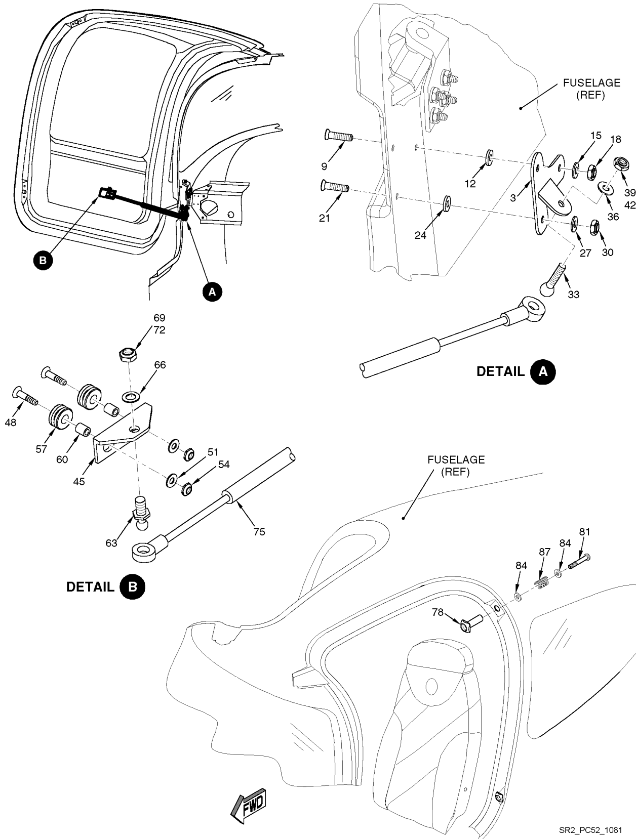
Figure 03 Gas Strut and Door Pin Receiver Installation
