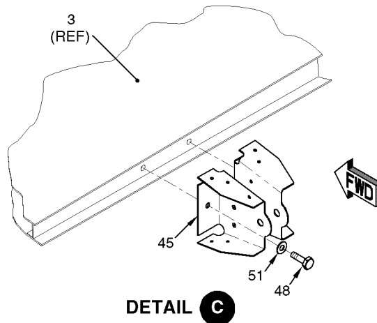
Figure 01 Horizontal Stabilizer
