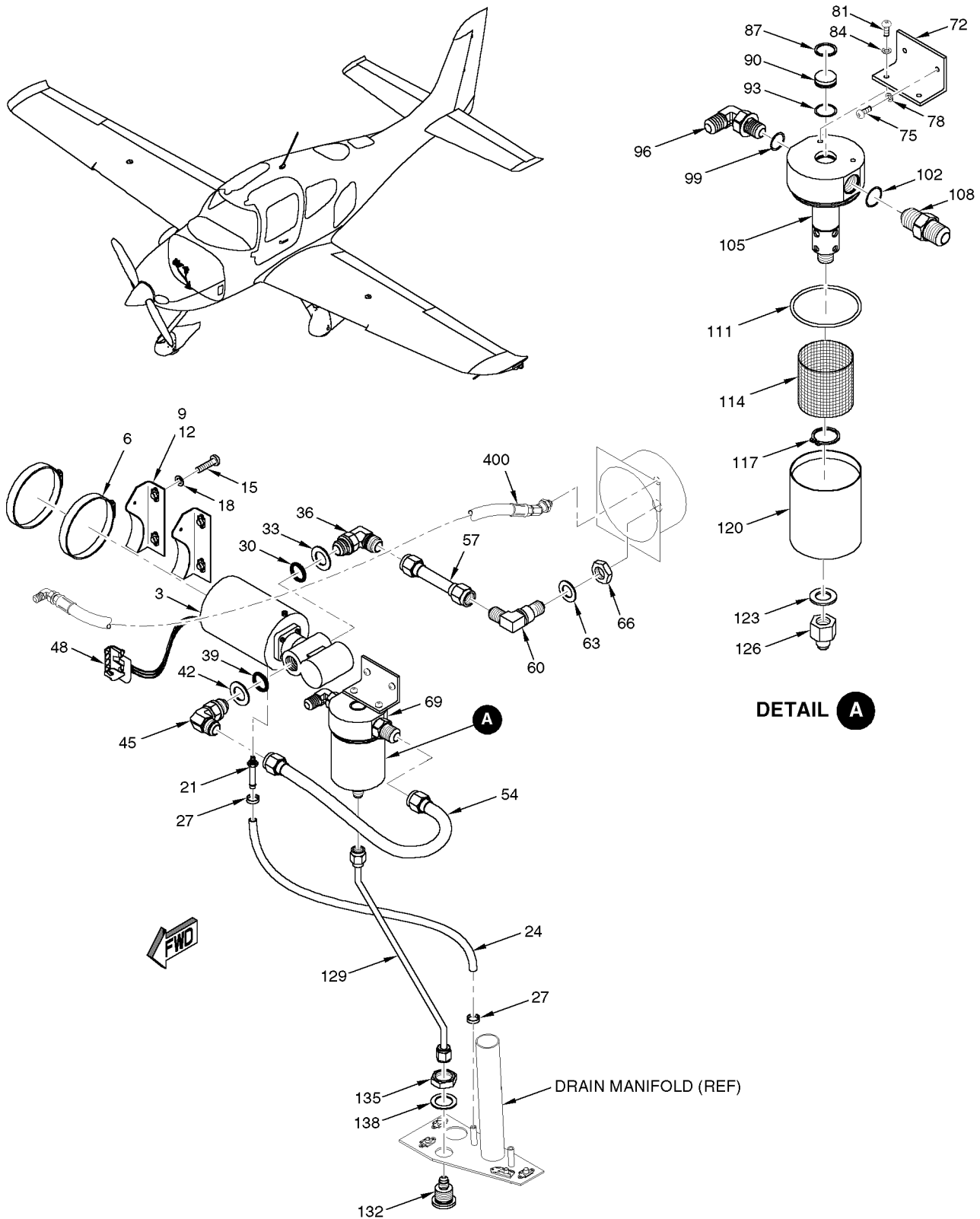
Figure 02 Gascolator and Electric Fuel Pump Installation
