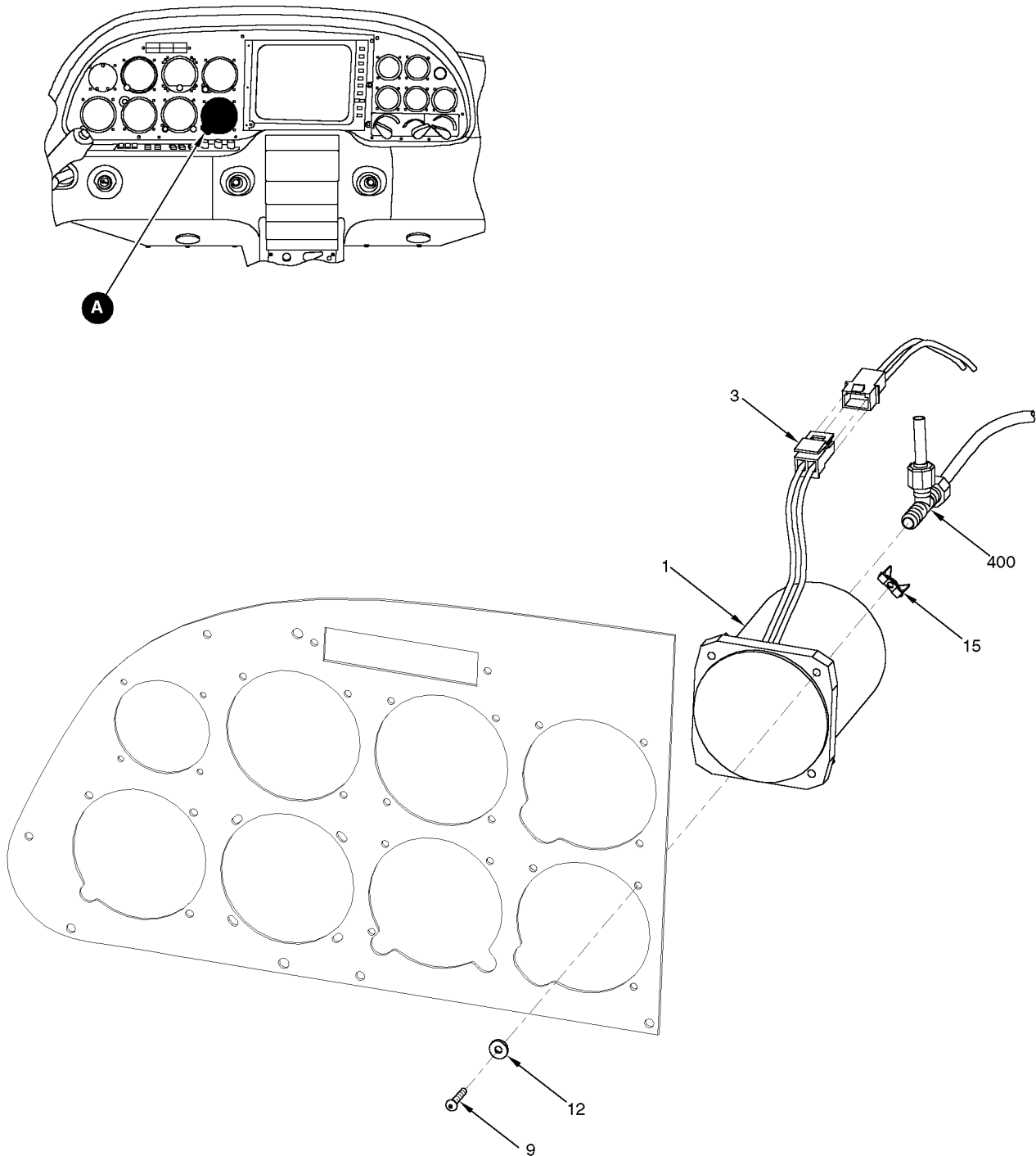
DETAIL A
