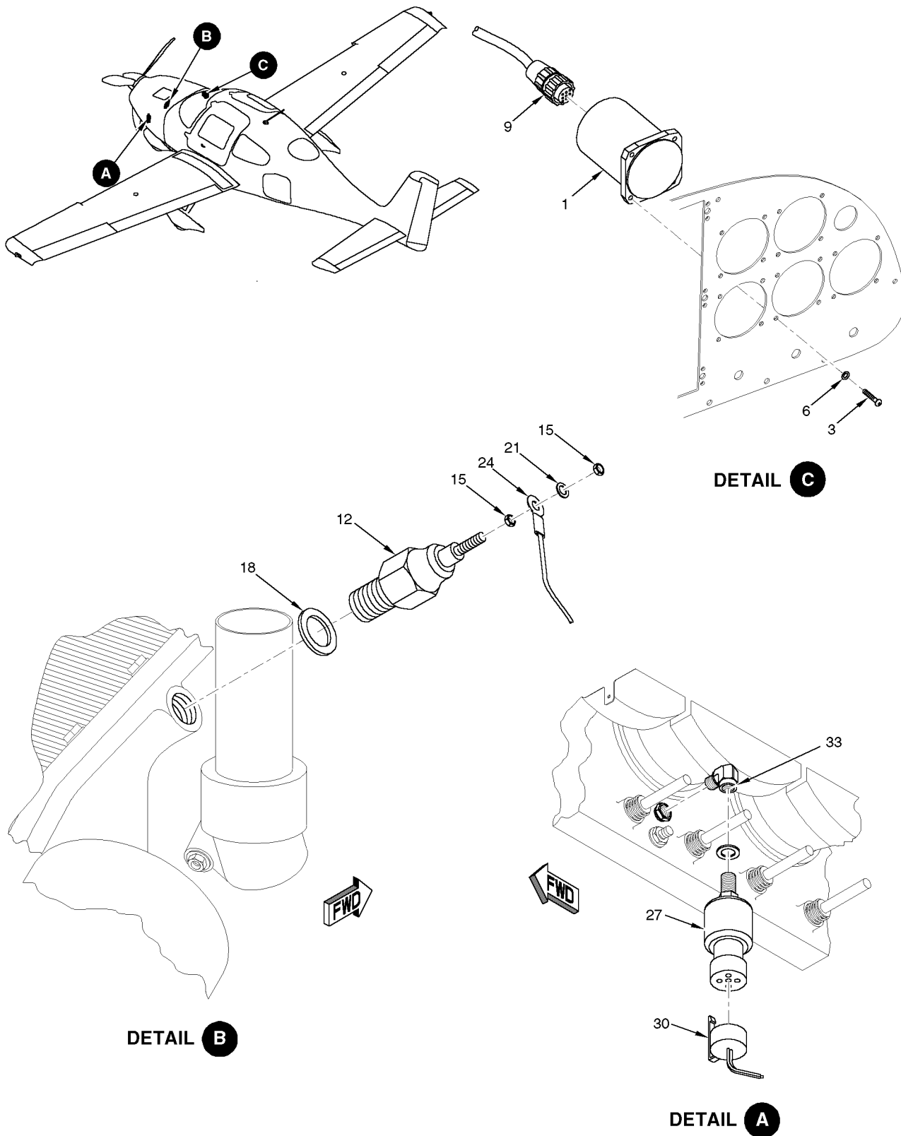
Figure 01 Oil Pressure/Temperature Sensors and Gage Installation
