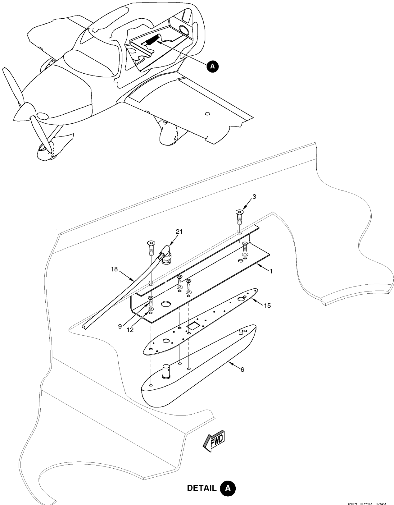
Figure 01 Marker Beacon Antenna Installation
