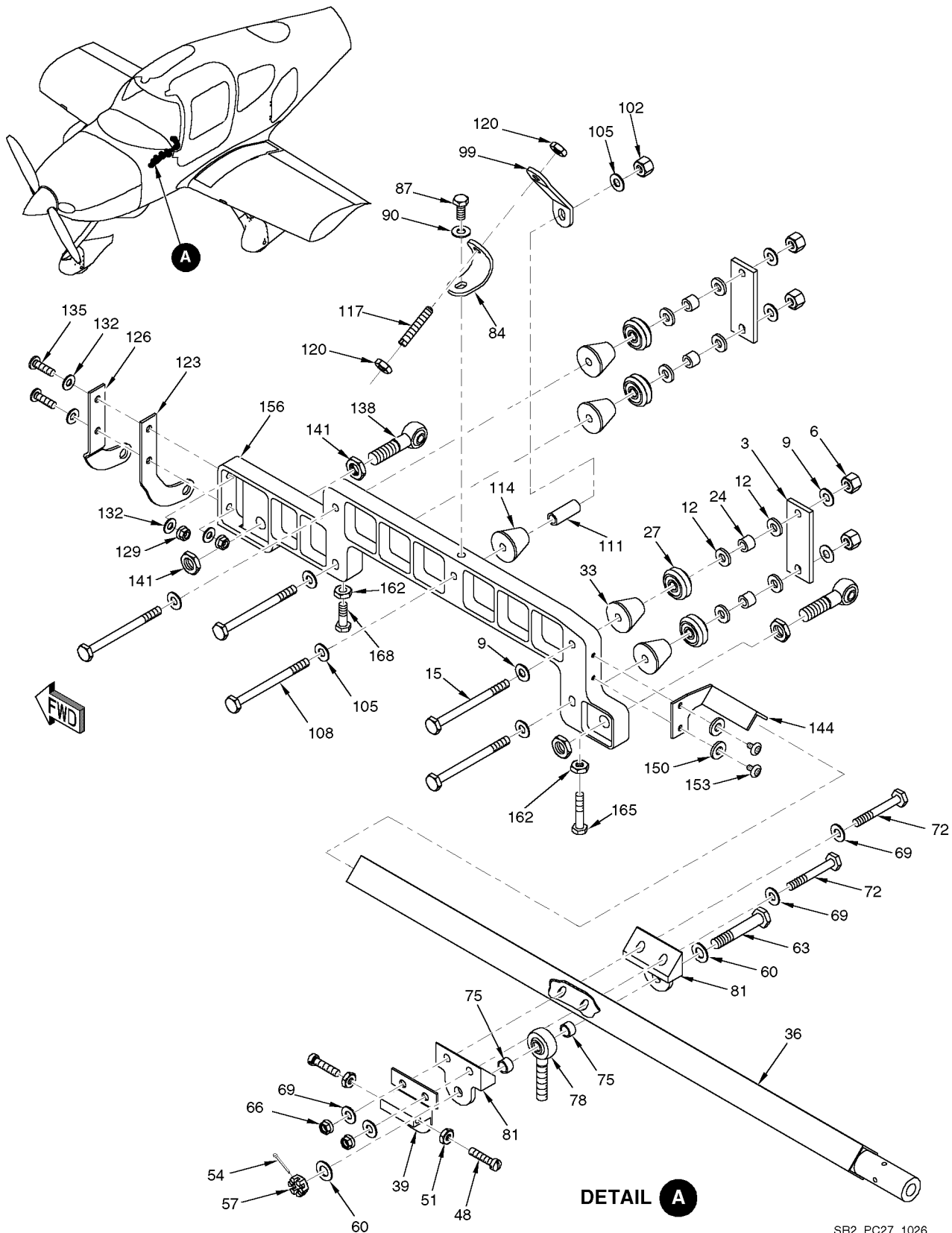
Figure 04 Yoke Assembly
