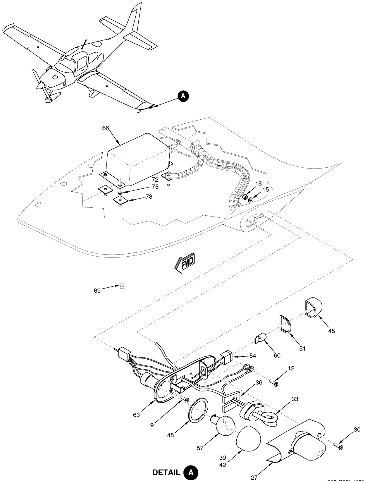
Figure 02 Anti-Collision Light and Module Installation
