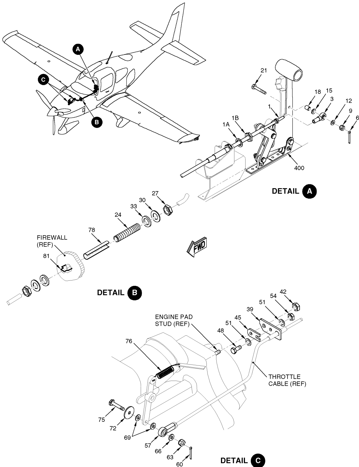
Figure 03 Throttle Control Installation
