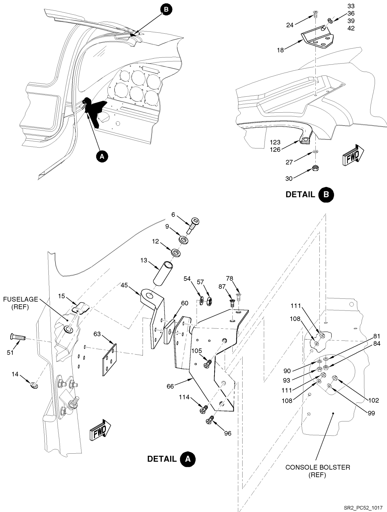
Figure 01 Cabin Door Installation
