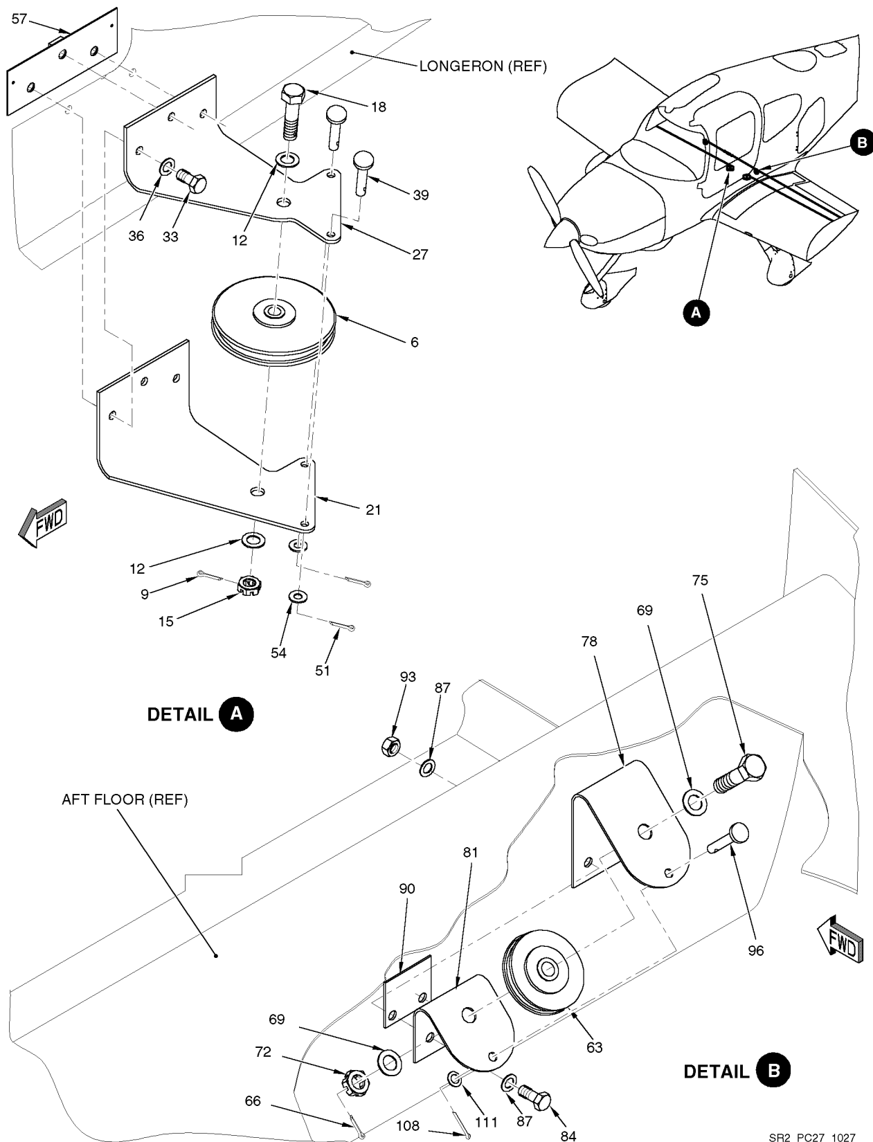
Figure 02 Aileron System Pulleys
