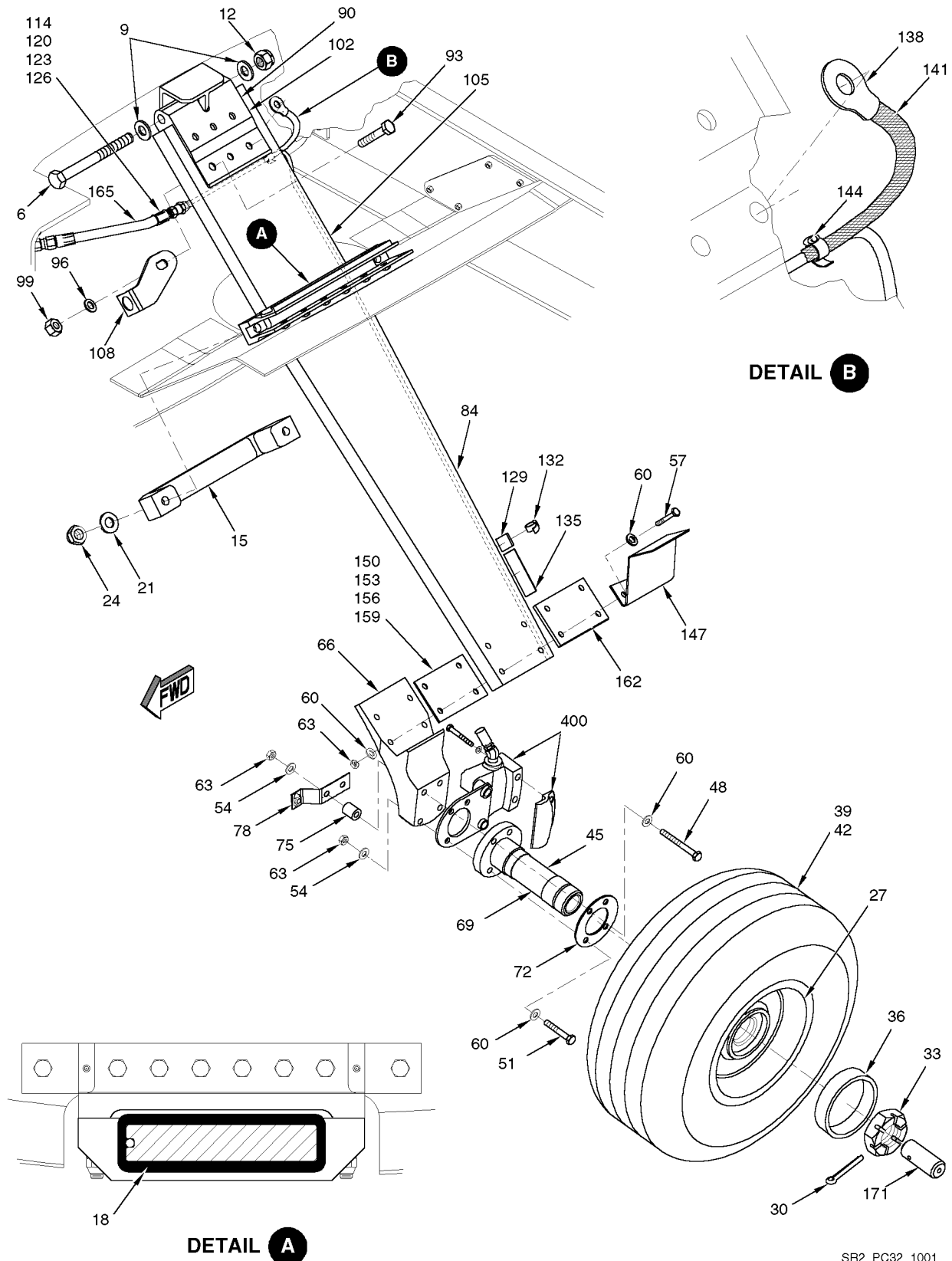
Figure 02 Main Landing Gear Assembly and Installation
