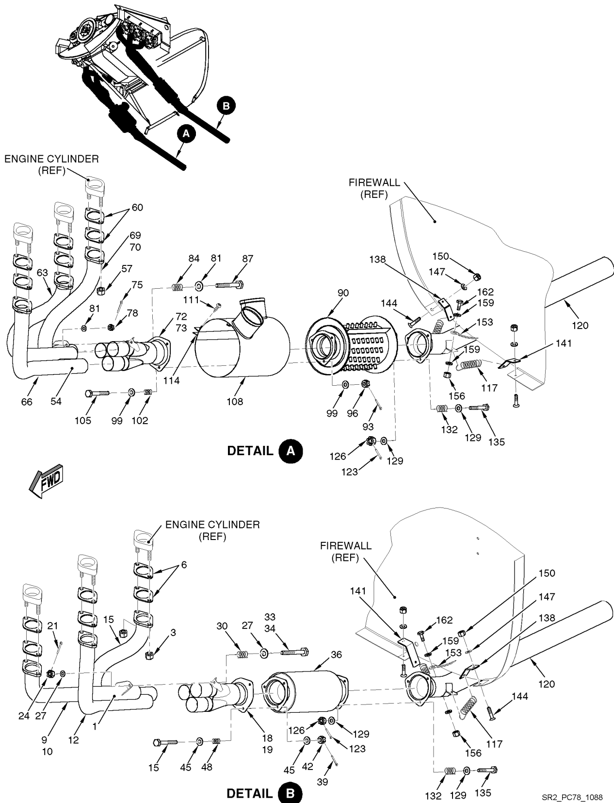
Figure 01 Exhaust System Installation
