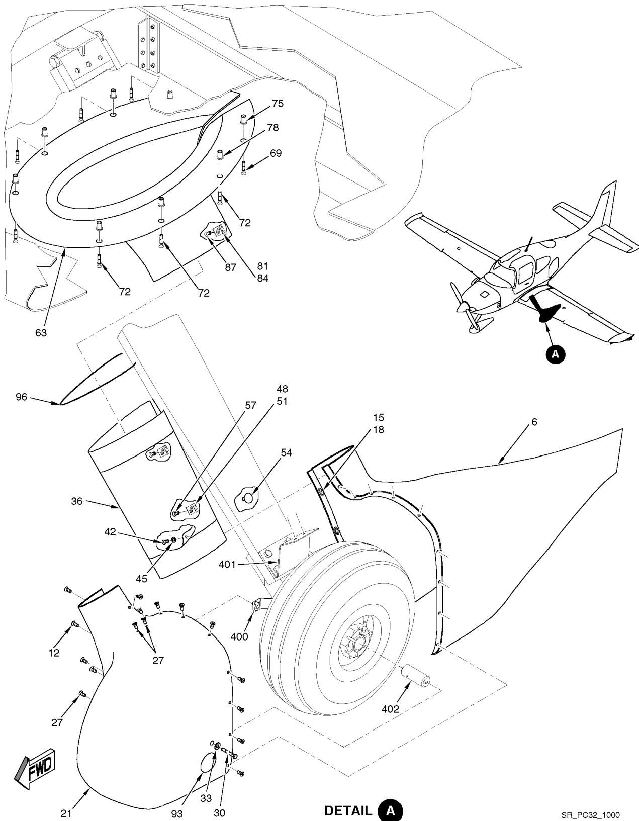
Figure 01 Main Landing Gear Fairing Assembly and Installation
