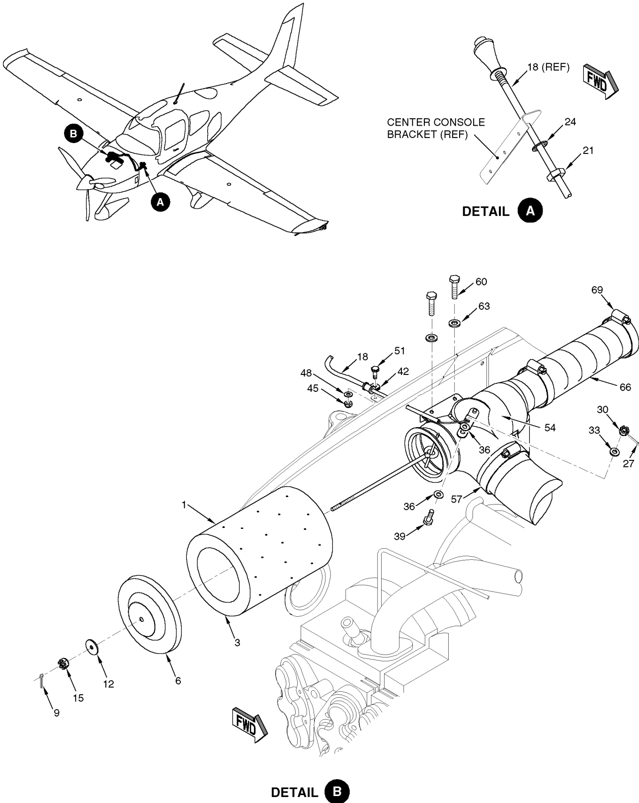
Figure 01 Induction System Installation
