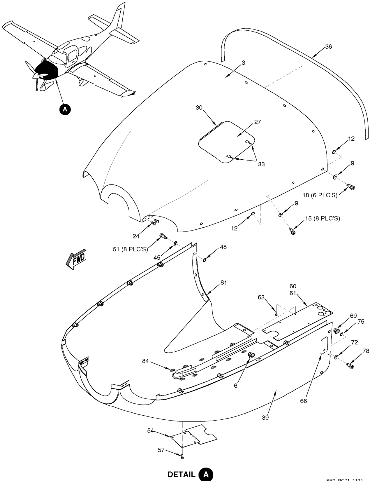
Figure 01 Engine Cowling Installation
