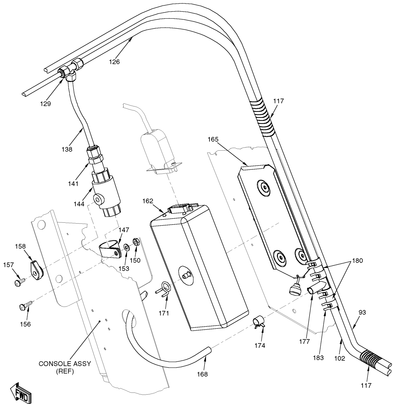
DETAIL C
