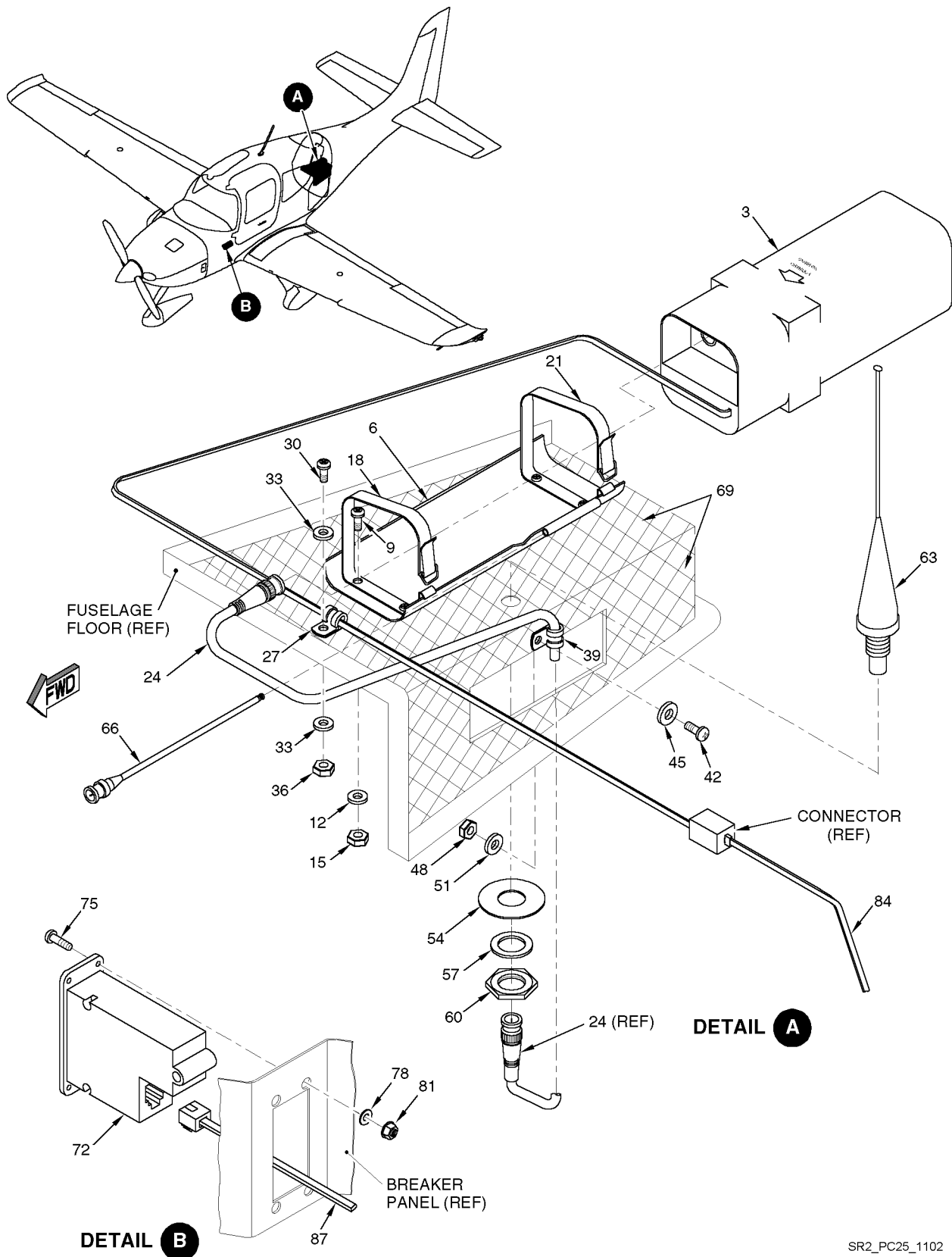
Figure 01 ELT Installation
