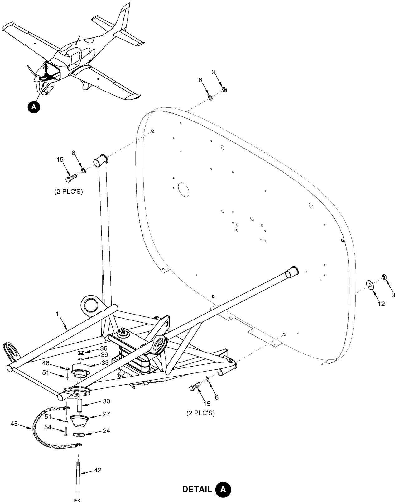
Figure 01 Engine Mount and Isolator Installation
