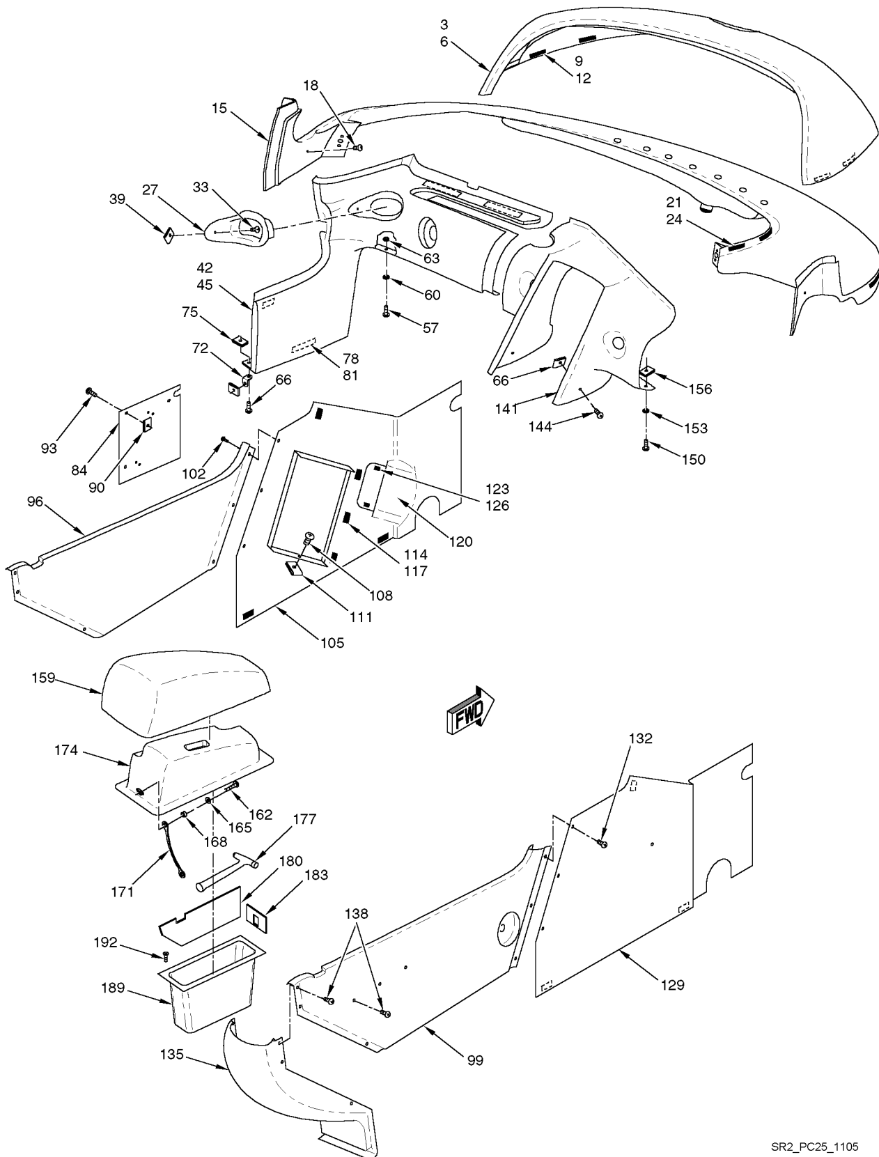
Figure 03 Console Installation
