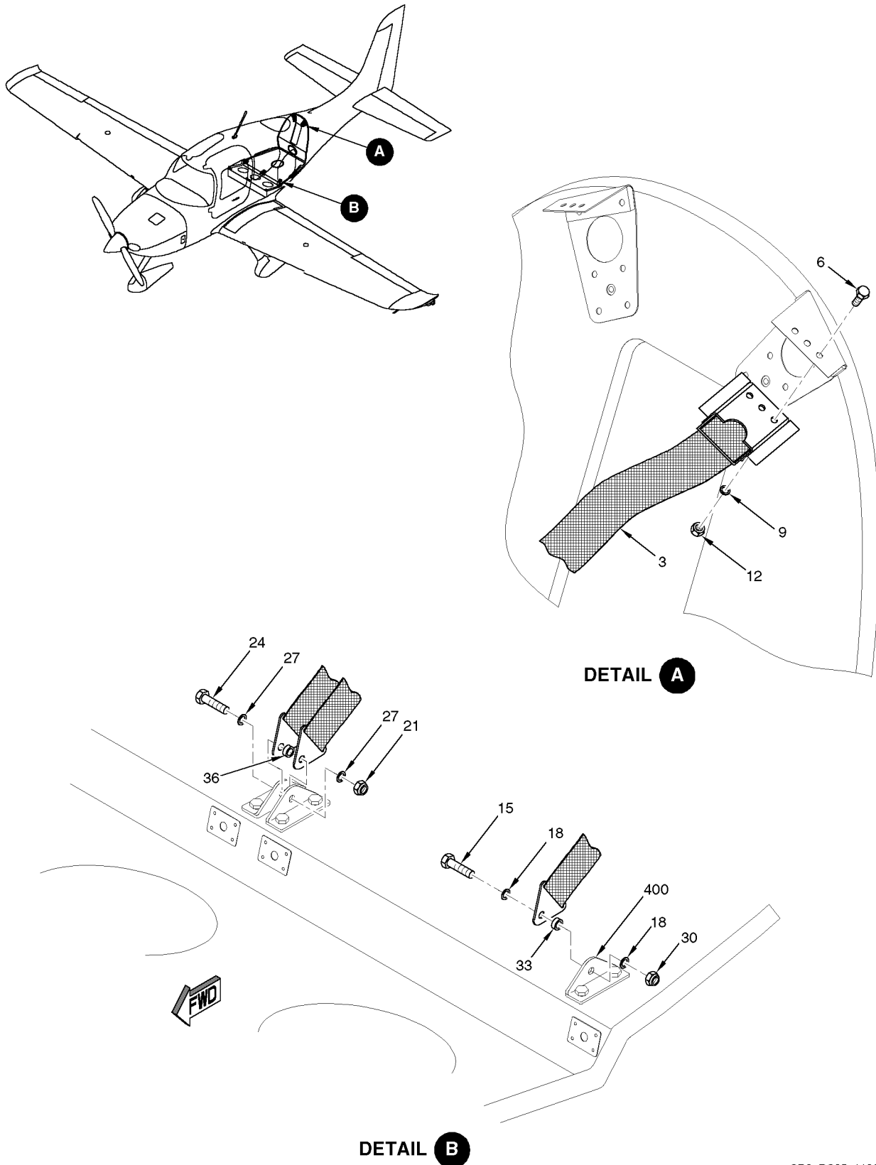
Figure 04 Seat Belt and Shoulder Harness Installation
