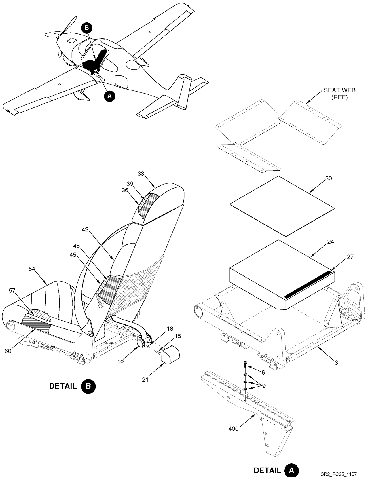
Figure 05 Forward Seats
