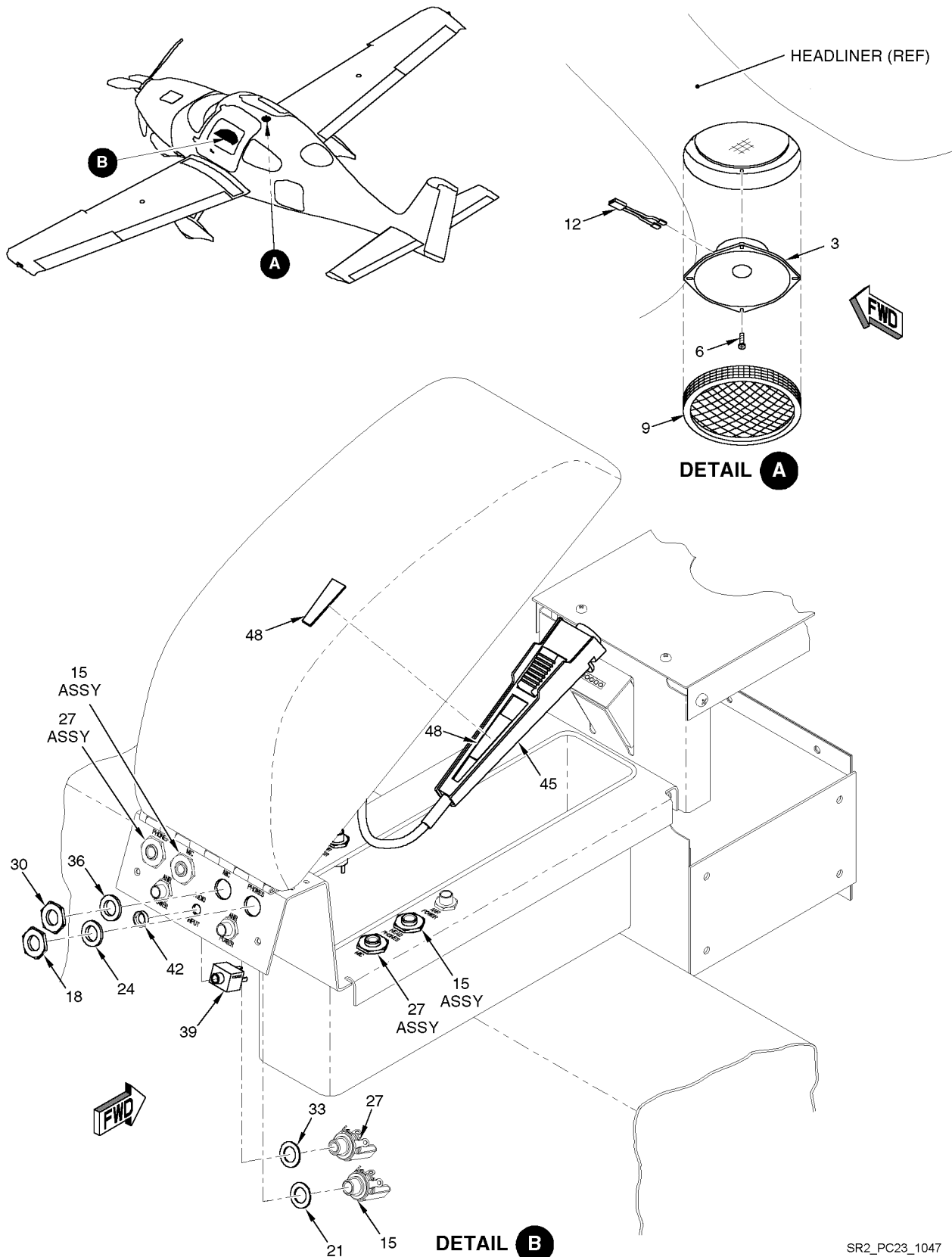
Figure 01 Audio Integration
