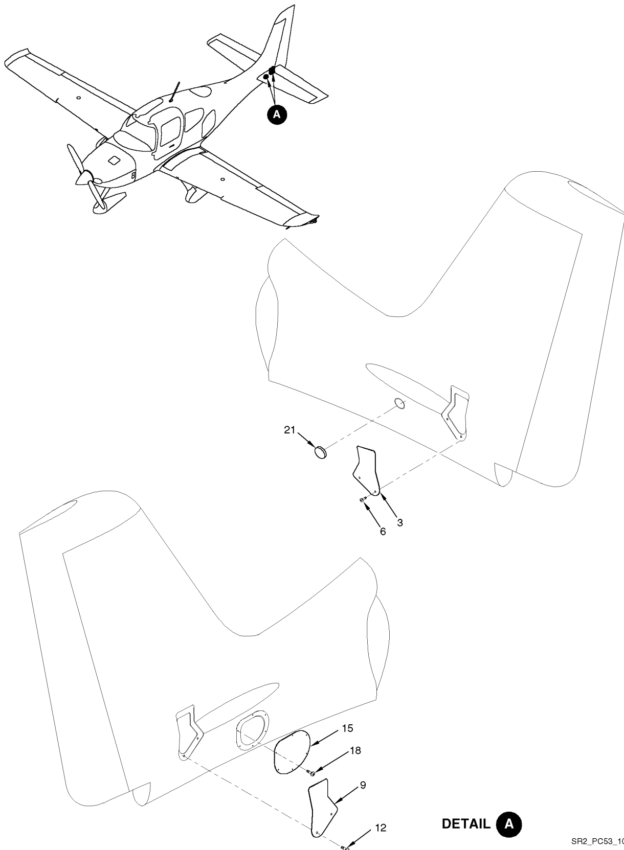
Figure 01 Access Panel Installation - Empennage
