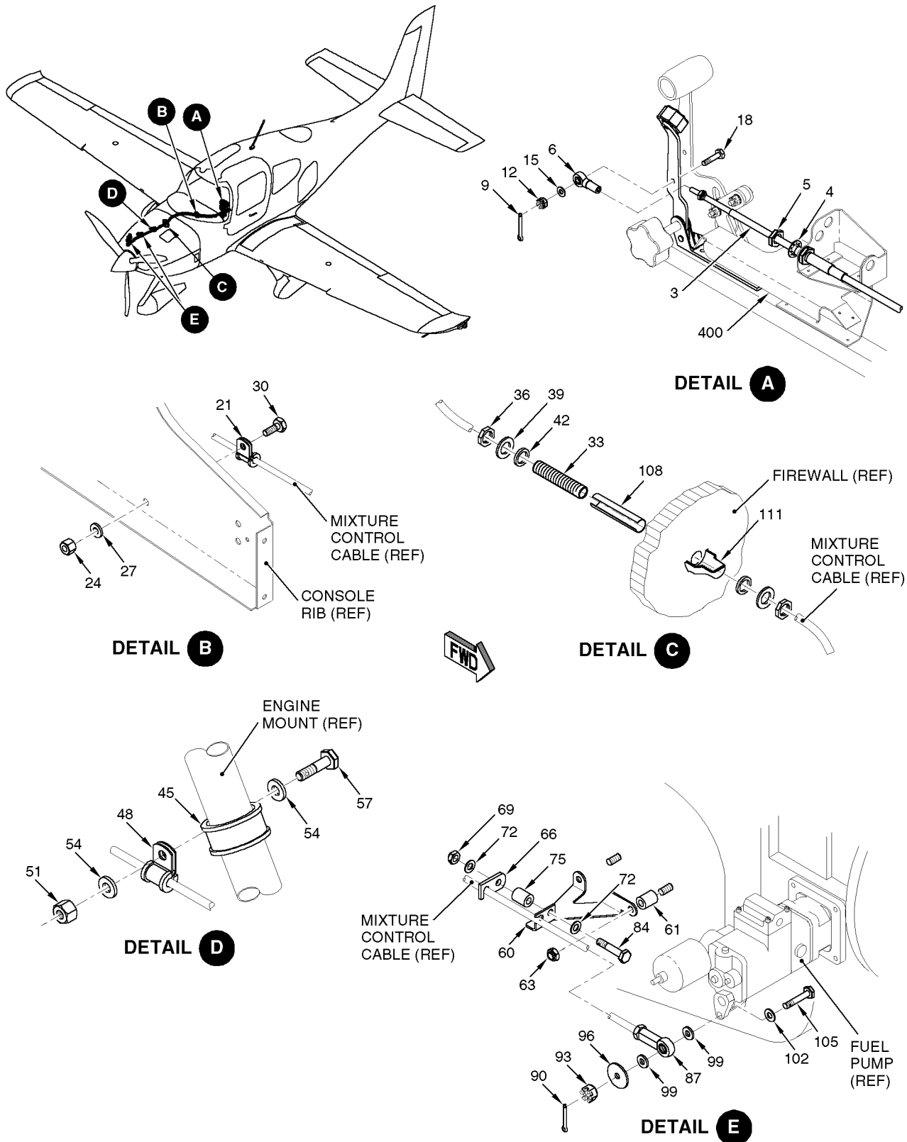
Figure 02 Mixture Control Installation
