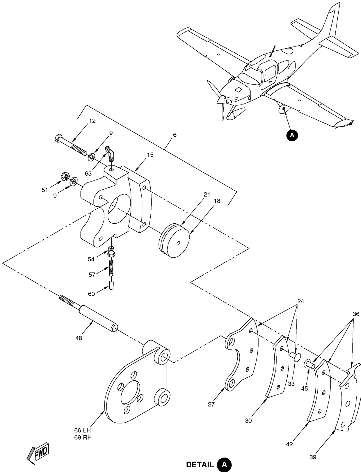
Figure 02 Brake Assembly
