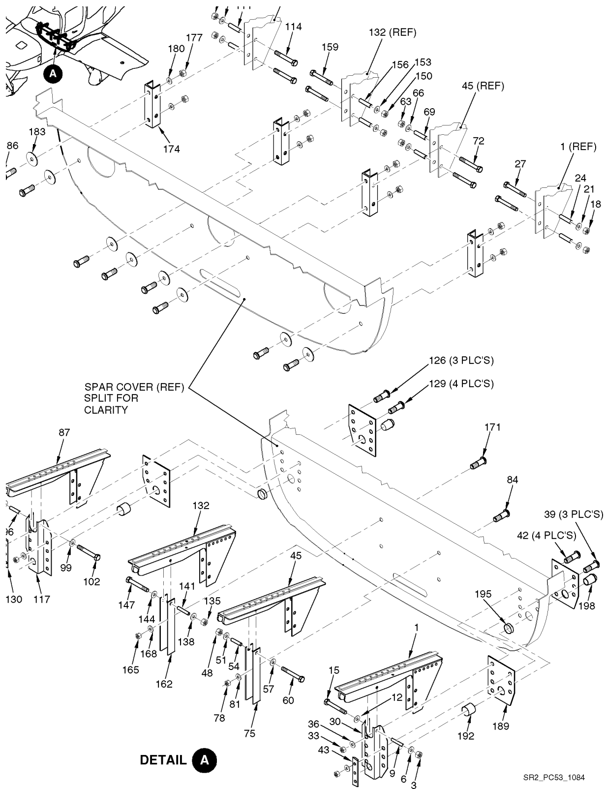
Figure 01 Seat Rail Installation
