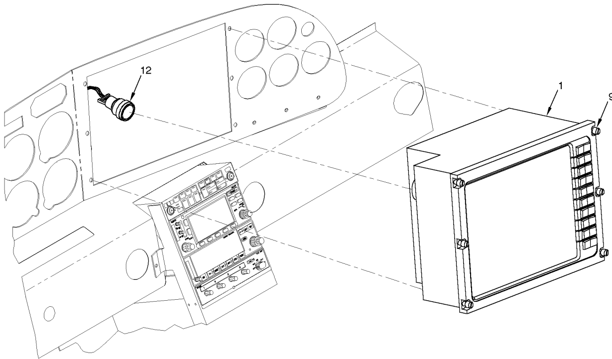
DETAIL A
