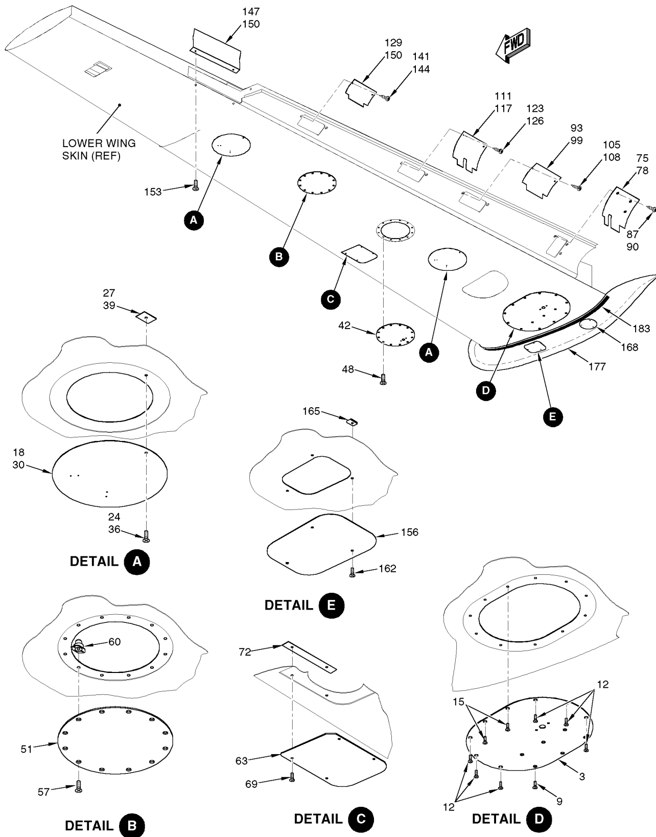
Figure 01 Lower Wing Access Panel Installation
