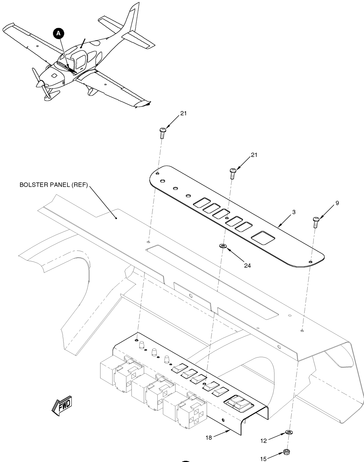
DETAIL A
