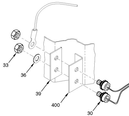
DETAIL B
