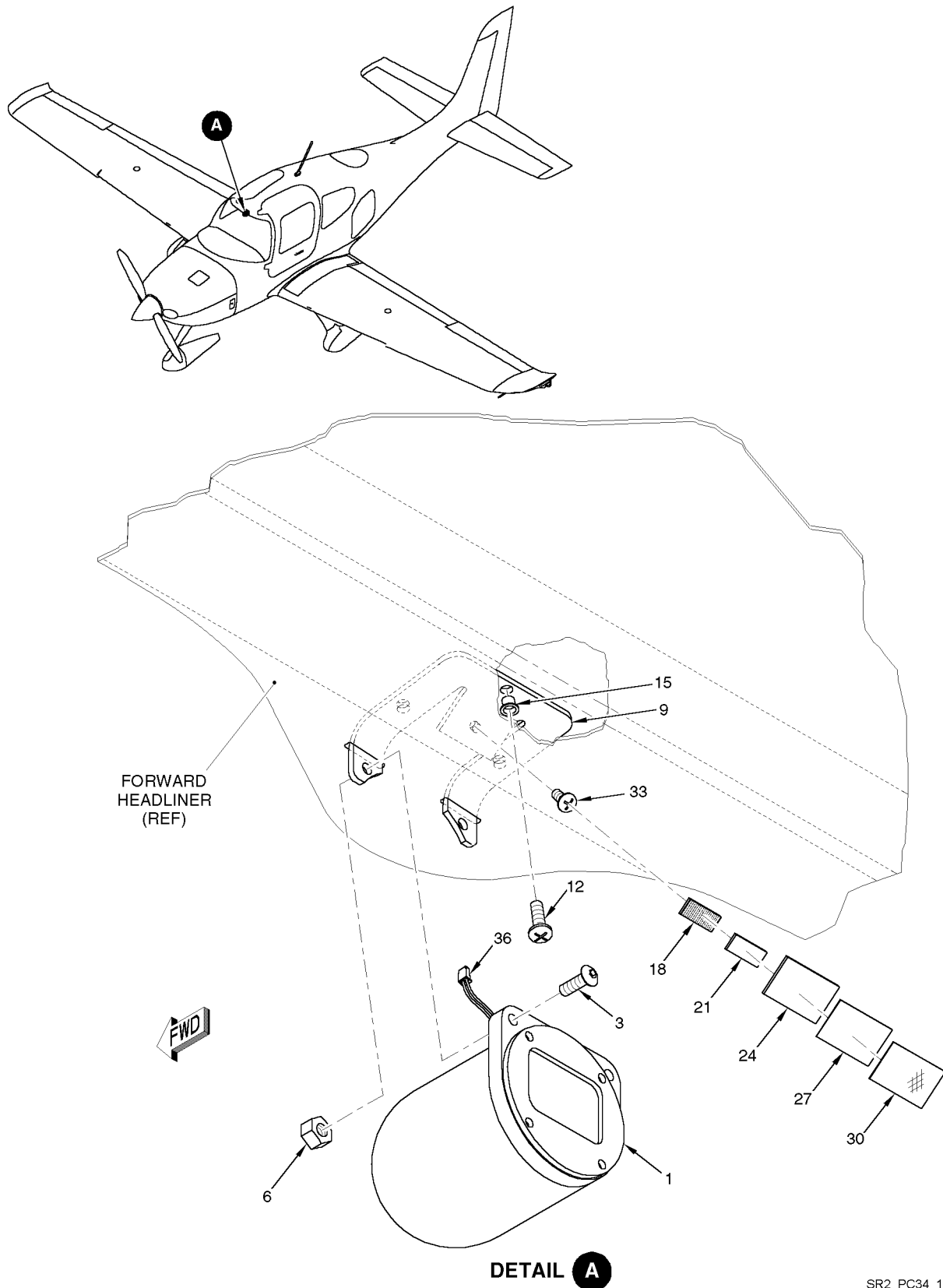
Figure 01 Magnetic Compass Installation
