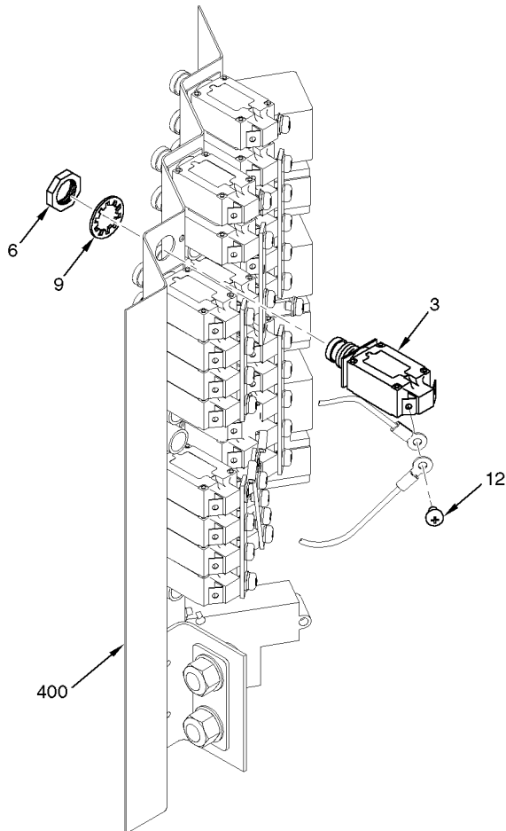
DETAIL A
