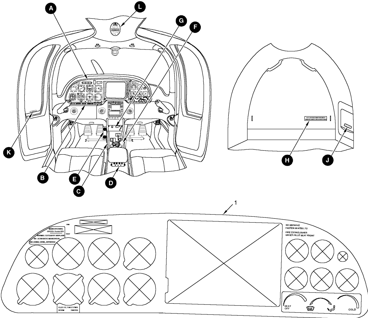
DETAIL A
