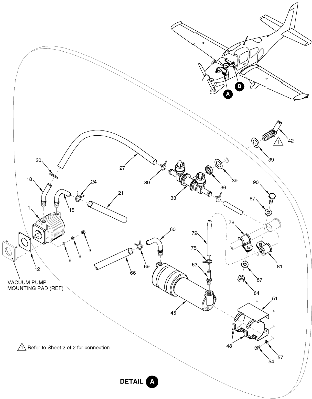
Figure 01 Vacuum System Installation (Sheet 1 of 2)
