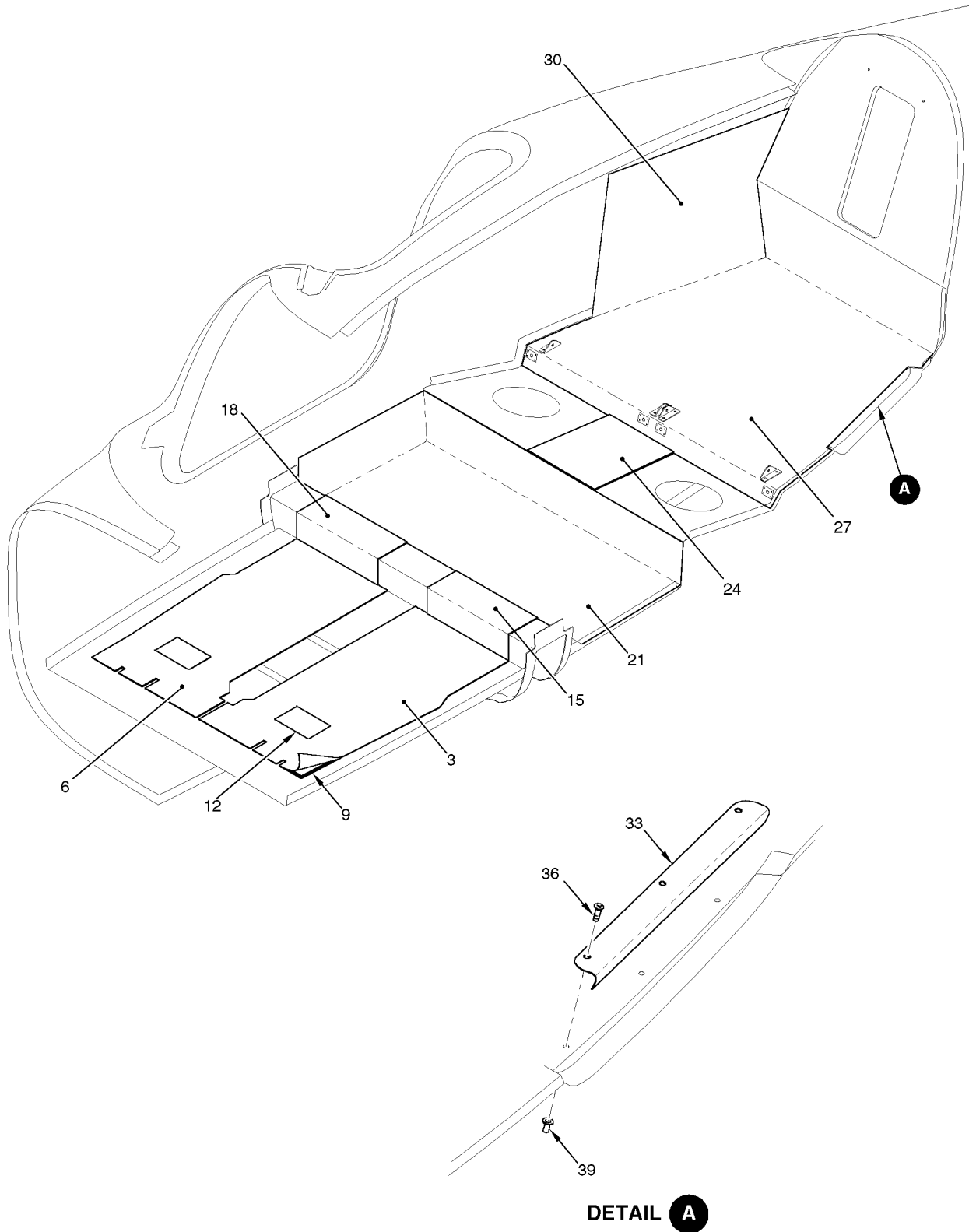
Figure 06 Floor Covering Installation
