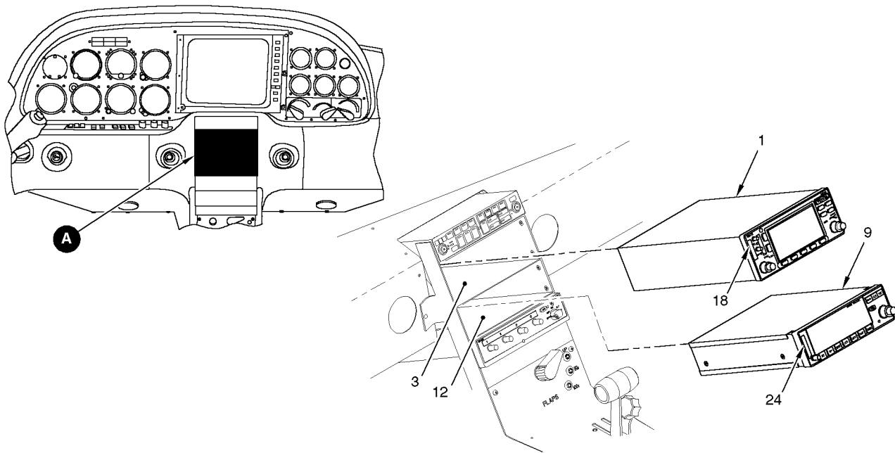
STANDARD INSTALLATION - OPTION A
