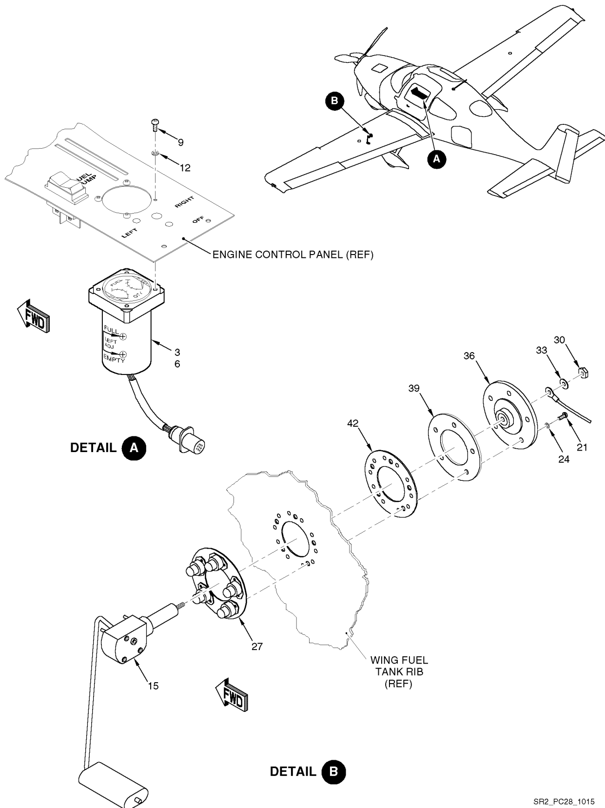
Figure 01 Fuel Indicator Installation
