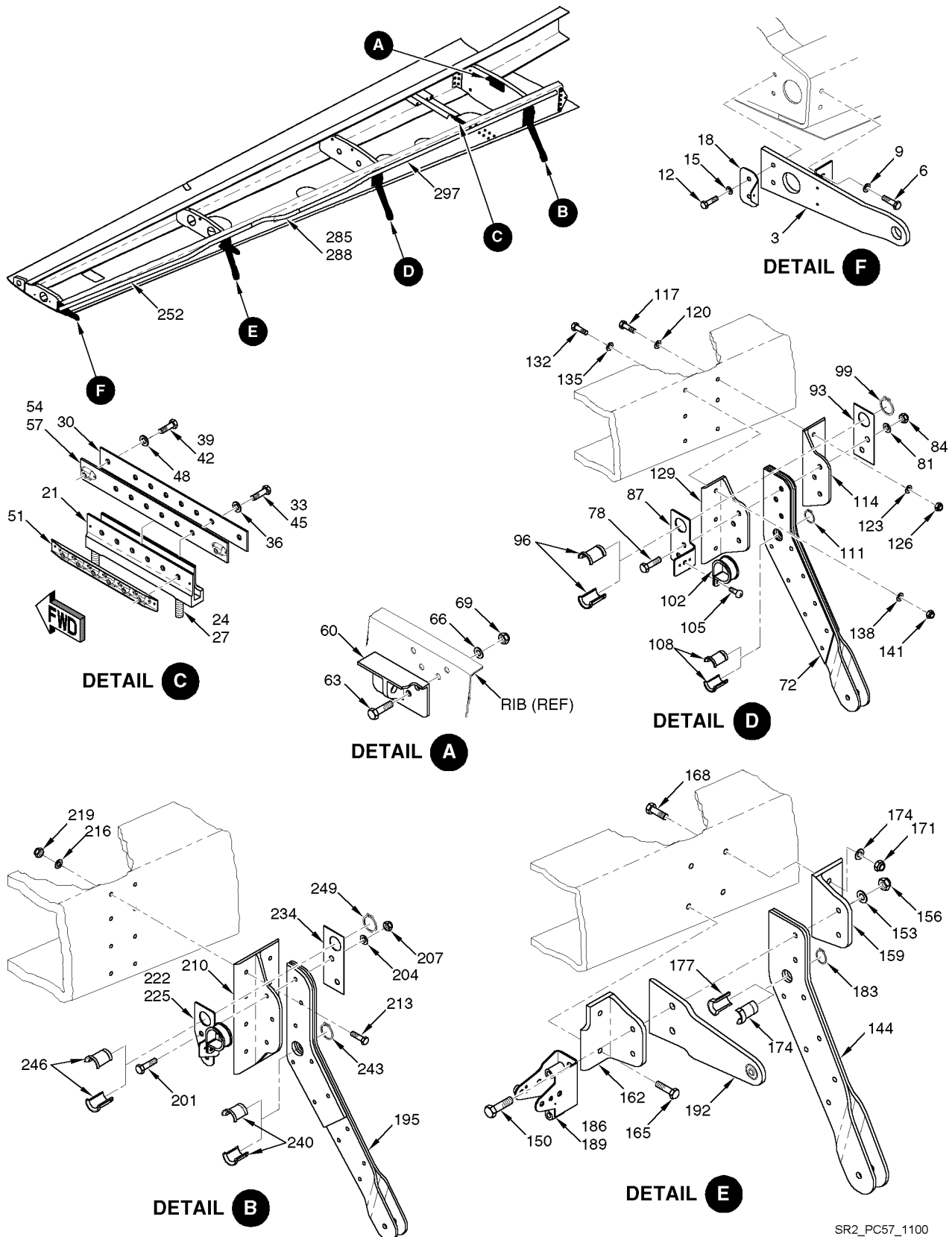
Figure 01 Flap and Aileron Hinge Installation
