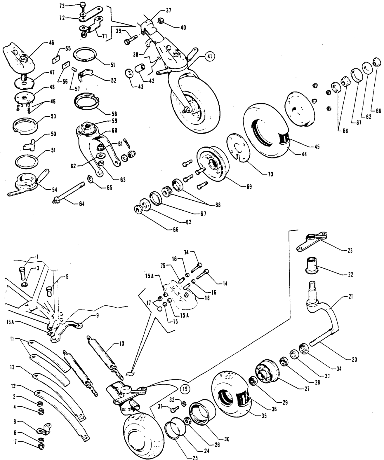
Figure 17. Tail Wheel Installation
