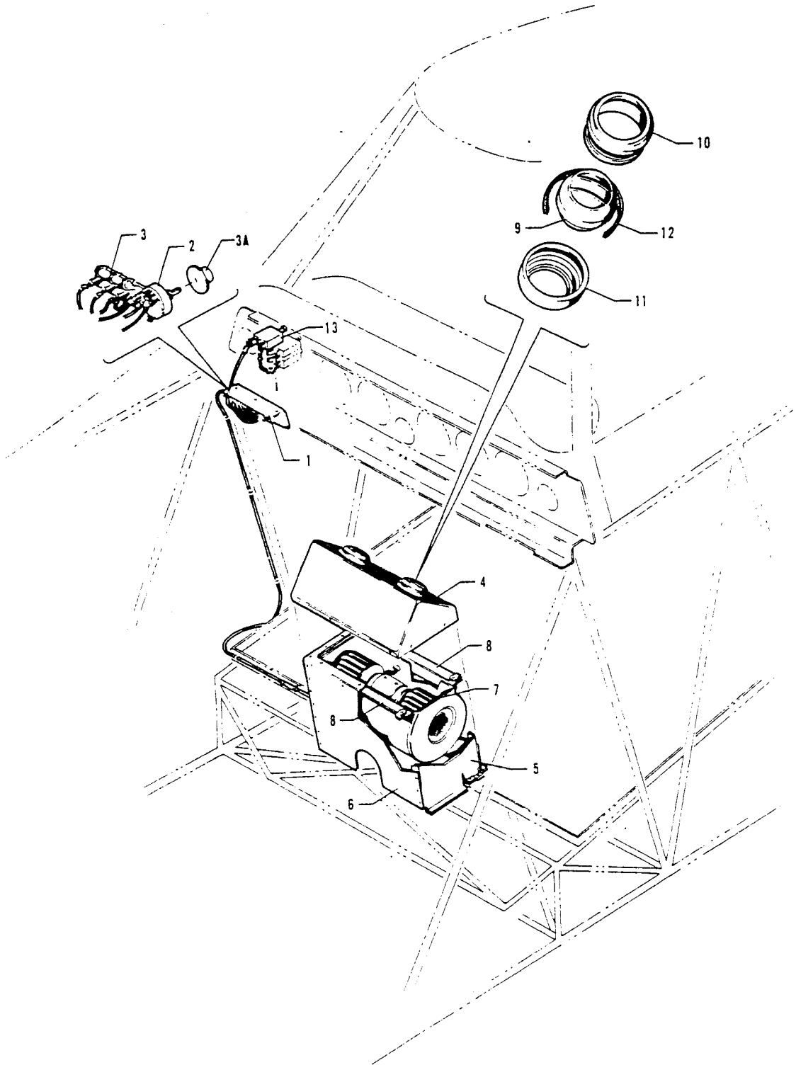
Figure 38. Cockpit Fan Installation
