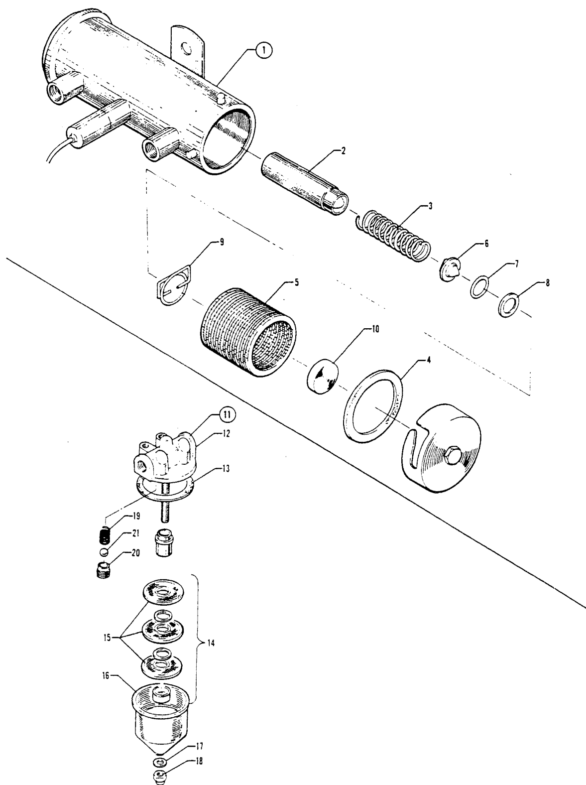
Figure 33C. Fuel System Components (Serial Nos. 25-7405573 and up)
