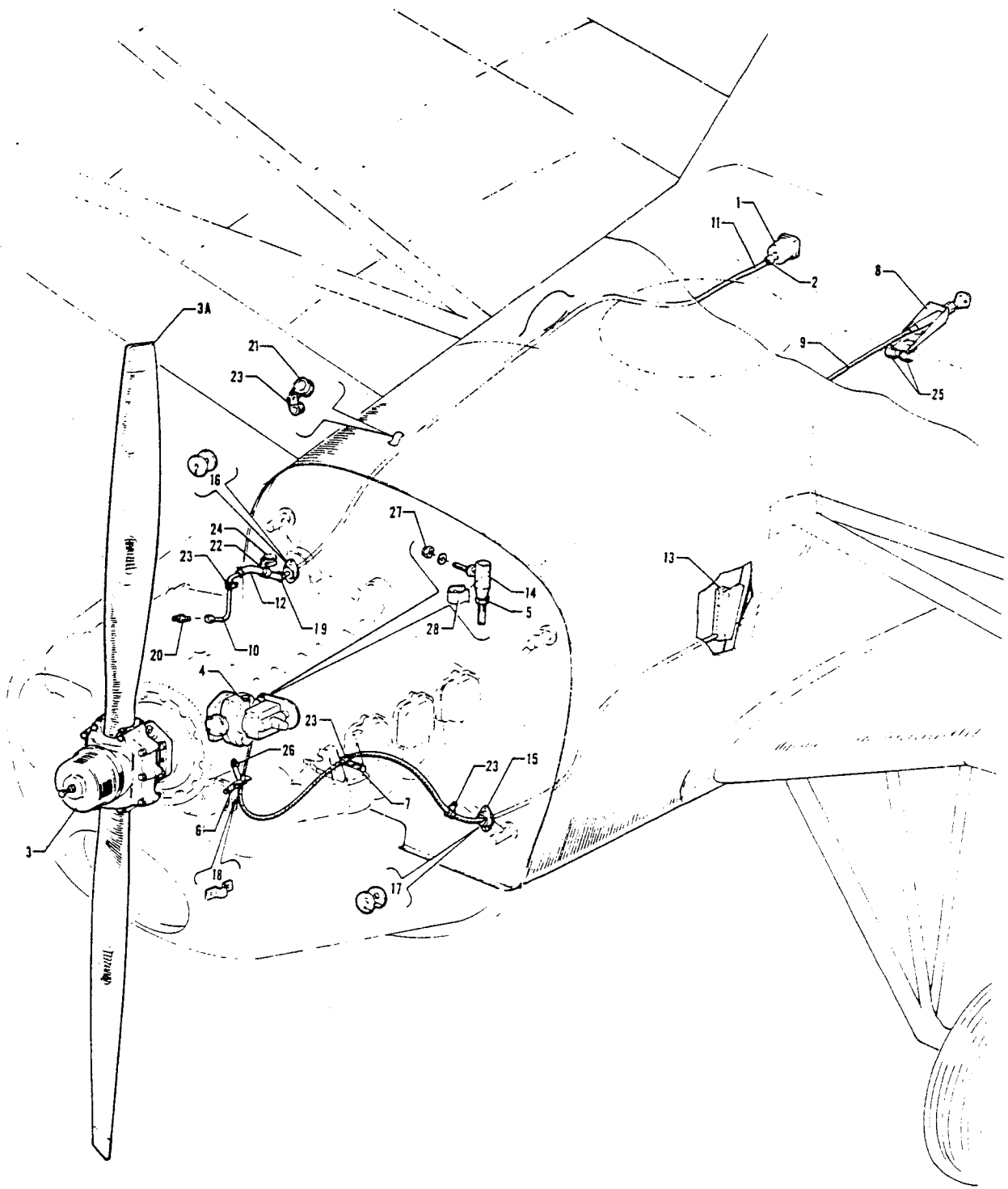
Figure 29. Constant Speed Propeller Installation
