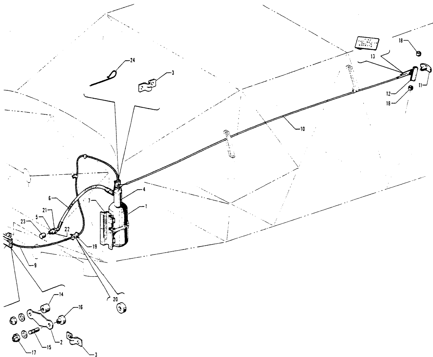
Figure 30 Engine Compartment Fire Extinguisher Installation (Serial Nos. 25-1 to 25-8056008 inclusive)
