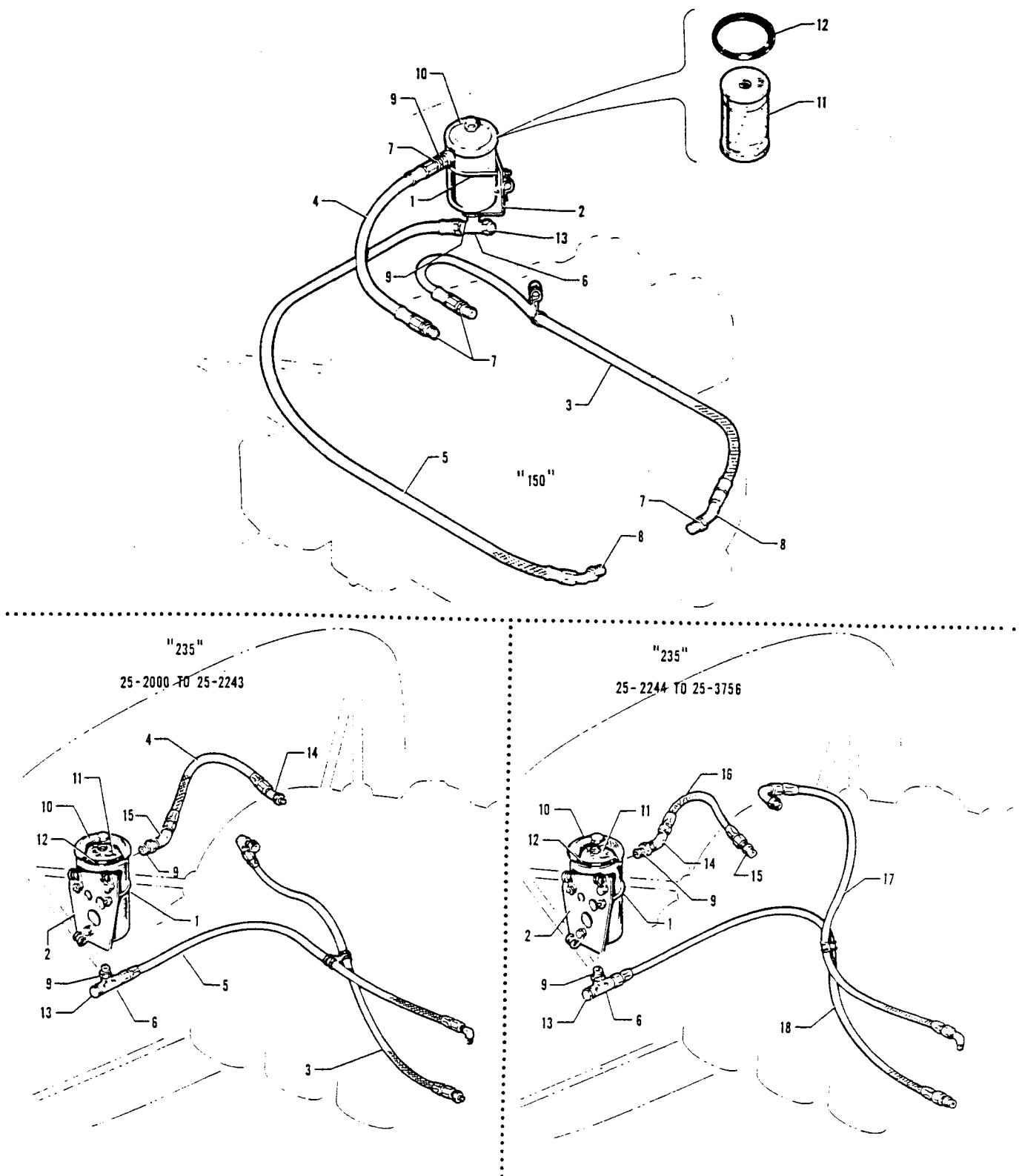
Figure 28. Oil Filter Installation (Serial Nos. 25-1 to 25-3756 inclusive)
