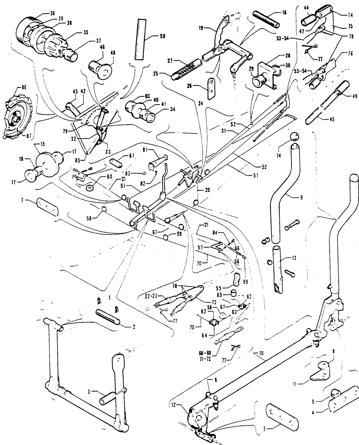
Figure 40 Control Systems Installation
