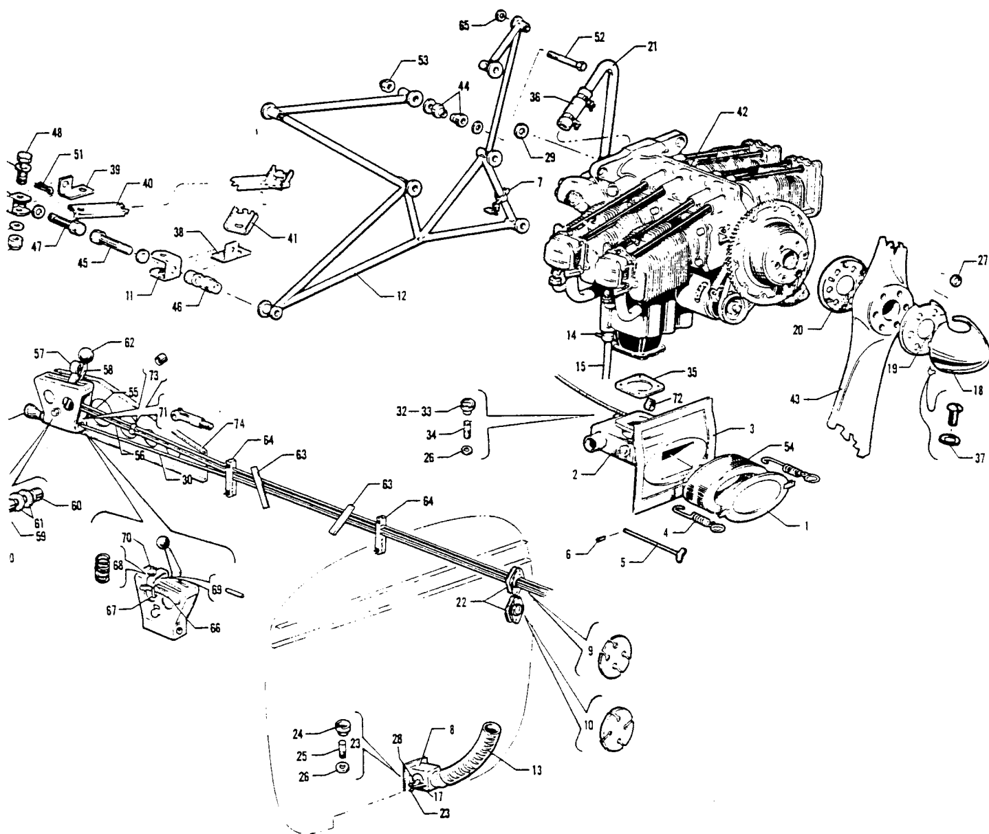
Figure 19. Power Plant Installation (PA-25-150 Only)
