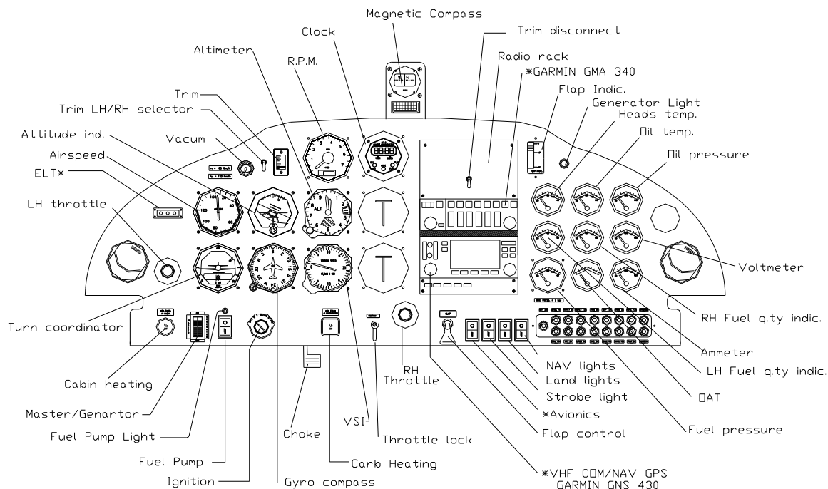
Fig. 7-2. INSTRUMENT PANEL
