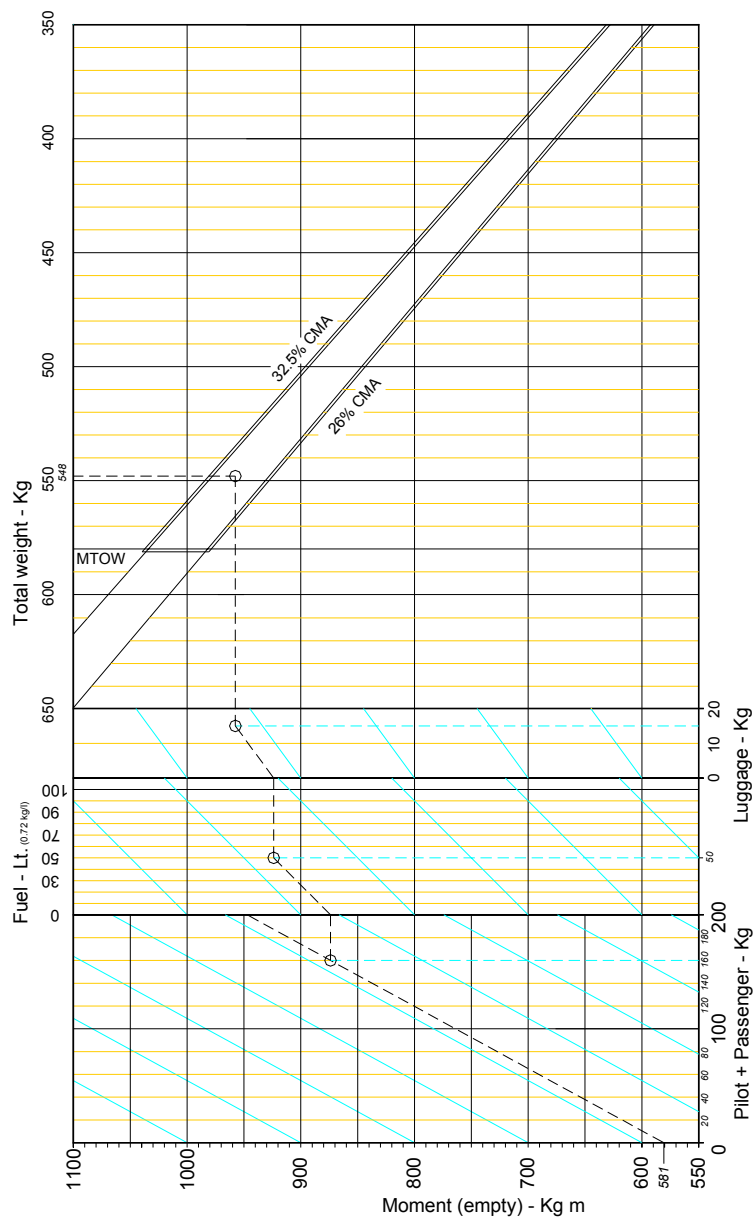
FIG. 6-2 Weight & balance chart
