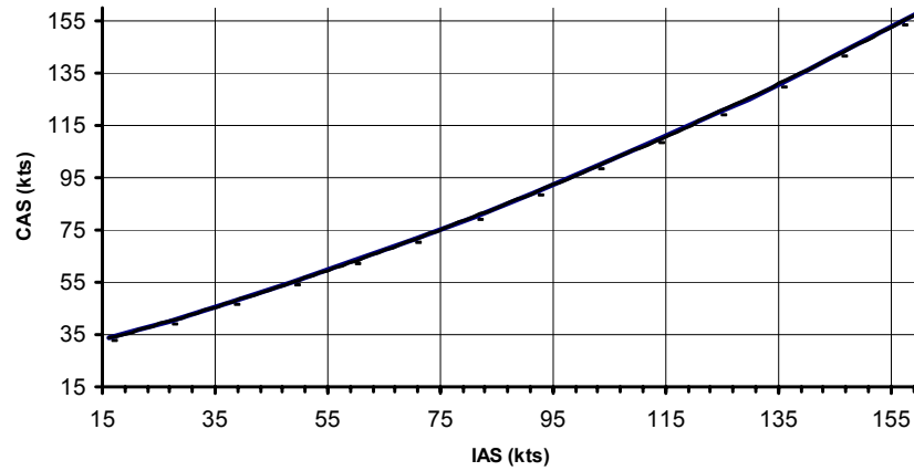
Fig. 5-1. CALIBRATED VS. INDICATED AIRSPEED -
