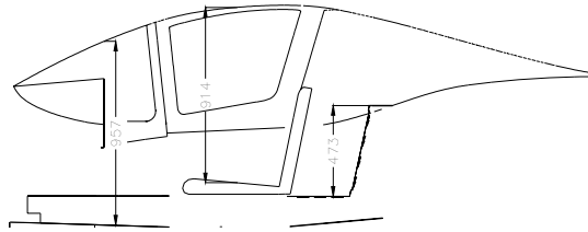
Fig 6-5 CABIN DIMENSIONS
