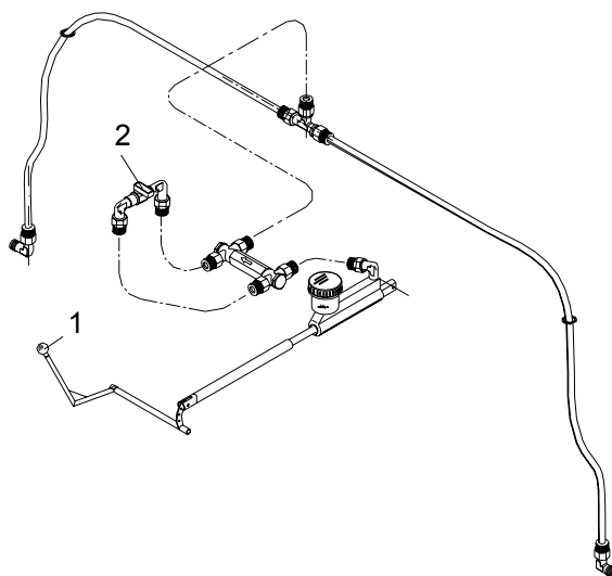
FIG. 7-6. BRAKE SYSTEM
