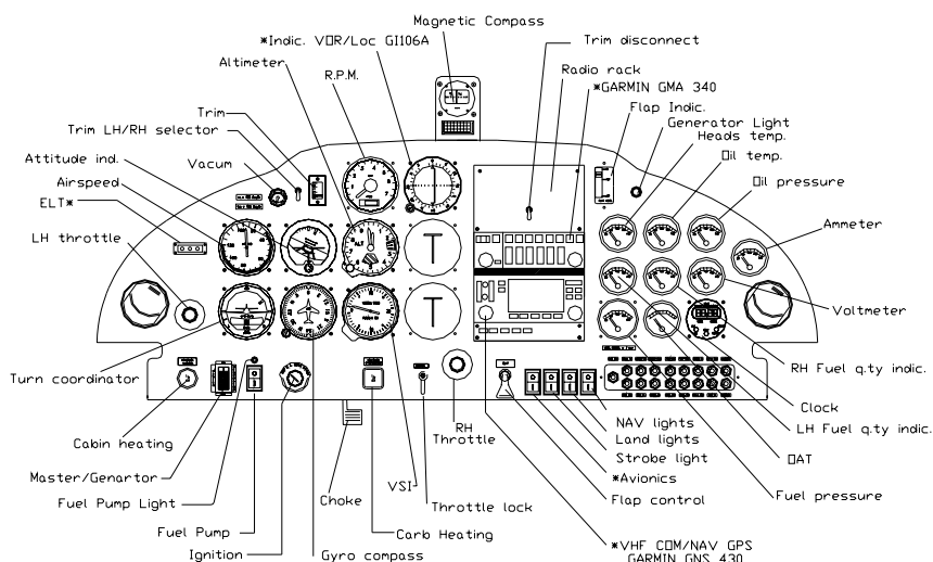
Fig. 7-2. INSTRUMENT PANEL
