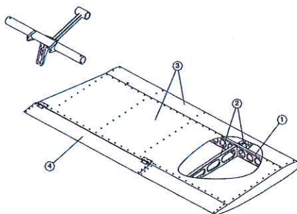
Fig. 7-2. STABILATOR STRUCTURE
