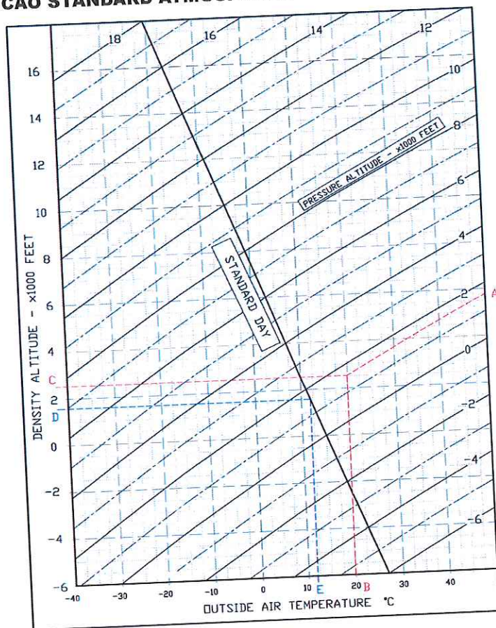
FIG. 5-2. ICAO CHART
