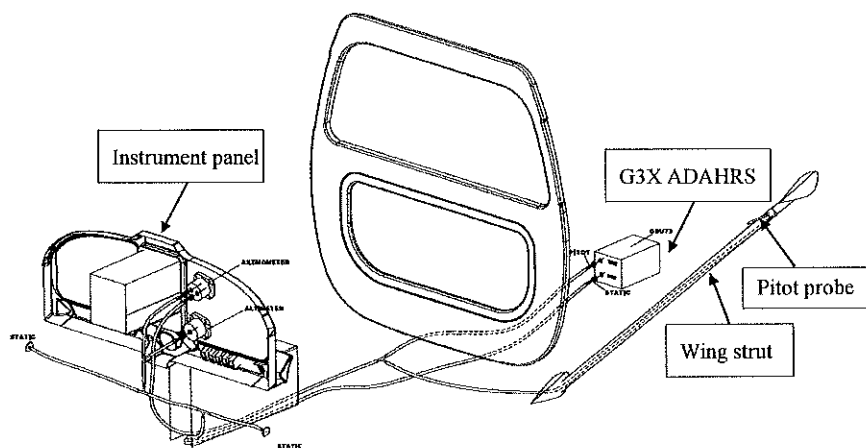
FIG. 7-8. PITOT-STATIC SYSTEM
