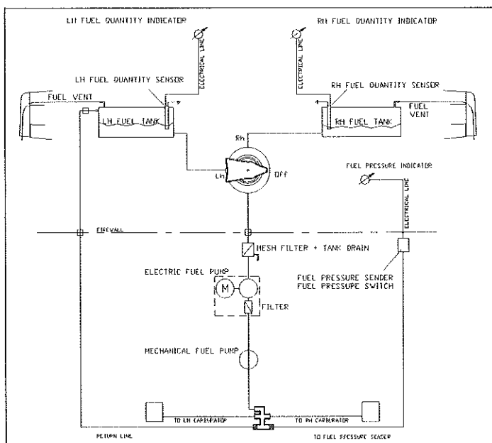
Fig. 7-7. FUEL SYSTEM SCHEMATIC
