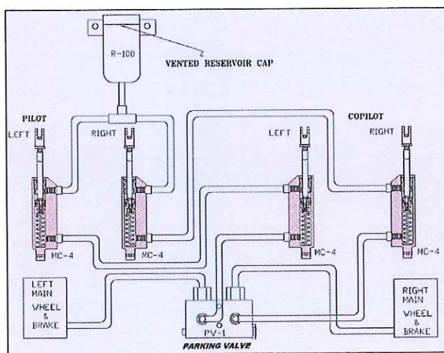
FIG. 7-9. BRAKE SYSTEM SCHEMATIC
