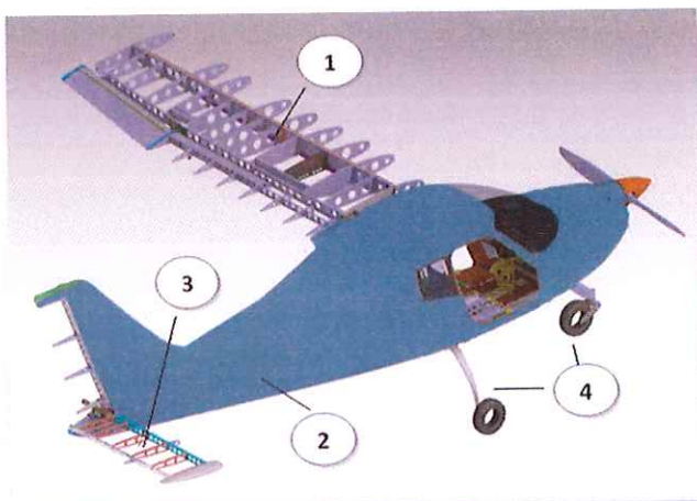
Fig. 7-1.P2008JC AIRFRAME
