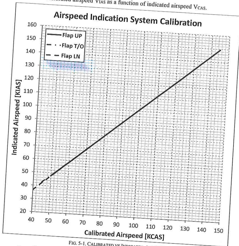
FIG. 5-1. CALIBRATED VS INDICATED AIRSPEED
