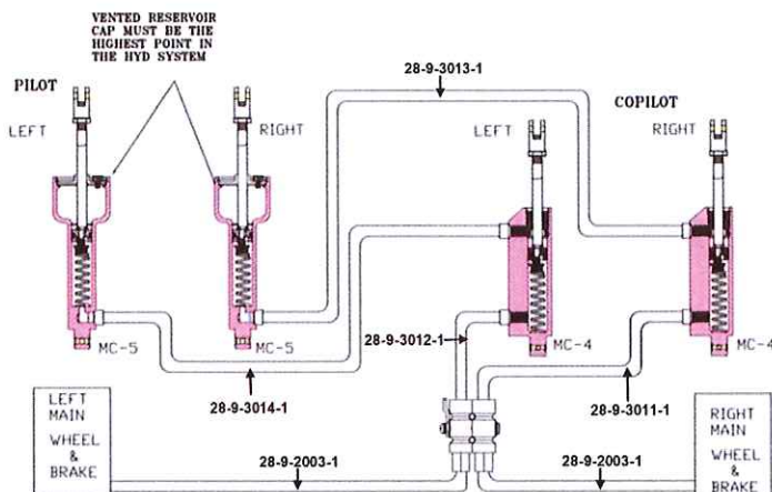
FIG. 7-10. BRAKE SYSTEM SCHEMATIC (MOD2008/124)
