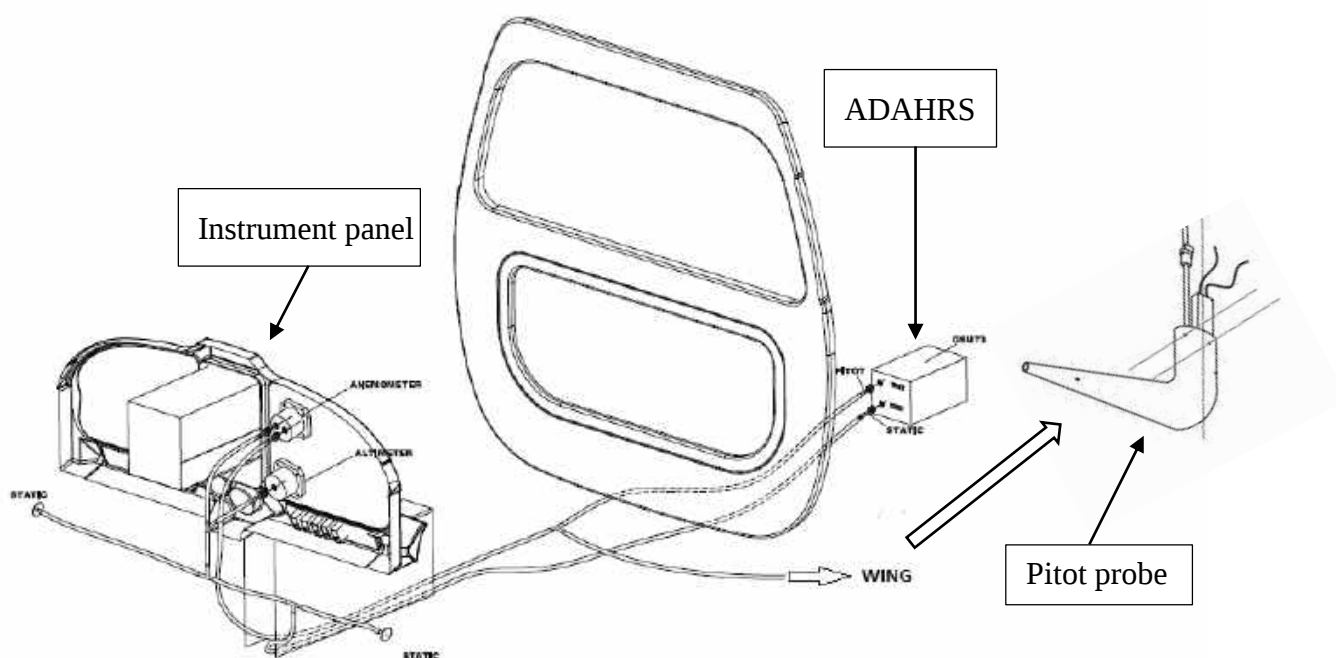
FIG.7-8. PITOT-STATIC SYSTEM
