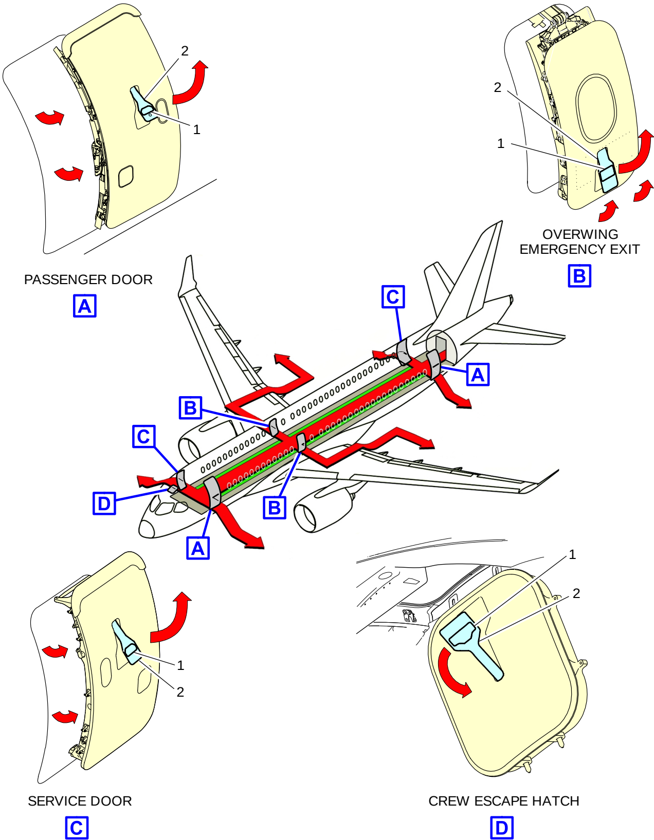
ICN-BD500-A-J154100-A-3AB48-24914-A-001-01 Figure 1 Emergency exits and evacuation
