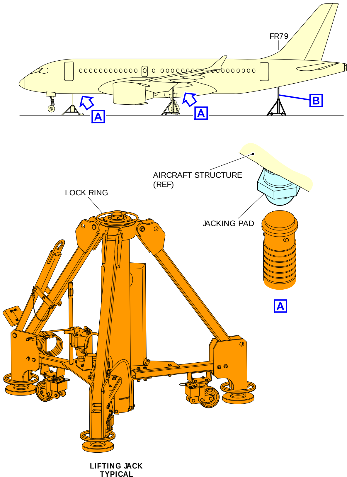
ICN-BD500-A-J071102-A-3AB48-25019-A-002-01 Figure 1 Jacking for maintenance - (Sheet 3 of 6)
