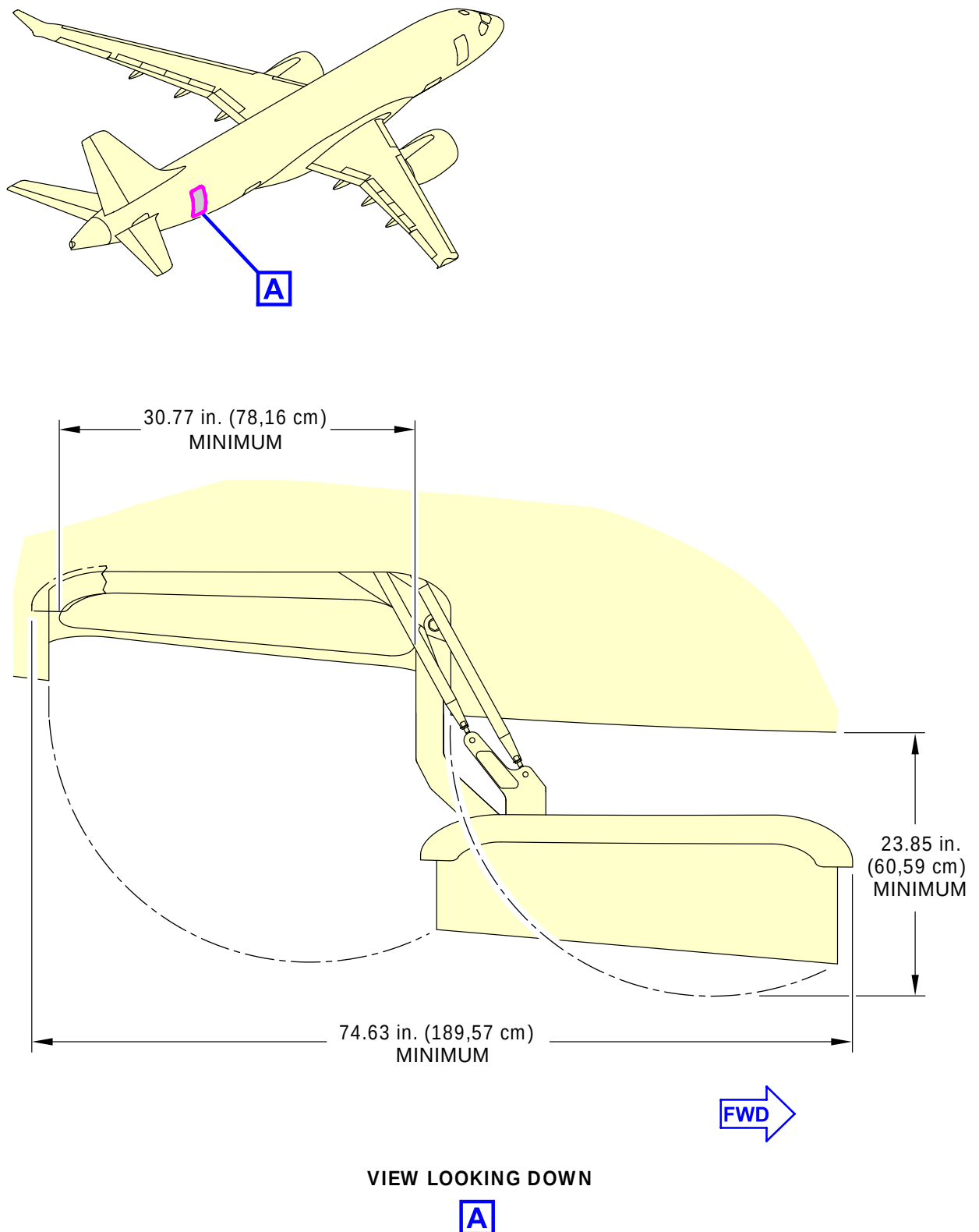
ICN-BD500-A-J061100-A-3AB48-00105-A-002-01 Figure 17 Aft service door opening and clearances
