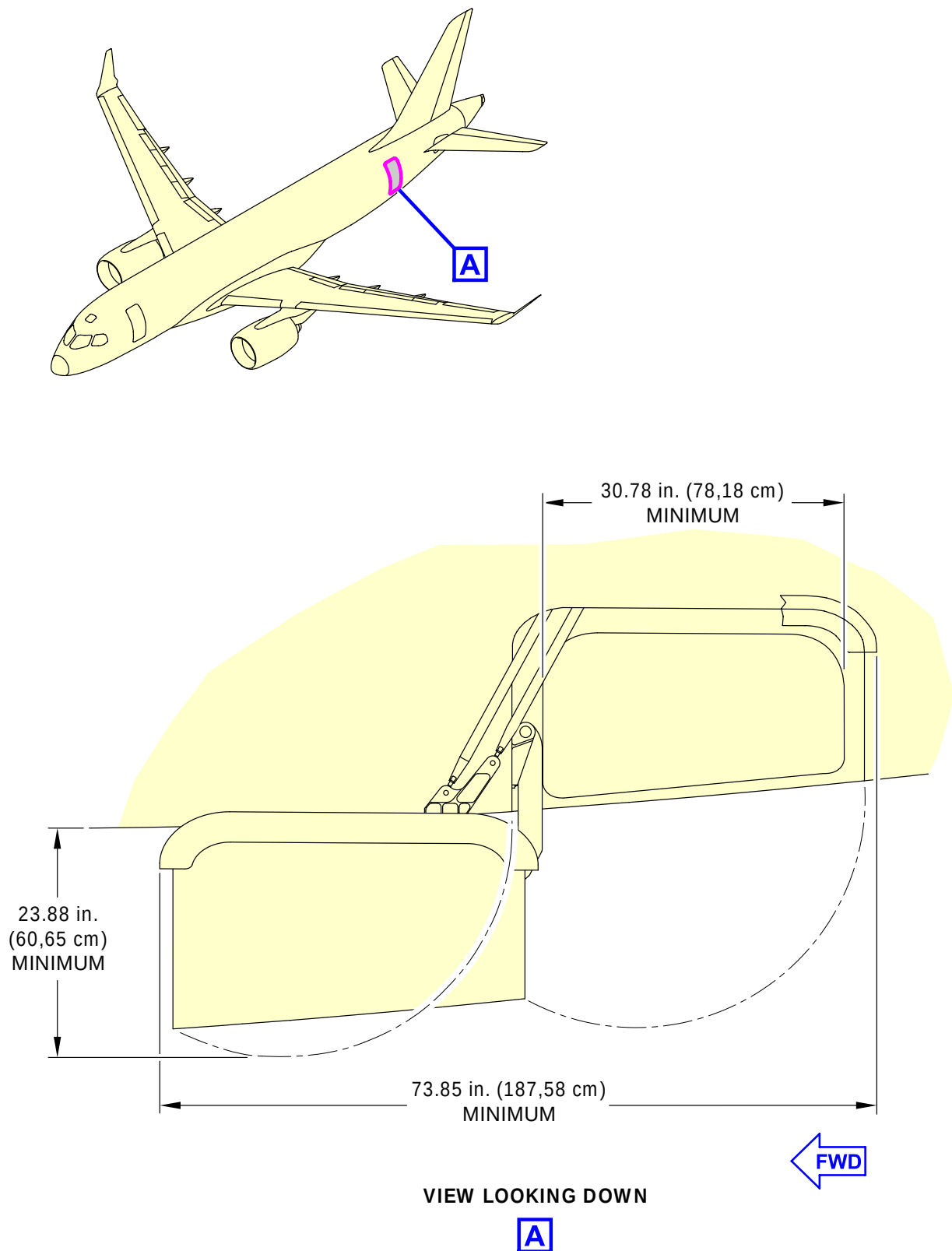
Figure 13 Aft passenger door opening and clearances
