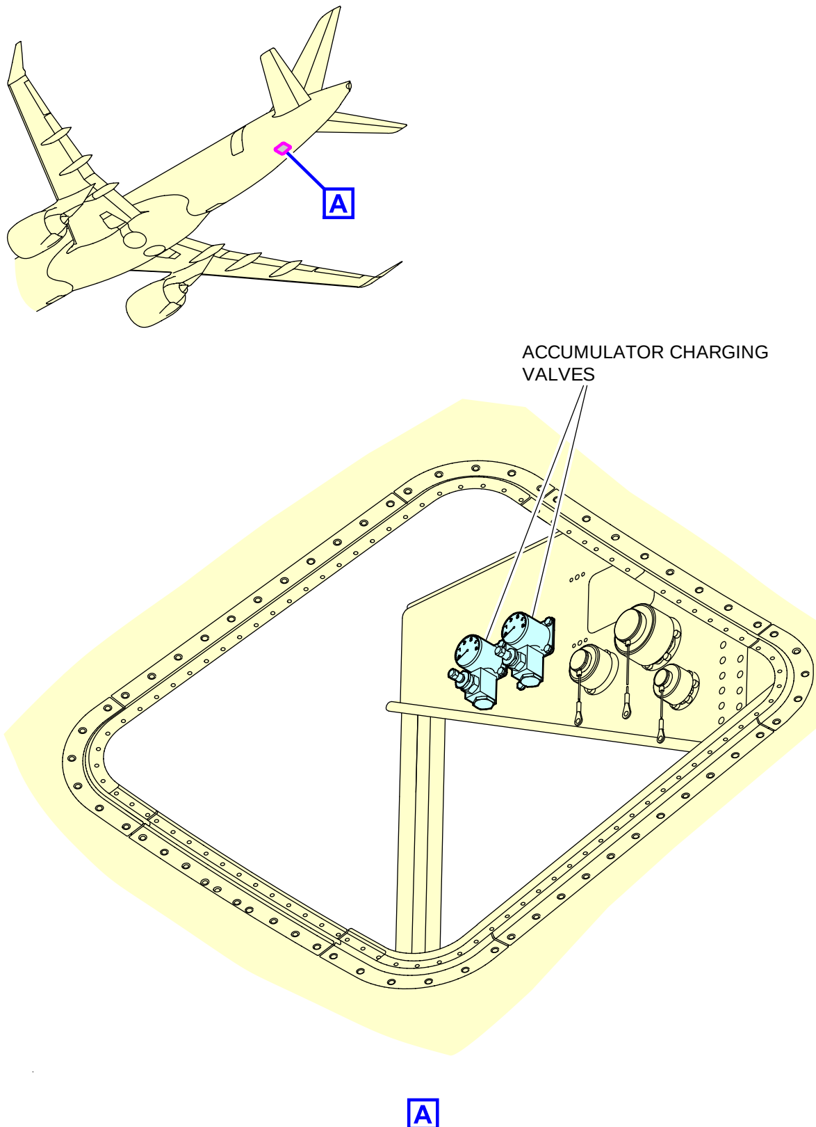
ICN-BD500-A-J000000-A-3AB48-22071-A-001-01 Figure 5 Accumulator charging valves
