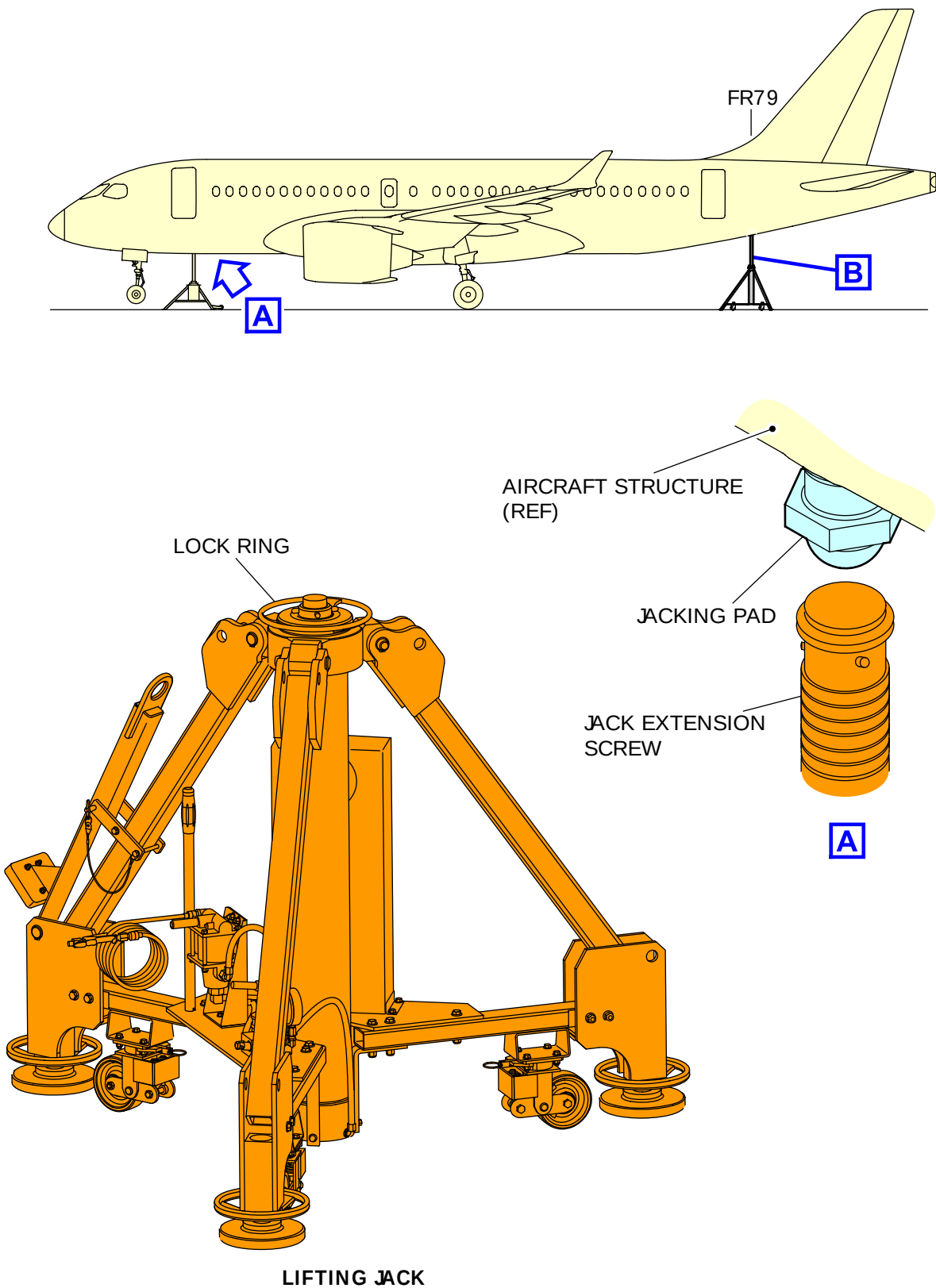
ICN-BD500-A-J071103-C-3AB48-47758-A-001-01 Figure 1 Jacking for maintenance - (Sheet 4 of 6)
