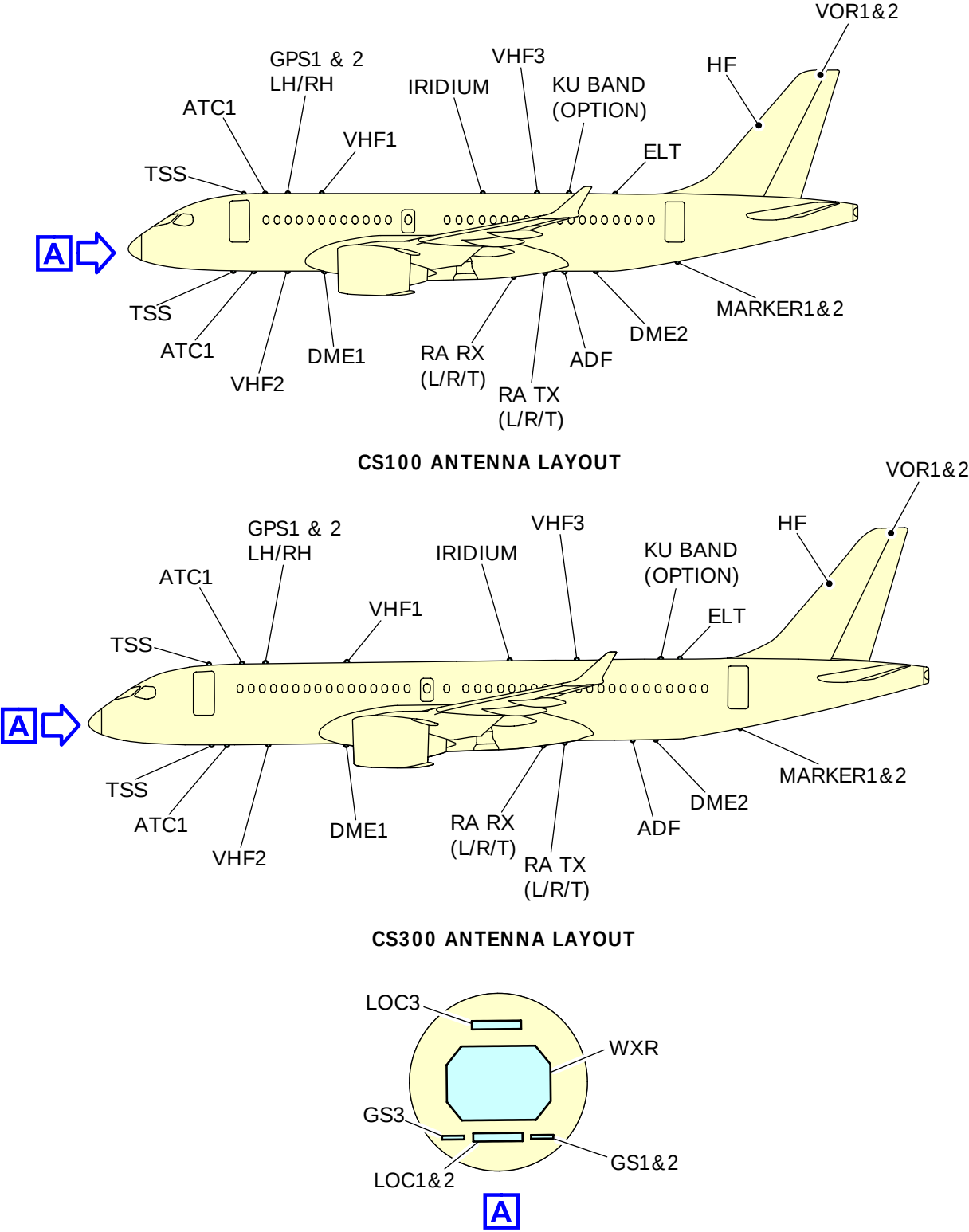
ICN-BD500-A-J230000-A-3AB48-81272-A-001-01 Figure 1 Aircraft antennas layout
