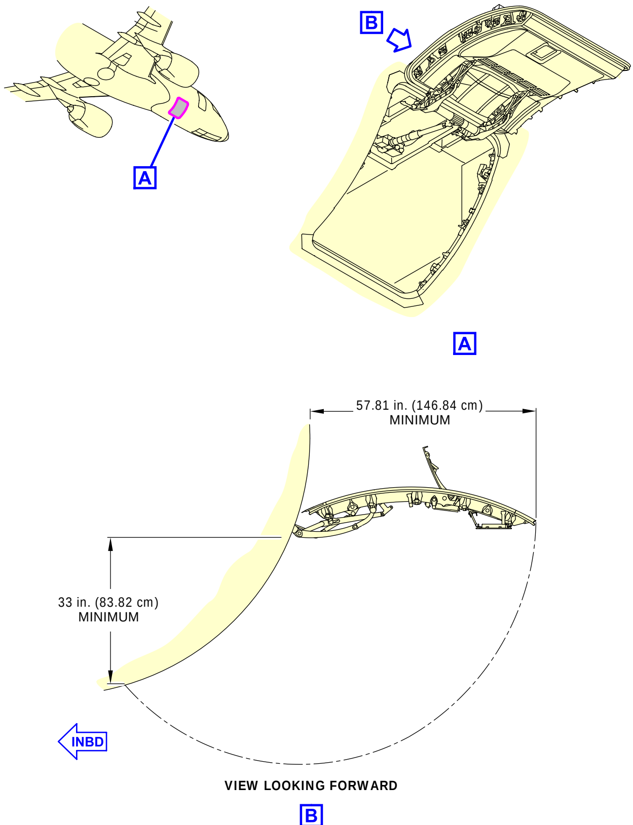
Figure 3 Forward cargo compartment - clearances - (Sheet 1 of 4)
