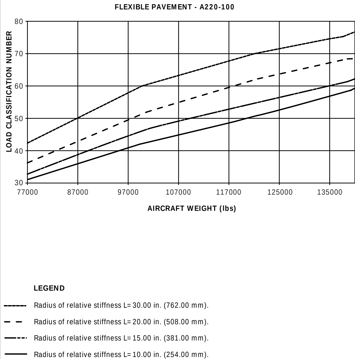
ICN-BD500-A-J000000-C-3AB48-57668-A-004-01 Figure 10 LCN results - Flexible pavement
