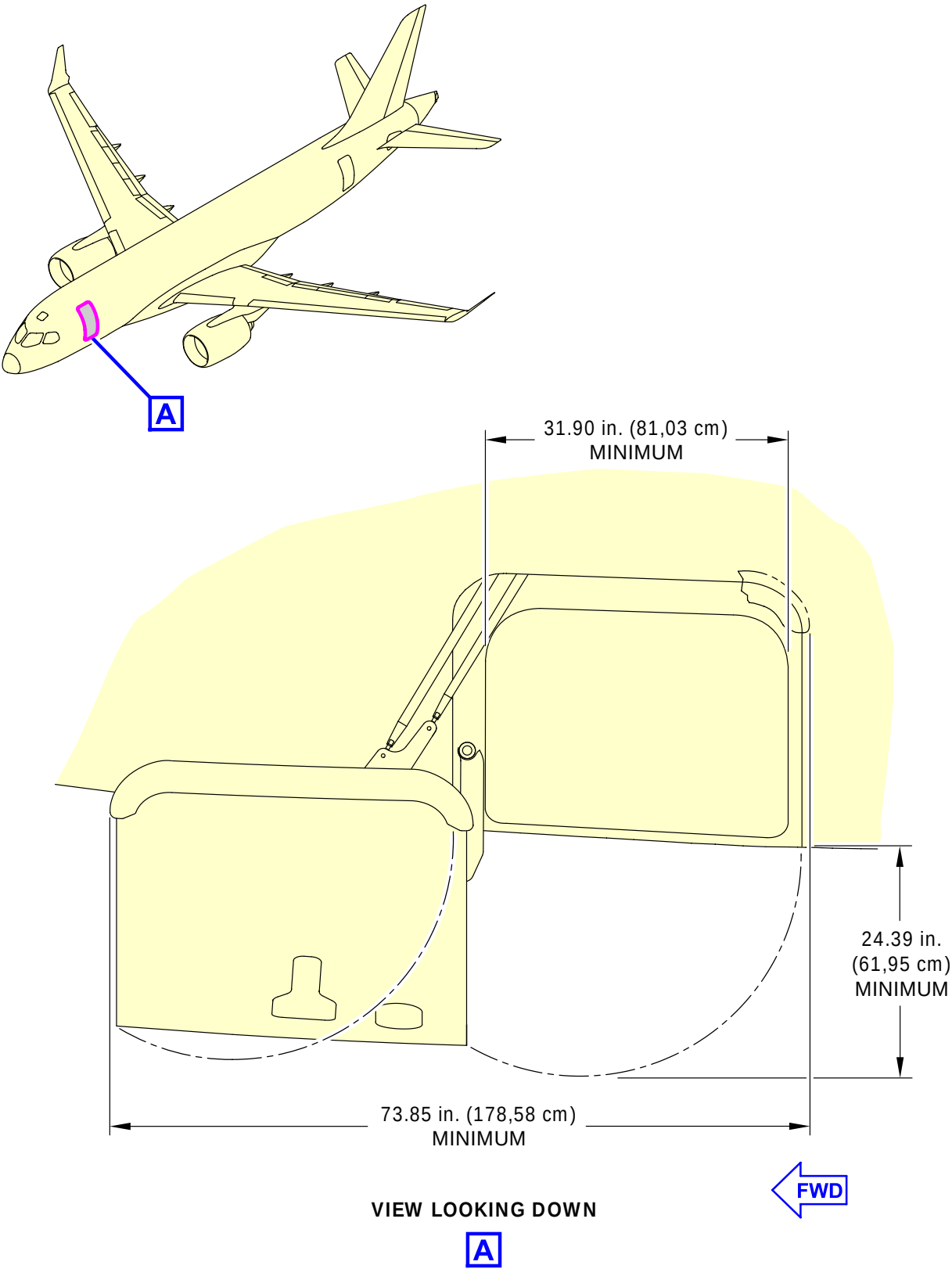
ICN-BD500-A-J061100-A-3AB48-00103-A-003-01 Figure 12 Forward passenger door opening and clearances
