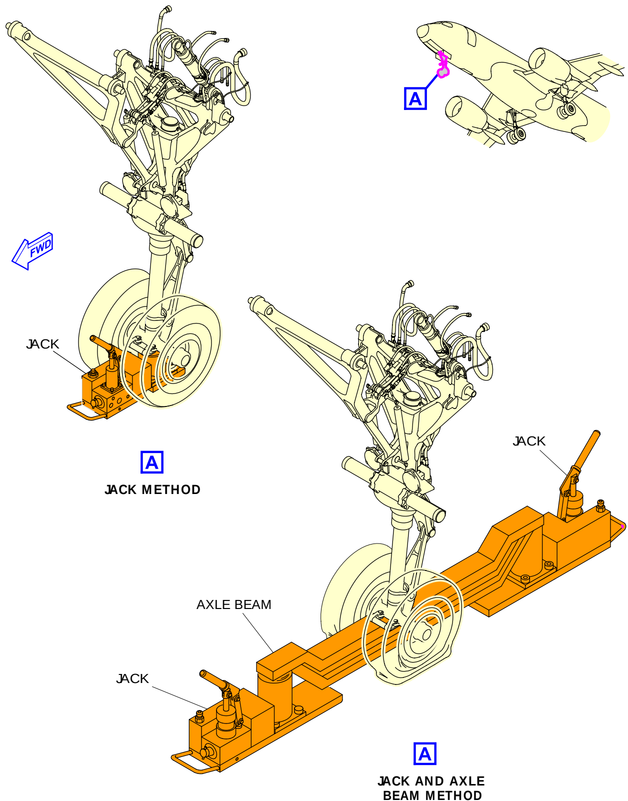
Figure 4 Nose landing gear jacking - (Sheet 1 of 2)
