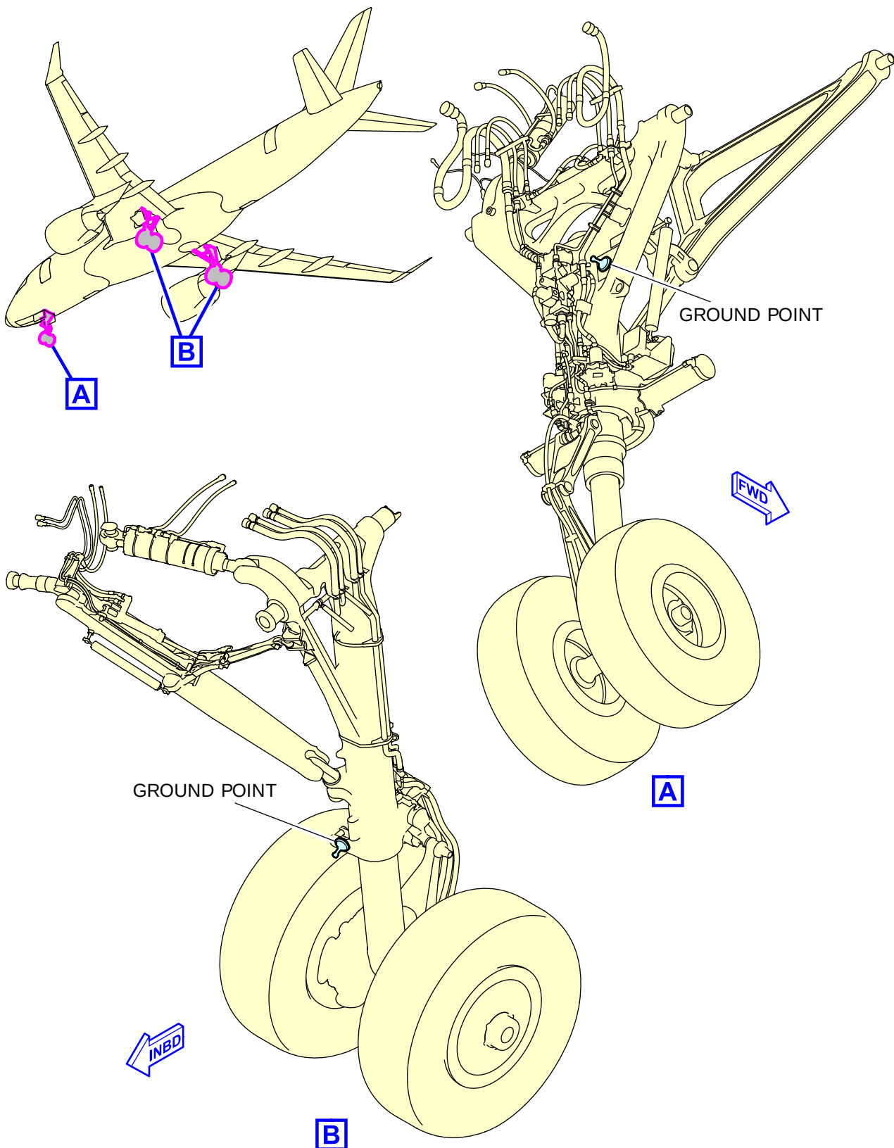
ICN-BD500-A-J000000-A-3AB48-22049-A-001-01 Figure 12 Landing gears grounding points
