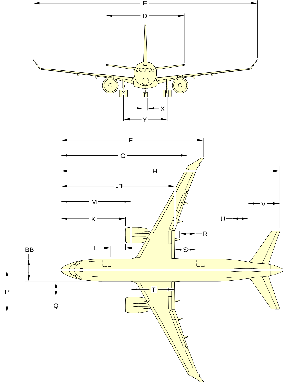
ICN-BD500-A-J061000-A-3AB48-00004-A-003-01 Figure 1 General aircraft dimensions - (Sheet 2 of 2)
