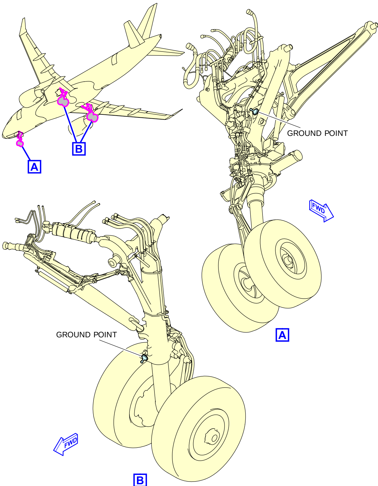
ICN-BD500-A-J000000-A-3AB48-22049-A-002-01 Figure 12 Landing gears grounding points
