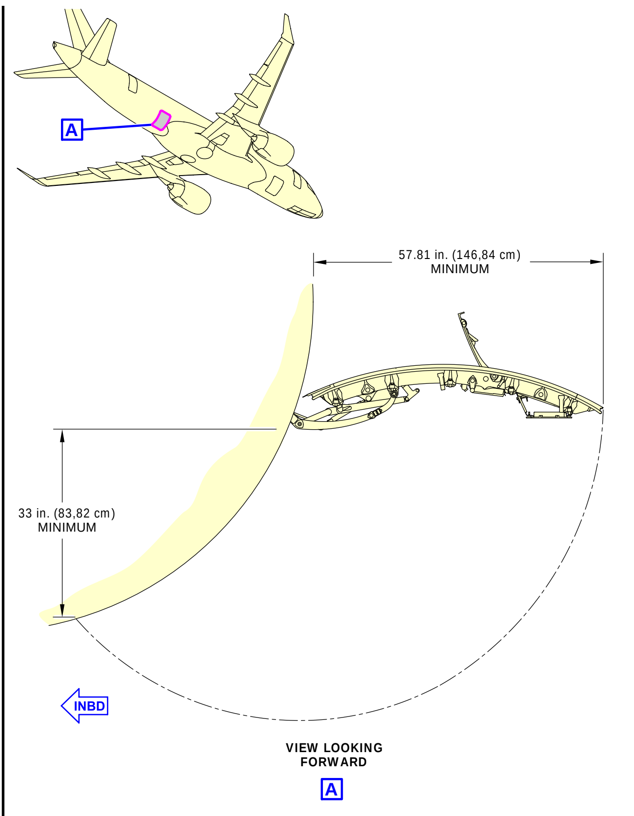
Figure 15 Aft cargo compartment door opening and clearances
