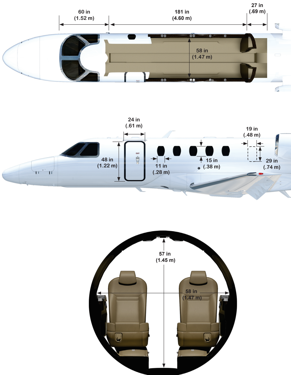
FIGURE II — CITATION CJ4 INTERIOR DIMENSIONS
