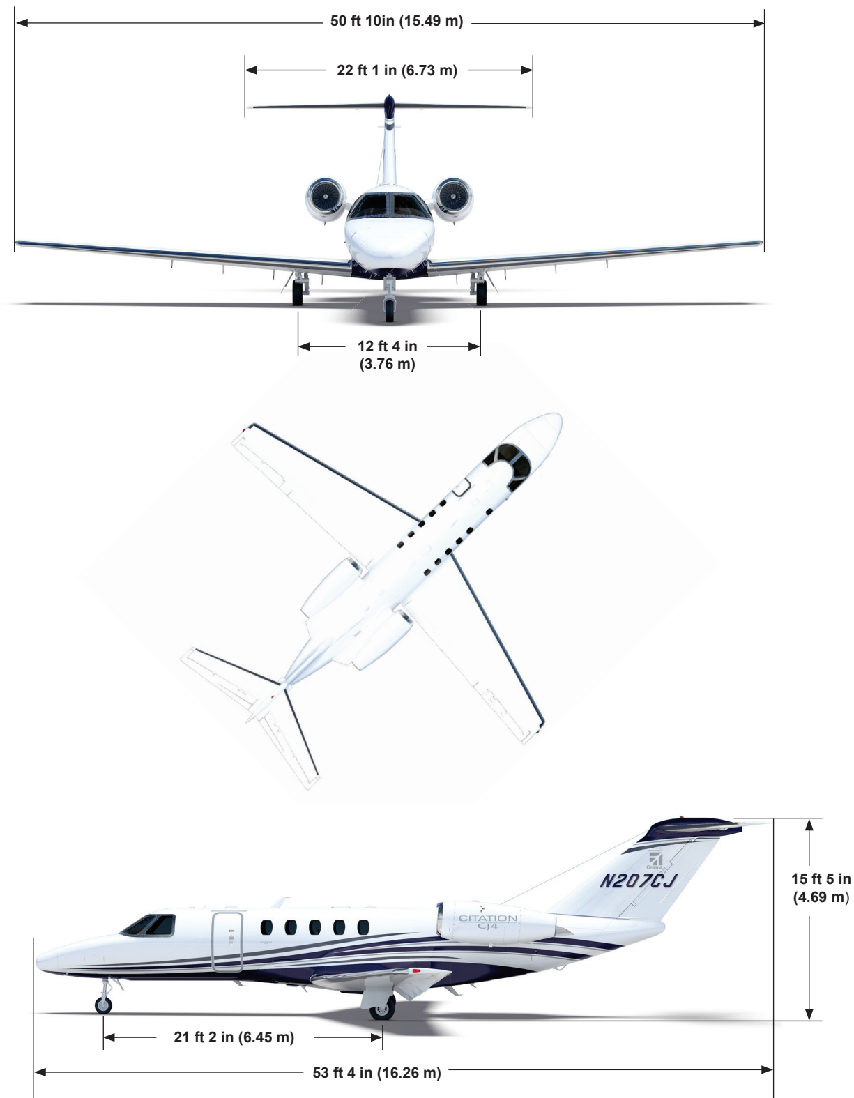
FIGURE I — CITATION CJ4 EXTERIOR DIMENSIONS
