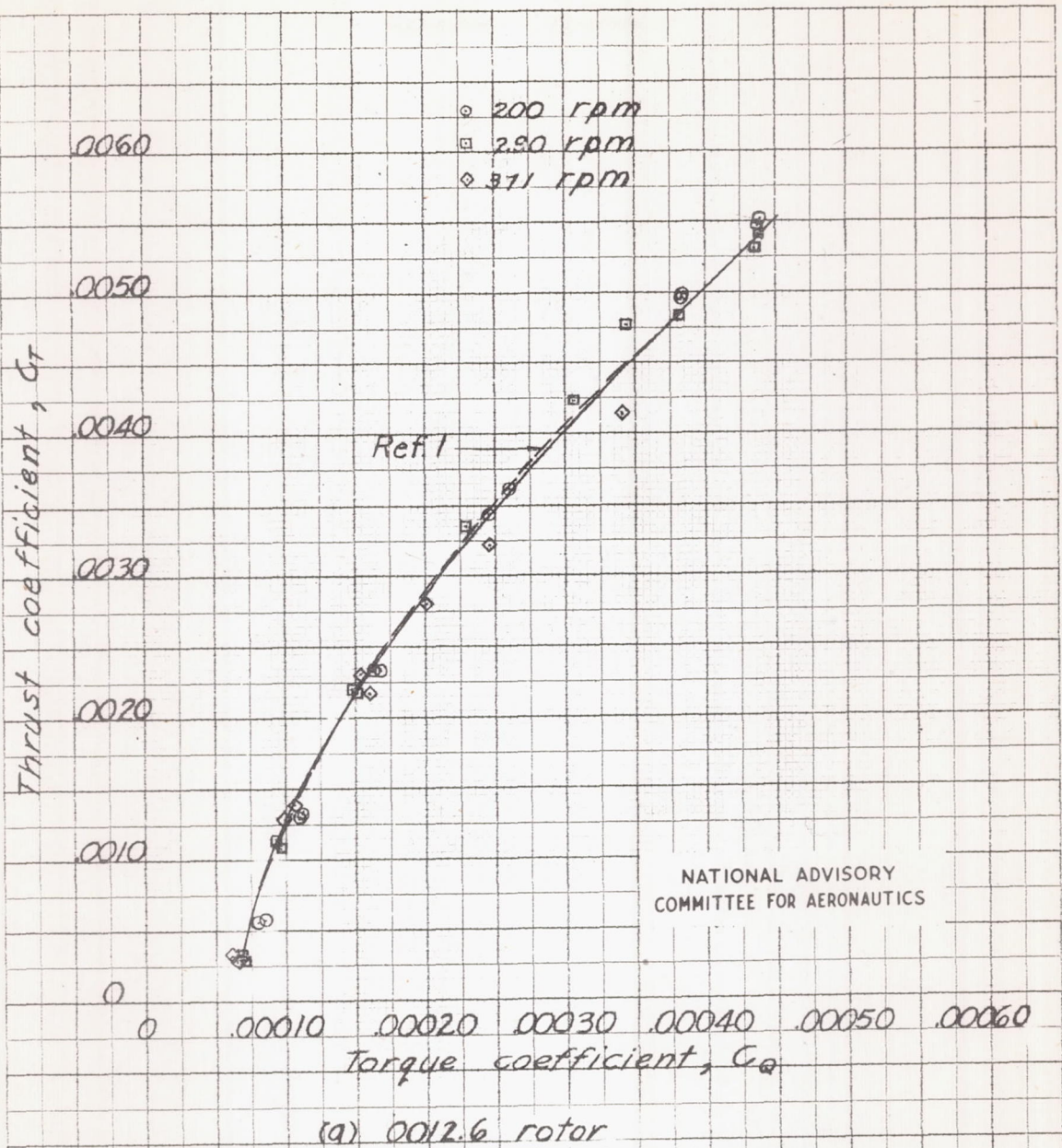
Figure 5.- Static-thrust performance of the PV-2 helicopter rotors.
