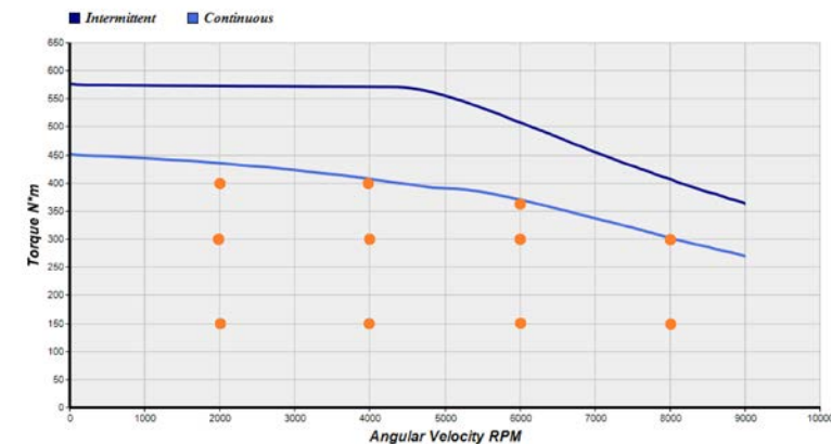
Motor Torque Speed Curves
