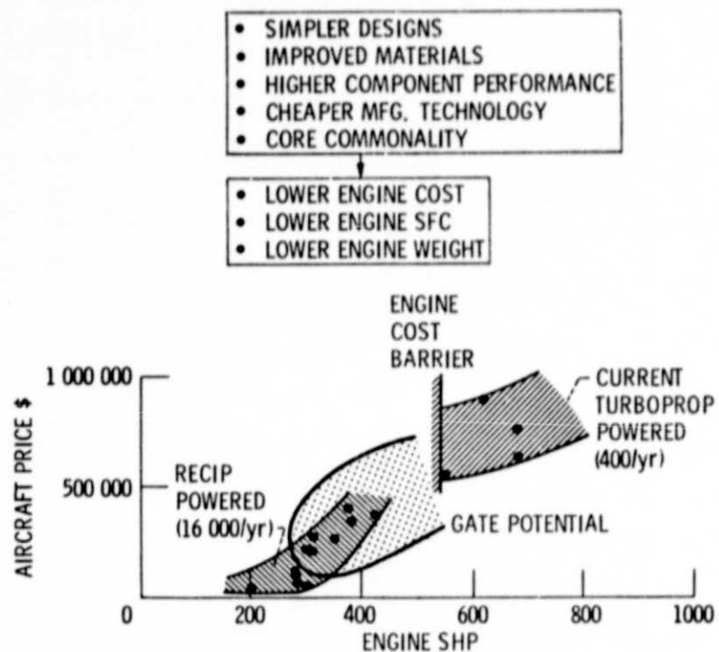
Figure 17. - Gate technology could expand domain of small turbine engines.
