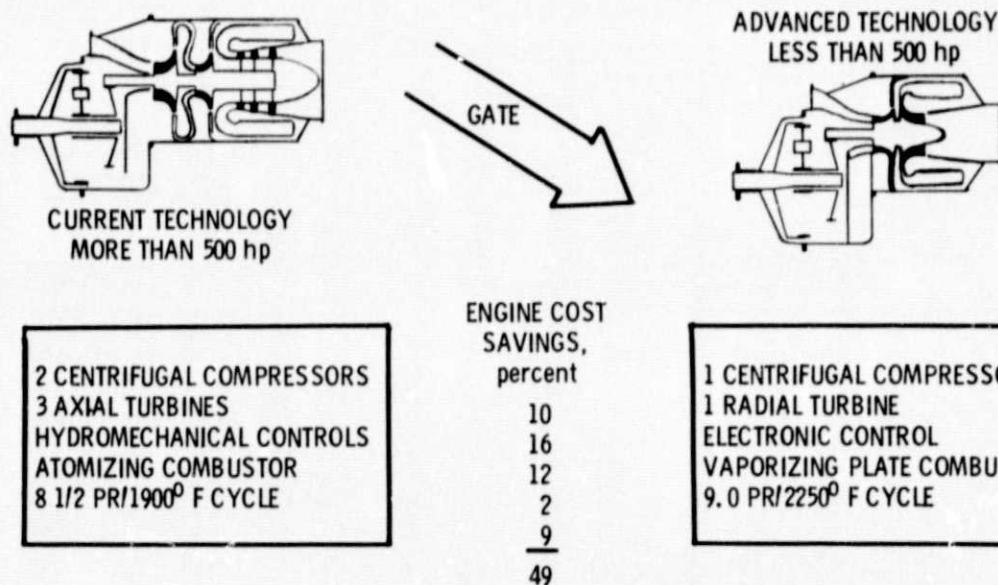
Figure 12. - Advanced technology investment reduces engine price (teledyne).
