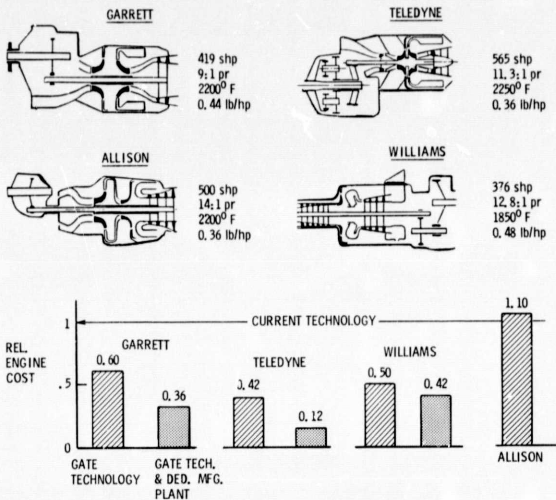
Figure 8. - The conceptual gate baseline engines and forecasted costs.
