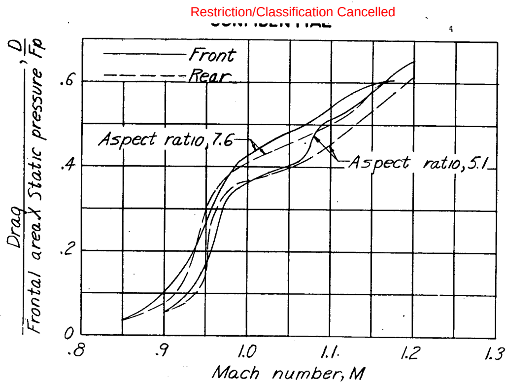
(a) Rectangular airfoils.
