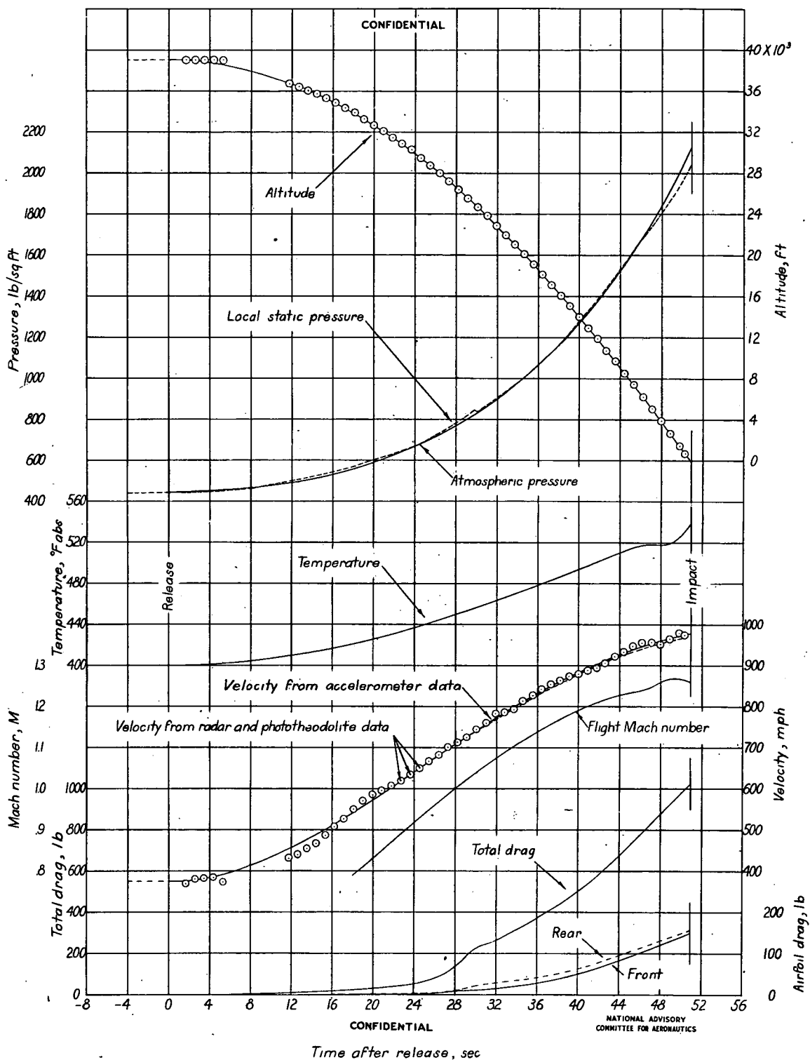
Figure 4.- Time history of free fall of 1330-pound test body mounting airfoils having 45^\circ sweepback. NACA 65-009 airfoil section.
