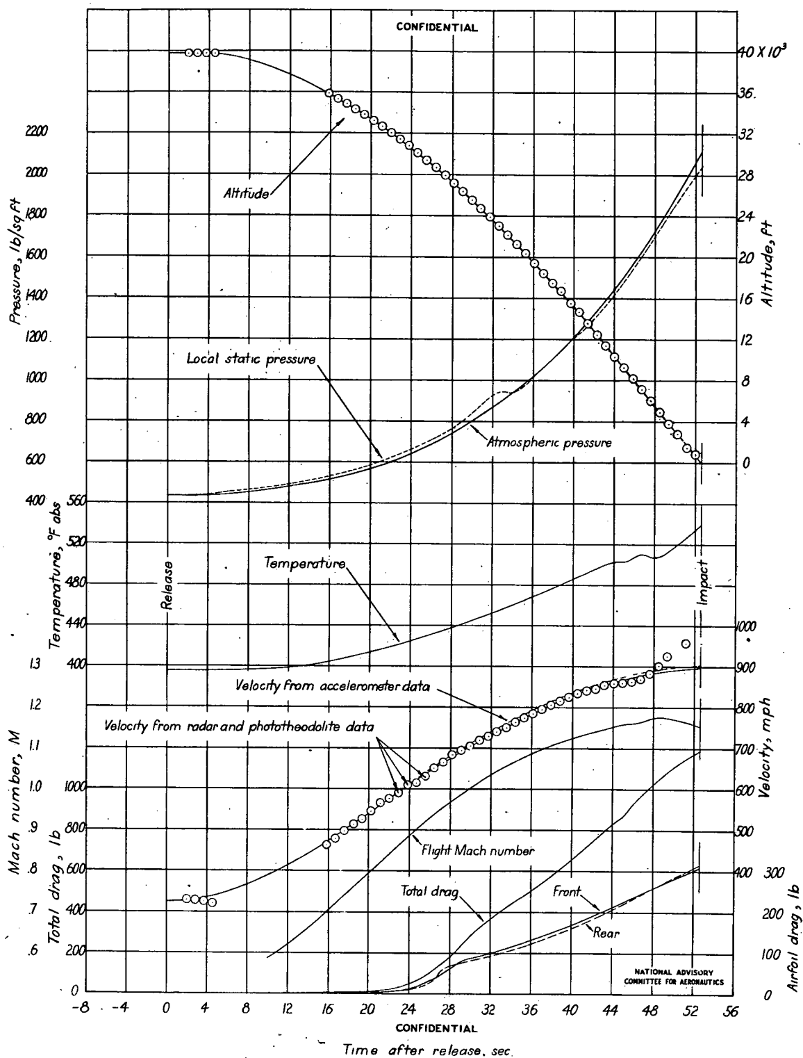
Figure 3.- Time history of free fall of 1322-pound test body mounting rectangular airfoils. NACA 65-009 airfoil section.
