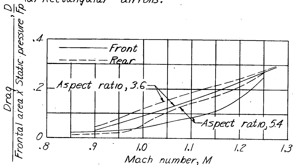
(b) Airfoils having 45^\circ sweepback.
