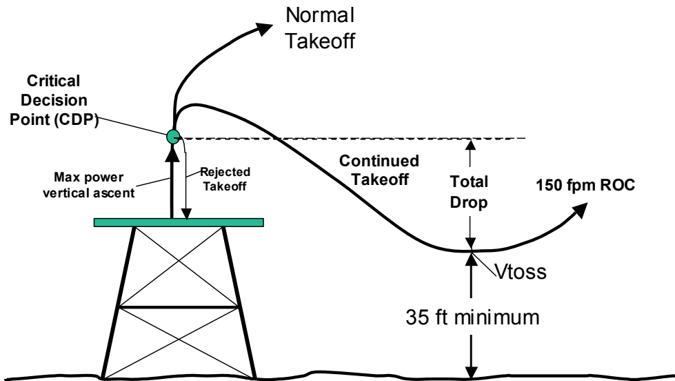
Figure 1. Heliport vertical takeoff profile.
