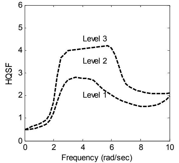
Figure 26. Handling qualities prediction boundaries
