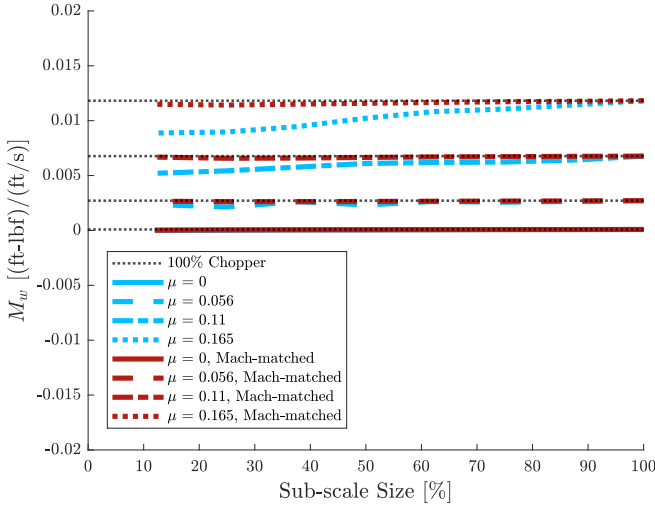
Figure 10. M_w from sub-scale vehicles of different lengths at \rho = 0.012 \text{ kg/m}^3 .
