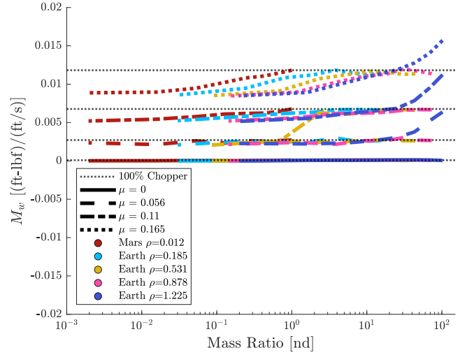
Figure 22. M_w from sub-scale vehicles of different lengths, gravitational accelerations, and atmospheric densities without Mach-matching.
