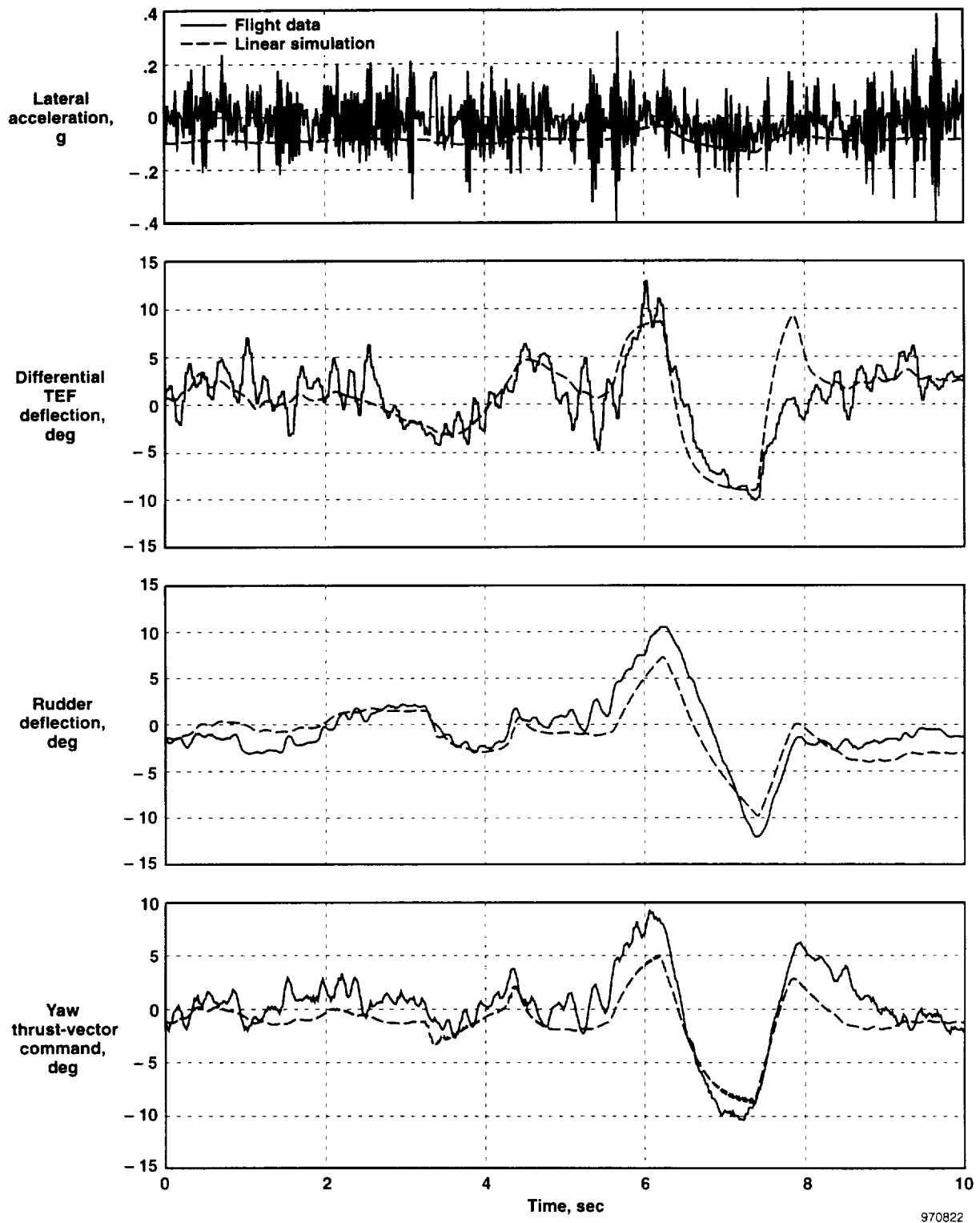
(b) Comparison of linear simulation response with flight data for a roll doublet at 45^\circ angle of attack.
