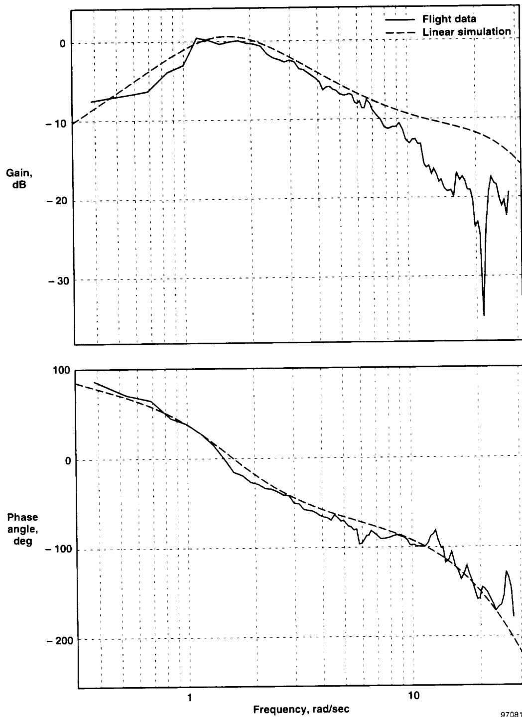
Figure 38. Frequency response comparison between linear simulation and flight data for Q/ALFC at 60^\circ angle of attack.
