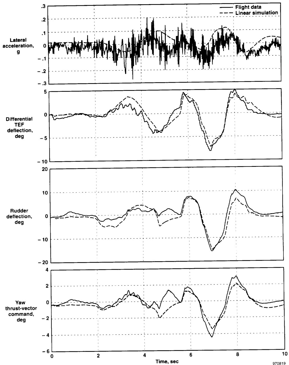
(b) Comparison of linear simulation response with flight data for a roll doublet at 30^\circ angle of attack.
