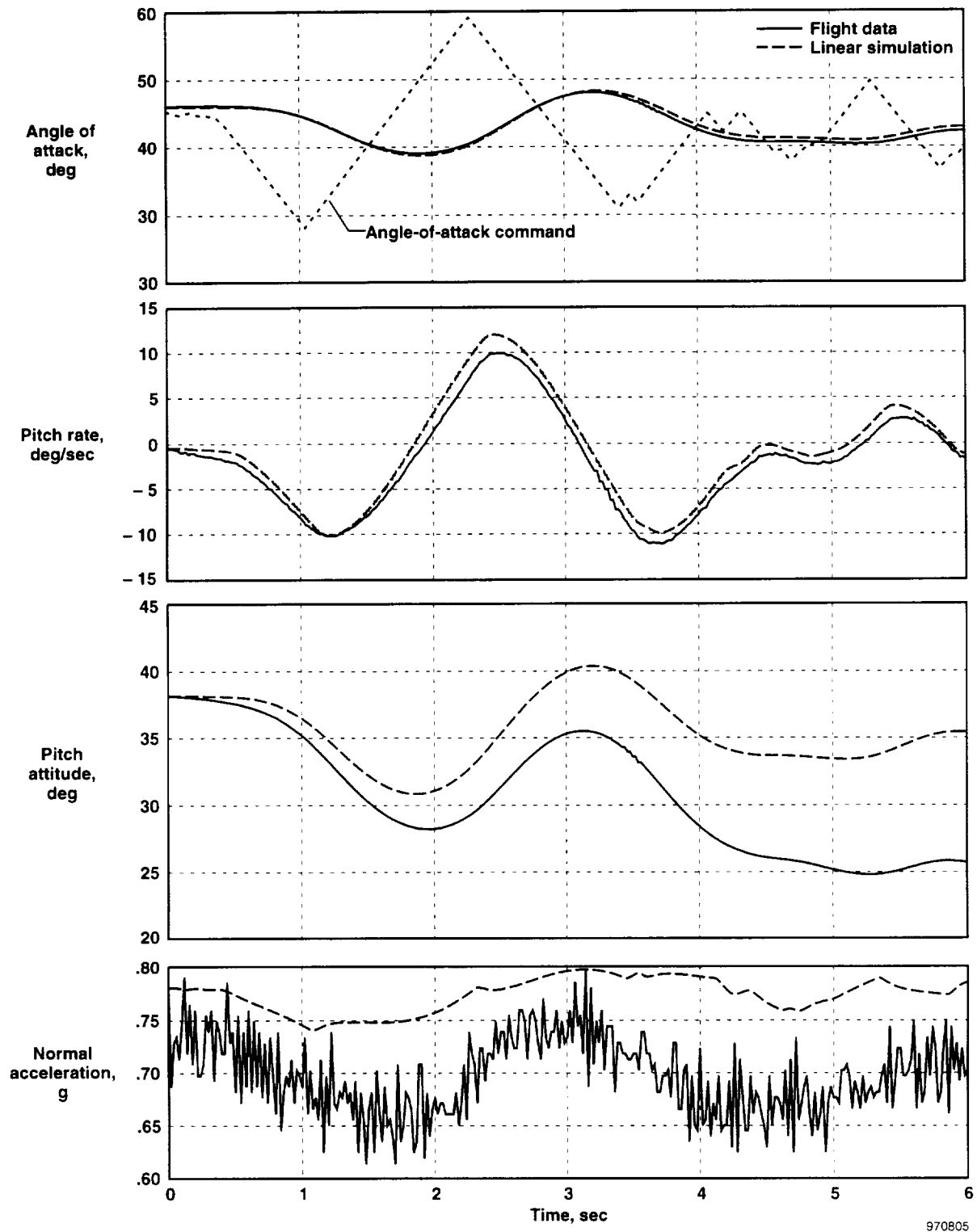
(a) Comparison of linear simulation response with flight data for a pitch doublet at 45^\circ angle of attack.
