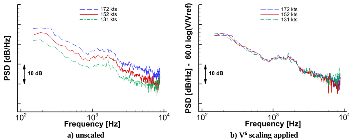
Fig. 5. Noise produced by the 804 aircraft in approach configuration with flaps deflected at 20^\circ and landing gear retracted. Spectra obtained from WingsNg integration of ARM-III test data for overhead position.
