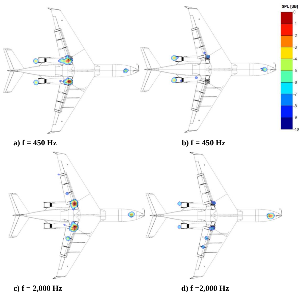
Fig. 19. Noise produced by 804 with Fowler flaps deflected 20°, without (left column) and with (right column) NR technologies installed – MLG fairings plus cavity chevrons and foam. Overhead position.
