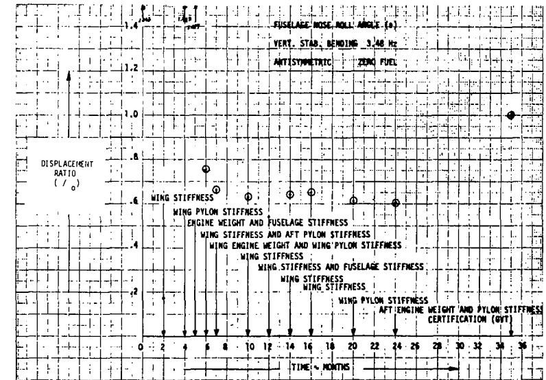
FIGURE 150. EVOLUTION OF DISPLACEMENT RATIO \theta
