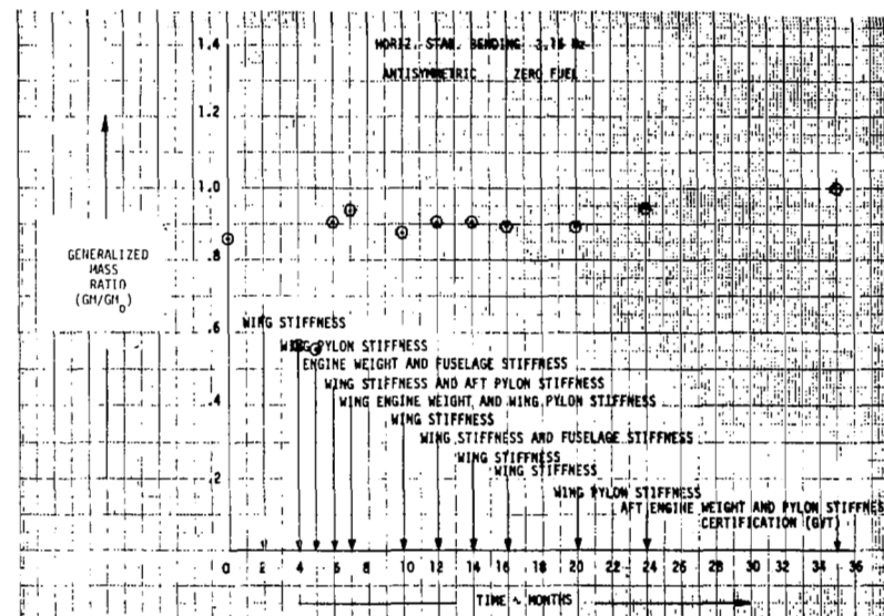
FIGURE 80. EVOLUTION OF GENERALIZED MASS RATIO
