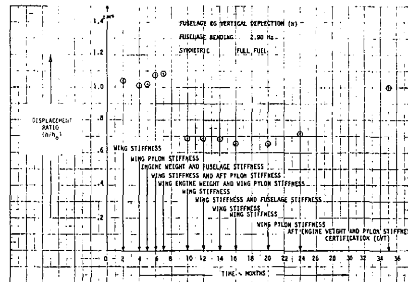
FIGURE 122. EVOLUTION OF DISPLACEMENT RATIO h
