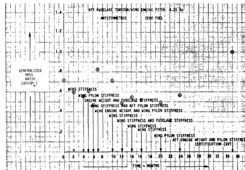
FIGURE 82. EVOLUTION OF GENERALIZED MASS RATIO
