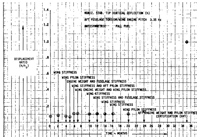
FIGURE 185. EVOLUTION OF DISPLACEMENT RATIO h
