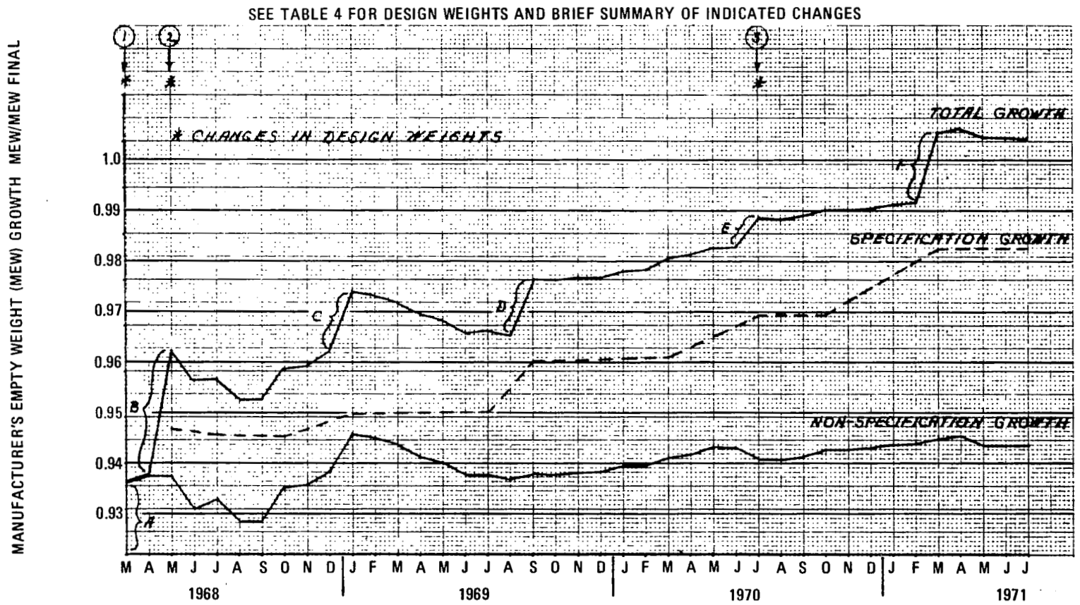
FIGURE 20. MANUFACTURER'S EMPTY WEIGHT GROWTH HISTORY
