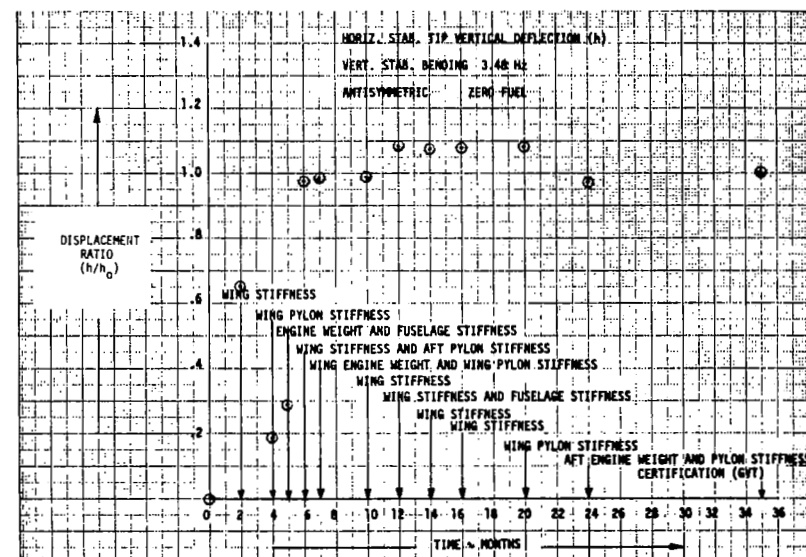
FIGURE 154. EVOLUTION OF DISPLACEMENT RATIO h
