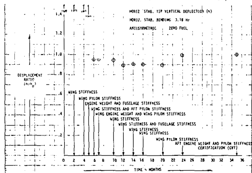
FIGURE 146. EVOLUTION OF DISPLACEMENT RATIO h
