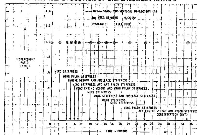
FIGURE 134. EVOLUTION OF DISPLACEMENT RATIO h
