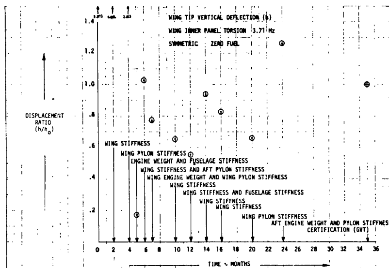
FIGURE 105. EVOLUTION OF DISPLACEMENT RATIO h
