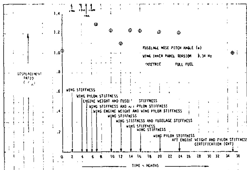
FIGURE 127. EVOLUION OF FUSELAGE \alpha DISPLACEMENT RATIO
