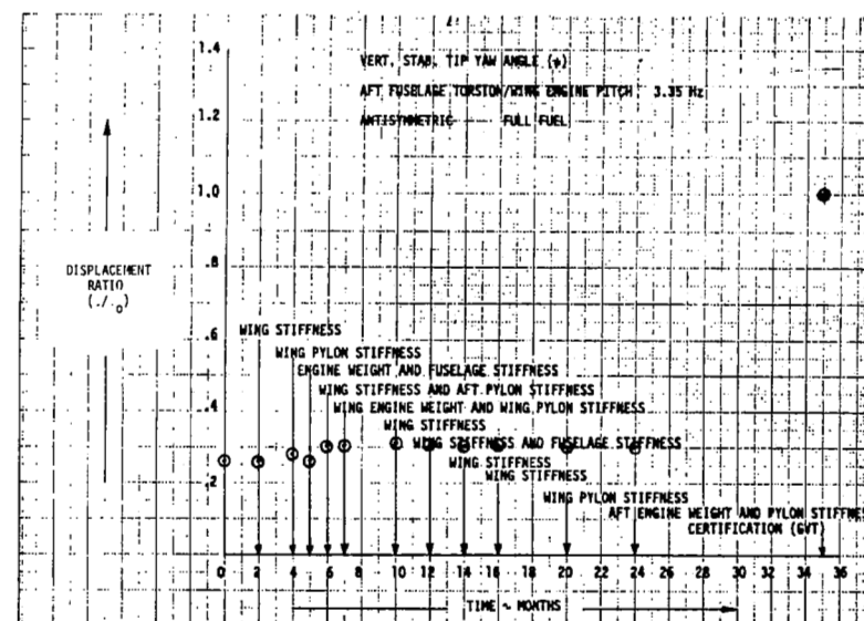
FIGURE 188. EVOLUTION OF DISPLACEMENT RATIO \psi
