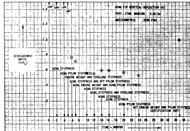
FIGURE 152. EVOLUTION OF DISPLACEMENT RATIO h
