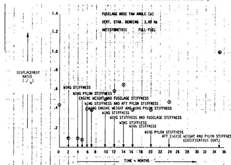
FIGURE 190. EVOLUTION OF DISPLACEMENT RATIO \psi
