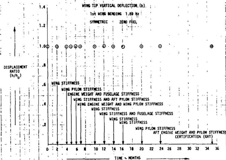
FIGURE 93. EVOLUTION OF DISPLACEMENT RATIO h
