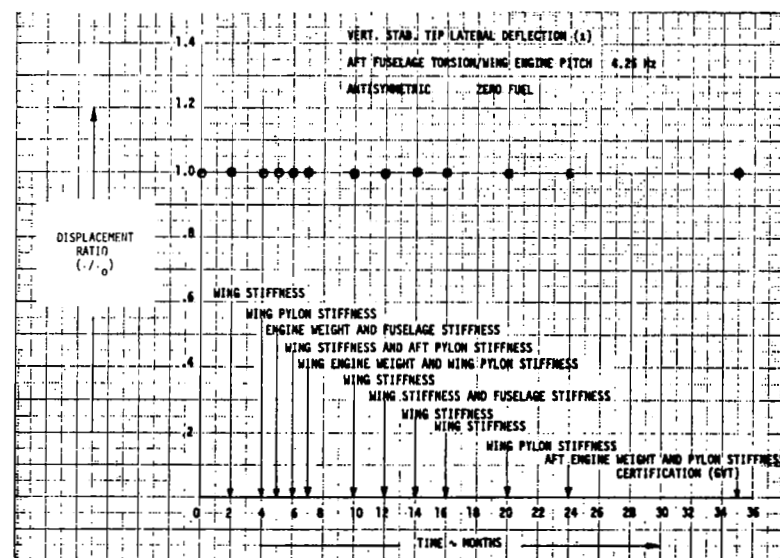
FIGURE 164. EVOLUTION OF DISPLACEMENT RATIO l
