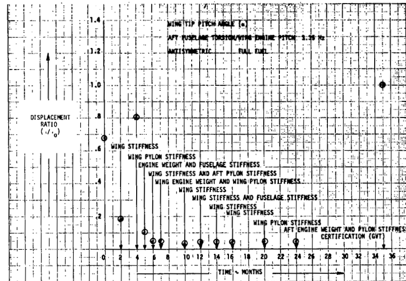
FIGURE 184. EVOLUTION OF DISPLACEMENT RATIO \alpha
