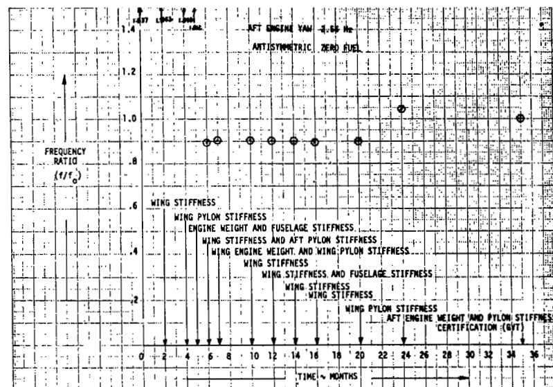
FIGURE 48. EVOLUTION OF FREQUENCY RATIO
