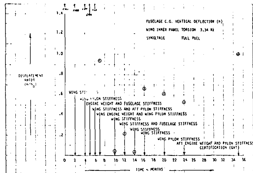
FIGURE 128. EVOLUTION OF DISPLACEMENT RATIO h
