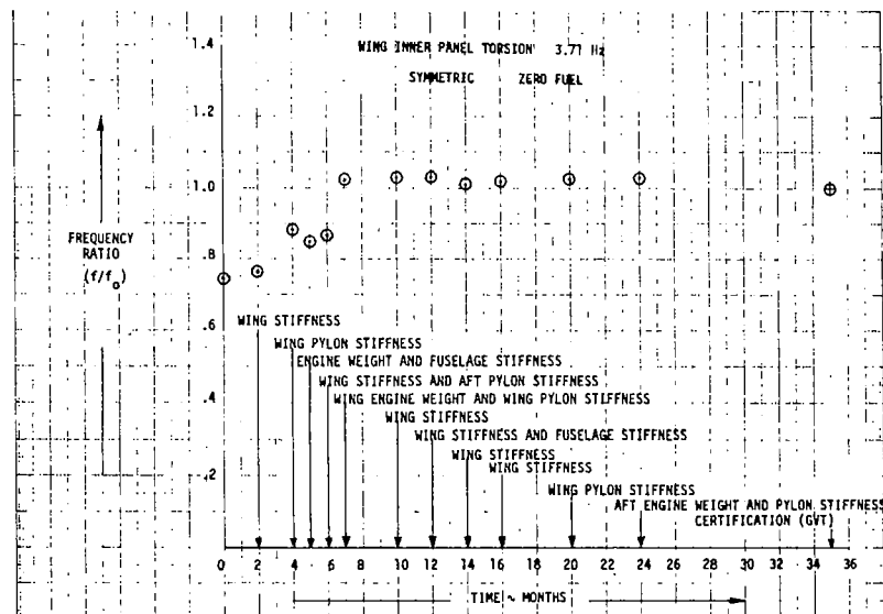
FIGURE 31. EVOLUTION OF FREQUENCY RATIO
