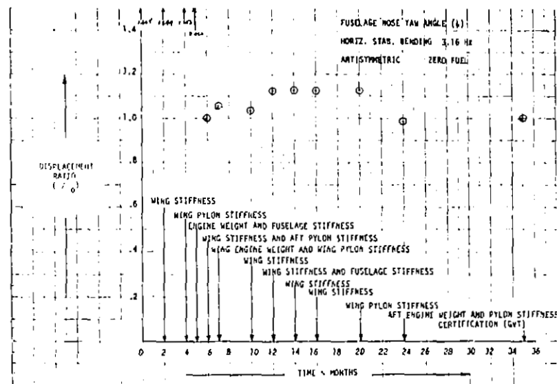
FIGURE 144. EVOLUTION OF DISPLACEMENT RATIO \psi
