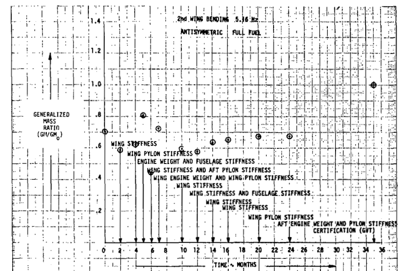
FIGURE 90. EVOLUTION OF GENERALIZED MASS RATIO
