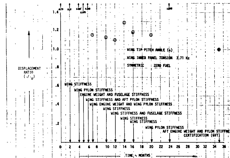
FIGURE 106. EVOLUTION OF DISPLACEMENT RATIO \alpha
