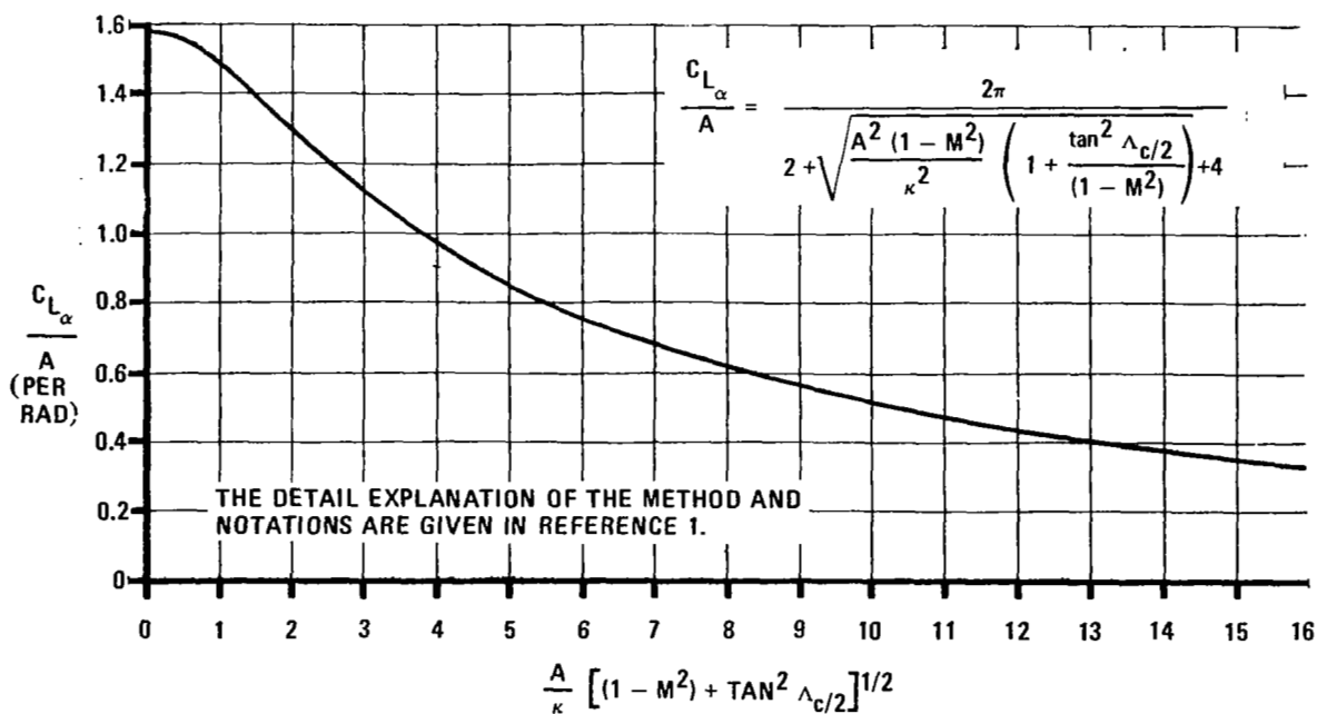
FIGURE 1. SUBSONIC WING LIFT-CURVE SLOPE
