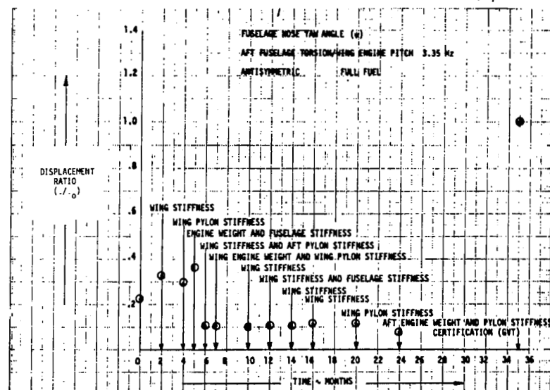
FIGURE 182. EVOLUTION OF DISPLACEMENT RATIO \theta
