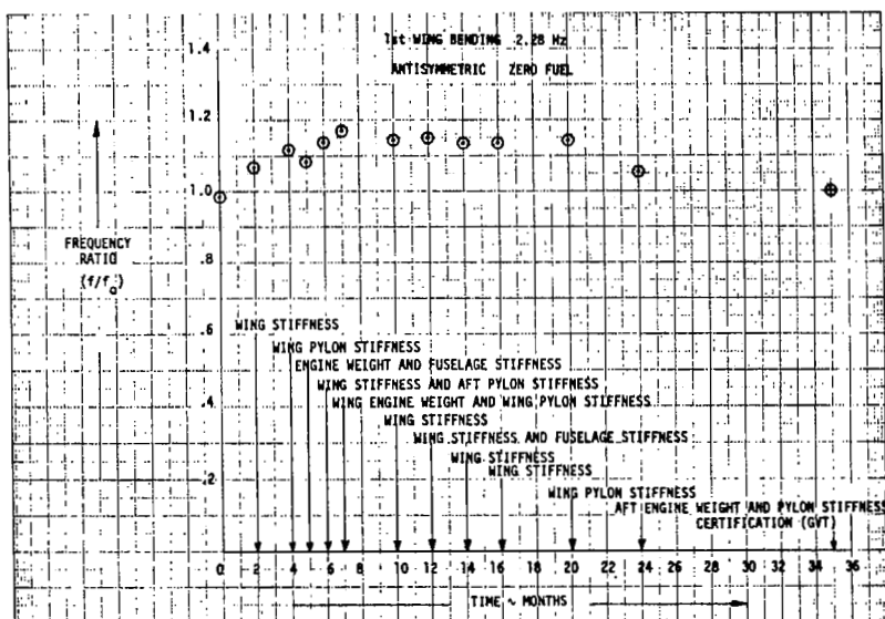
FIGURE 47. EVOLUTION OF FREQUENCY RATIO
