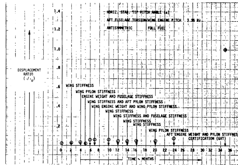
FIGURE 186. EVOLUTION OF DISPLACEMENT RATIO \alpha
