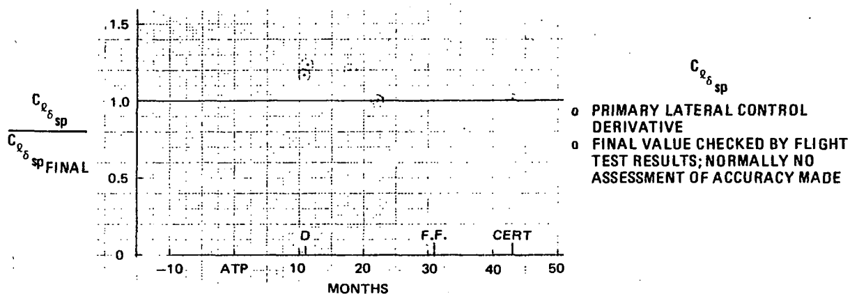
FIGURE 19. HISTORICAL UNCERTAINTIES OF LATERAL-DIRECTIONAL AERODYNAMIC PARAMETERS
