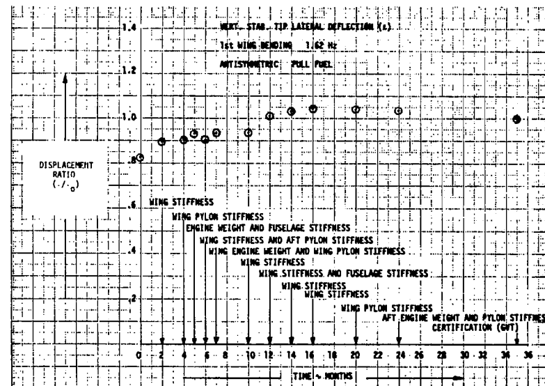
FIGURE 172. EVOLUTION OF DISPLACEMENT RATIO \beta
