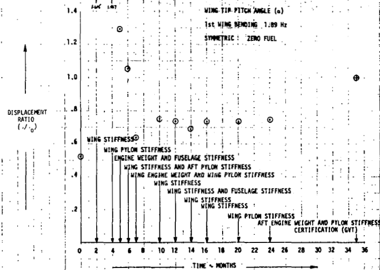
FIGURE 94. EVOLUTION OF DISPLACEMENT RATIO \alpha
