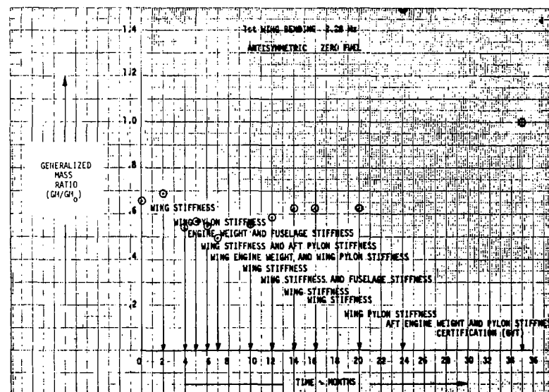
FIGURE 78. EVOLUTION OF GENERALIZED MASS RATIO
