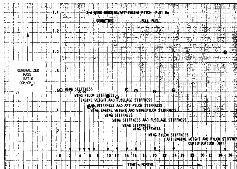
FIGURE 76. EVOLUTION OF GENERALIZED MASS RATIO
