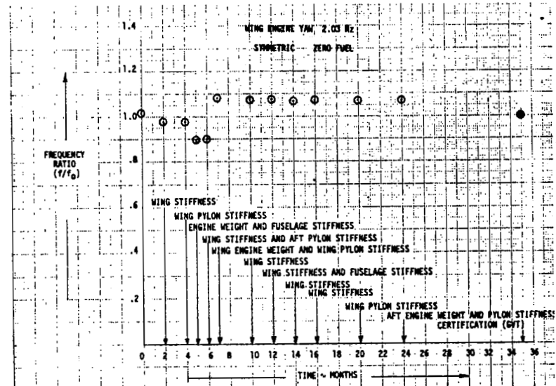
FIGURE 28. EVOLUTION OF FREQUENCY RATIO
