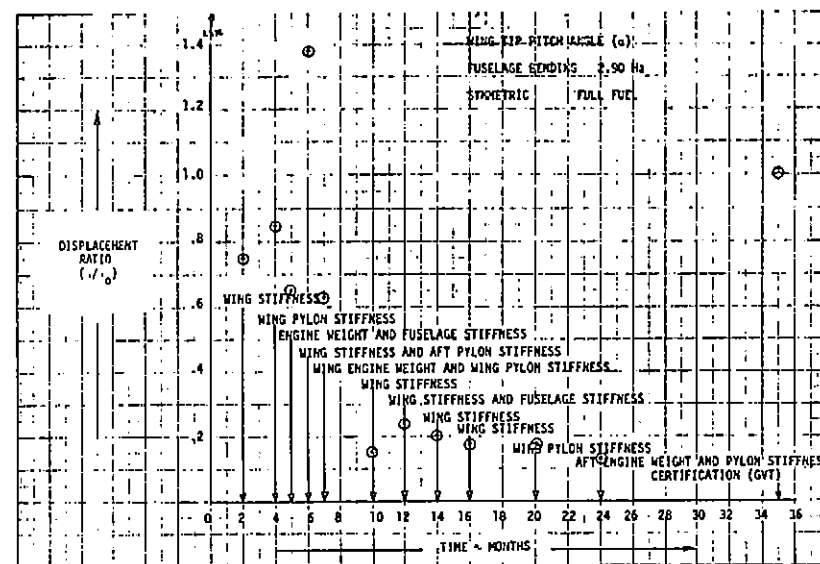
FIGURE 124. EVOLUTION OF DISPLACEMENT RATIO \alpha
