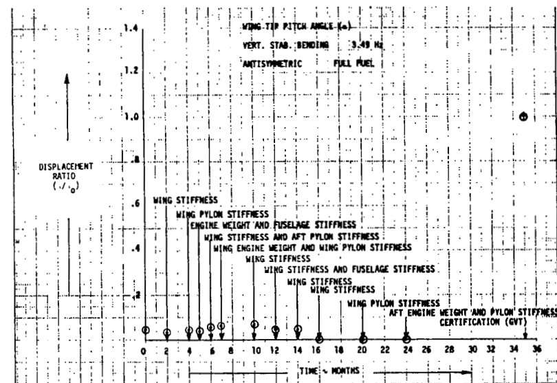
FIGURE 192. EVOLUTION OF DISPLACEMENT RATIO \alpha
