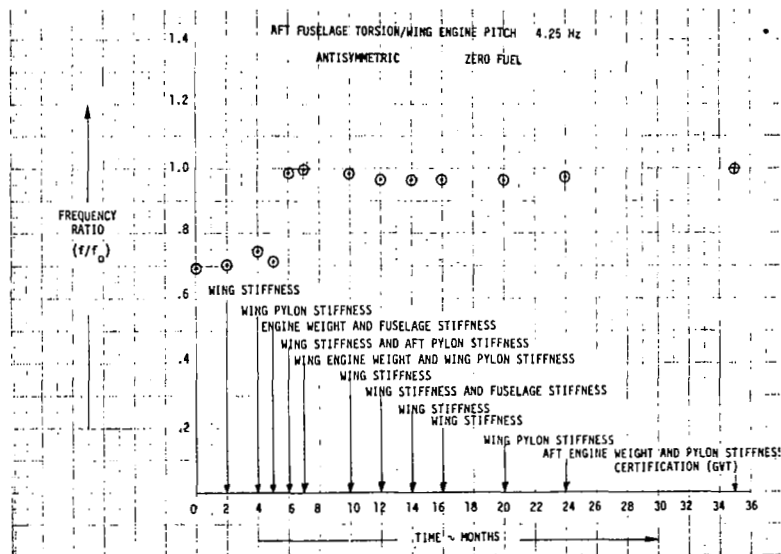
FIGURE 51. EVOLUTION OF FREQUENCY RATIO
