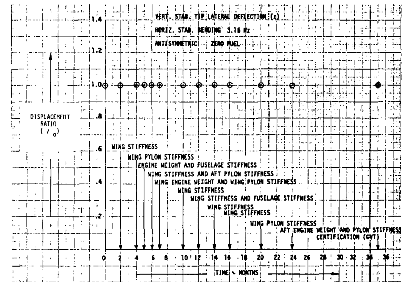
FIGURE 148. EVOLUTION OF DISPLACEMENT RATIO \rho
