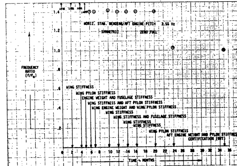
FIGURE 30. EVOLUTION OF FREQUENCY RATIO
