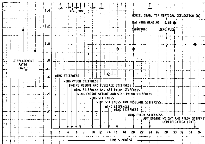
FIGURE 113. EVOLUTION OF DISPLACEMENT RATIO h
