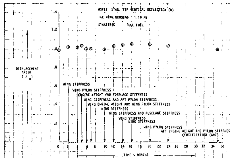
FIGURE 120. EVOLUTION OF DISPLACEMENT RATIO \alpha
