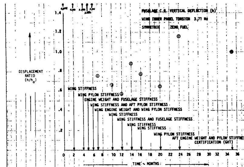
FIGURE 104. EVOLUTION OF DISPLACEMENT RATIO h
