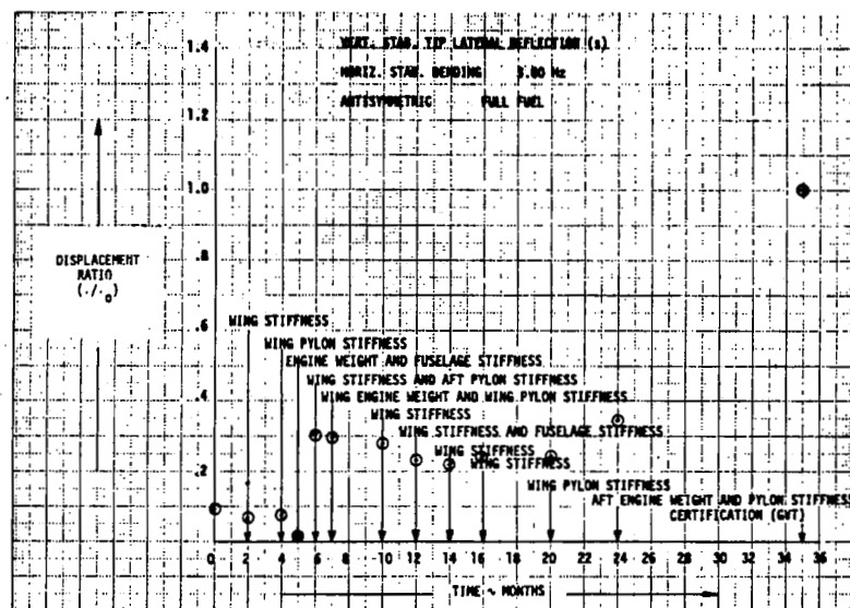
FIGURE 179. EVOLUTION OF DISPLACEMENT RATIO \delta
