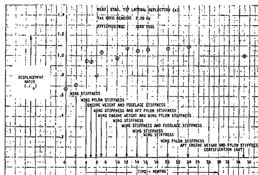
FIGURE 142. EVOLUTION OF DISPLACEMENT RATIO \epsilon
