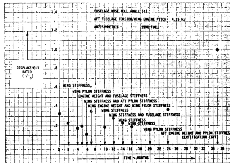
FIGURE 158. EVOLUTION OF DISPLACEMENT RATIO \theta
