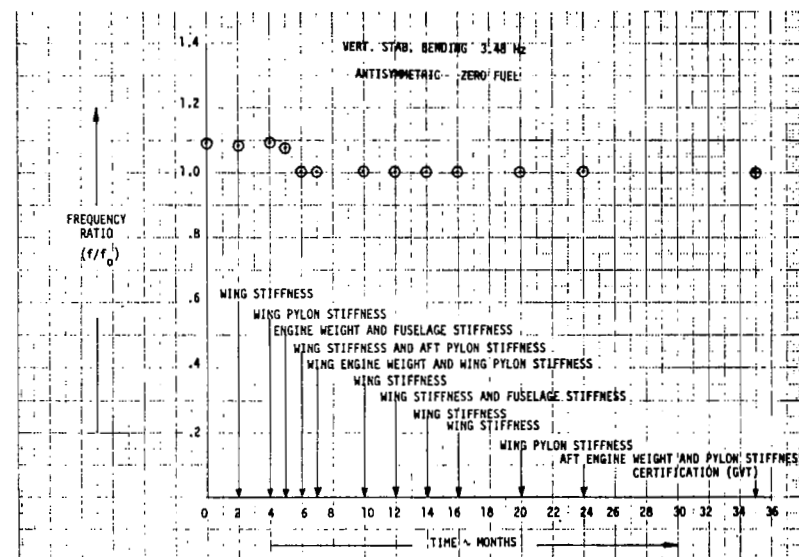
FIGURE 50. EVOLUTION OF FREQUENCY RATIO
