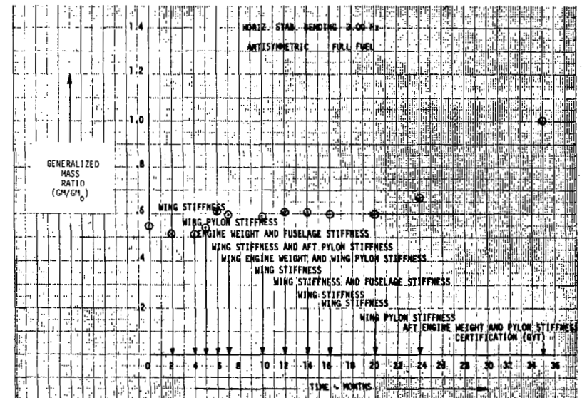
FIGURE 88. EVOLUTION OF GENERALIZED MASS RATIO
