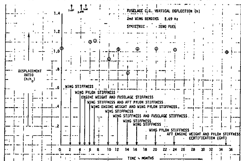
FIGURE 110. EVOLUTION OF DISPLACEMENT RATIO h
