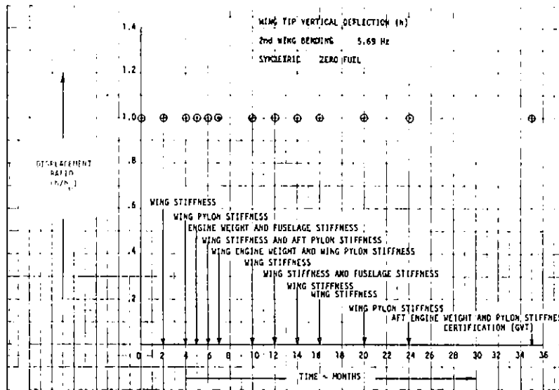
FIGURE 111. EVOLUTION OF DISPLACEMENT RATIO h
