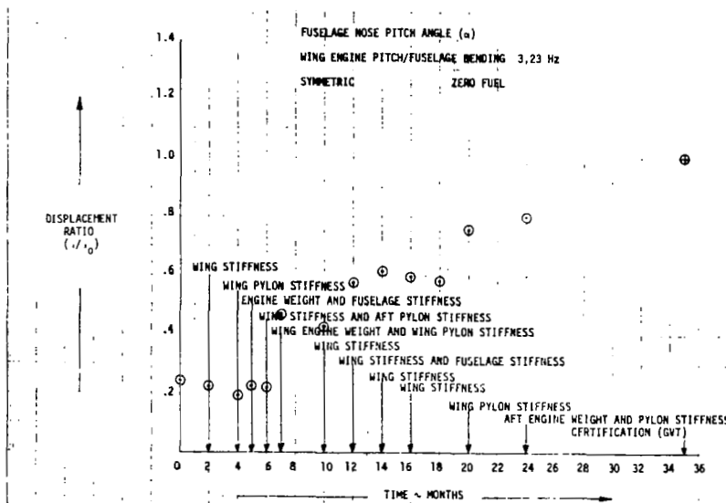
FIGURE 97. EVOLUTION OF DISPLACEMENT RATIO \alpha
