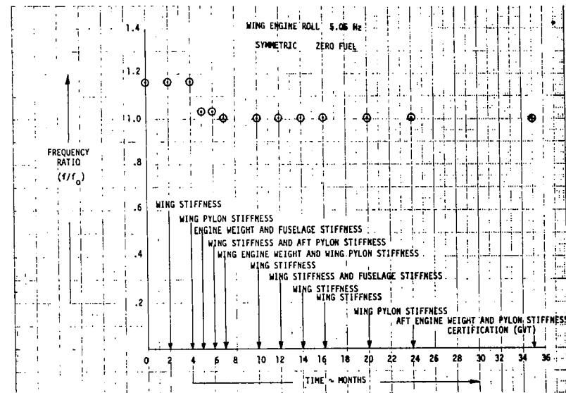
FIGURE 32. EVOLUTION OF FREQUENCY RATIO
