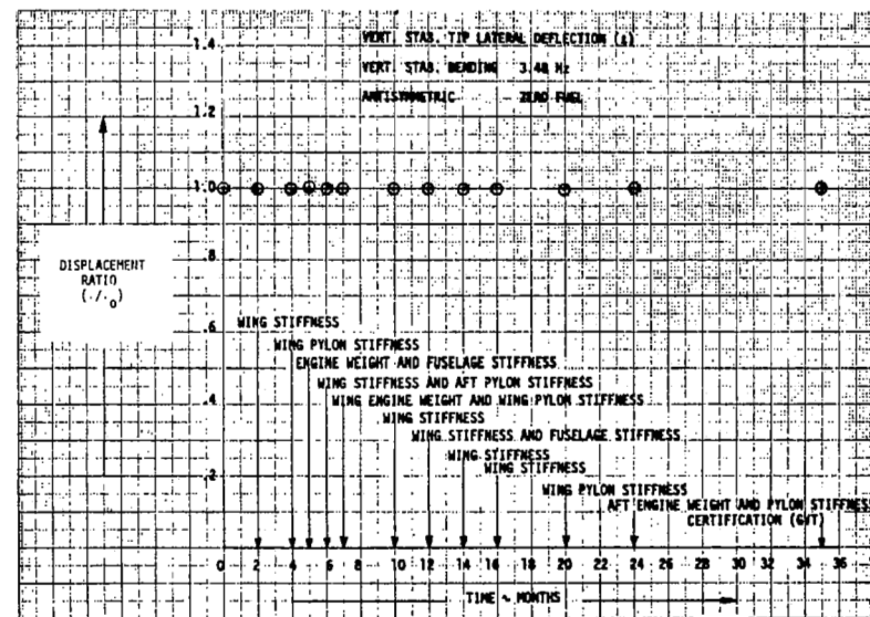
FIGURE 156. EVOLUTION OF DISPLACEMENT RATIO \rho
