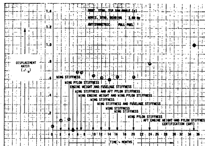
FIGURE 180. EVOLUTION OF DISPLACEMENT RATIO \delta
