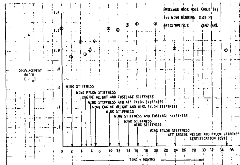
FIGURE 136. EVOLUTION OF DISPLACEMENT RATIO \theta
