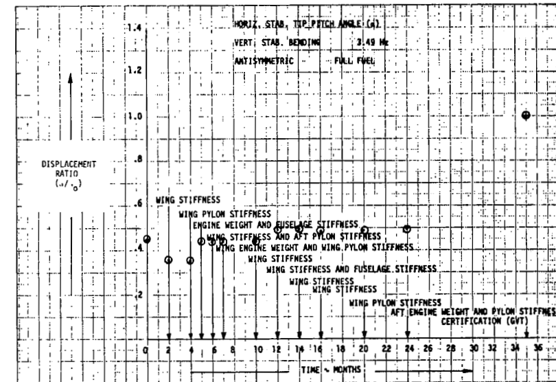
FIGURE 194. EVOLUTION OF DISPLACEMENT RATIO \alpha
