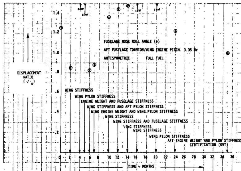
FIGURE 181. EVOLUTION OF DISPLACEMENT RATIO \theta
