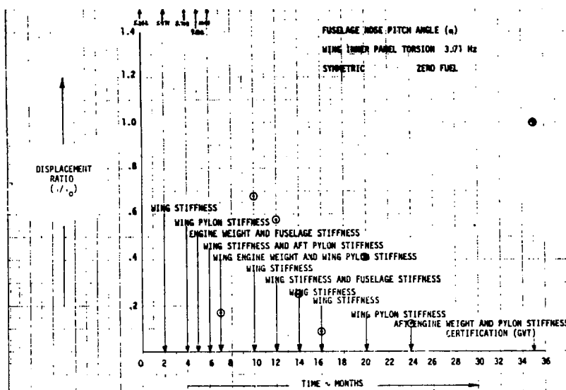
FIGURE 103. EVOLUTION OF DISPLACEMENT RATIO \alpha
