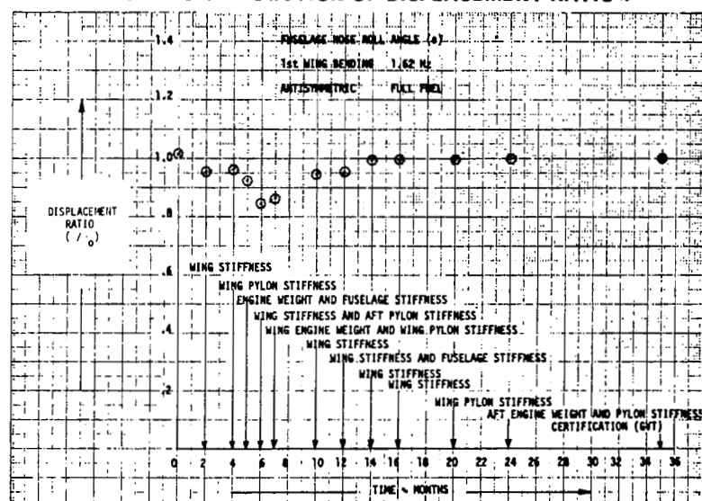
FIGURE 166. EVOLUTION OF DISPLACEMENT RATIO \theta
