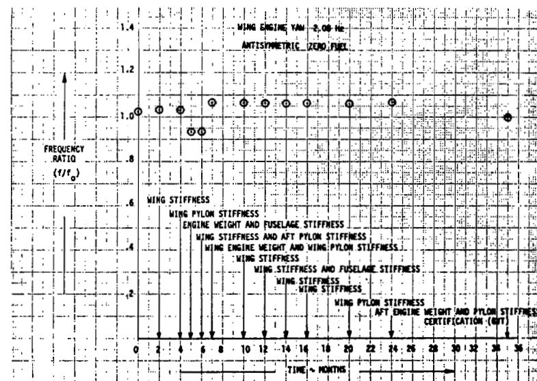
FIGURE 46. EVOLUTION OF FREQUENCY RATIO
