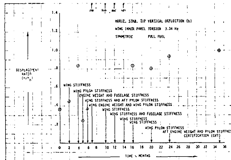
FIGURE 130. EVOLUTION OF DISPLACEMENT RATIO h
