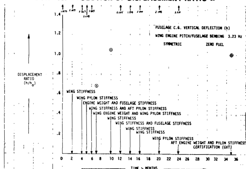
FIGURE 98. EVOLUTION OF DISPLACEMENT RATIO h
