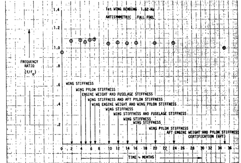
FIGURE 56. EVOLUTION OF FREQUENCY RATIO
