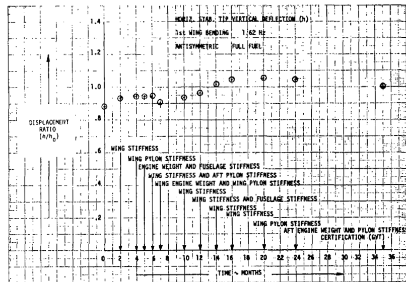
FIGURE 170. EVOLUTION OF DISPLACEMENT RATIO h
