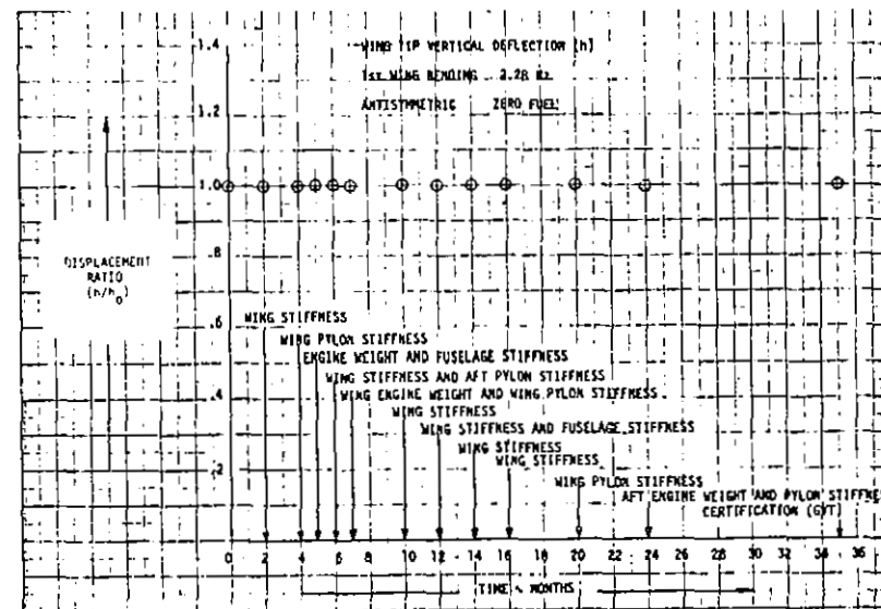
FIGURE 138. EVOLUTION OF DISPLACEMENT RATIO h
