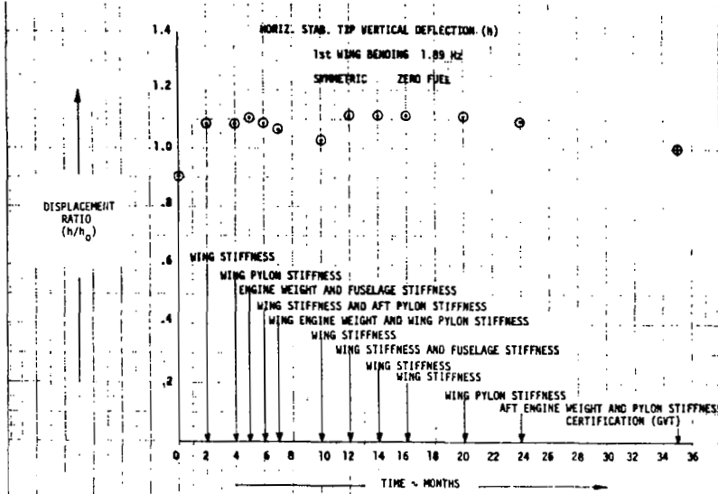
FIGURE 95. EVOLUTION OF DISPLACEMENT RATIO h
