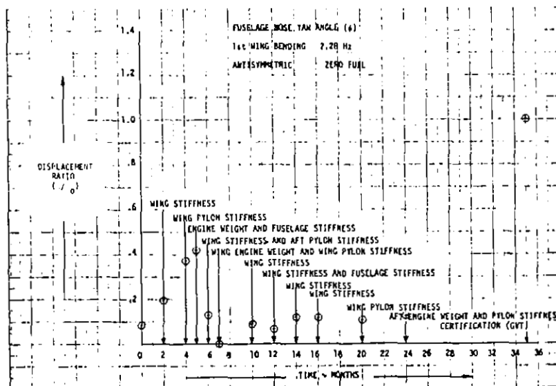
FIGURE 137. EVOLUTION OF DISPLACEMENT RATIO \psi
