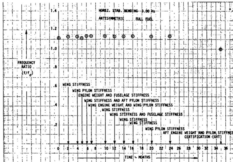
FIGURE 57. EVOLUTION OF FREQUENCY RATIO
