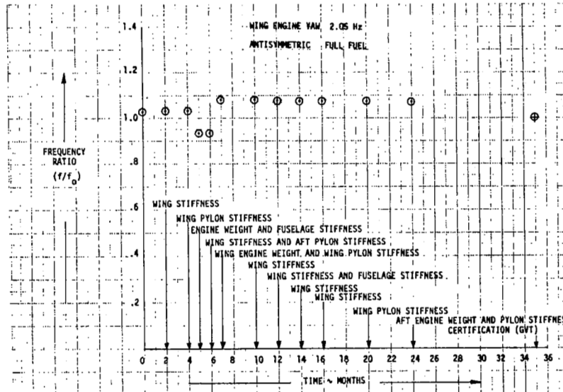
FIGURE 55. EVOLUTION OF FREQUENCY RATIO
