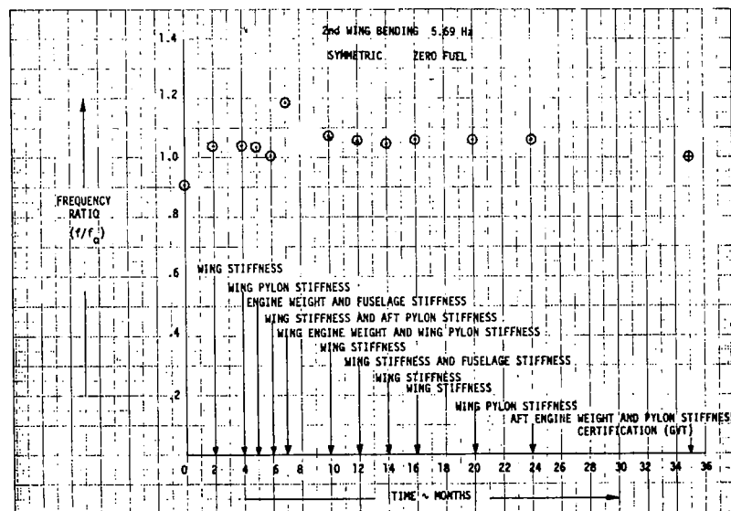
FIGURE 33. EVOLUTION OF FREQUENCY RATIO
