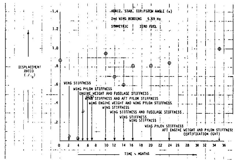
FIGURE 114. EVOLUTION OF DISPLACEMENT RATIO \alpha
