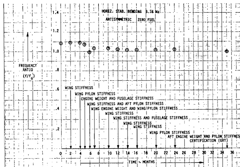
FIGURE 49. EVOLUTION OF FREQUENCY RATIO
