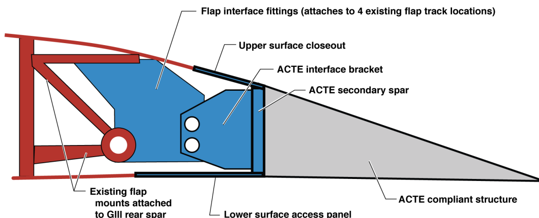
Figure 5. ACTE interface components (representative cross section).
