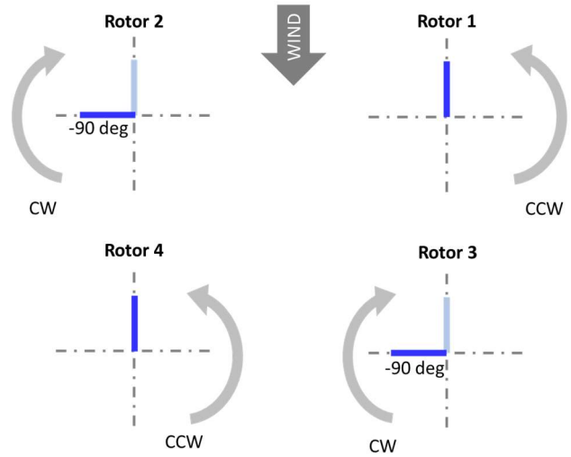
Figure 18: Schematic of rotors phased with -90 deg separation for R2 and R3 with respect to R1 and R4.
