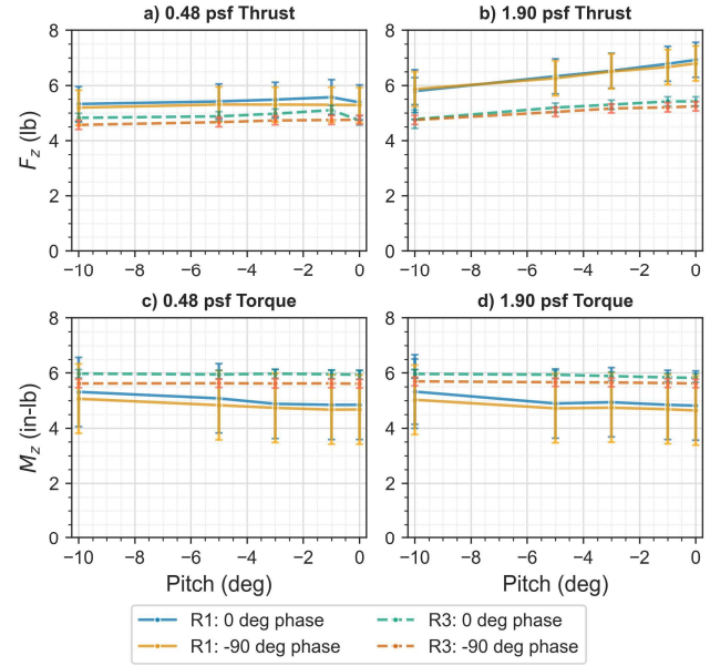
Figure 17: Starboard rotors phase comparison for thrust and torque or tandem configuration at dz/R=0.33 , q = 0.48 psf and 1.90 psf, RPM=3000, and tilt=0 deg.
