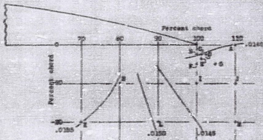
Figure 3.-Contours of C_{Dmin} . Symmetrical, auxiliary airfoil used as a flap. Reference point and flap axis: 25 percent point of flap chord.
