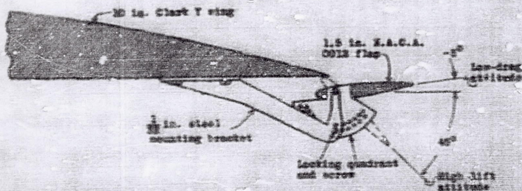
Figure 1.-Longitudinal cross section of wind-tunnel model. Flap mounted in the optimum position.
