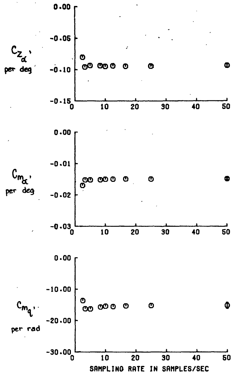
Figure 15. Estimated longitudinal derivatives as a function of sampling rate. Aircraft C.
