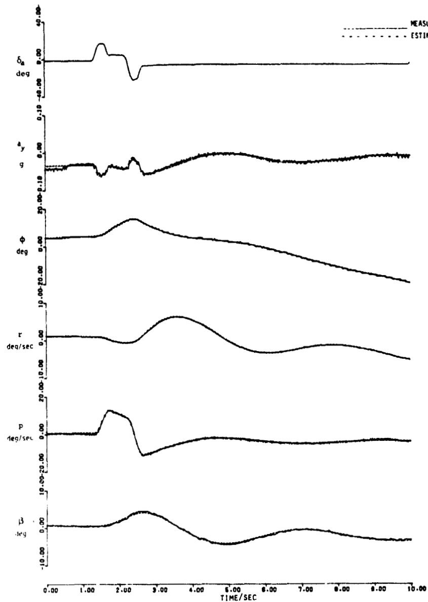
(a) Aircraft A; \delta_a pulse.
