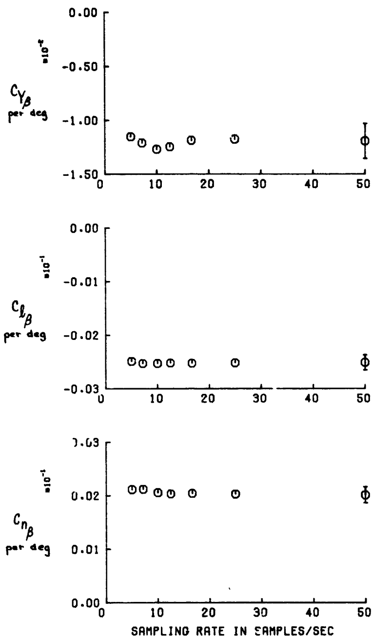
(c) C_{Y\beta} , C_{L\beta} , C_{n\beta} for case 1:10B
