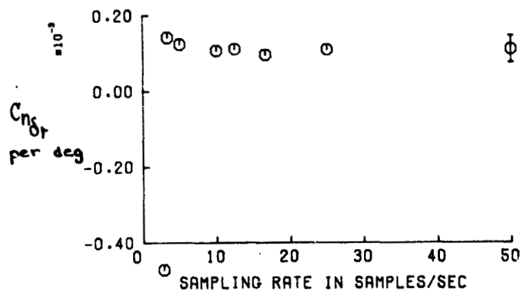
(e) C_{Y\delta r} , C_{L\delta r} , C_{n\delta r} FIGURE 11. CONCLUDED.
