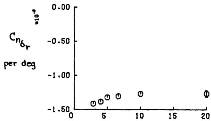
(s) C_{Y\delta_r} , C_{l\delta_r} , C_{n\delta_r} FOR CASE 7.17.
