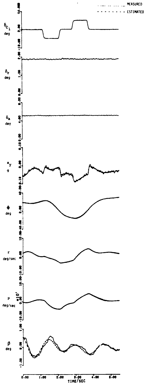
(b) Aircraft B; \delta_{C_1} pulse.
