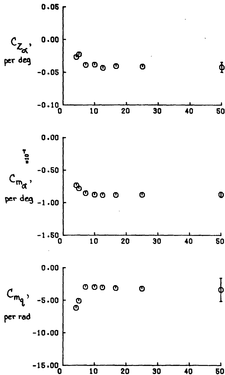
(c) C_{Z_{\alpha}} , C_{m_{\alpha}} , C_{m_q} , for case 2:4.
