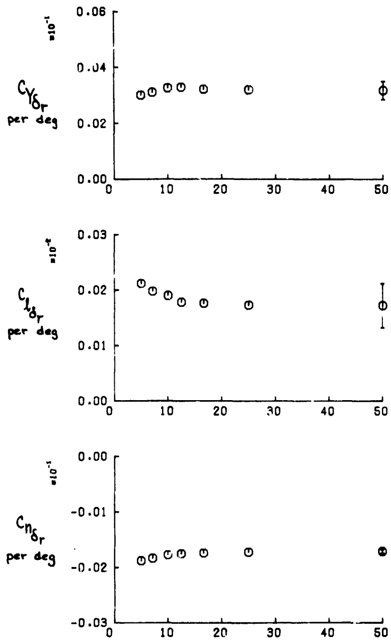
(p) C_{Y\delta r} , C_{L\delta r} , C_{n\delta r} for case 1:2. Figure 10. Continued.
