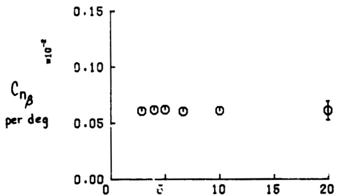
(c) C_{Y\beta} , C_{I\beta} , C_{n\beta} FOR CASE 7:9
