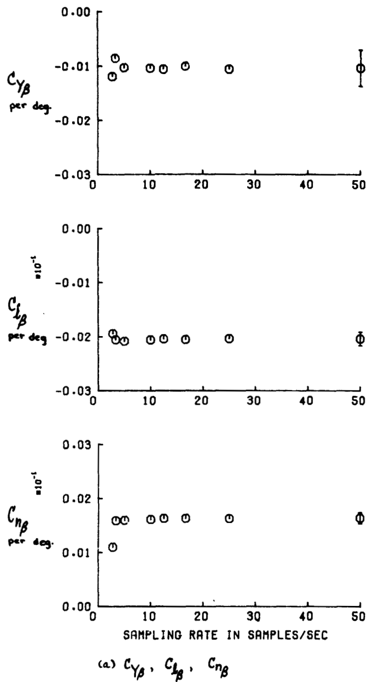
Figure 11. Estimated lateral-directional derivatives as a function of sampling rate, Aircraft C.
