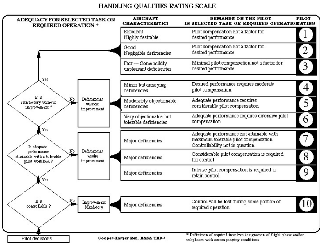
Figure 6.1. Cooper-Harper Handling Qualities Rating Scale [Cooper and Harper, 1969].
