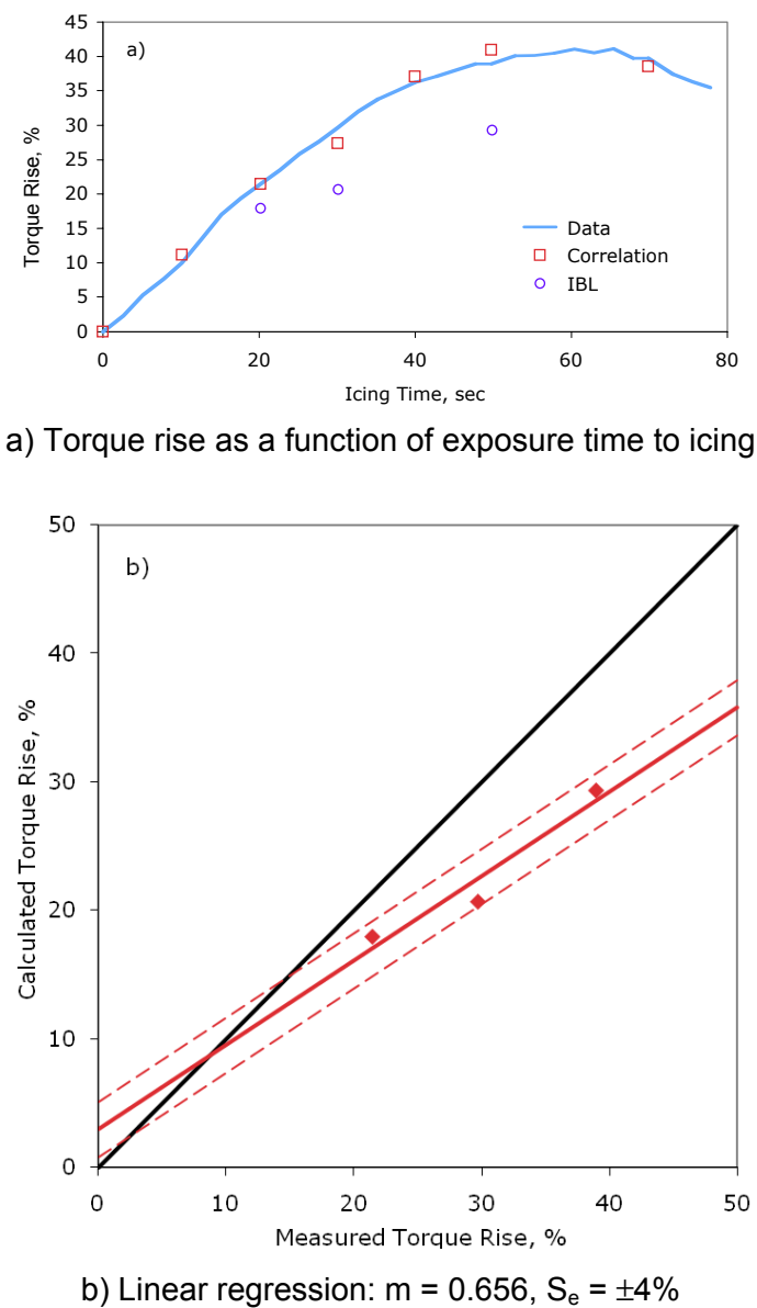
Figure 2.38. Predictive accuracy of Interactive Boundary Layer (IBL) method [Britton, 1992].
