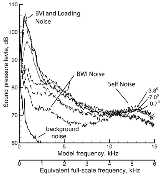
Figure 3.12. Measured noise spectra for a range of shaft angles showing the dominant noise sources for different frequency ranges.
