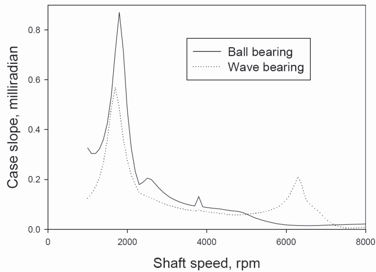
Figure 3.20. Angular vibration of transmission case for 28 \times excitation.
