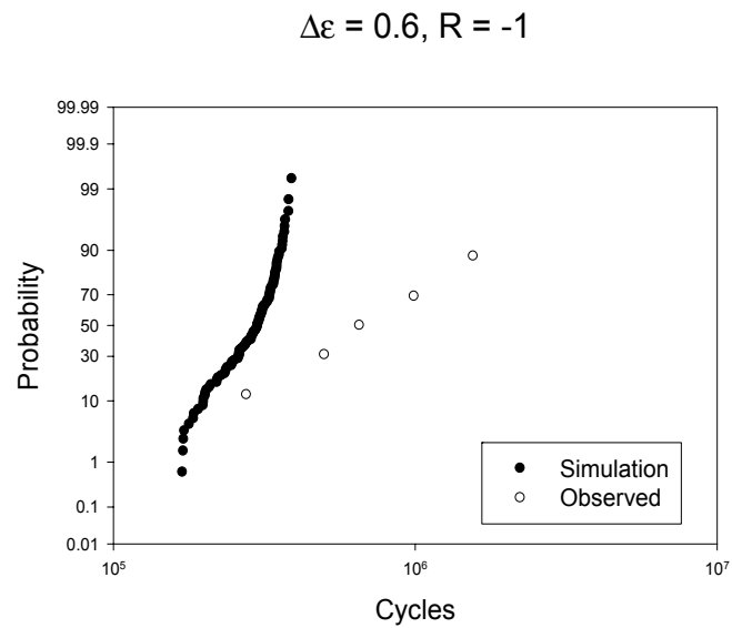
Figure 8.1. Comparison of fatigue life of “seeded” fatigue test bars with the simulated crack propagation lives using the distribution of the simulated largest inclusion in the test bar as the starting crack size.
