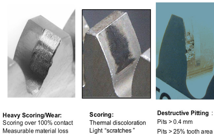
Figure 7.10. Conceptual gear failure mechanism map.
