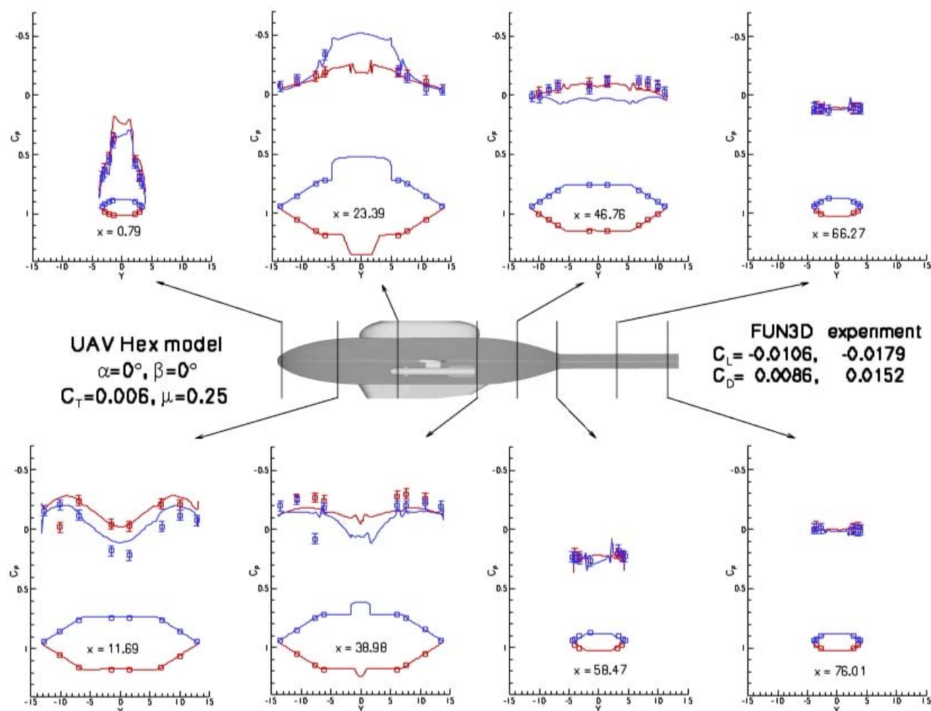
Figure 4.17. Computational pressures from FUN3D using an actuator-disk model compared with experiment for the UAV Hex model [Jones et al., 2006], taken from Mineck and Jones [to be published].
