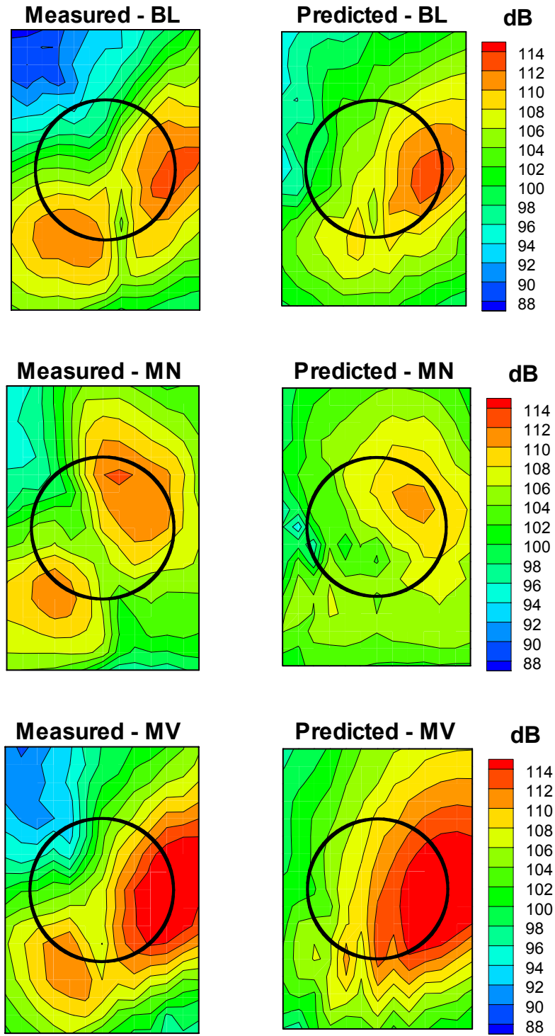
Figure 3.15. HART-II midfrequency measured versus predicted BVI SPL for Baseline (BL), Minimum Noise (MN), and Minimum Vibration (MV) cases. Predictions use measured blade motion.
