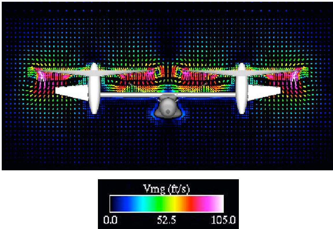
Figure 9.5. Under development: Tools incorporating CFD into the conceptual design process (LCTR2 images courtesy of G. Rajagopalan, Sukra-Helitek, Inc.).
