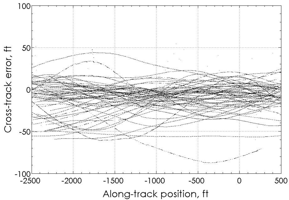
Figure 6.24. Lateral tracking position error [Decker et al., 2007].
