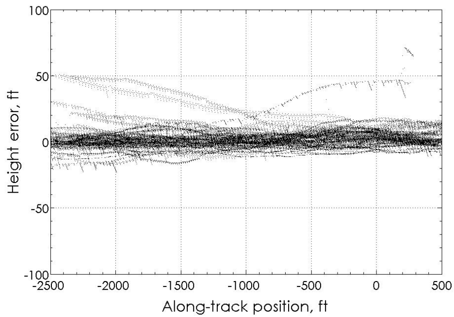
Figure 6.23. Height tracking error [Decker et al., 2007].
