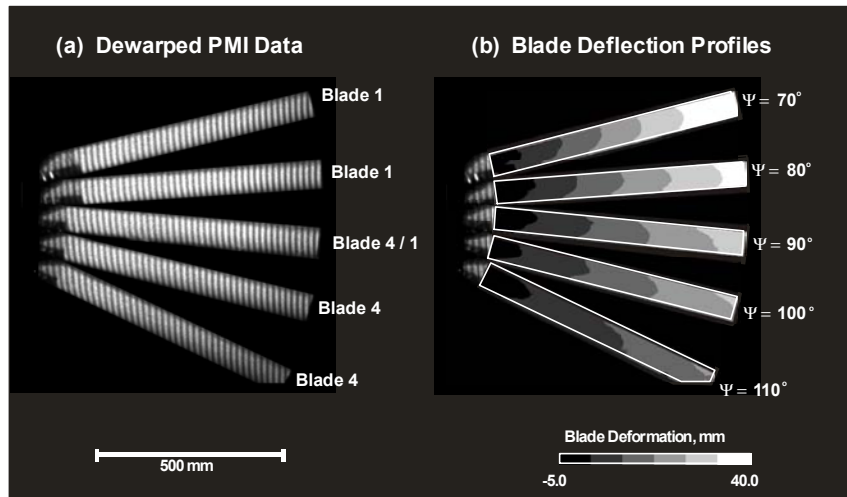
Figure 5.15. Azimuth-dependent PMI measured blade-deformation profiles, rotor shaft angle = -3^\circ [Fleming and Gorton, 1998].
