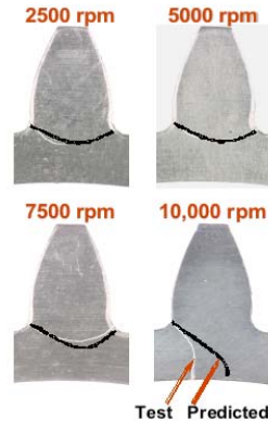
Figure 7.15. Comparison of analytically predicted and experimental gear root crack trajectories.
