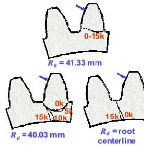
Figure 7.15. Comparison of analytically predicted and experimental gear root crack trajectories.
