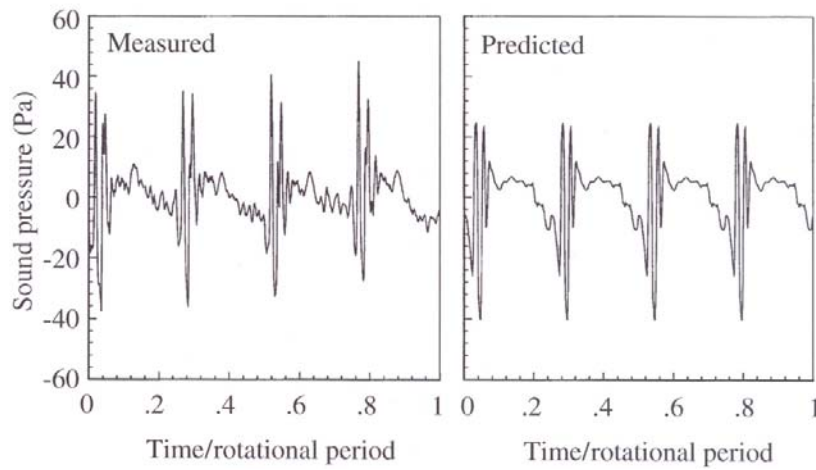
Figure 3.6 Measured and predicted acoustic time histories for HART test conditions. Microphone position corresponds to locations noted in figures 3.5a–e, respectively (from Brooks et al. [2000]).
