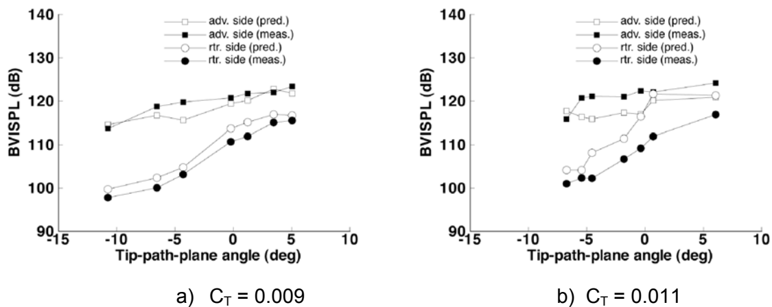
Figure 3.7. Measured and predicted maximum BVISPL vs. \alpha'_{TPP} for two different rotor thrusts.
