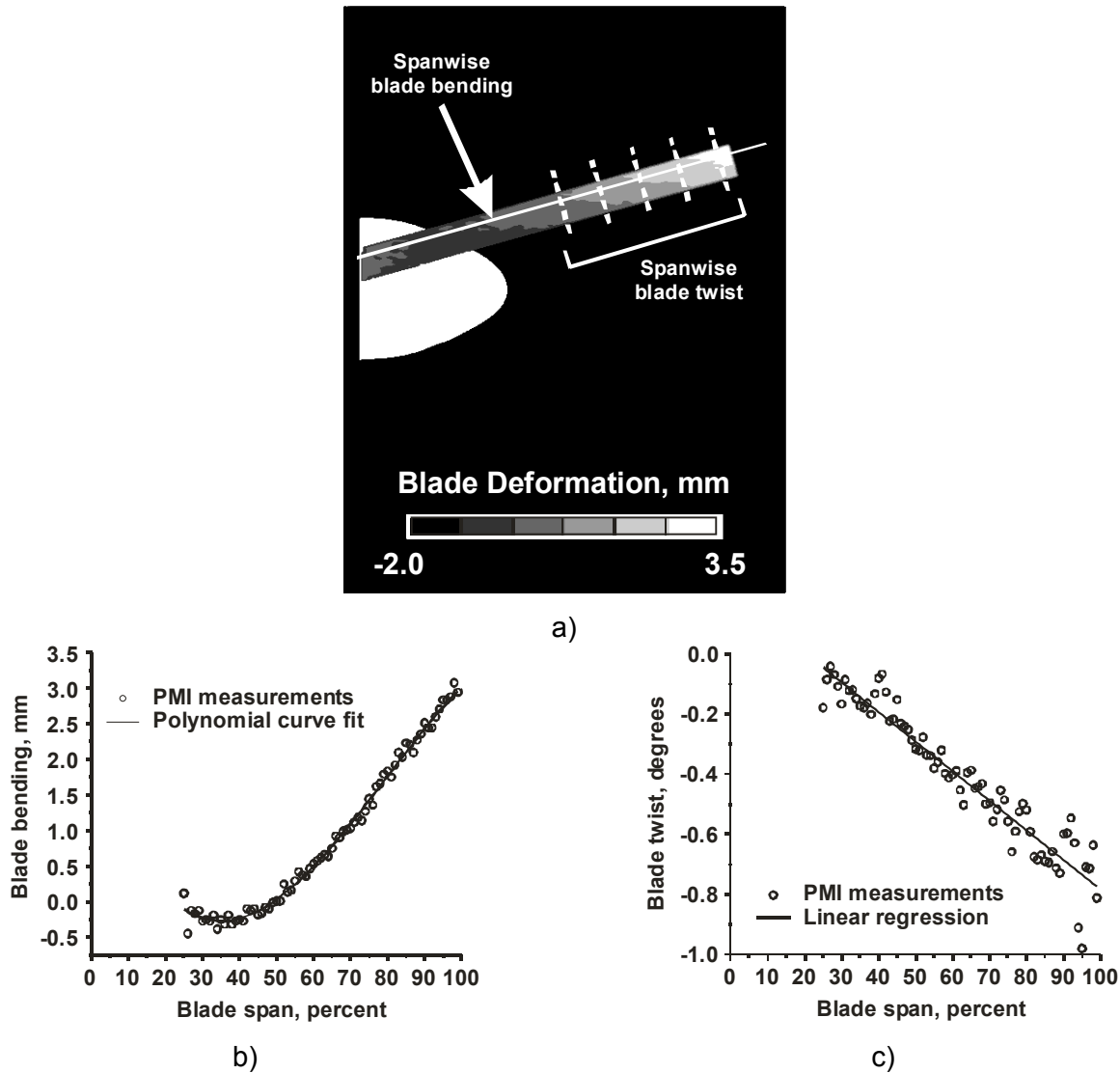
Figure 5.16. Blade-deformation measurements on Active Twist Rotor blades using PMI: (a) blade-deformation contours, (b) blade-bending distances as a function of span, and (c) blade-twist measurements as function of span [Fleming, 2002].
