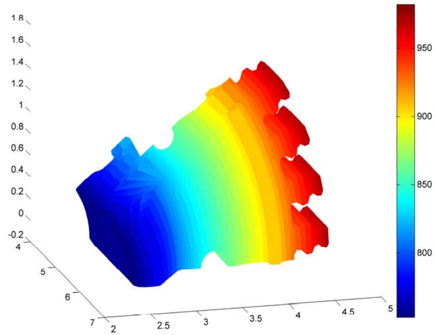
Figure 8.2. Comparison of (a) stress distribution in ksi and (b) temperature profile in °F with (c) probability of failure due to an inclusion-initiated crack, exponential scale—powers of 10, for a turboshaft engine disk.
