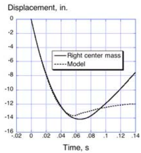
c) Displacement
