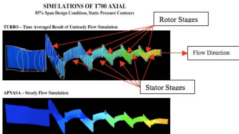
Figure 7.2. TURBO and APNASA predictions of T700 axial-compressor performance.
