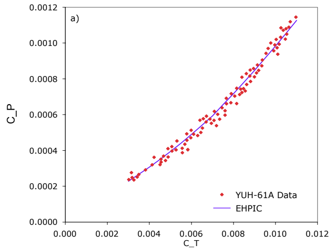
a) C_P as a function of C_T for Boeing YUH-61A
