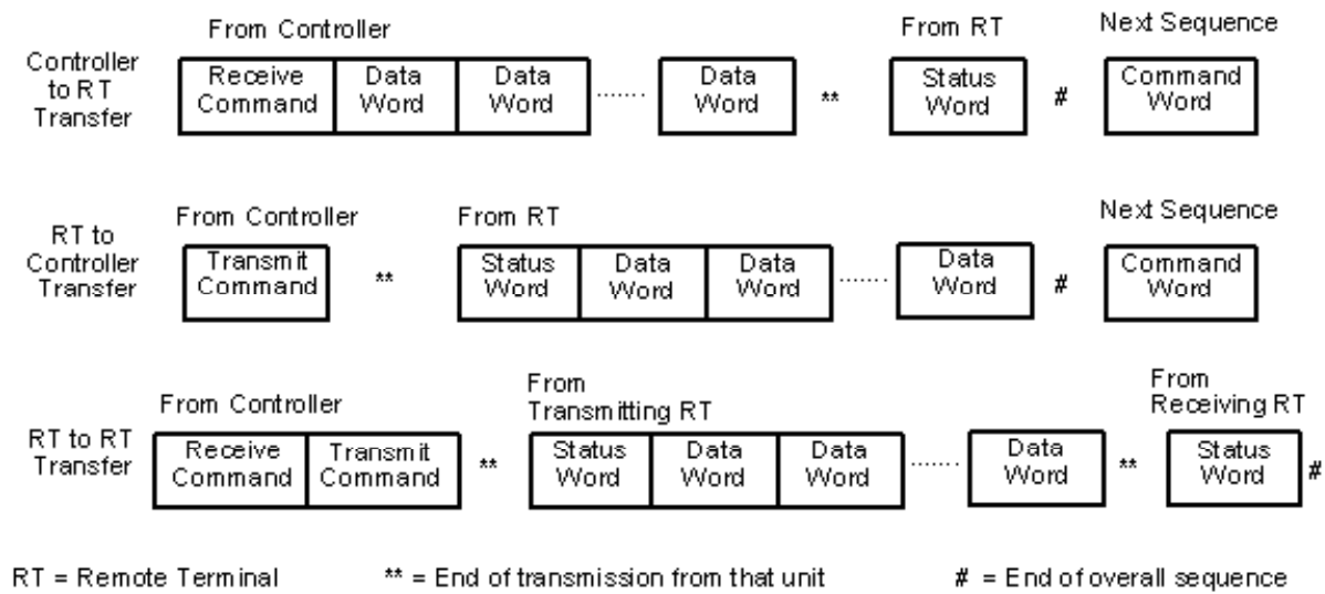
Figure 6.11. MIL-STD-1553 data-message formats [Garlington, 2000].
