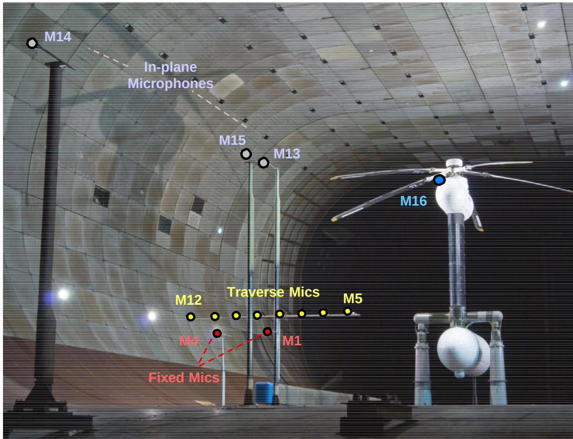
Figure 14a: SMART rotor in 40- by 80-foot anechoic test section and microphone configuration (looking downstream).
