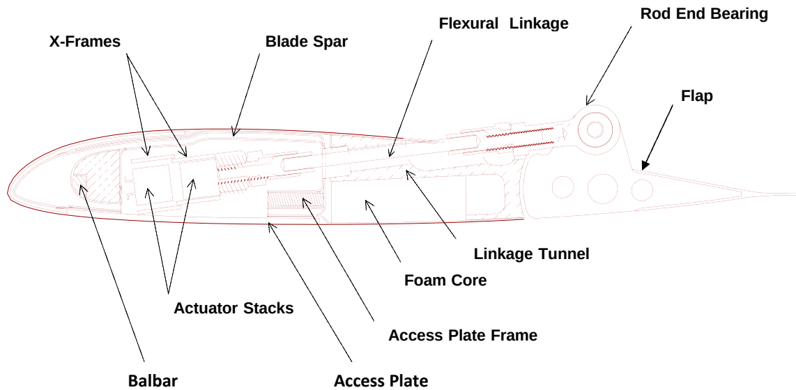
Figure 7b: Active flap rotor blade cross section.
