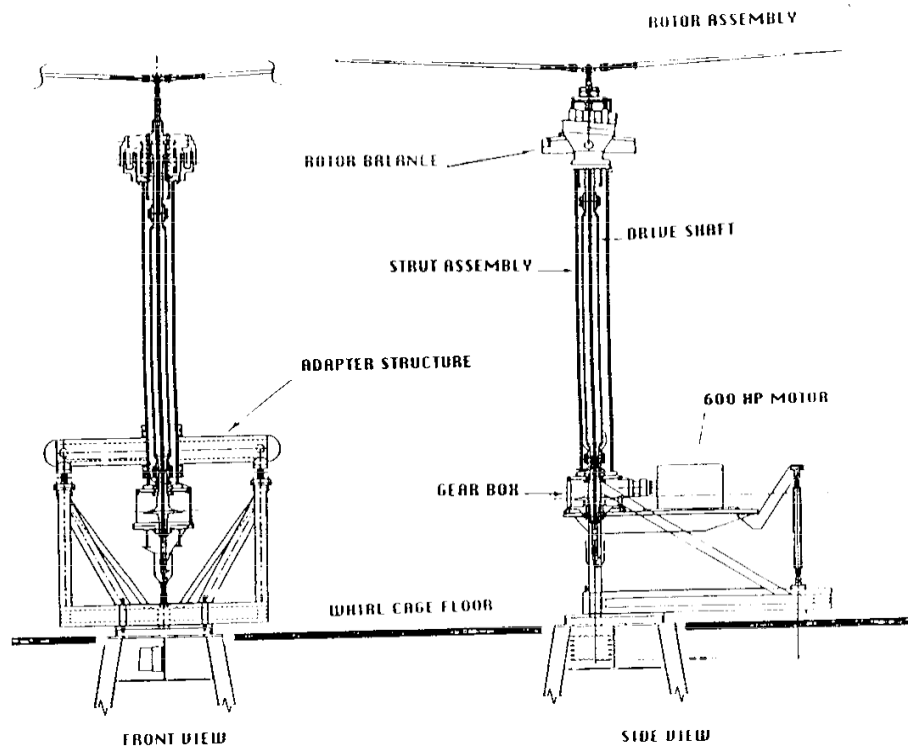
Figure 1a: Test stand, rotor, elevator setup (for LHX test).
