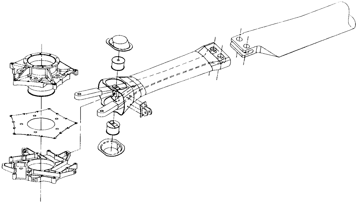
Figure 5: MD900 hub and blade root attachment structure.
