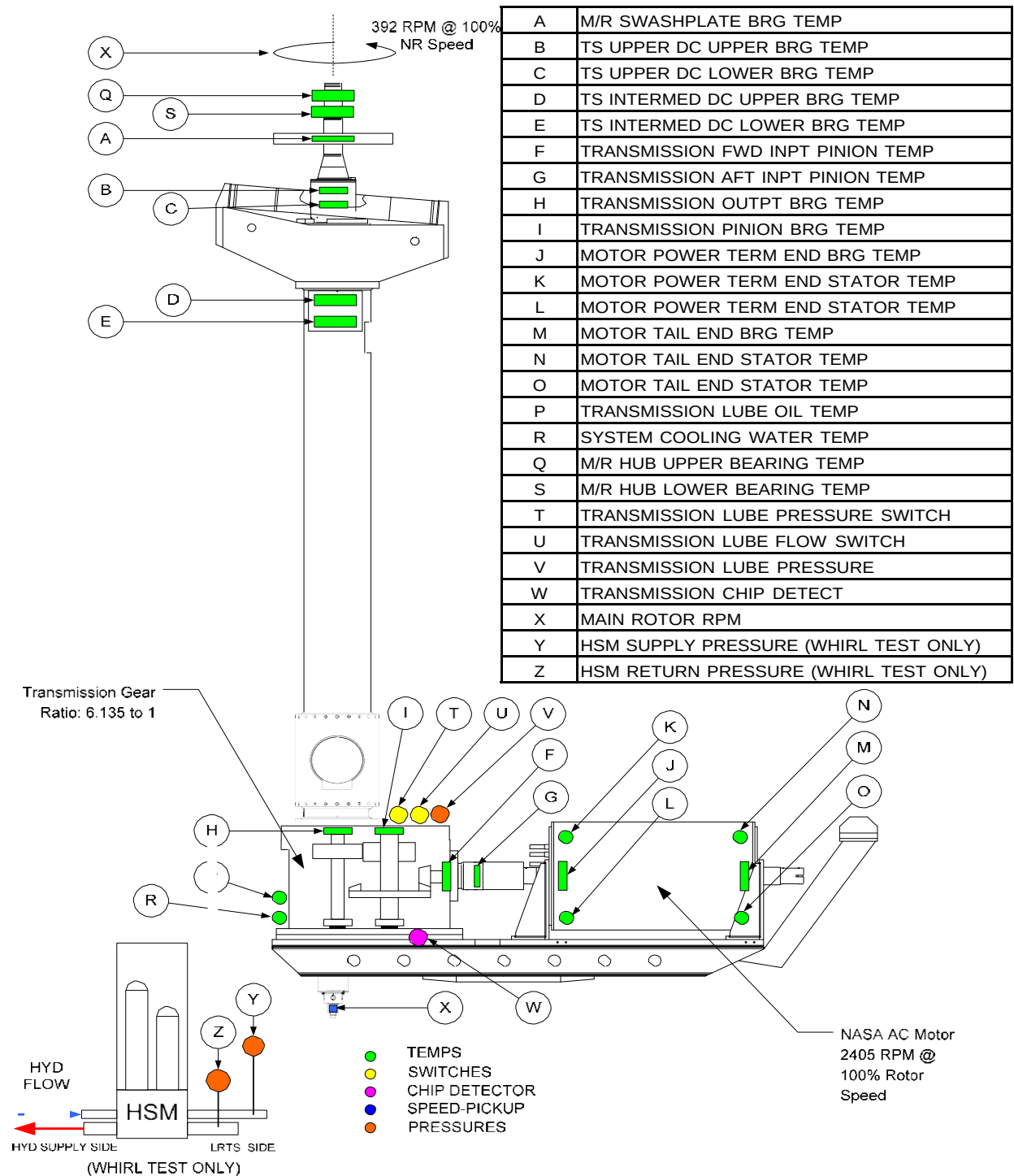
Figure 2b: Health monitoring system parameters.
