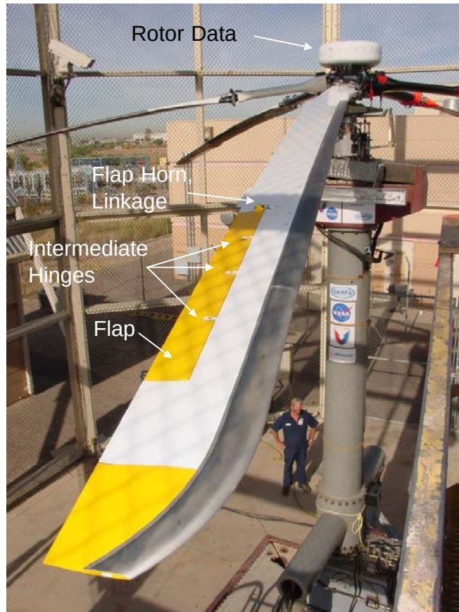
Figure 1c: SMART rotor at whirl tower (2003).
