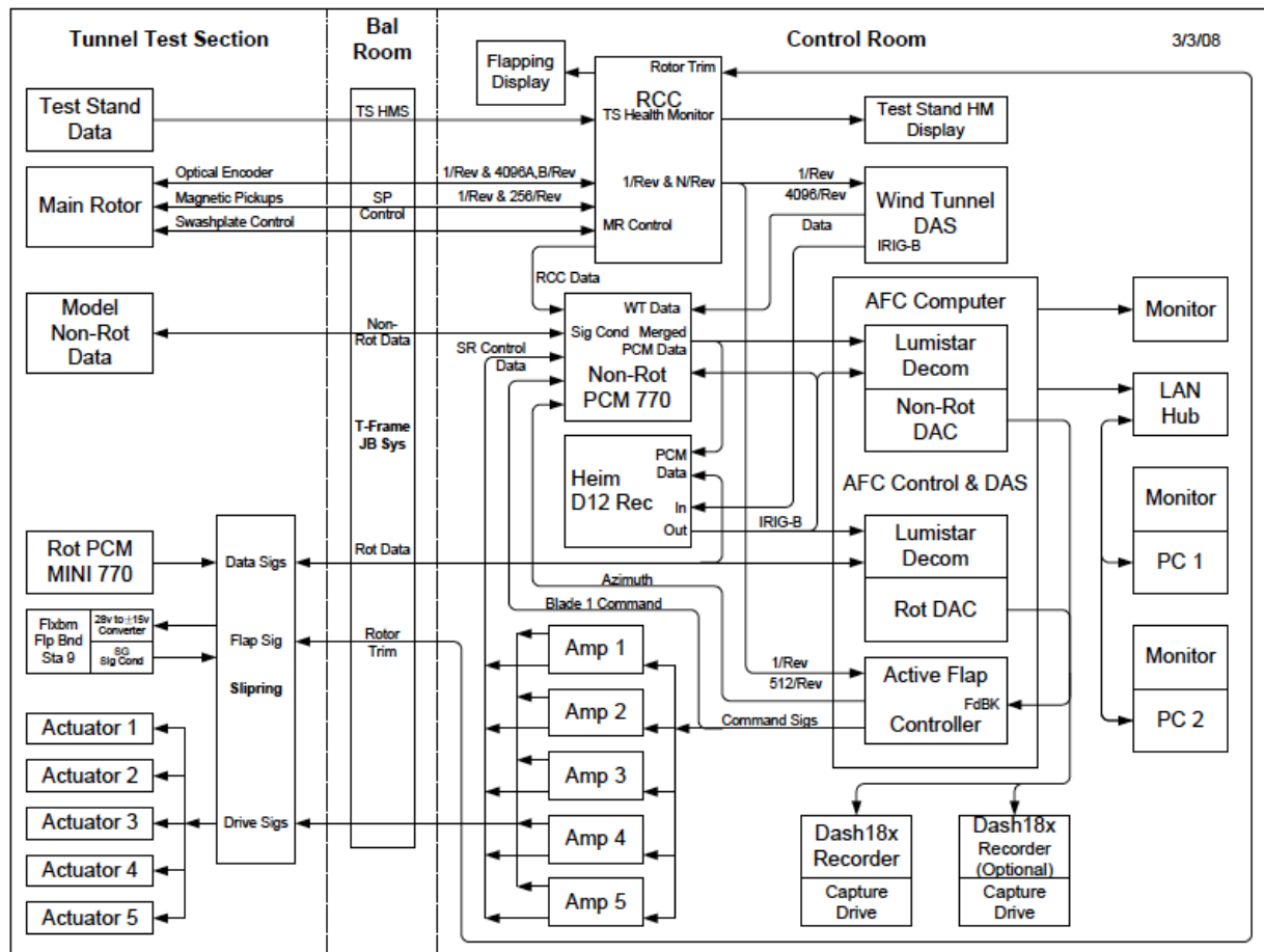
Figure 11: SMART rotor data/control system.
