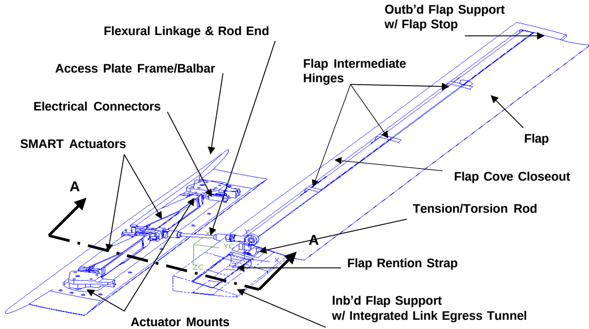
Figure 7a: Active flap components.
