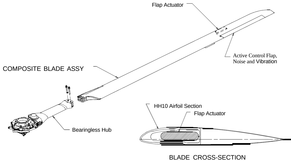
Figure 6: SMART rotor blade, trailing-edge flap, and actuator installation.
