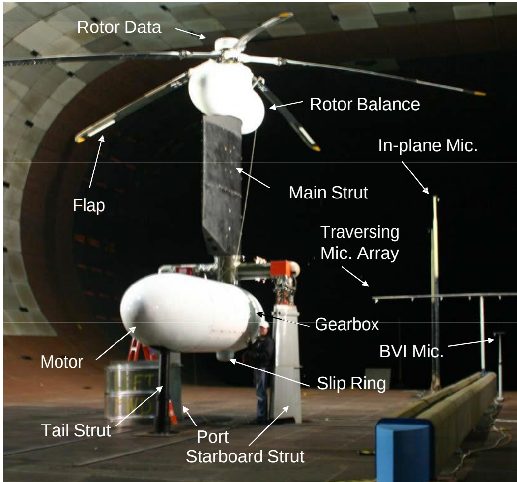
Figure 1e: SMART rotor in the NFAC 40- by 80-foot wind tunnel (looking upstream).
