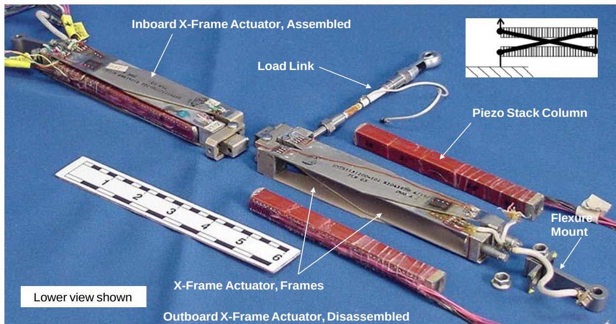
Figure 8: 2X-frame actuator, including piezoelectric stack columns.
