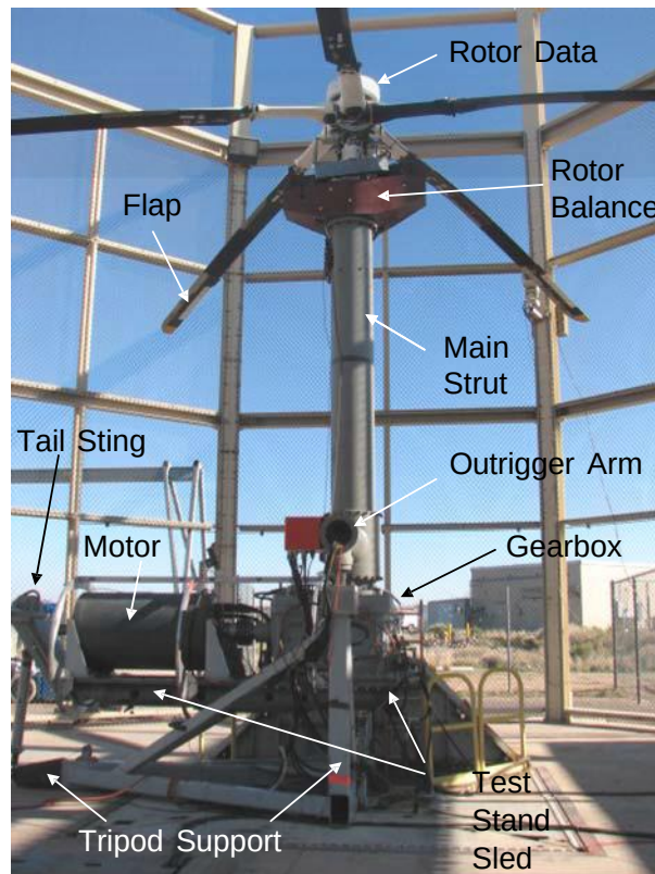
Figure 1b: System integration test at whirl tower showing LRTS test stand and SMART rotor setup (2008).
