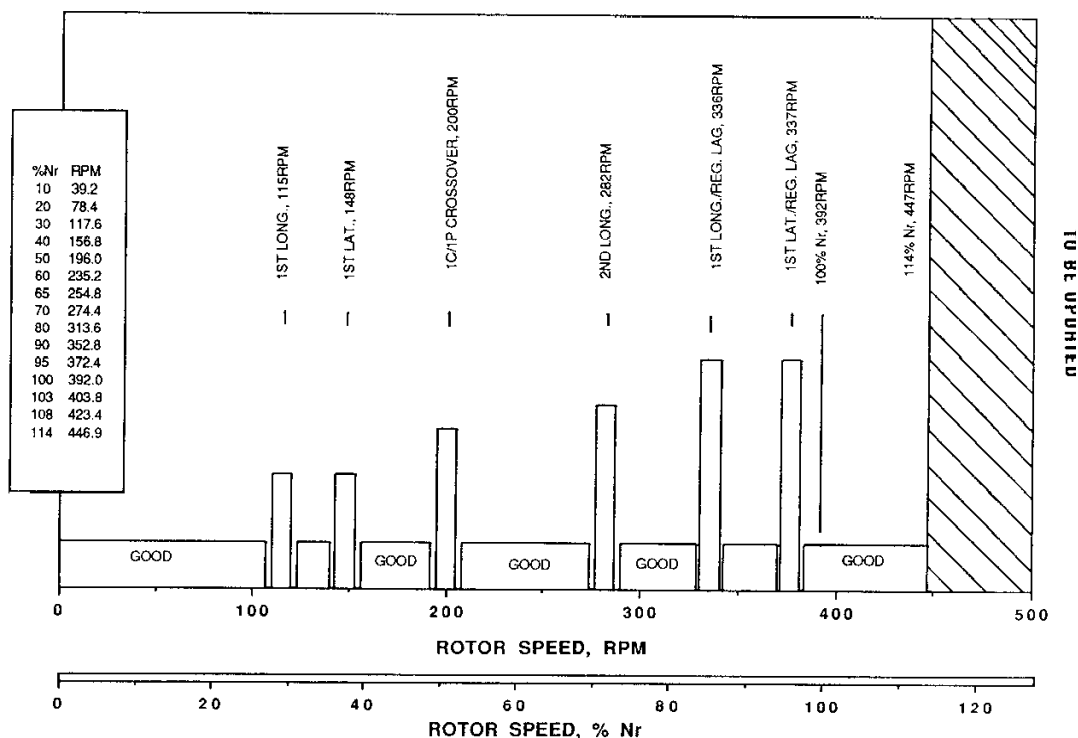
Figure 16: MDART full-scale rotor whirl tower test frequency run chart.
