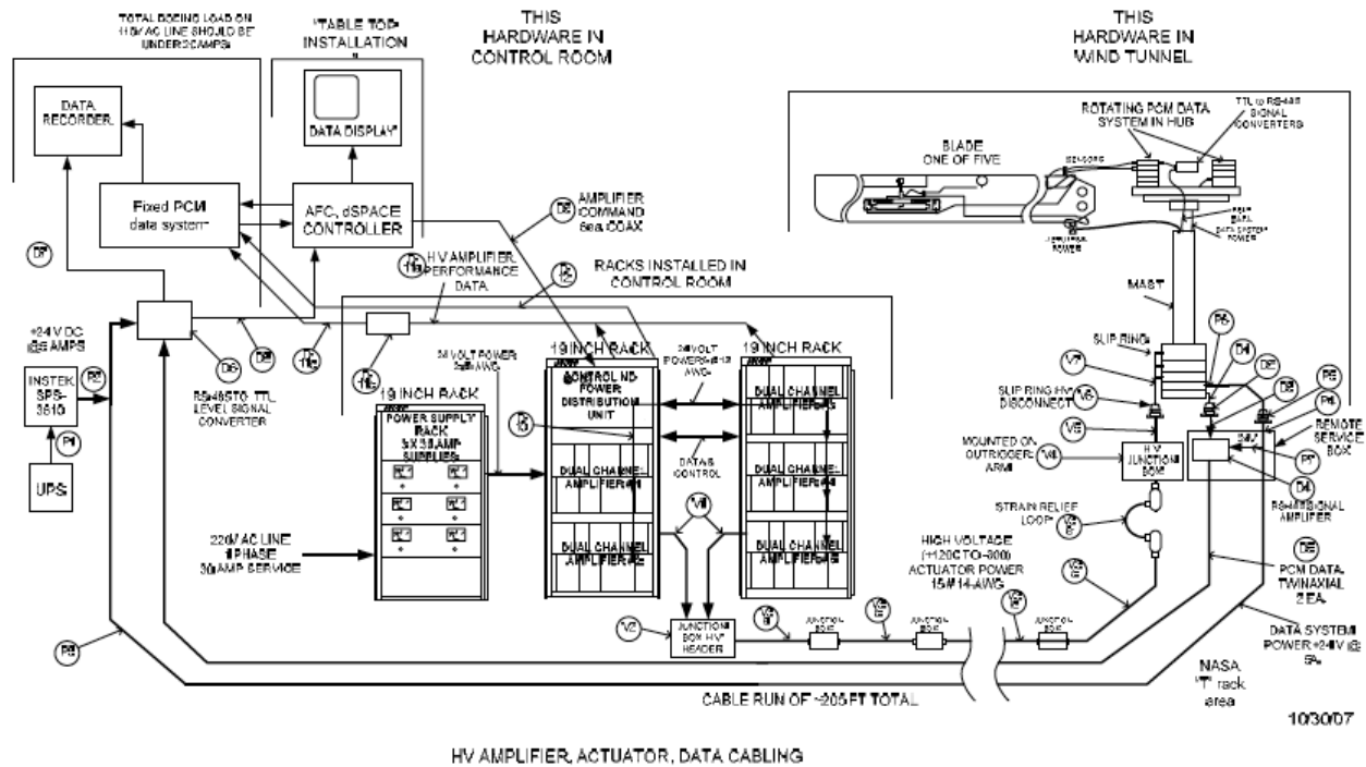
Figure 12: Data acquisition and active flap control system.
