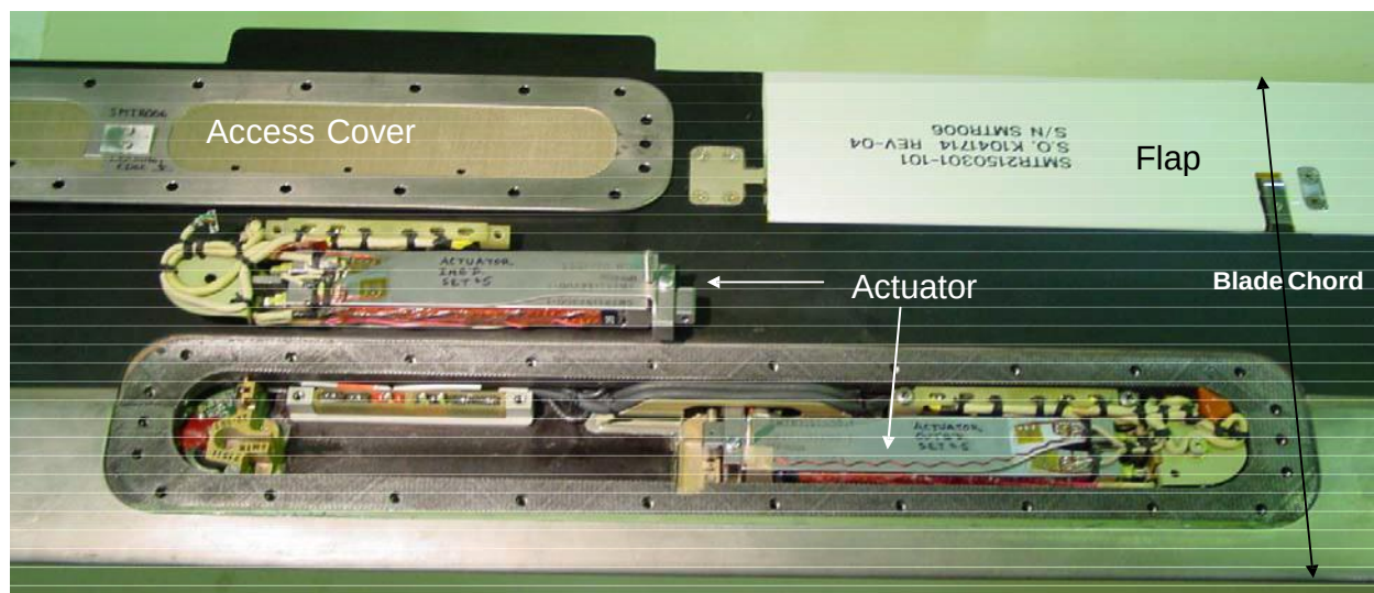
Figure 9: Blade, flap, and actuator close-up.
