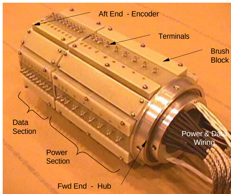
Figure 4: Slip ring for data (14 ch) and power (28V—4 ch, 1500V—8 ch).
