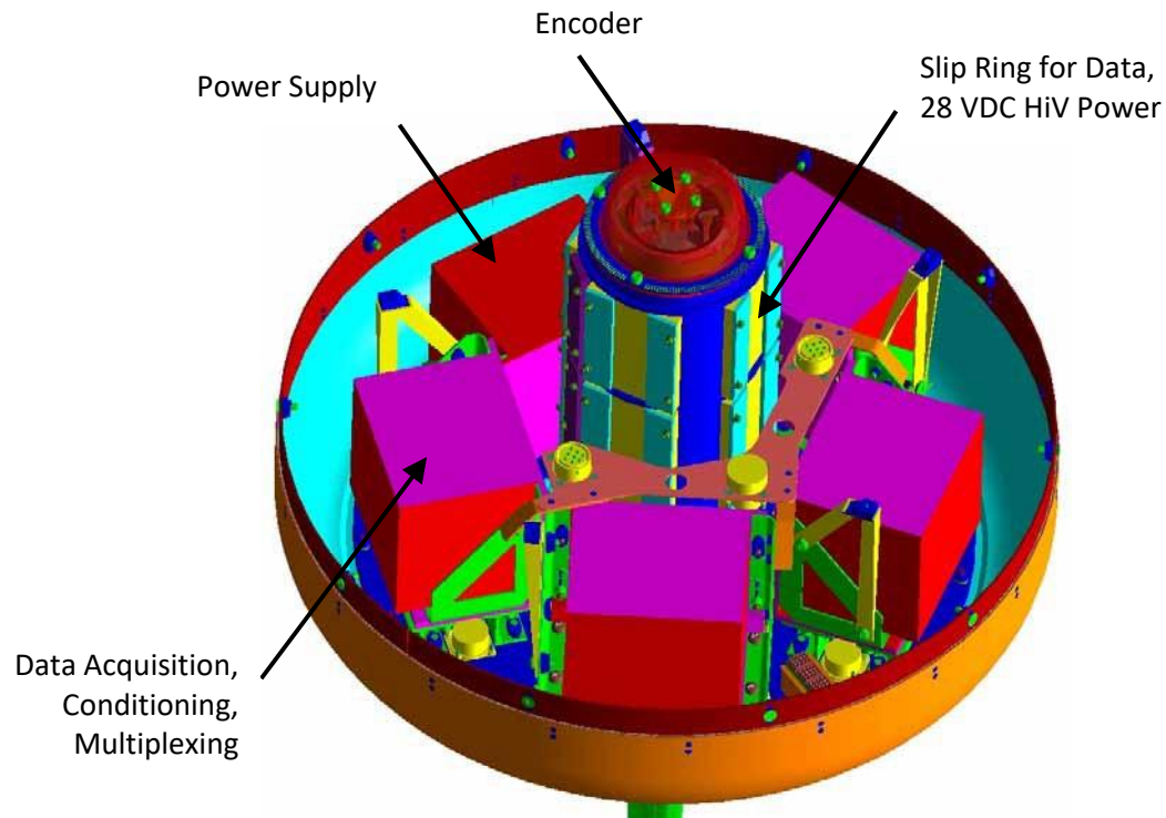
Figure 3: Hub-mounted data/power transfer system (note: in wind tunnel the slip ring and encoder are mounted below the transmission).
