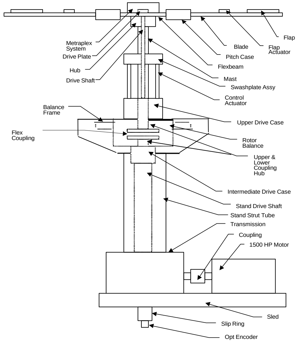
Figure 2a: Schematic of SMART rotor and test stand components.
