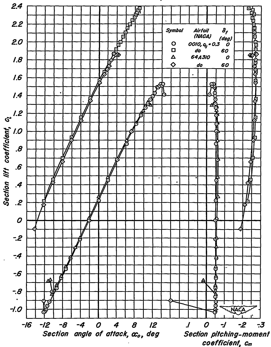
(a) Smooth airfoils; Reynolds number, 3.7 \times 10^6 .
