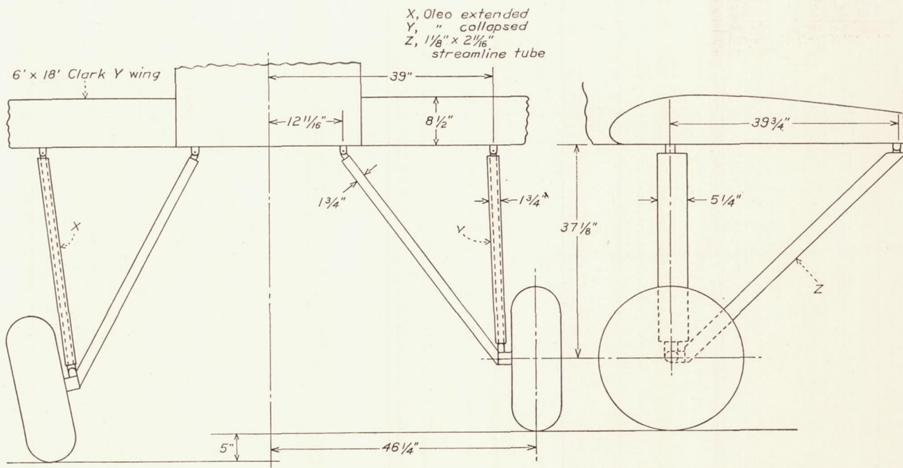
FIGURE 39.—Drag and dimensions of gear 14c. Drag of gear at 100 m.p.h. (oleos extended) : 8.50–10 wheels, 41.0 pounds.
