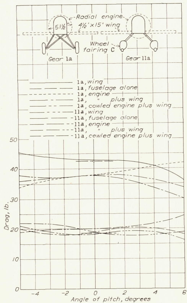
FIGURE 41.—Drag at 100 m.p.h. of landing gears 1a and 11a measured in the presence of the 4\frac{1}{2} - by 15-foot wing and the engine.
