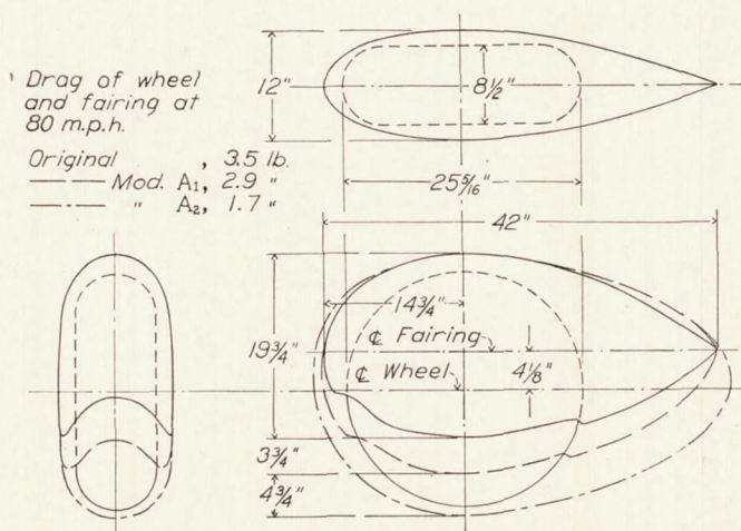
FIGURE 4.—Drag and dimensions of wheel fairing A.
