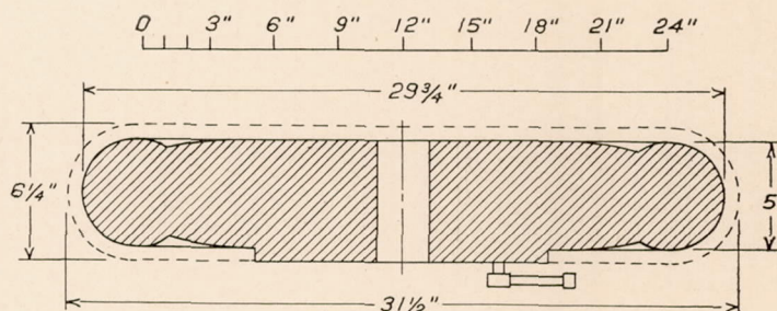
30 by 5 disk wheel and high-pressure tire. 30 by 5 disk wheel and 32 by 6 high-pressure tire. (dotted) Drag=5.9 lb. (30 by 5) at 80 m.p.h. Drag=6.9 lb. (32 by 6) at 80 m.p.h.
