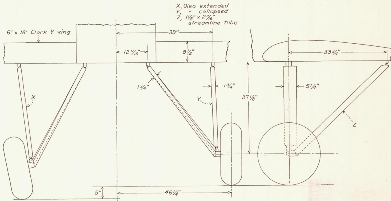
FIGURE 38.—Drag and dimensions of gear 14b. Drag of gear at 100 m.p.h. (oleos extended) : 8.50–10 wheels, 41.0 pounds.
