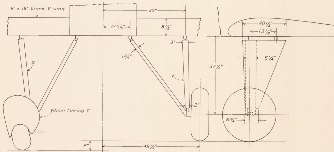
FIGURE 37.—Drag and dimensions of gear 14a.
