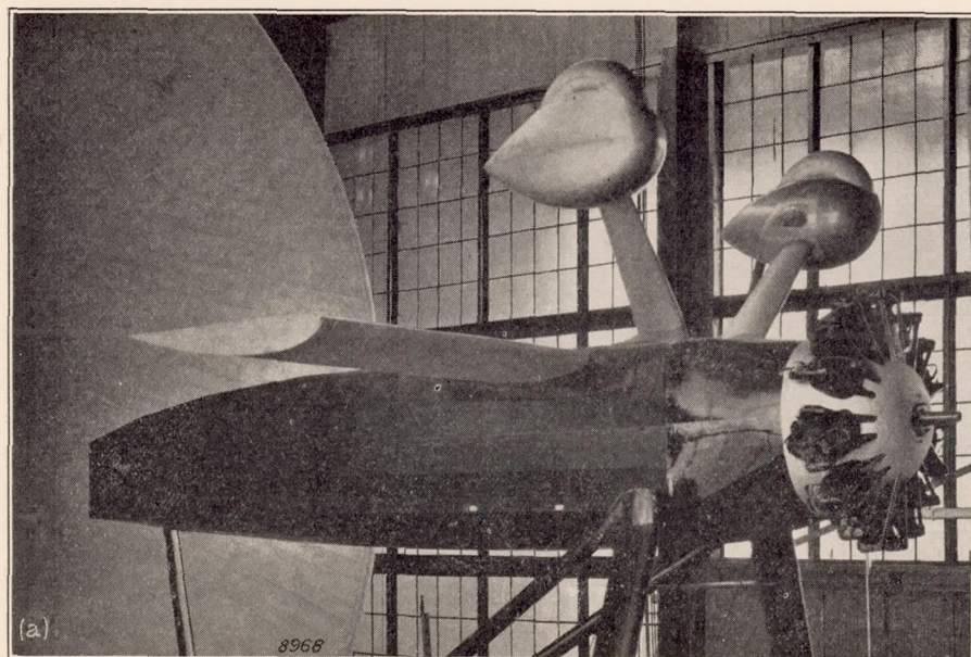
a. Landing gear 11a mounted on the fuselage with the 4\frac{1}{2} - by 15-foot wing and the engine.
