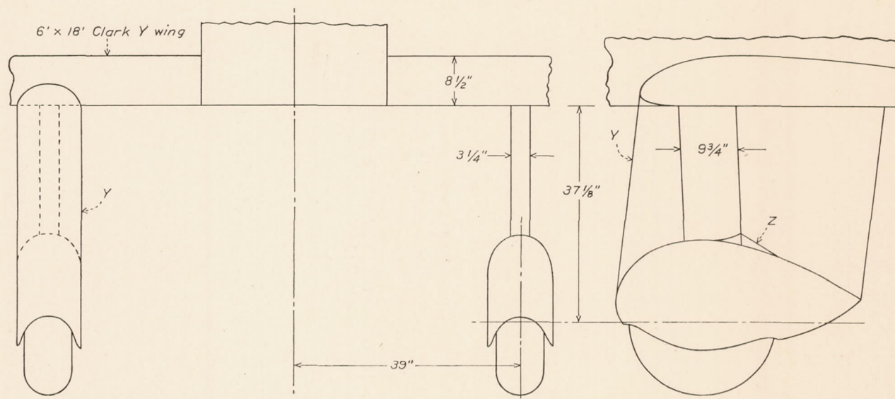
FIGURE 36.—Drag and dimensions of gear 13.
