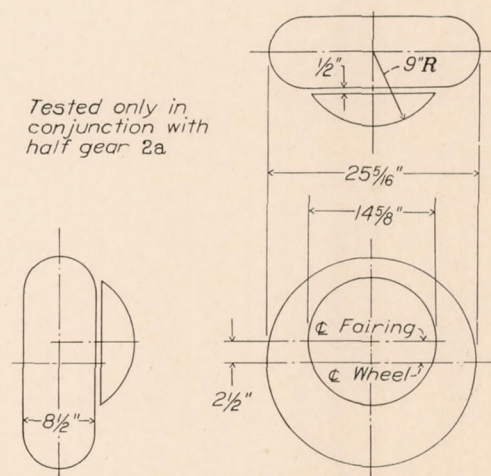
FIGURE 9.—Dimensions of wheel fairing F.
