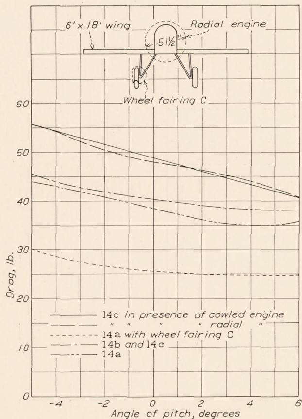
FIGURE 44.—Drags at 100 m.p.h. of gears 14a, 14b, and 14c mounted on fuselage and the 6- by 18 foot wing.
