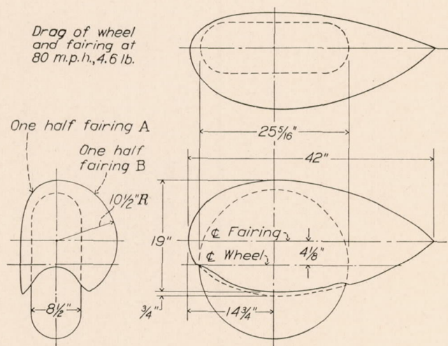
FIGURE 6.—Drag and dimensions of wheel fairing C.
