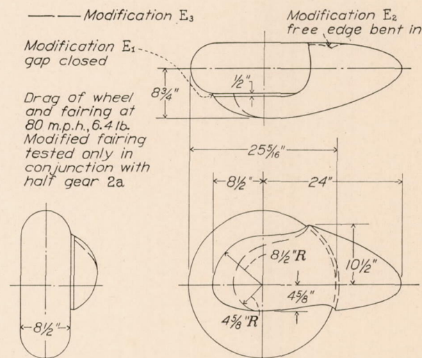
FIGURE 8.—Drag and dimensions of wheel fairing E.
