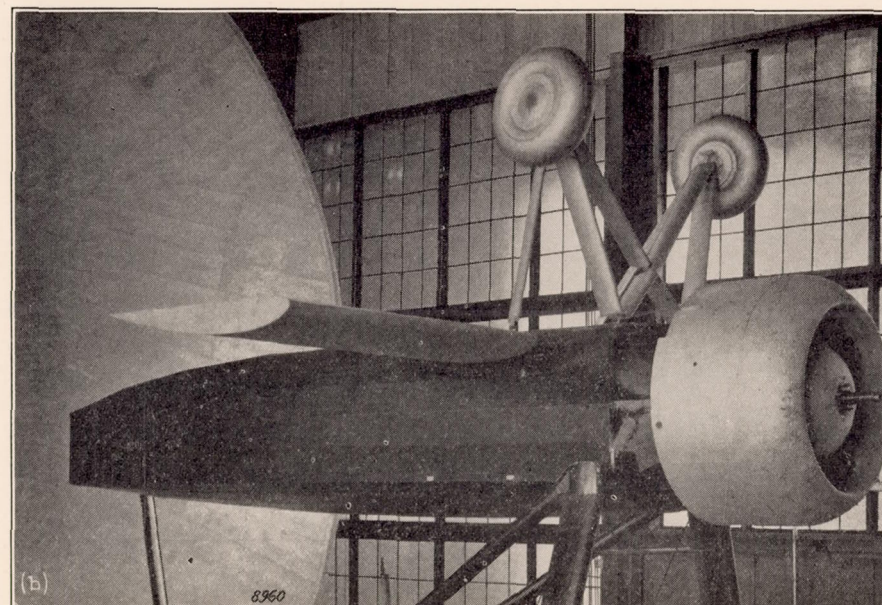
b. Landing gear 1a mounted on the fuselage with the 4\frac{1}{2} - by 15-foot wing and the cowled engine.
