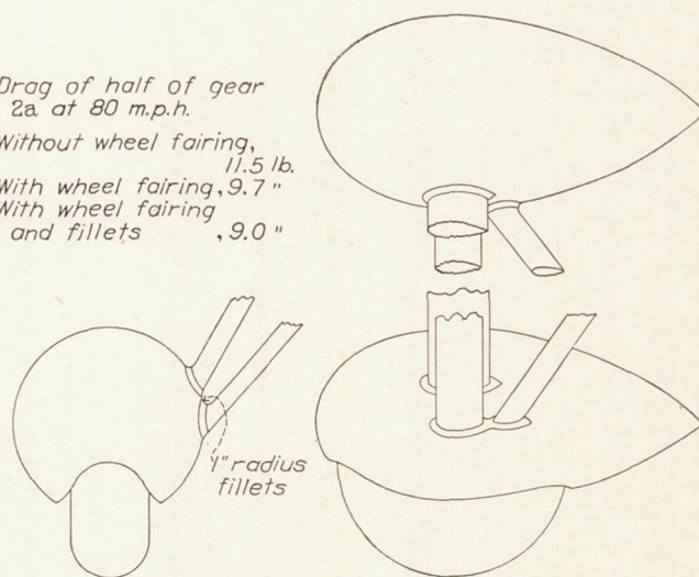
FIGURE 12.—Drag of one-half gear 2a with wheel fairing B.
