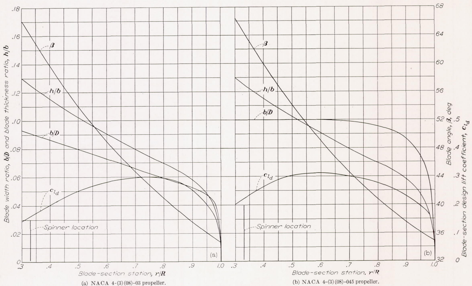
FIGURE 2.—Blade-form curves.
