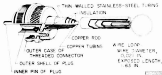
(B) CONSTRUCTION DETAILS OF WIRE-LOOP ASSEMBLY AND SUPPORTING-STRUT ASSEMBLY
