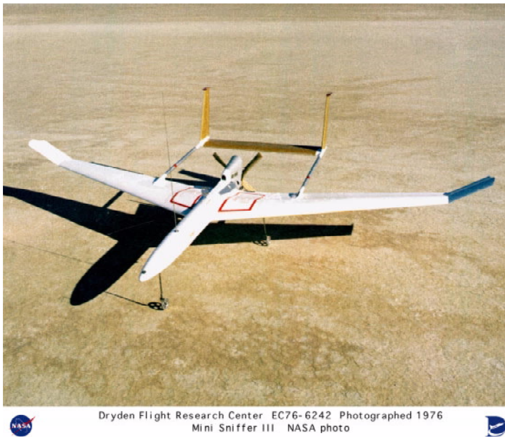
Figure 9 Mini-Sniffer Aircraft
