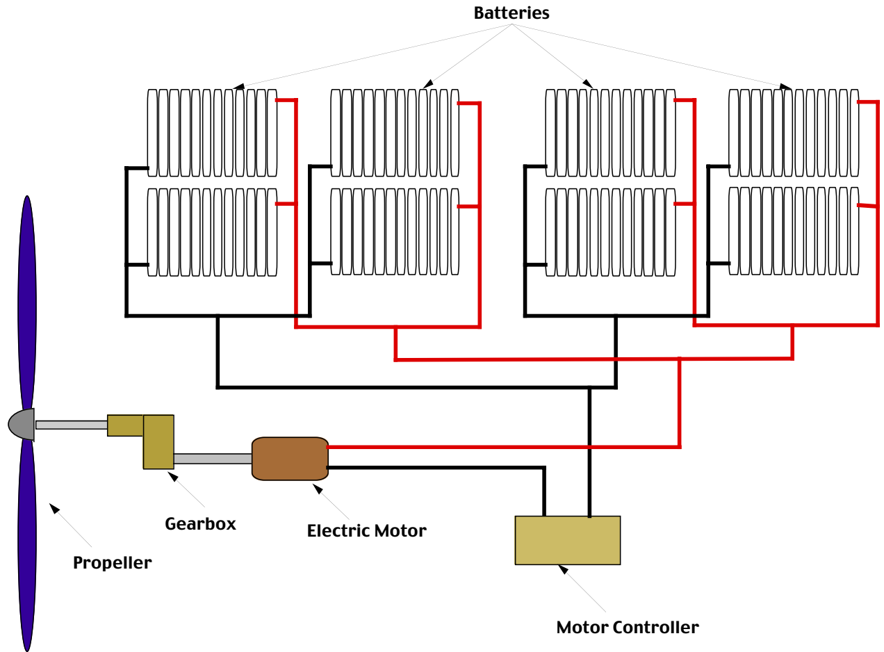
Figure 7 Battery Powered Propulsion System
