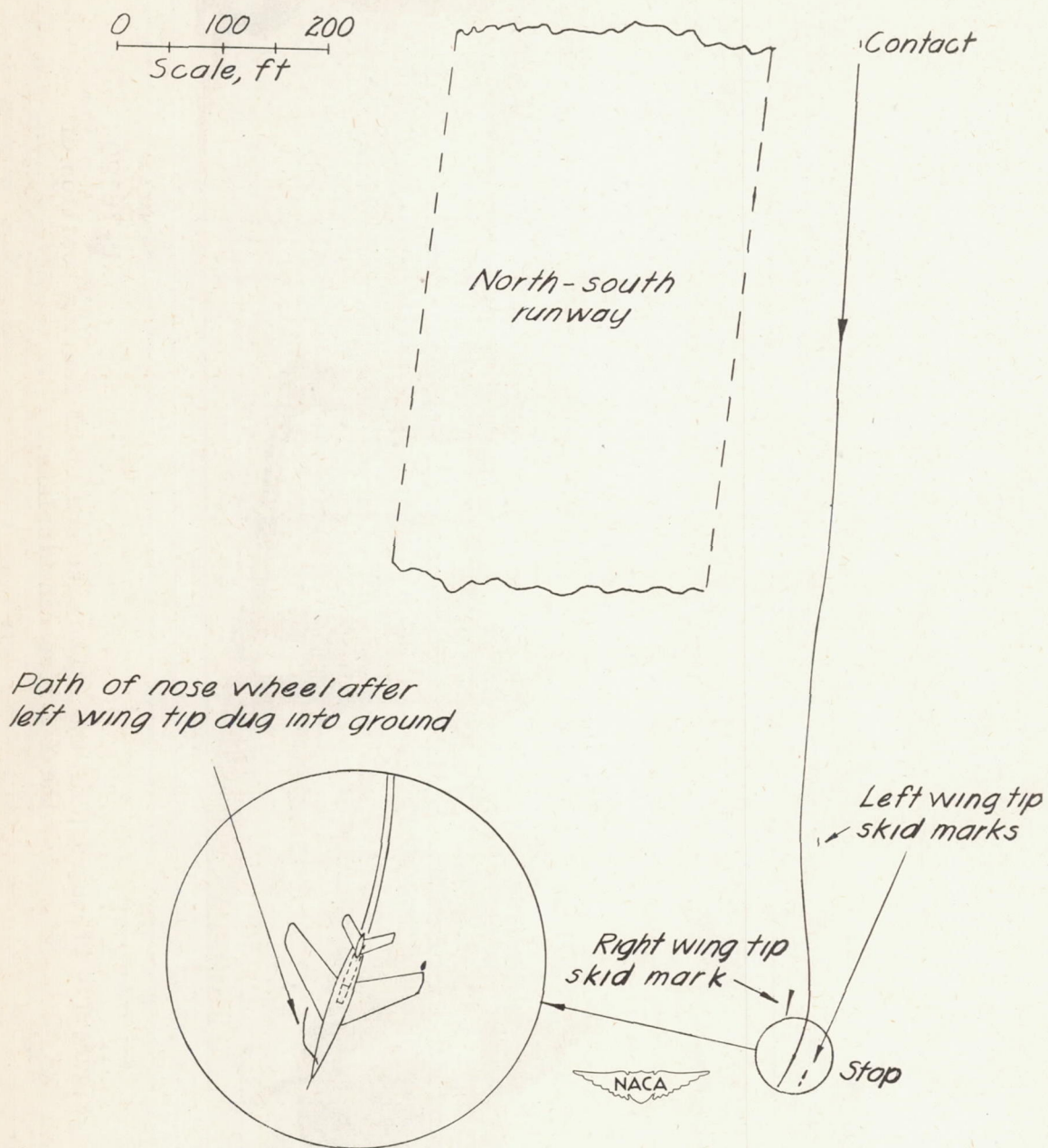
Figure 6.- Ground path of the Bell X-2 research airplane.
