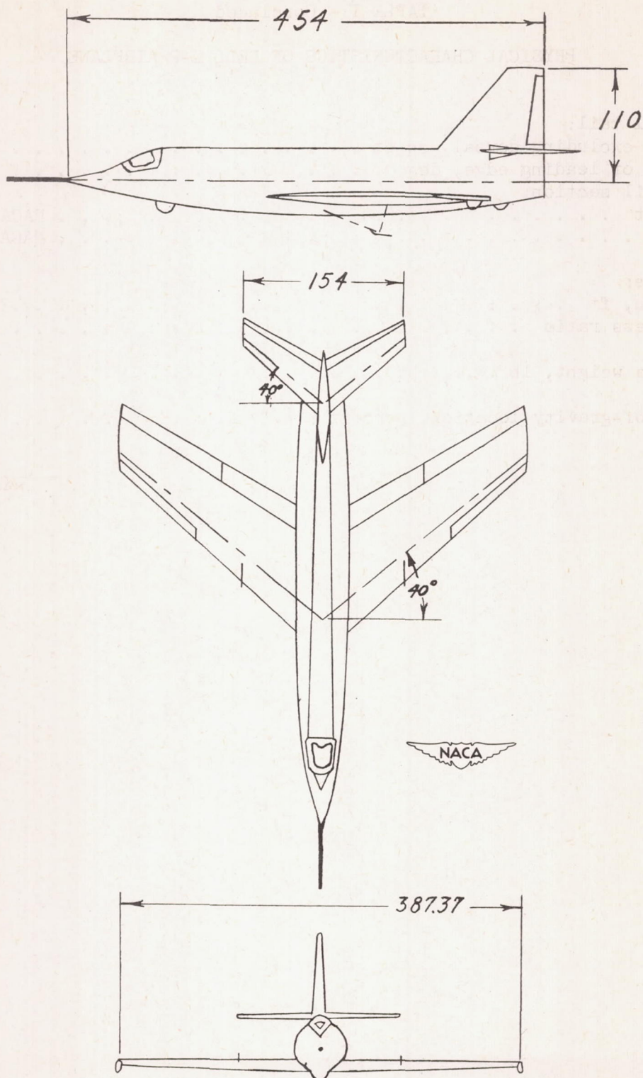
Figure 1.- Three-view drawing of the Bell X-2 research airplane. All dimensions are in inches.
