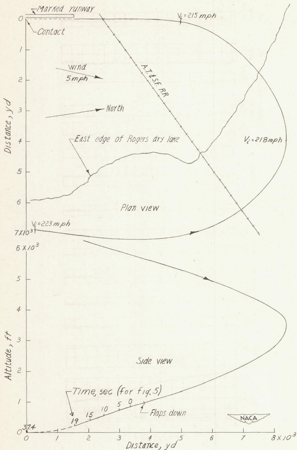
Figure 4.- Landing approach pattern of the Bell X-2 research airplane.
