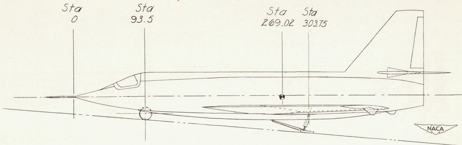
Figure 2.- Drawing showing the landing-skid and nose-wheel installation on the Bell X-2 research airplane.
