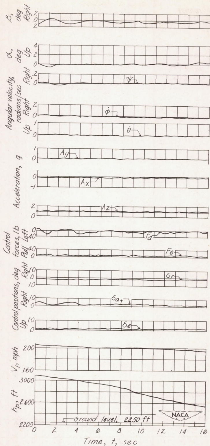
Figure 5.- Time history of landing of Bell X-2 research airplane. Stabilizer setting, 2.2^\circ leading edge down; weight, 10,337 pounds.
