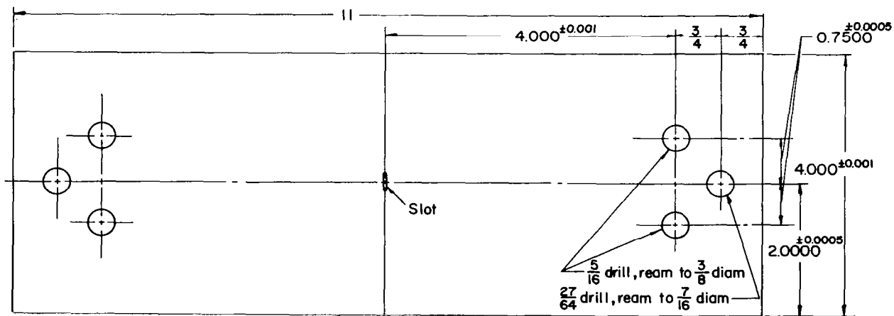
c. Center-Notched Specimens
