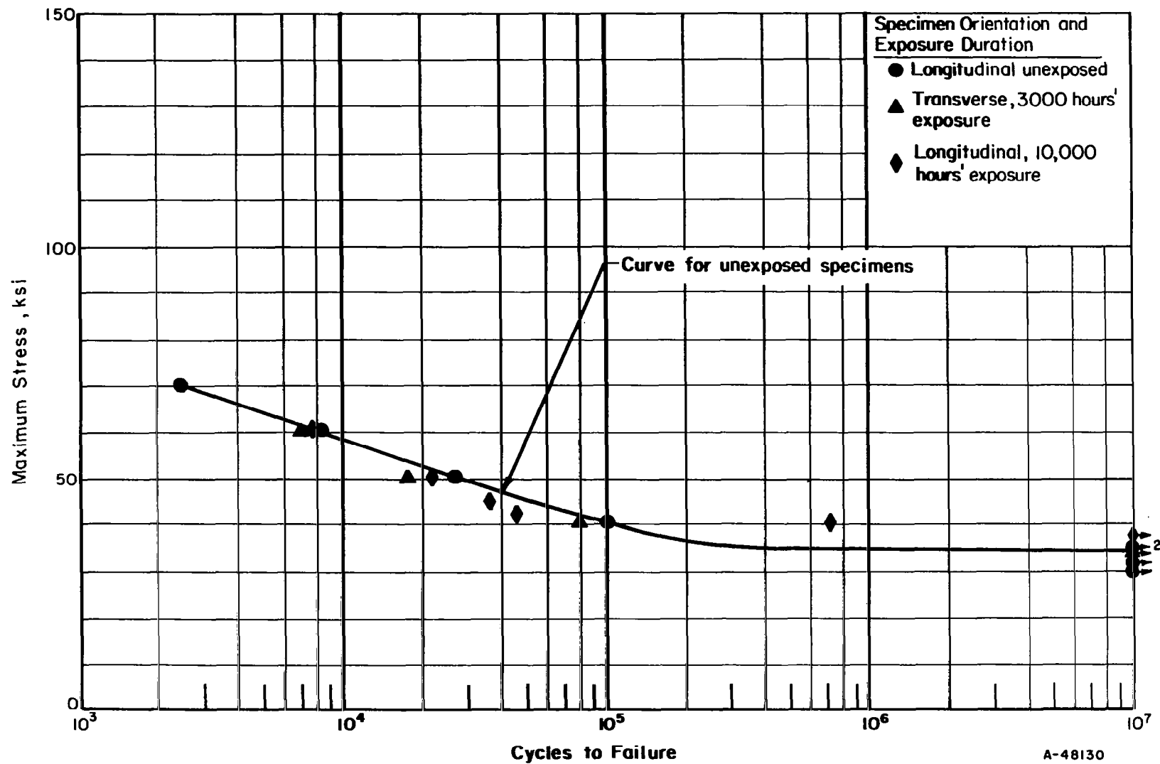
FIGURE 35. EFFECT OF STRESSED EXPOSURE ON FATIGUE BEHAVIOR OF NOTCHED ( K_t = 4.0 ) Ti-8Al-1Mo-1V ALLOY AT 550 F AND 25-KSI MEAN STRESS
