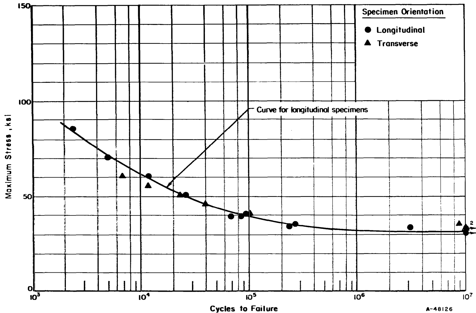
FIGURE 31. EFFECT OF SPECIMEN ORIENTATION ON FATIGUE BEHAVIOR OF UNEXPOSED NOTCHED ( K_t = 4.0 ) Ti-8Al-1Mo-1V ALLOY AT ROOM TEMPERATURE AND 25-KSI MEAN STRESS
