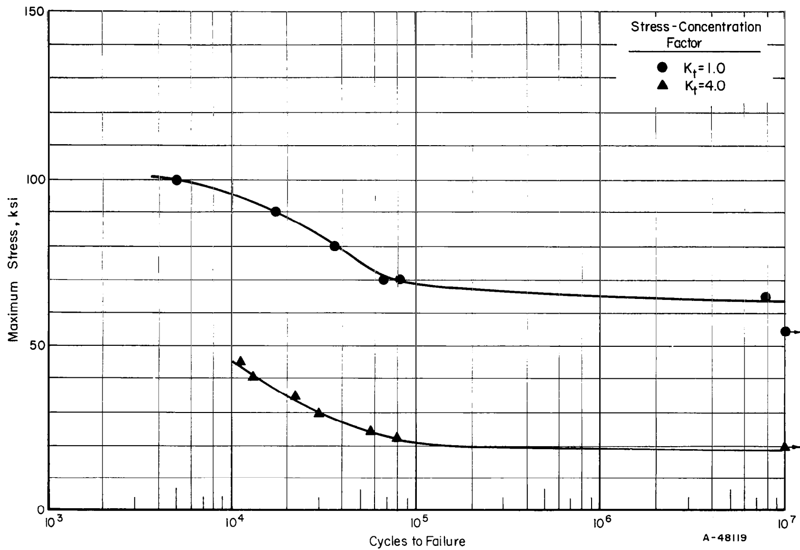
FIGURE 24. FATIGUE BEHAVIOR OF UNEXPOSED LONGITUDINAL Ti-8Al-1Mo-1V ALLOY SPECIMENS AT 550 F AND ZERO MEAN STRESS
