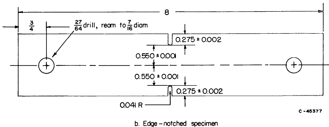
FIGURE 1. FATIGUE SPECIMENS
