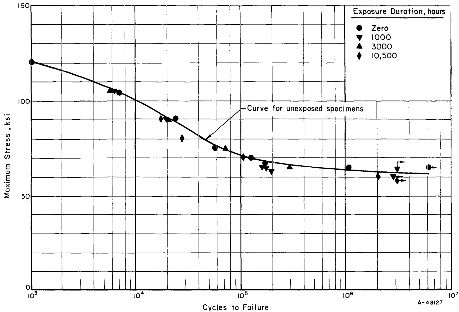
FIGURE 32. EFFECT OF STRESSED EXPOSURE ON FATIGUE BEHAVIOR OF NOTCHED ( K_t = 4.0 ) AM-350 STAINLESS STEEL AT -110^\circ\text{F} AND 40-KSI MEAN STRESS
